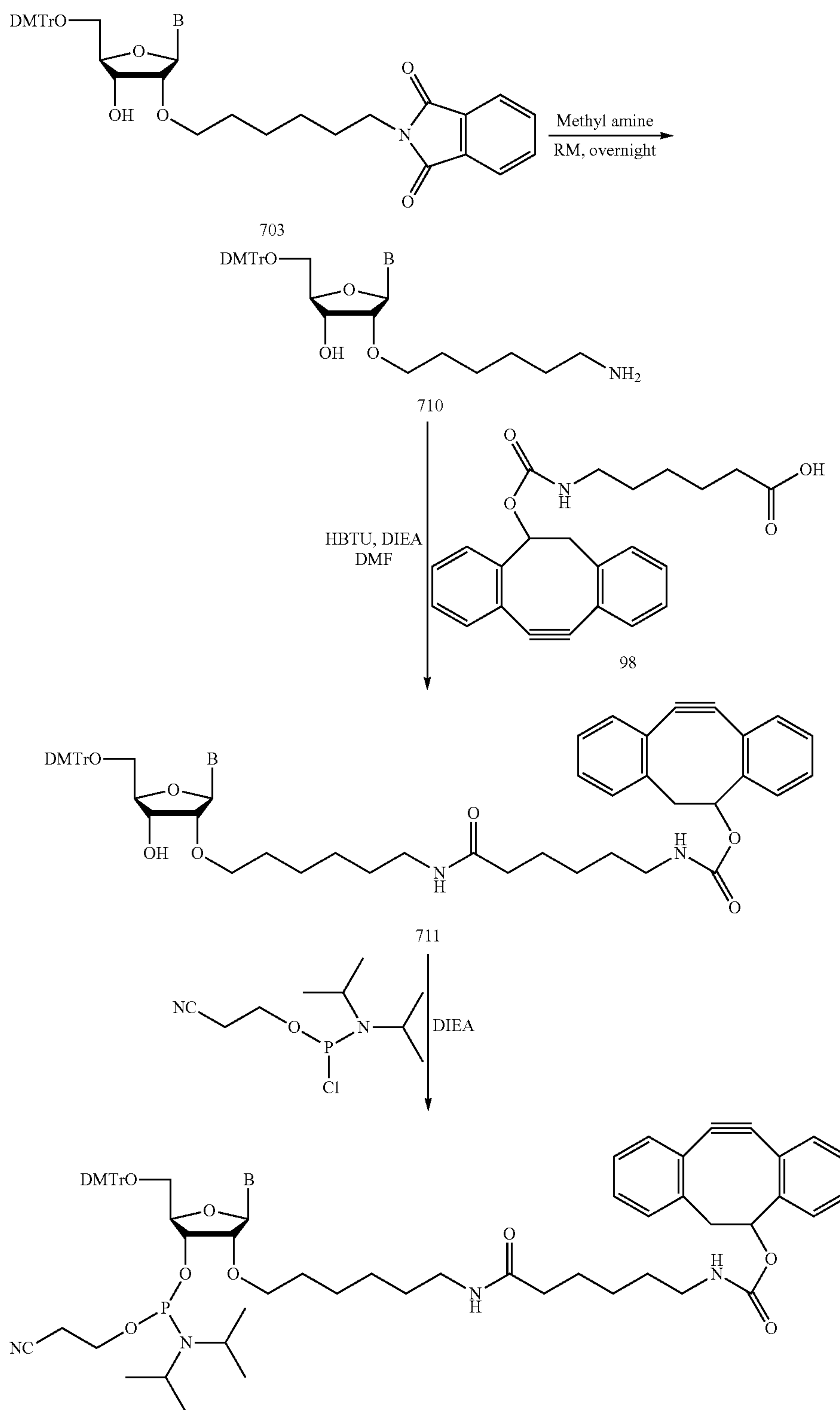
Scheme 14
