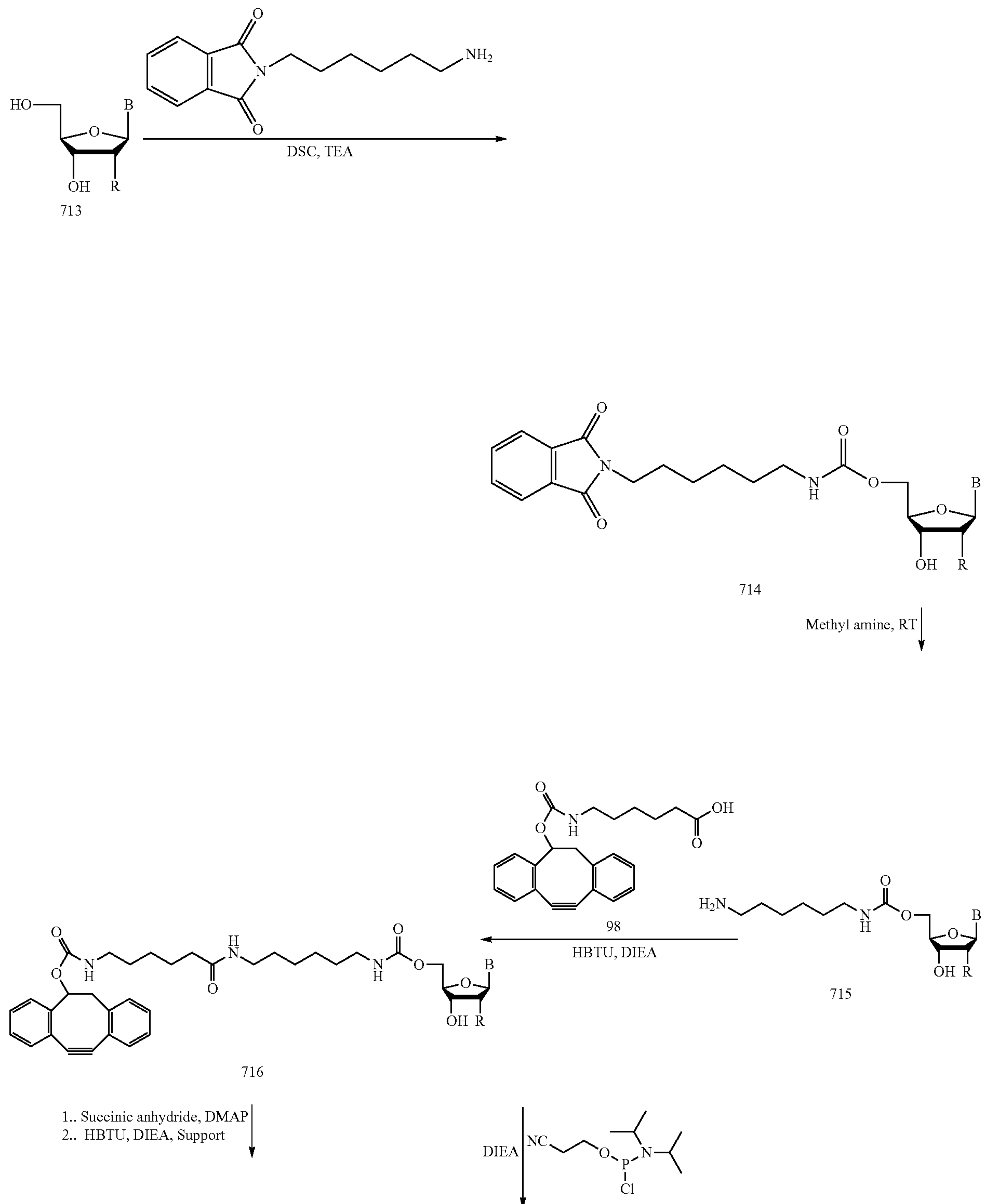
Scheme 15
