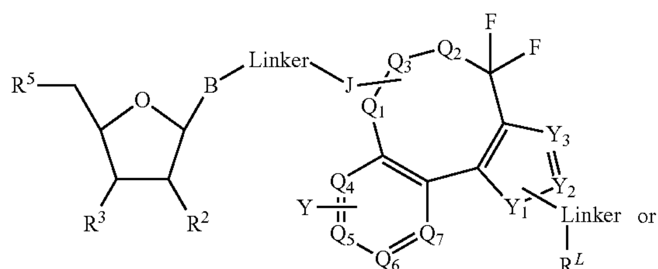
Formula (XVa)
