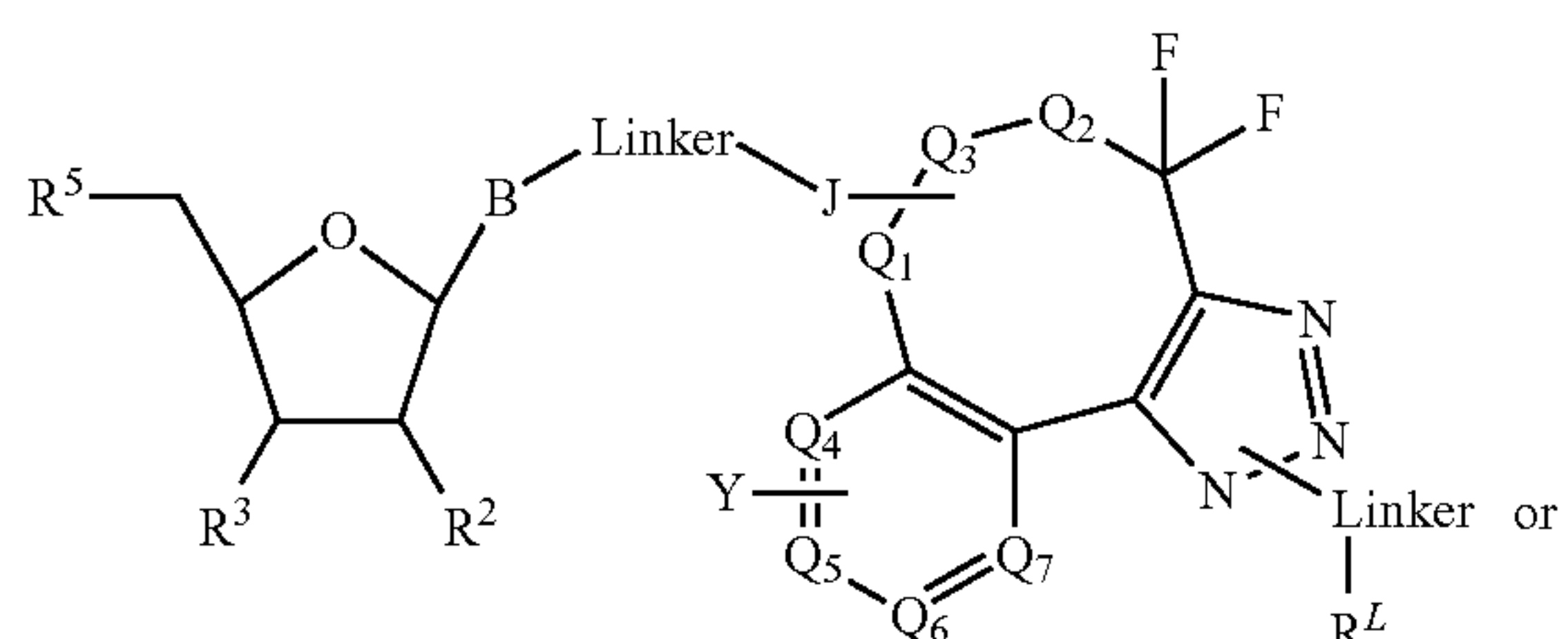
Formula (XVIa)
