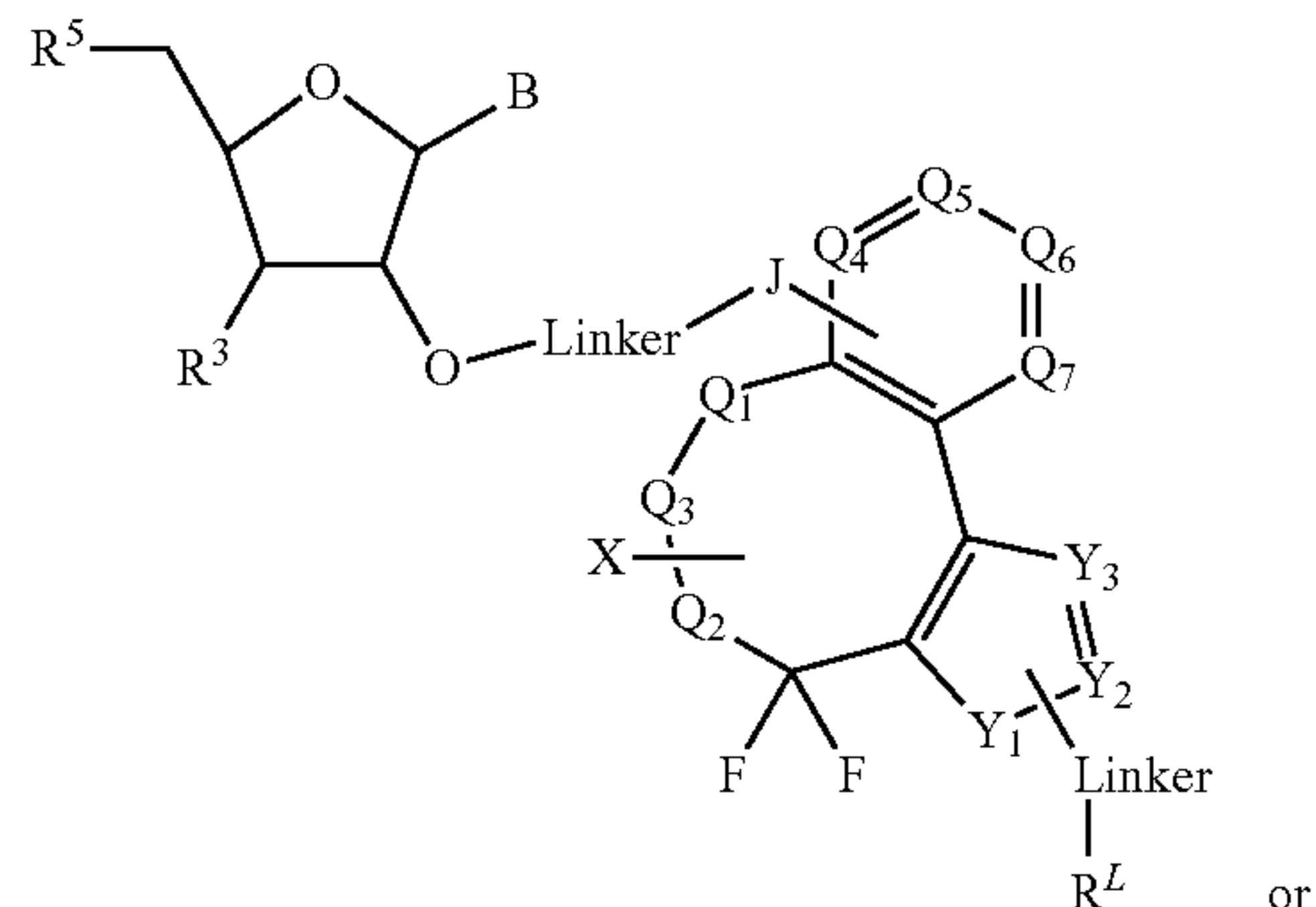
Formula (Vb)
