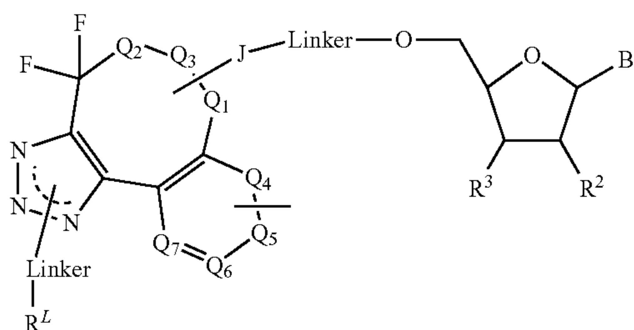
Formula (Xb)
