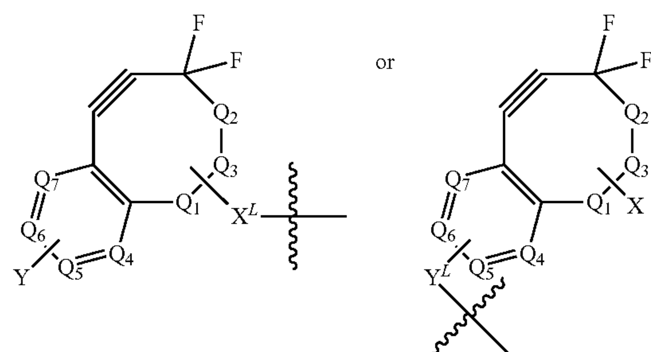
Formula (XI)
