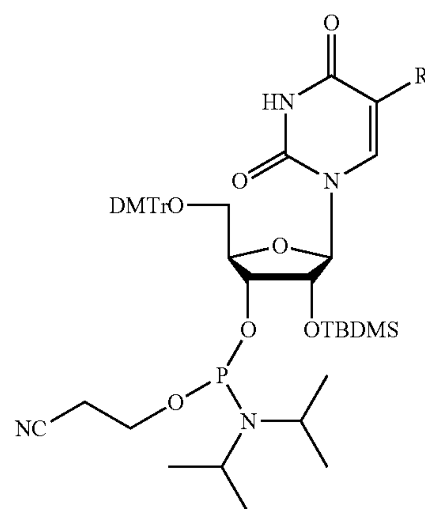
Scheme 17
