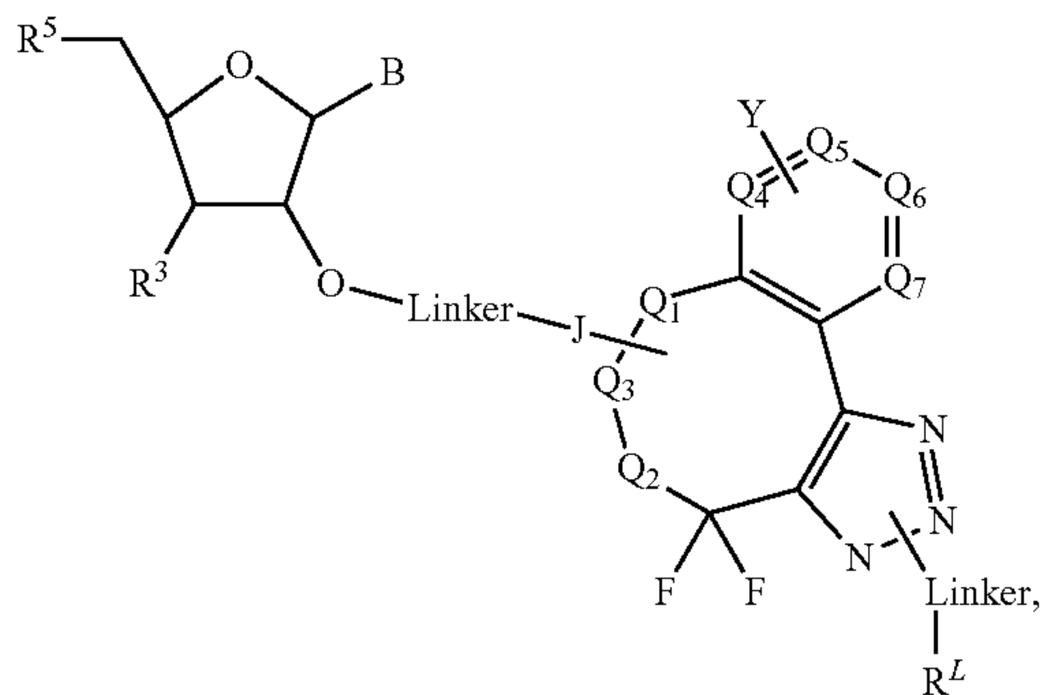
Formula (VIb)
