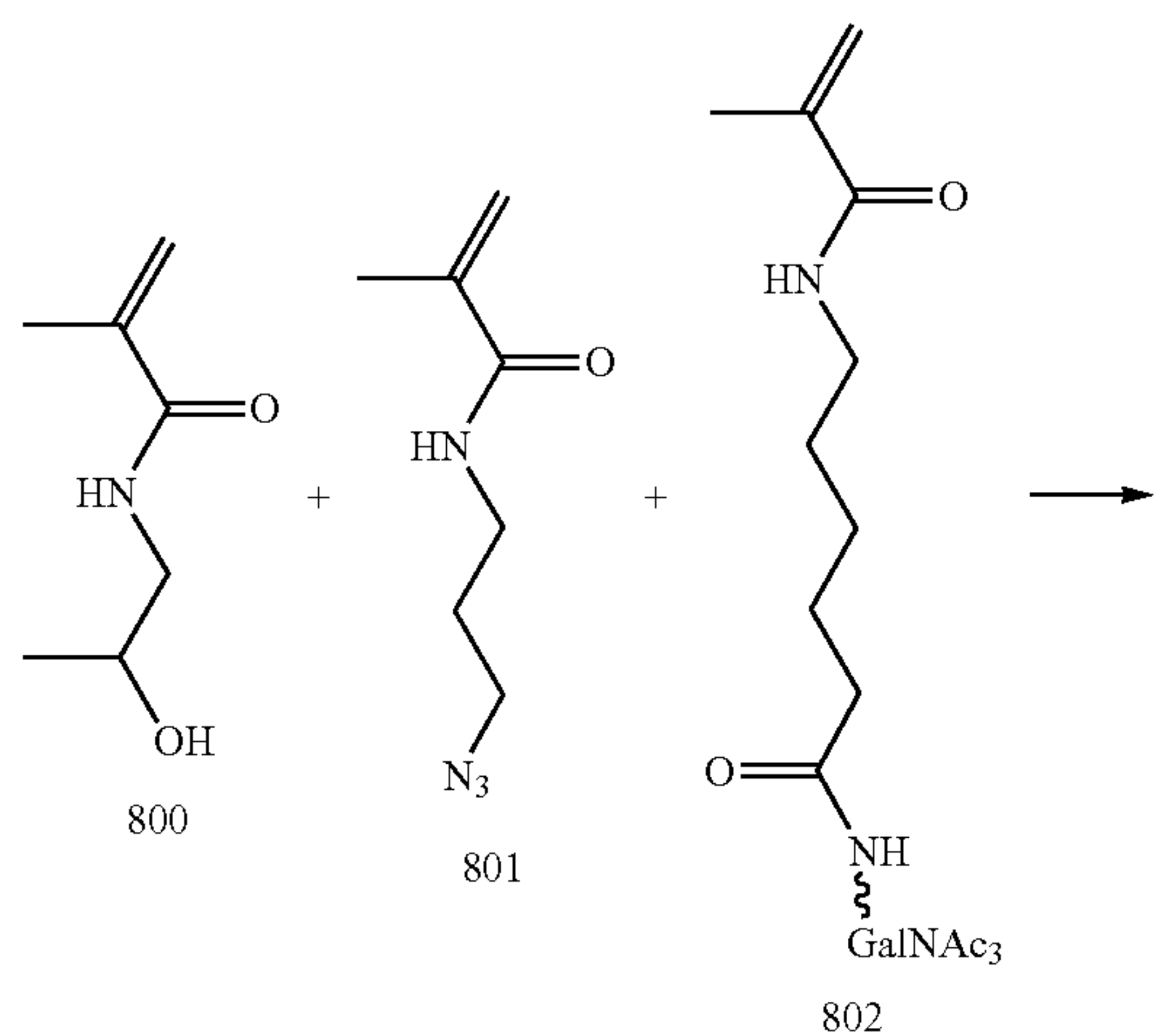
Scheme 21
