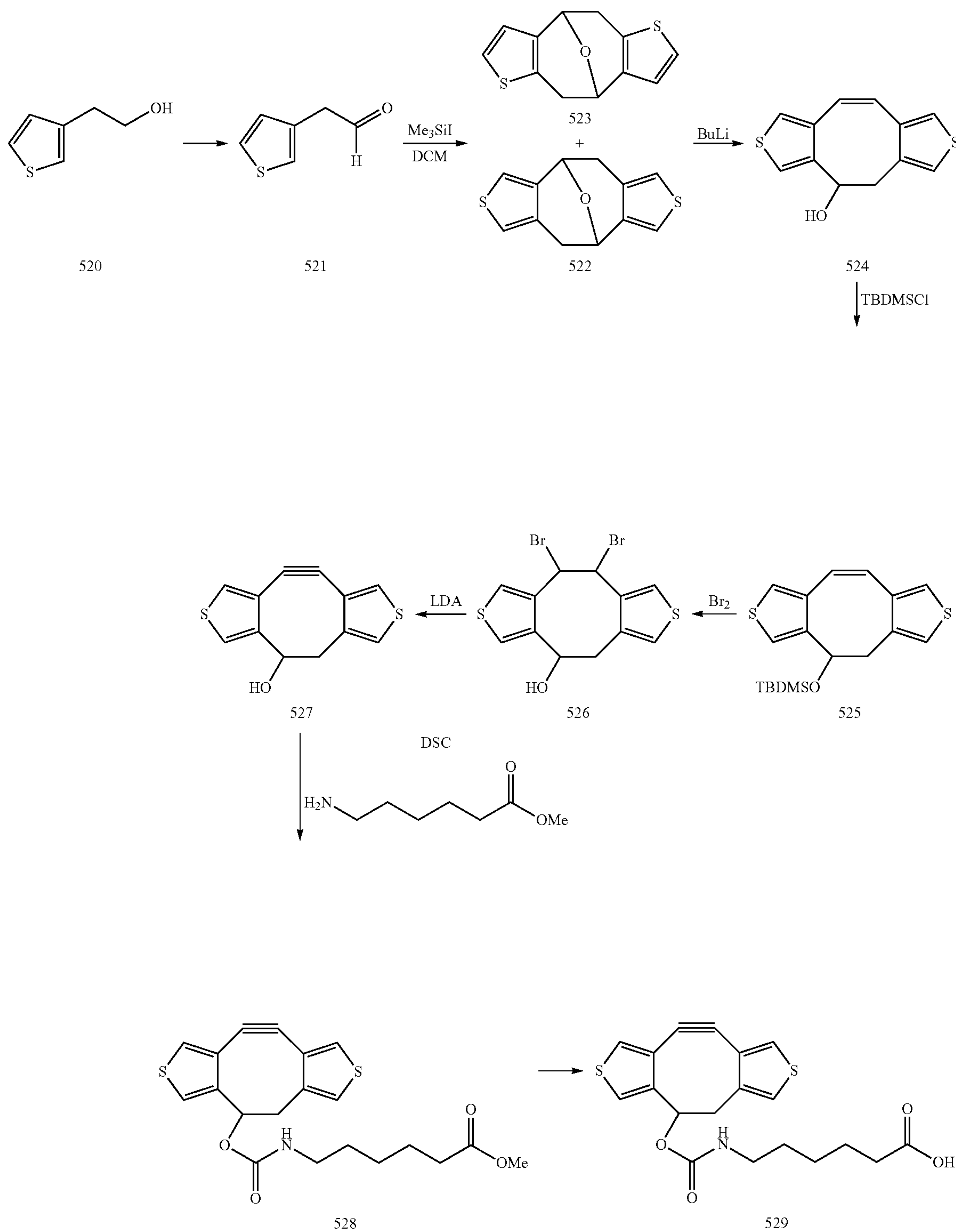
Scheme 6
