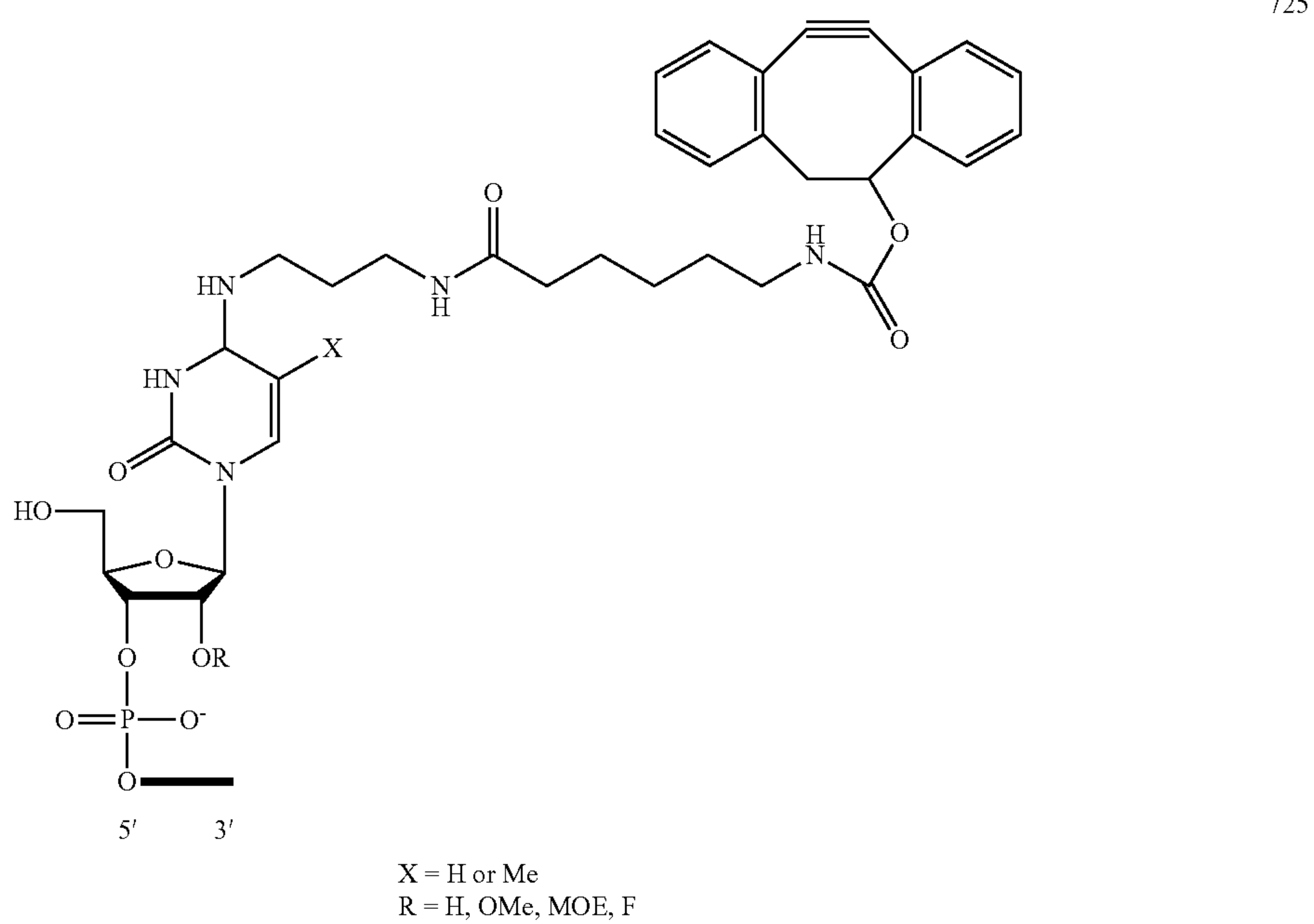
Scheme 19
