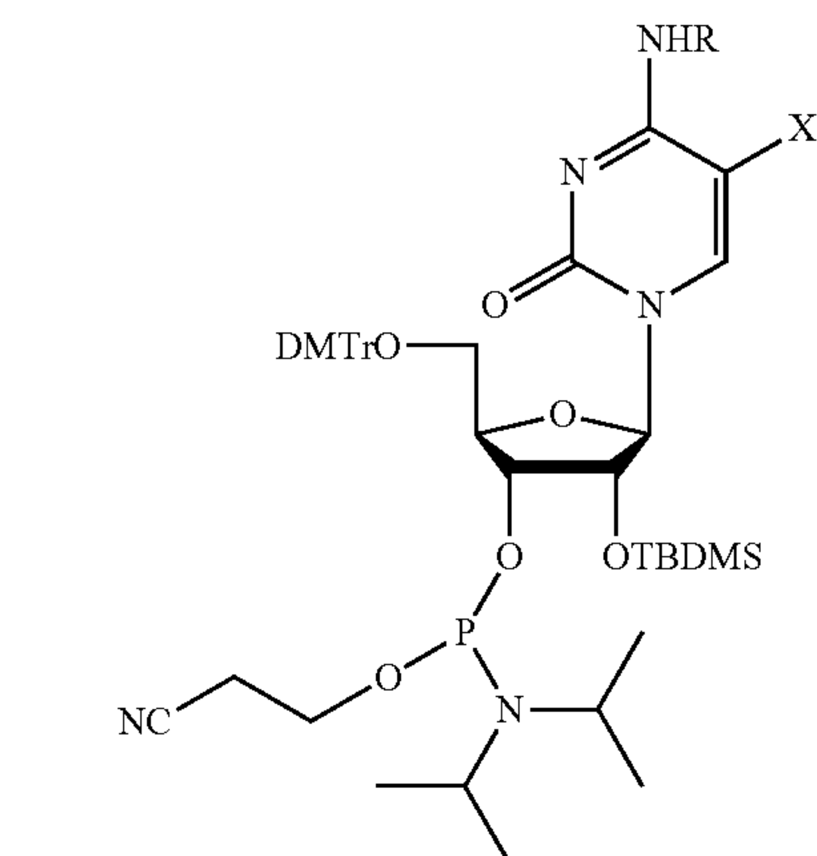
Scheme 16
