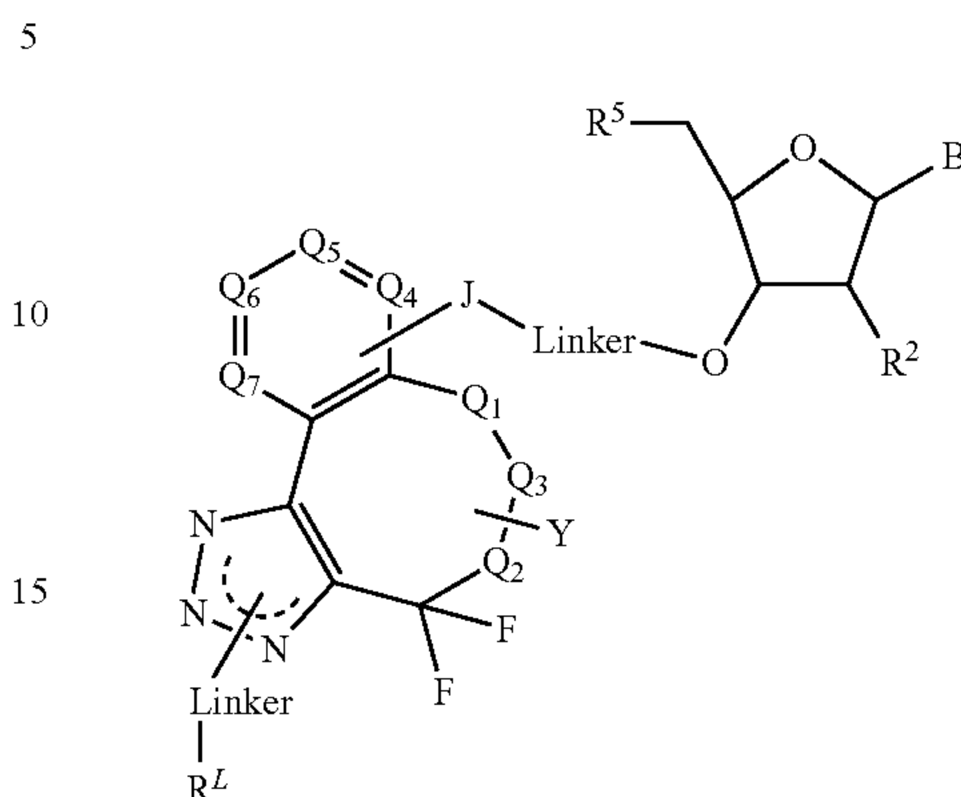
Formula (VIIIa)
