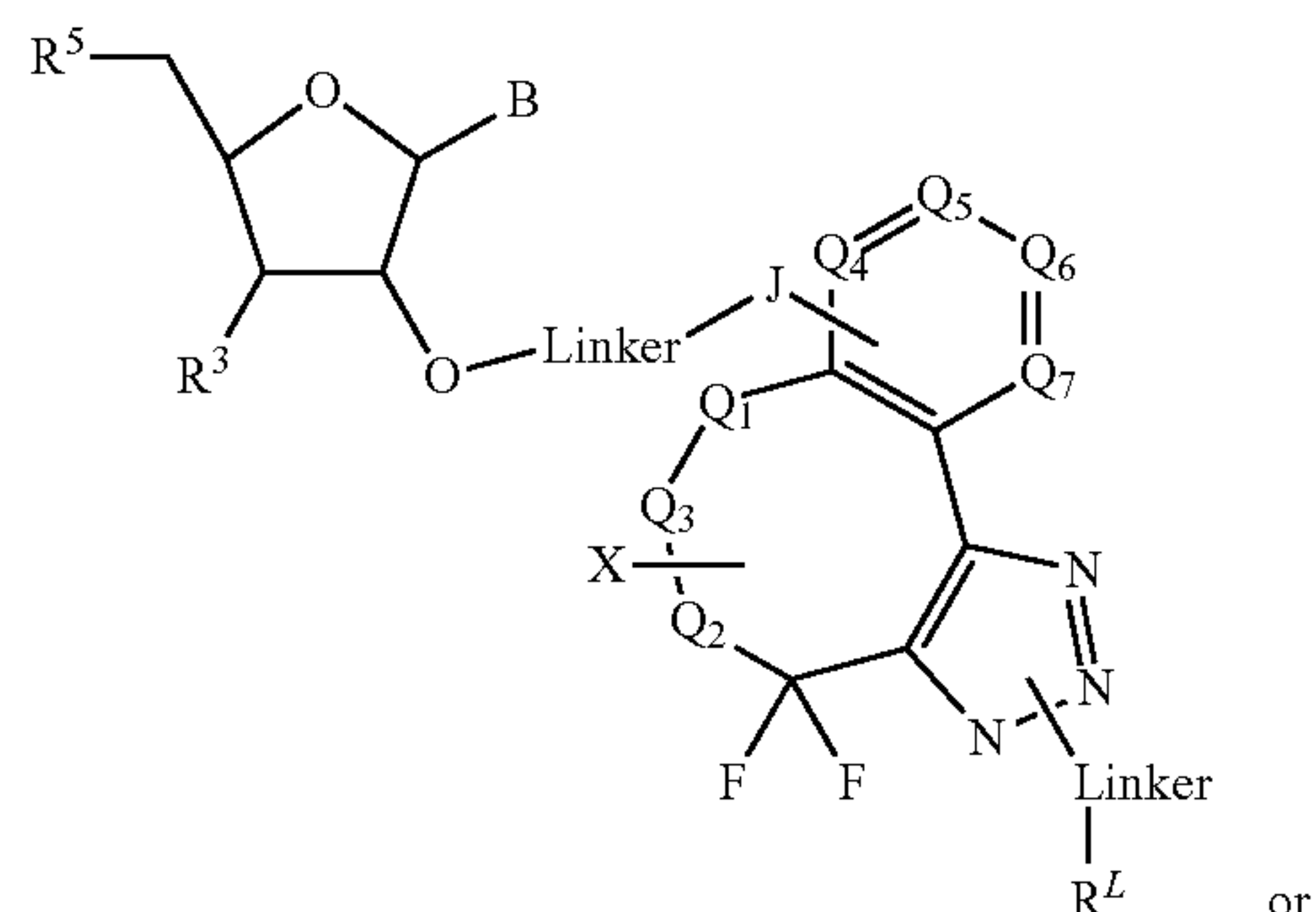
Formula (VIa)
