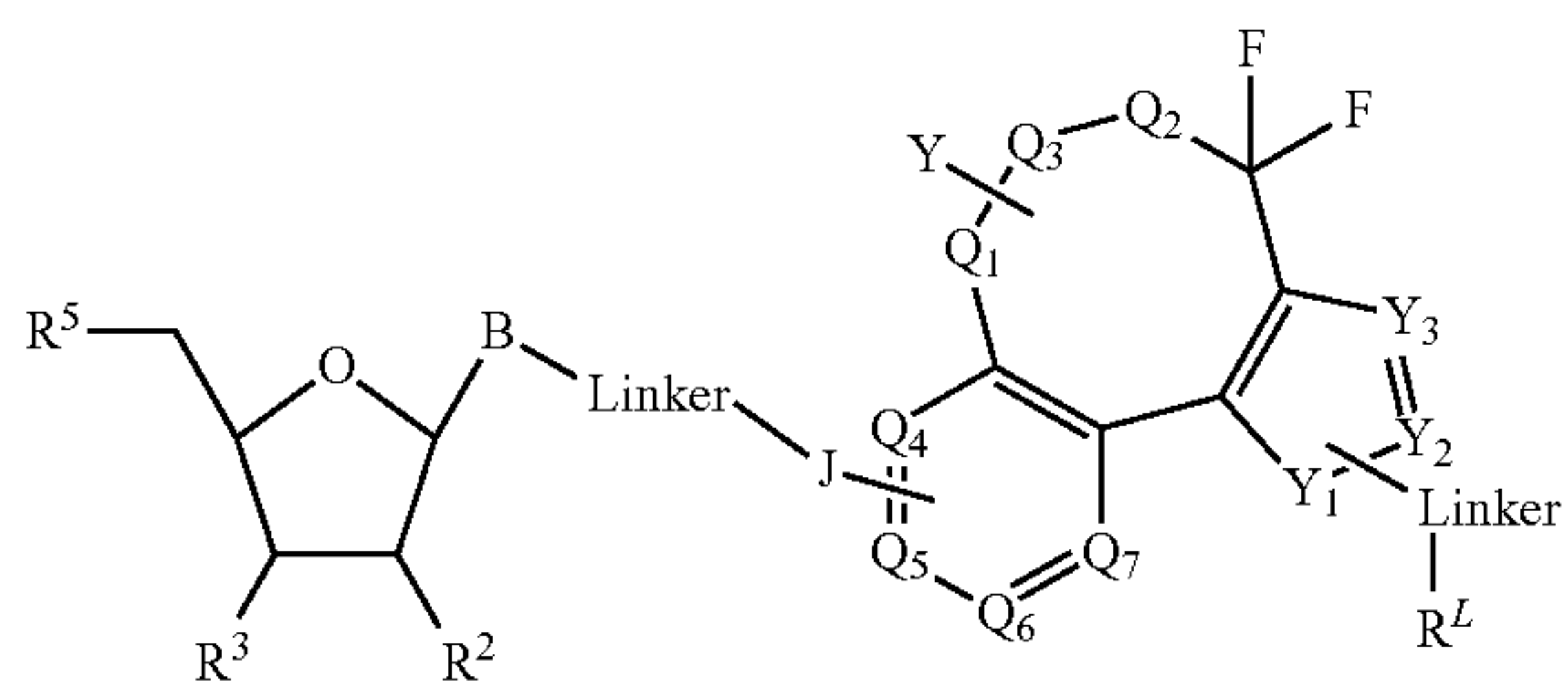
Formula (XVb)
