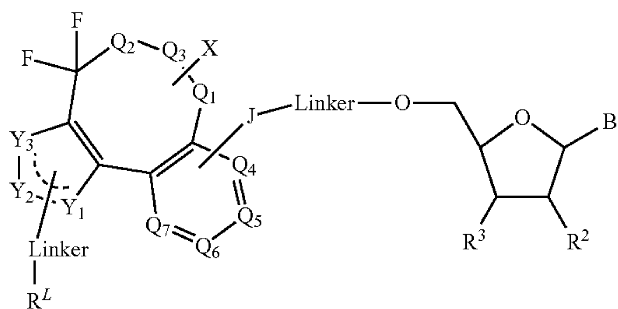
Formula (IXb)
