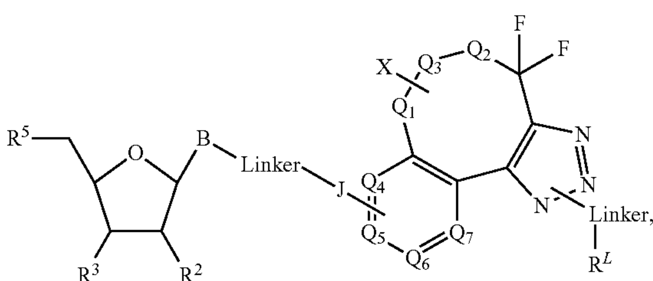
Formula (XVb)
