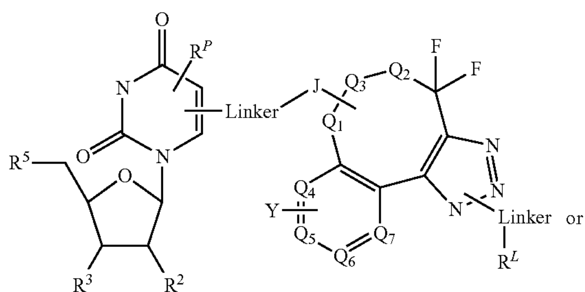
Formula (XVIIa)
