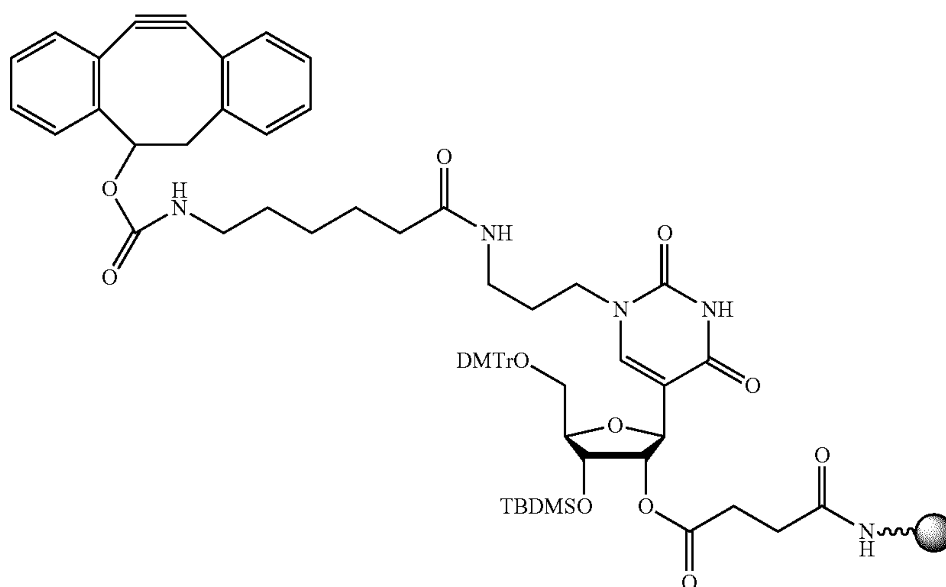
Scheme 20
