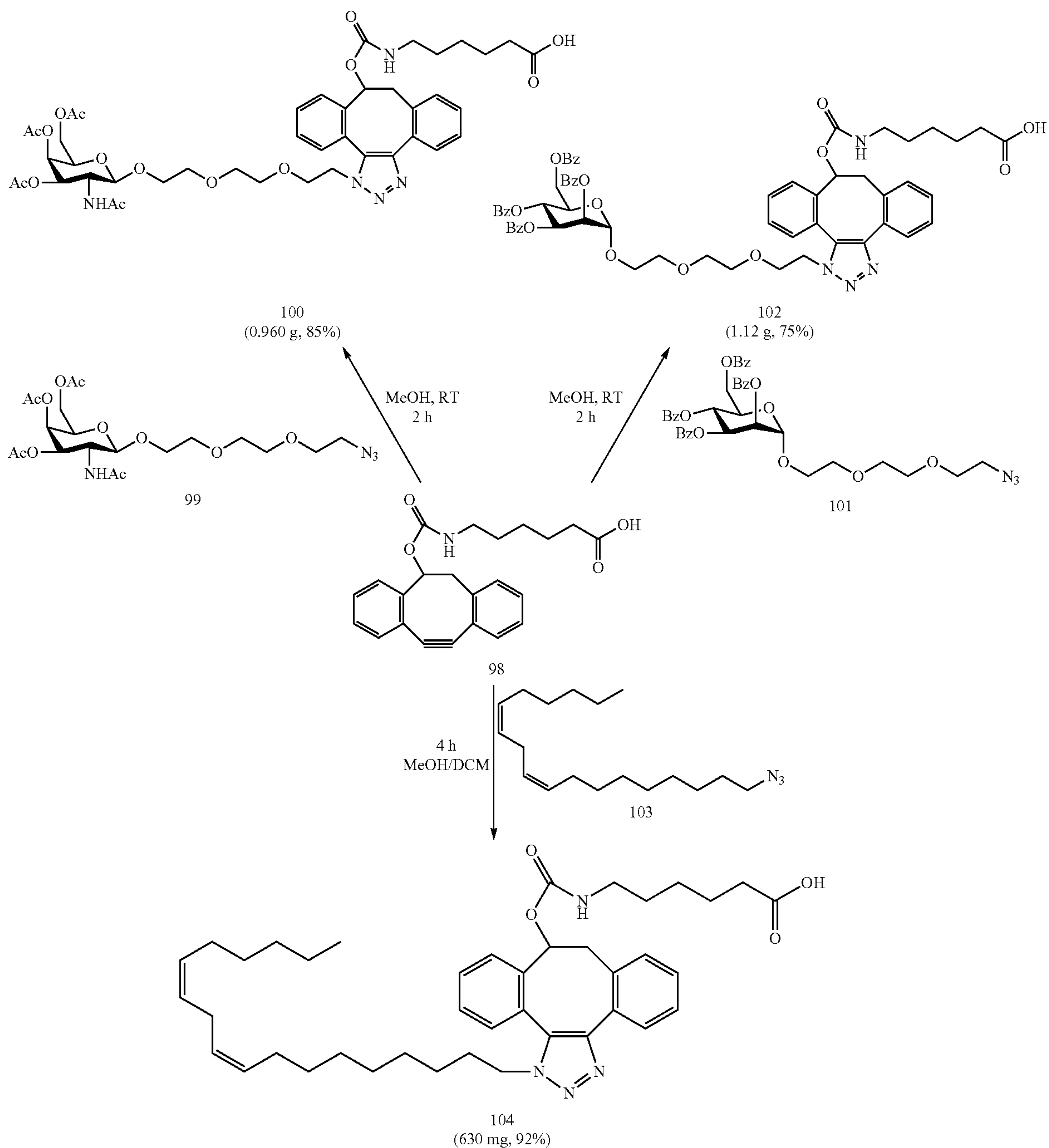
Scheme 2
