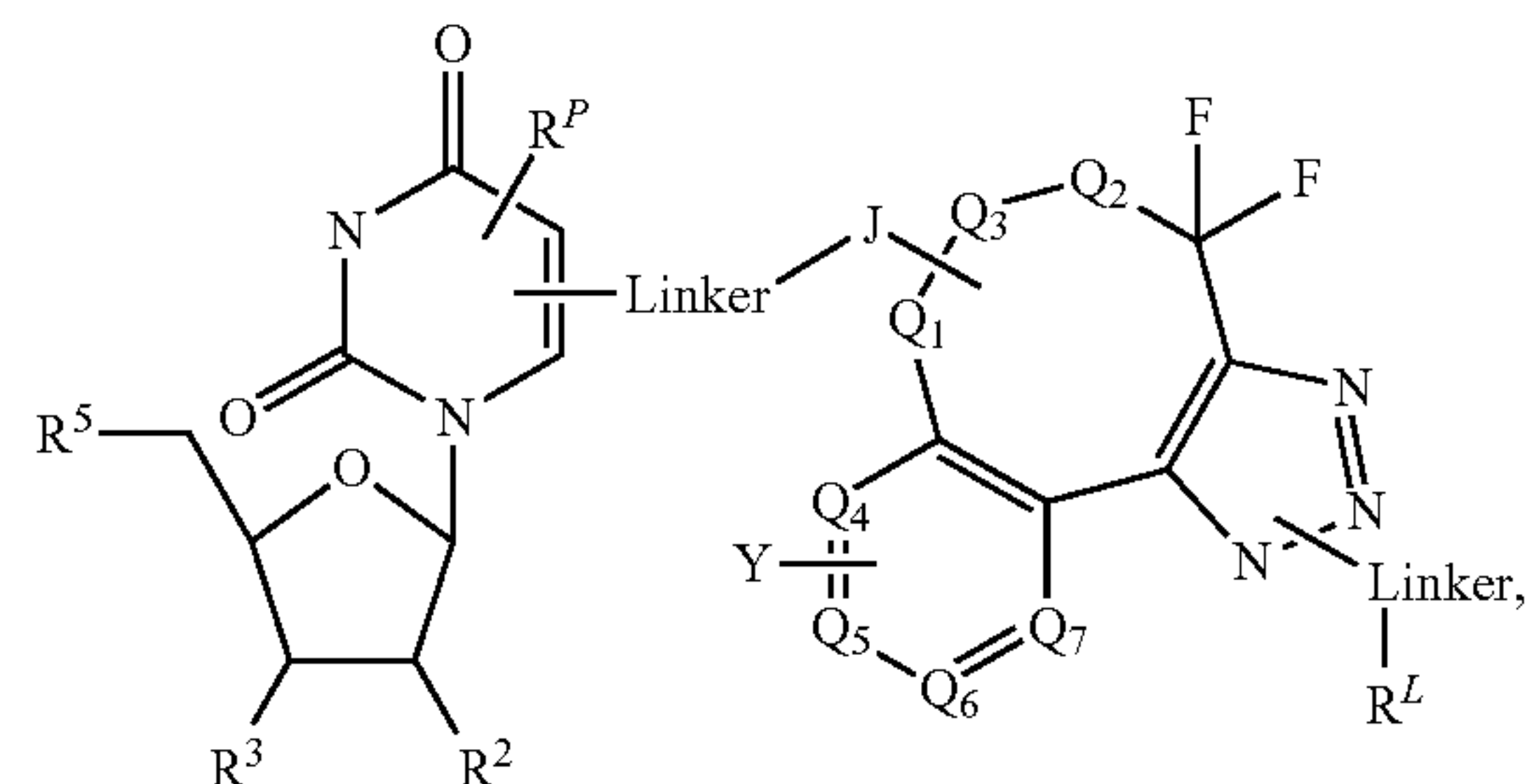
Formula (XVIIa)
