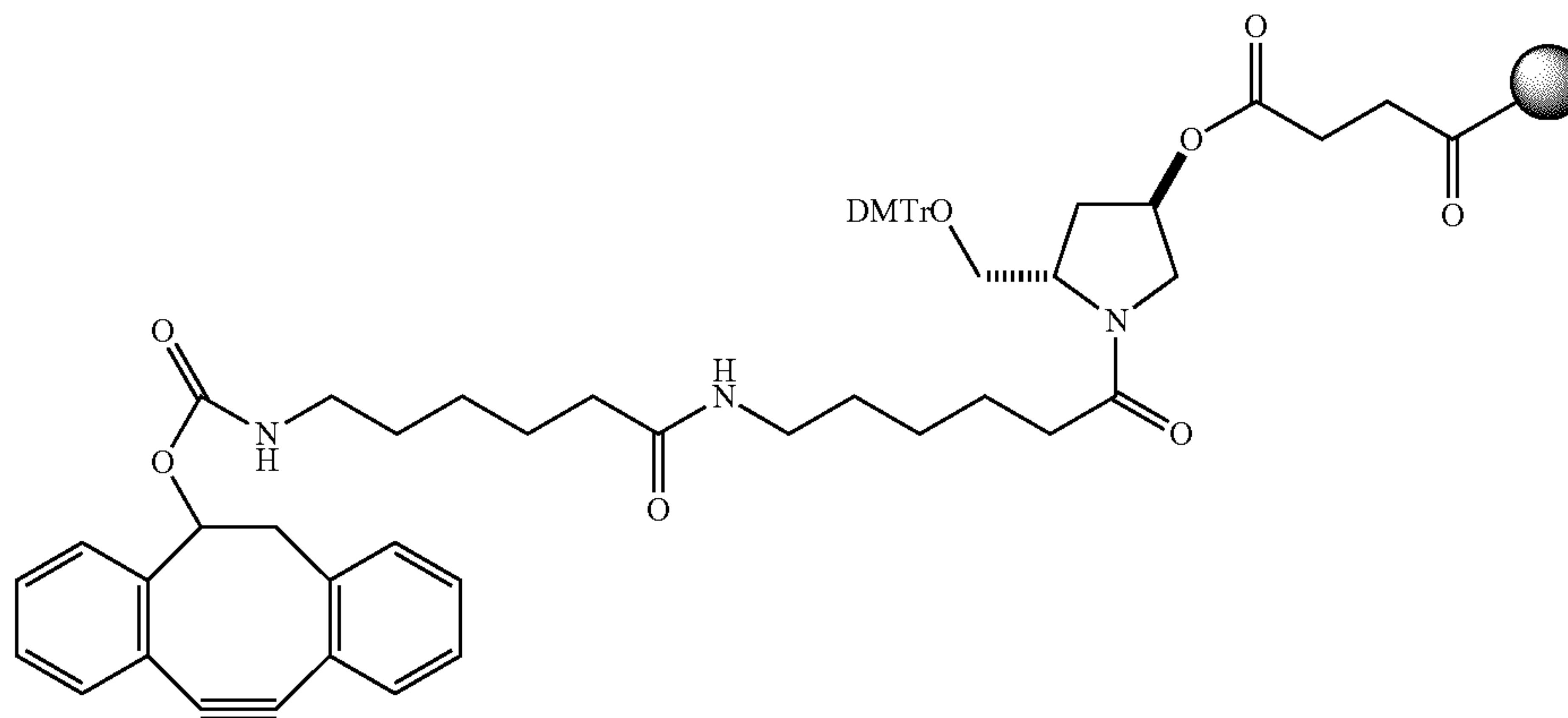
Scheme 3
