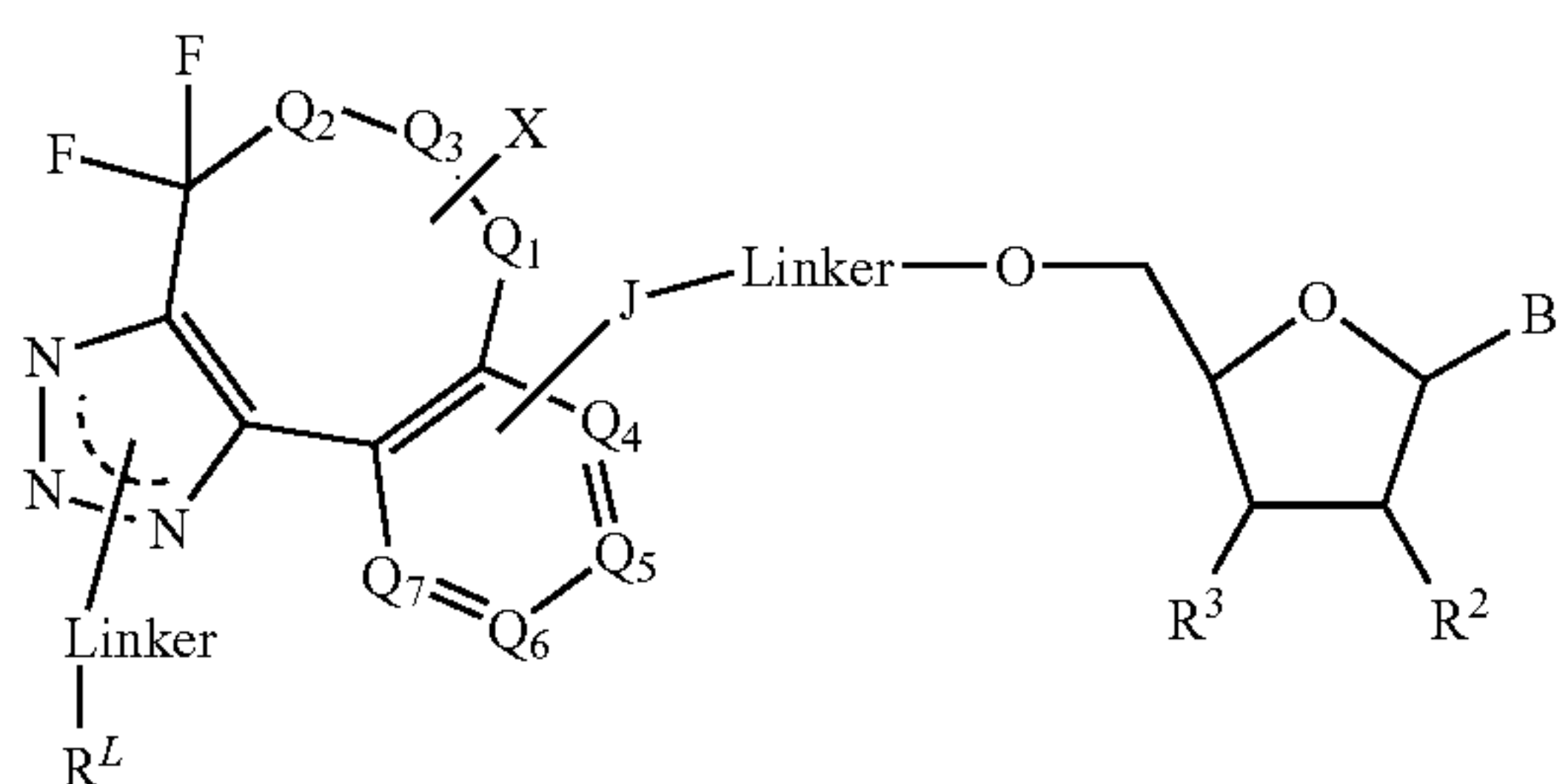
Formula (Xb)
