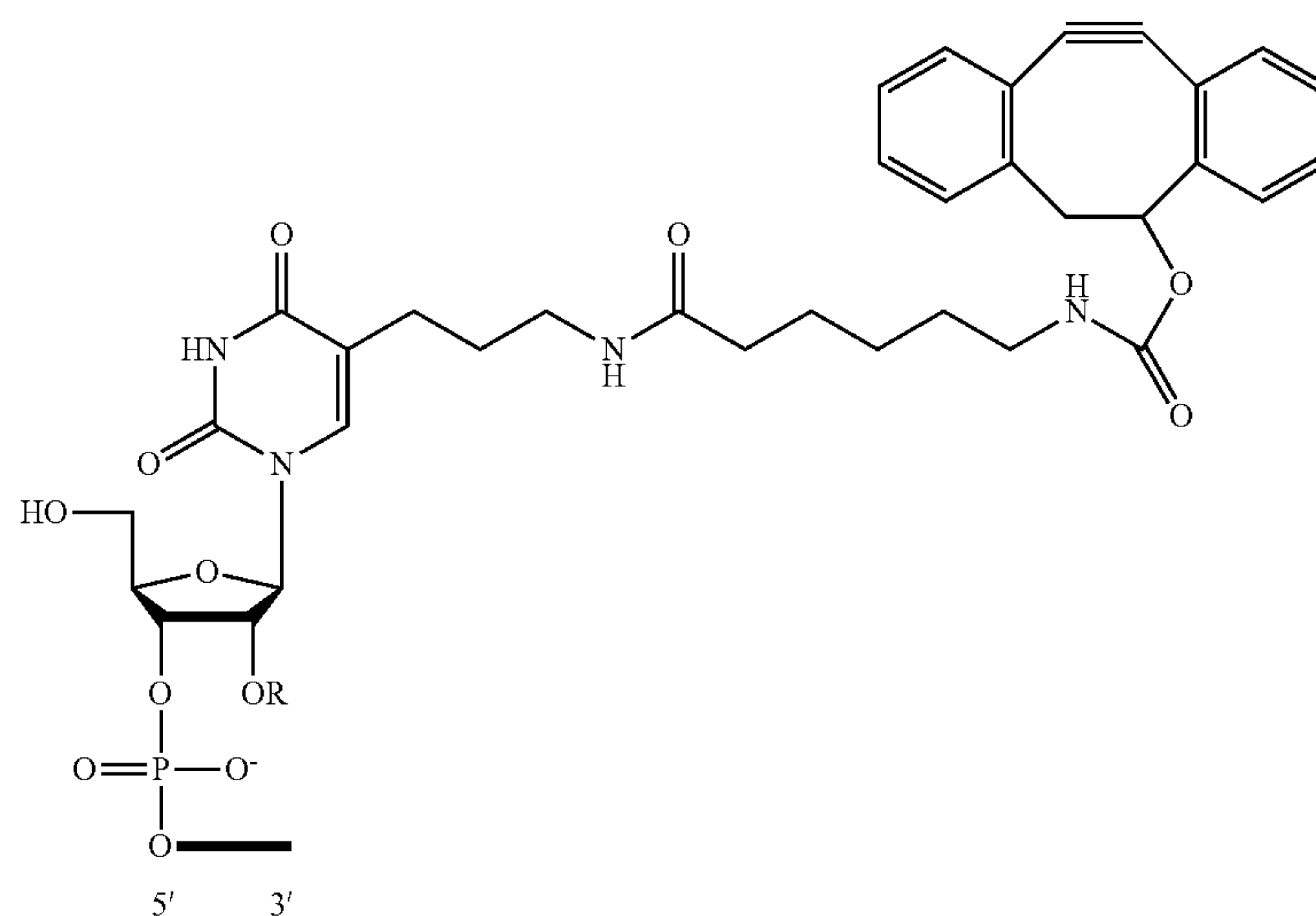
Scheme 18
