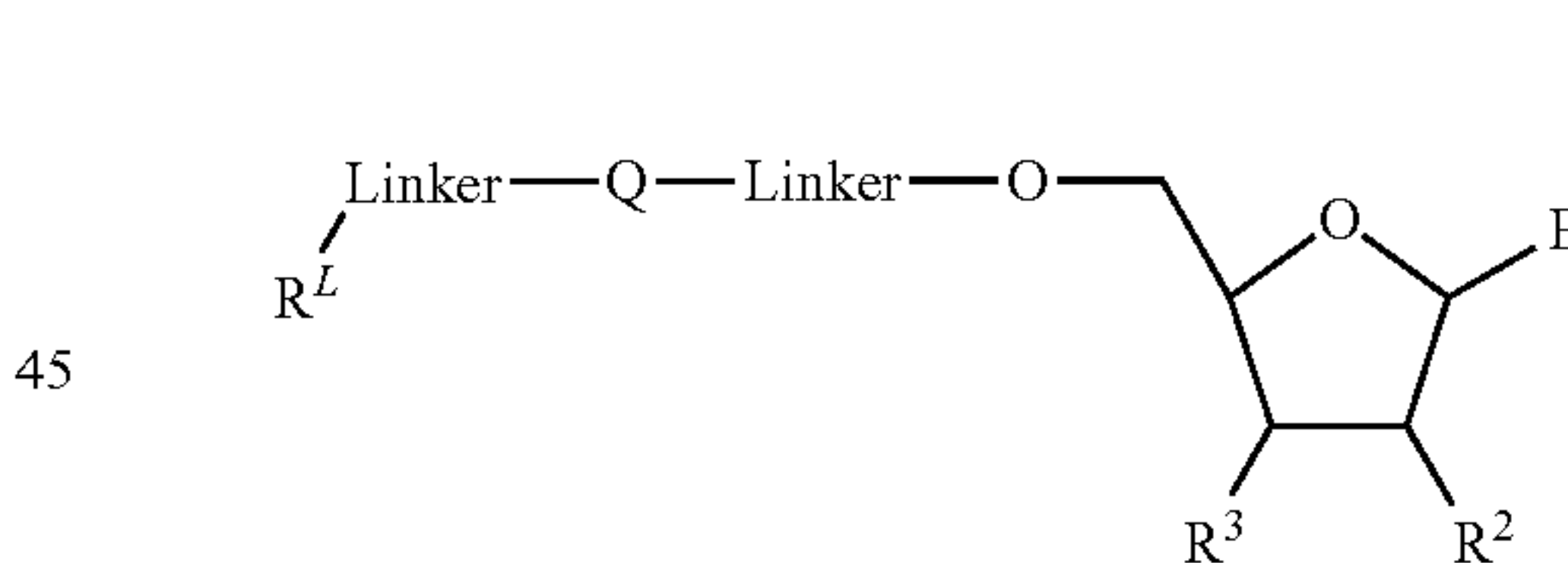
Formula (IXa)
