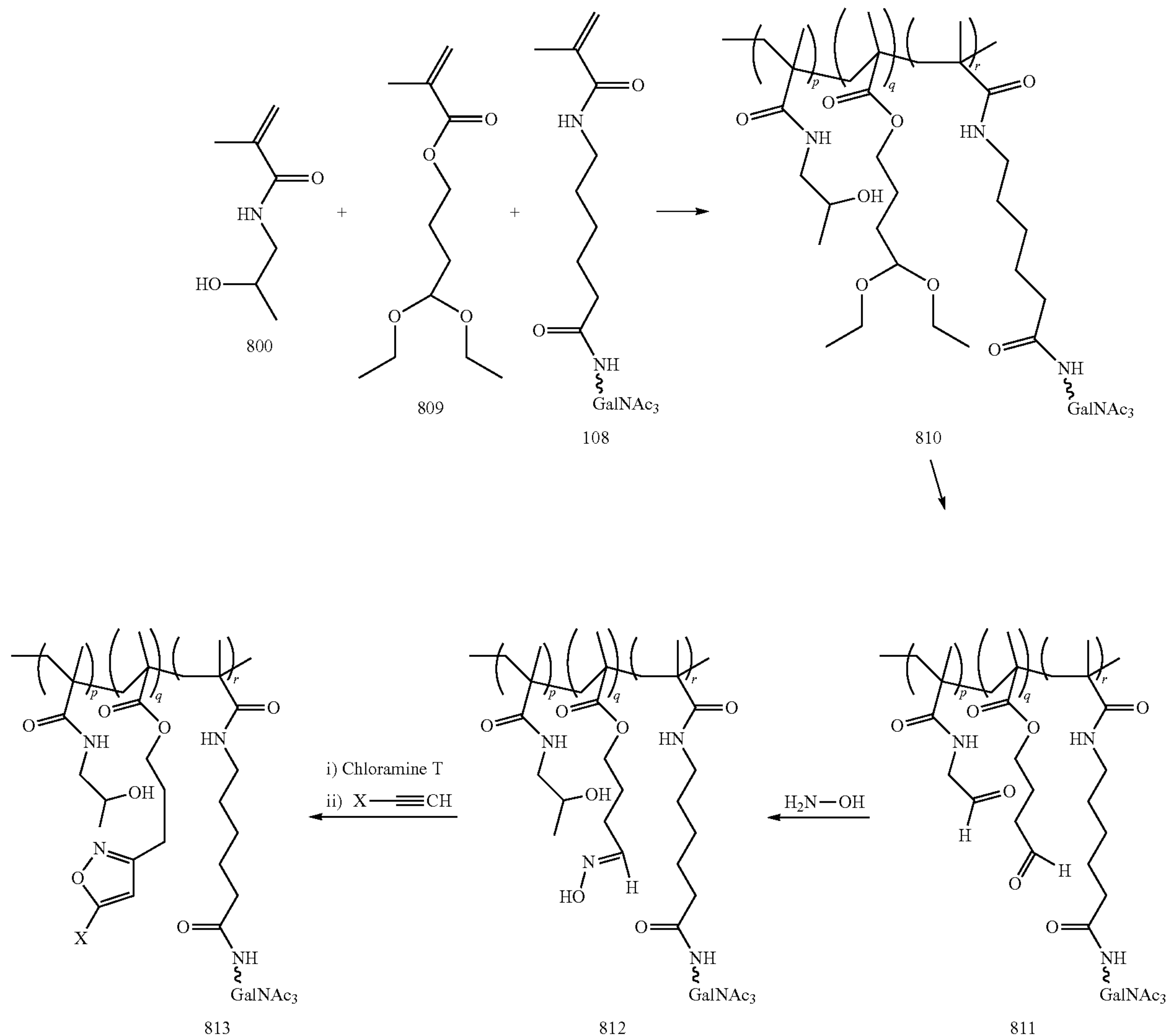
Scheme 22
