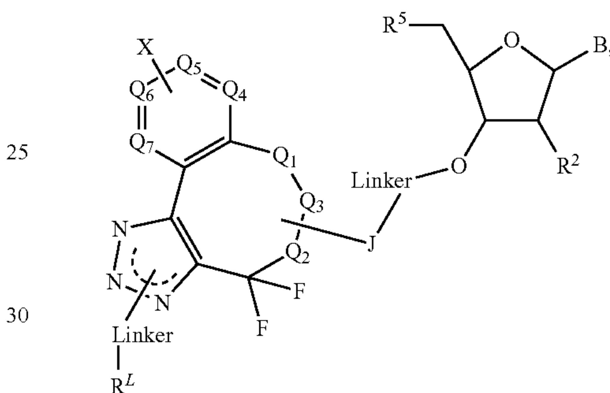
Formula (VII)
