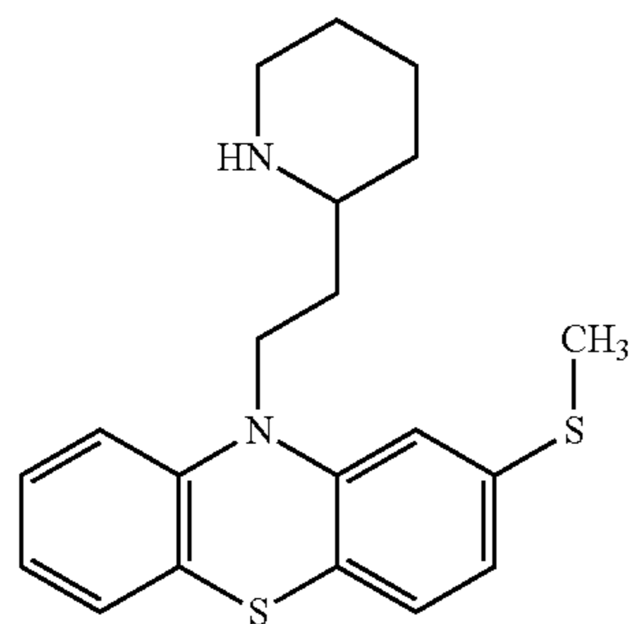
2-(methylsulfanyl)-10-[2-(piperidin-2-yl)ethyl]-10H-phenothiazine
