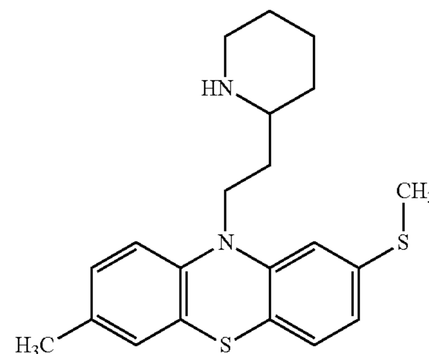
7-Methyl-2-methylsulfanyl-10-(2-piperidin-2-ylethyl)-10H-phenothiazine
