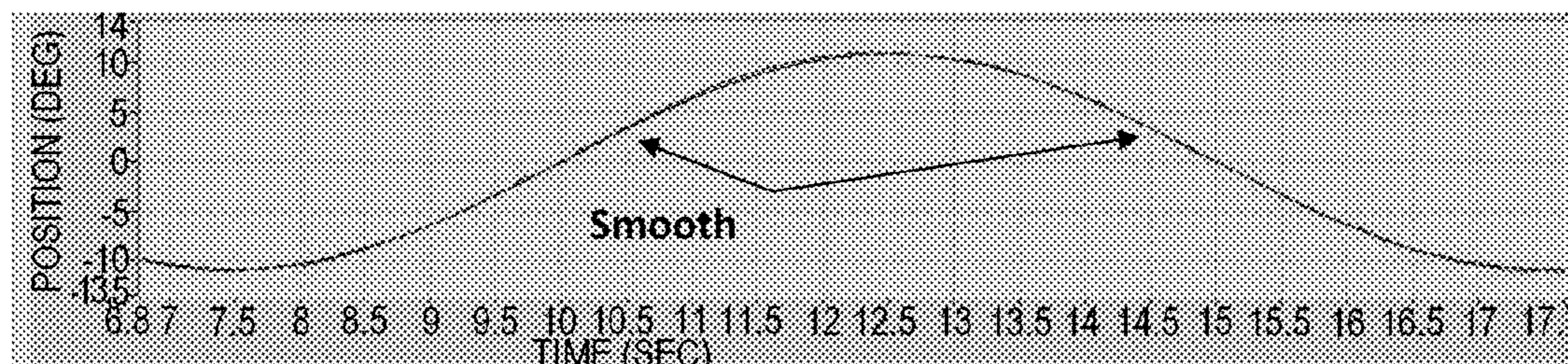
Normal Smooth
