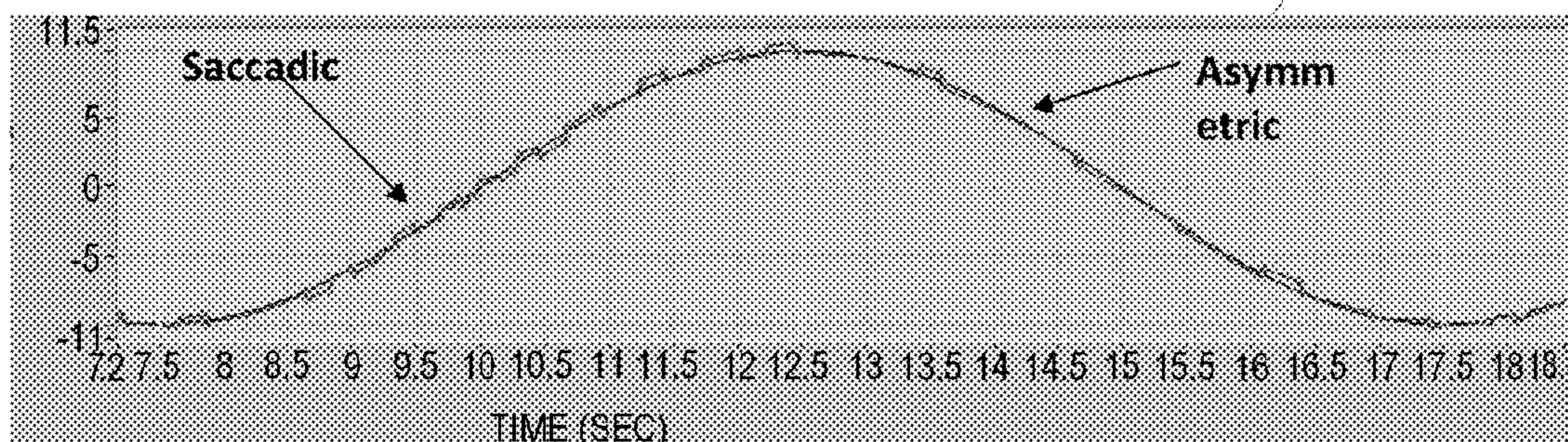
Abnormal Smooth
