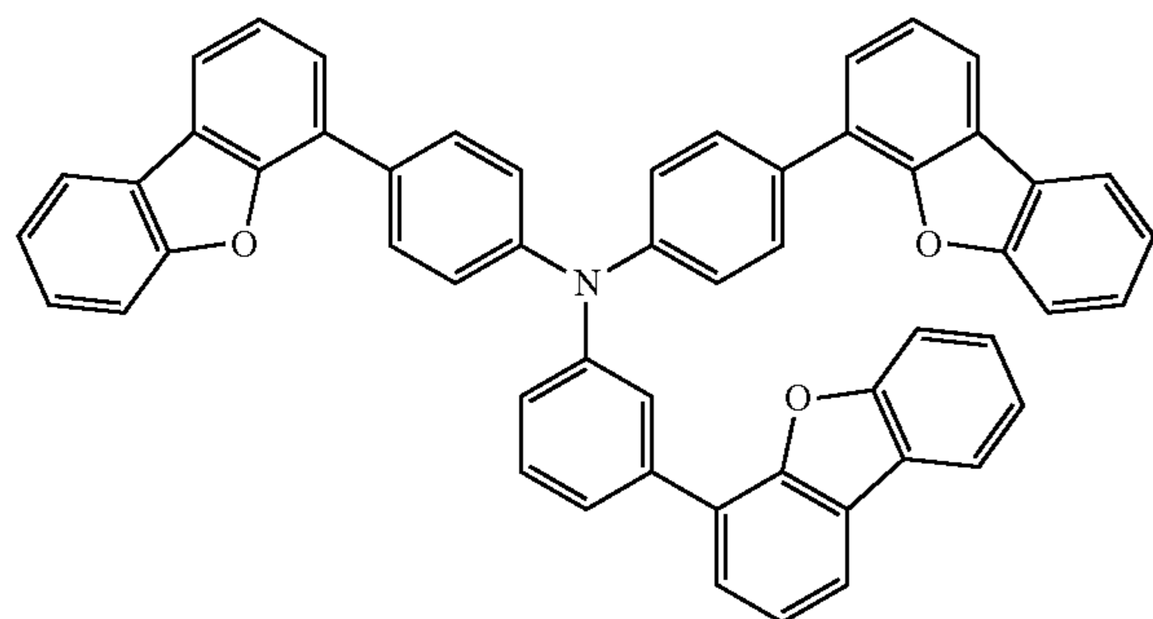
Synthesis Example 3
