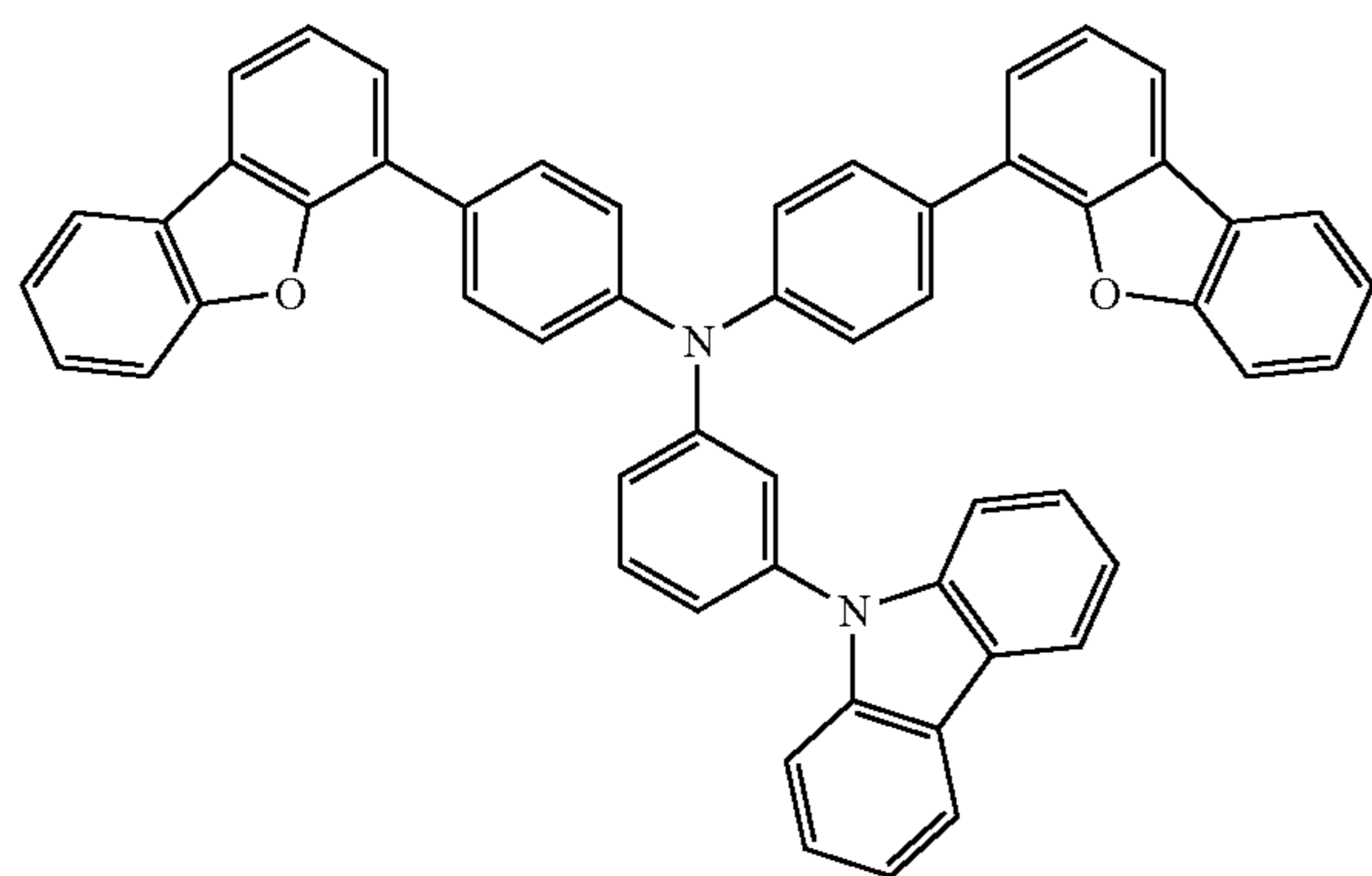
Synthesis Example 4
