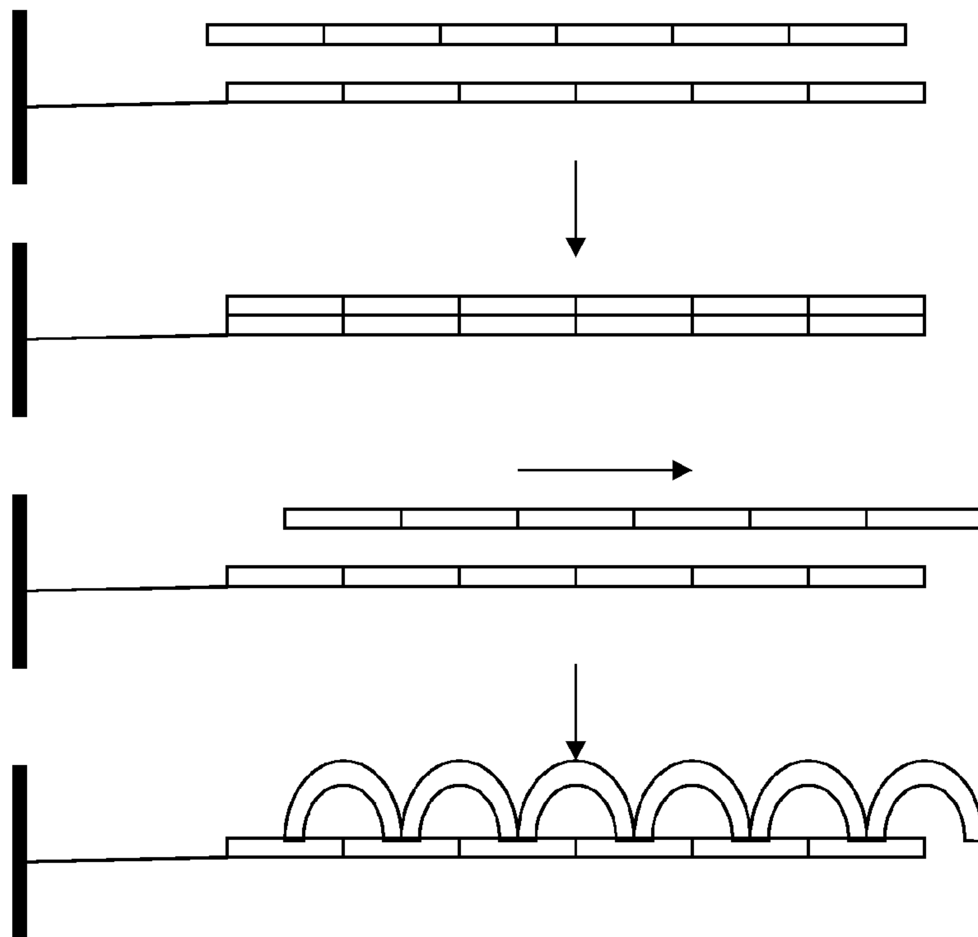
Combinatorial Tag With "Commas-less" Property
