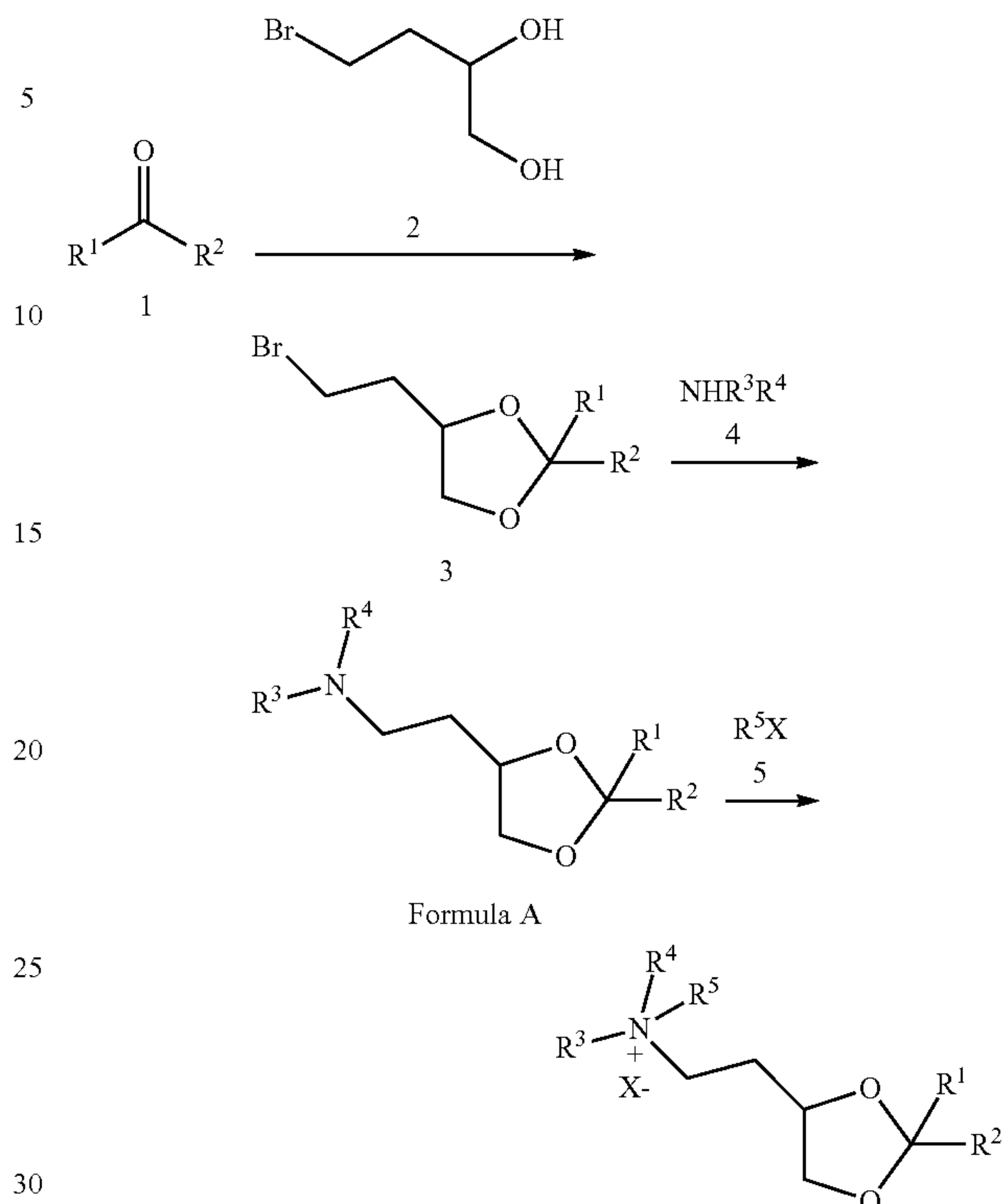
Scheme 1
