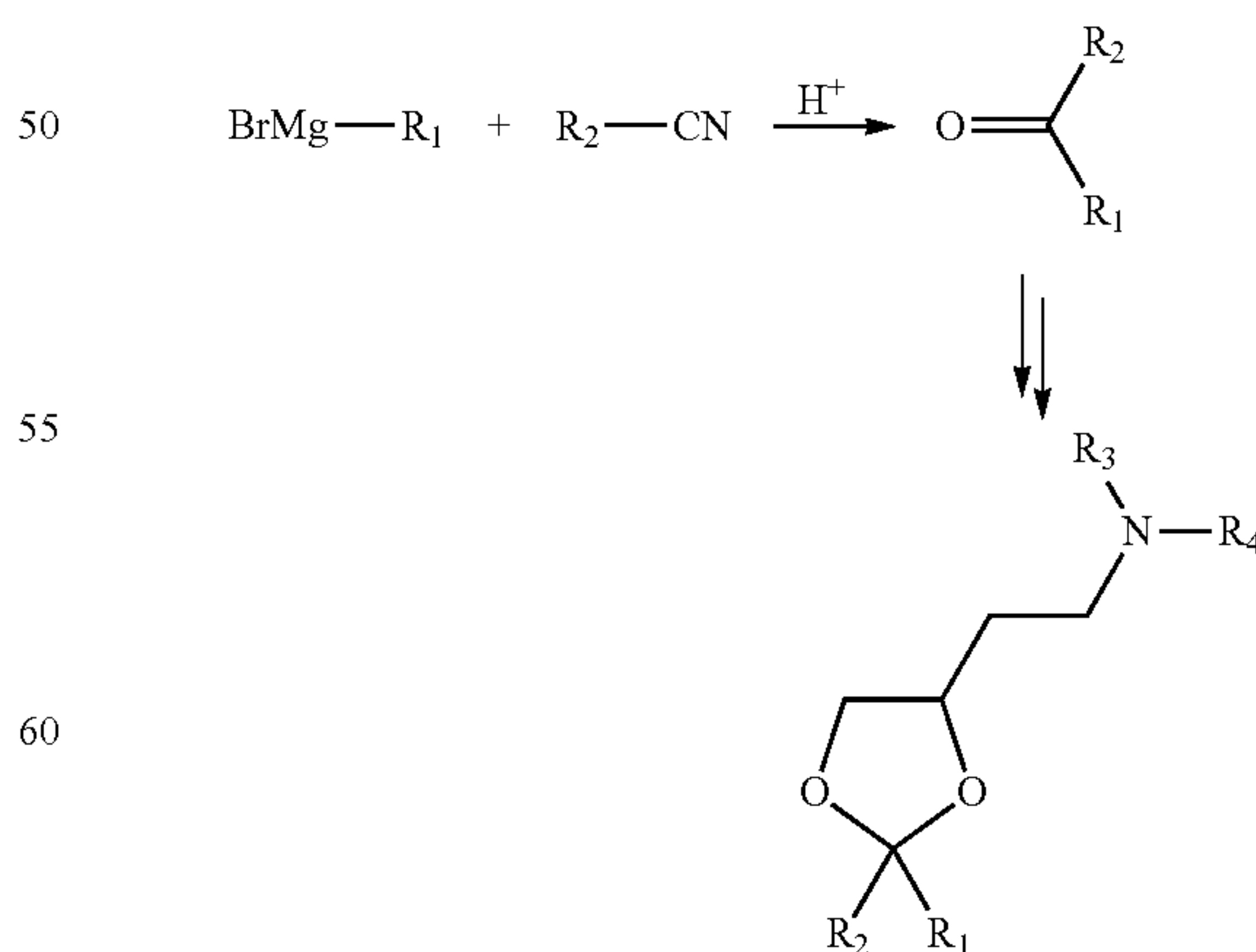
Scheme 2
