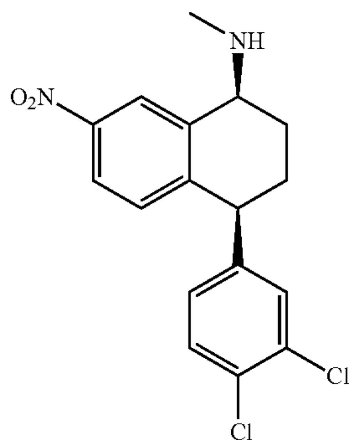
Nitro Sertraline
