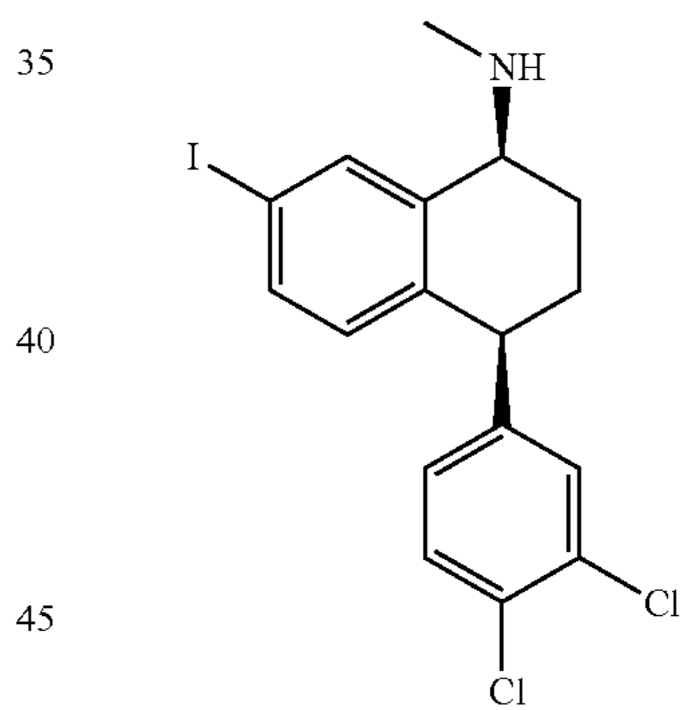
Sertraline iodine
