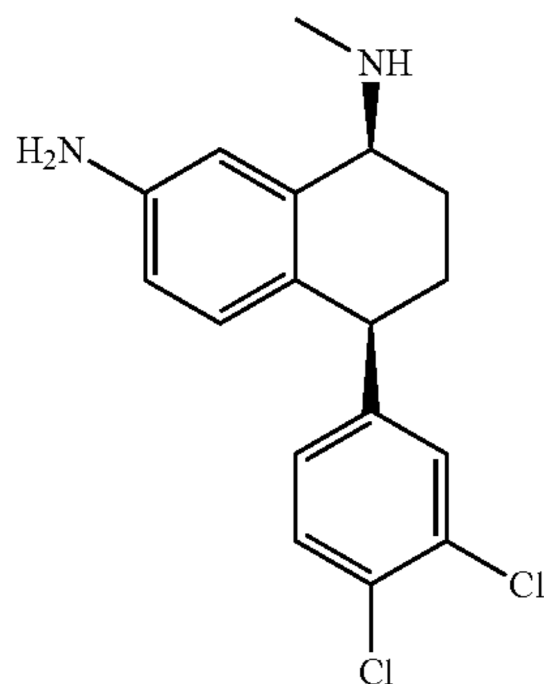
Sertraline aniline
