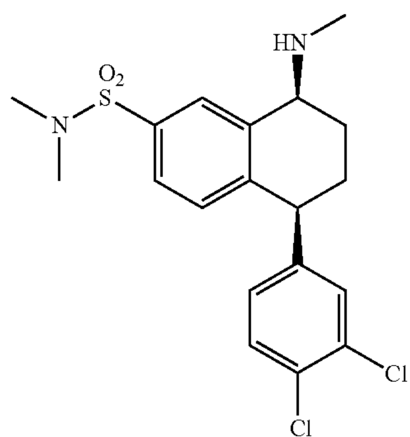
Sertraline N,N-Dimethylsulfonamide
