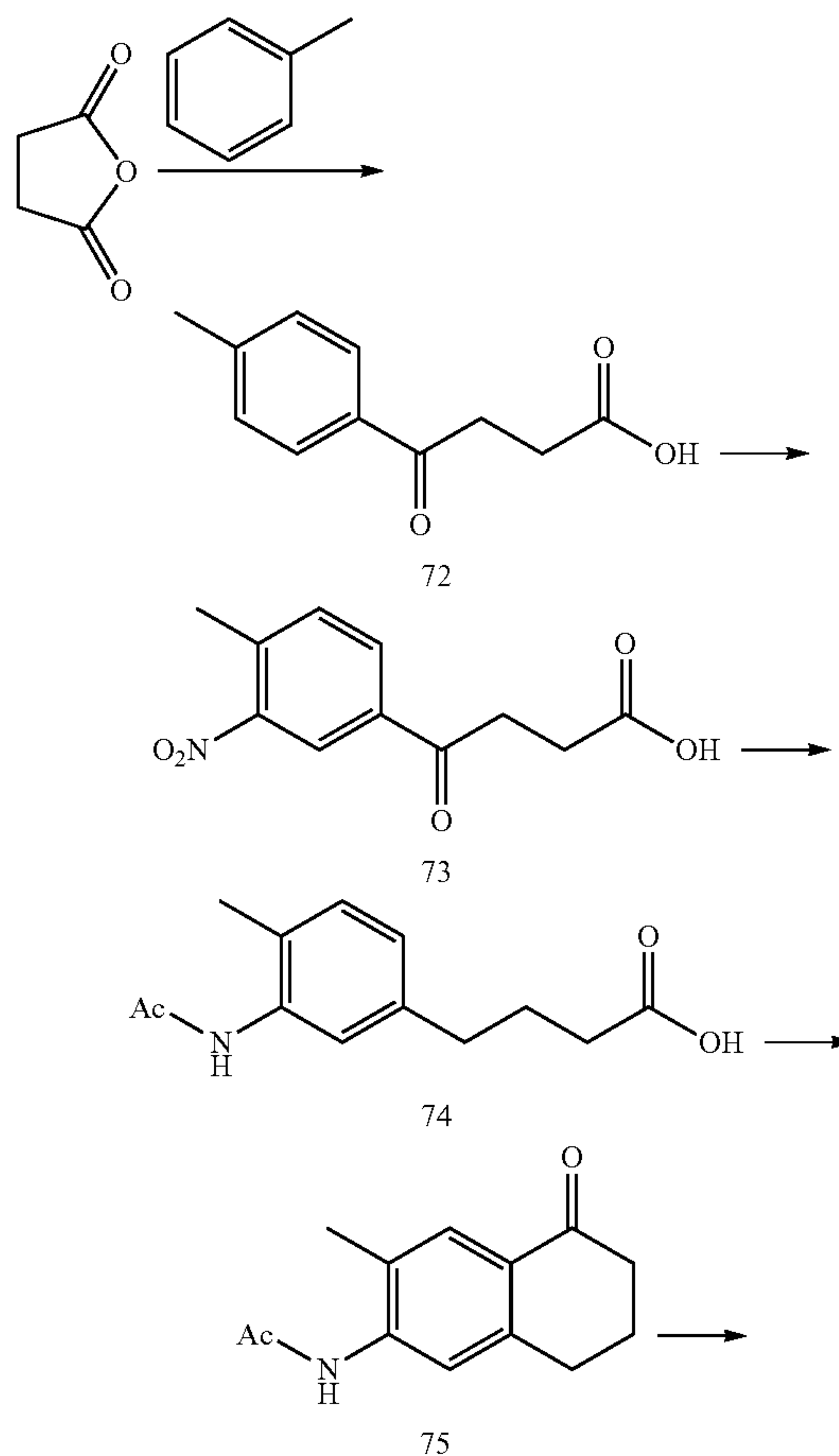
Scheme 18:
