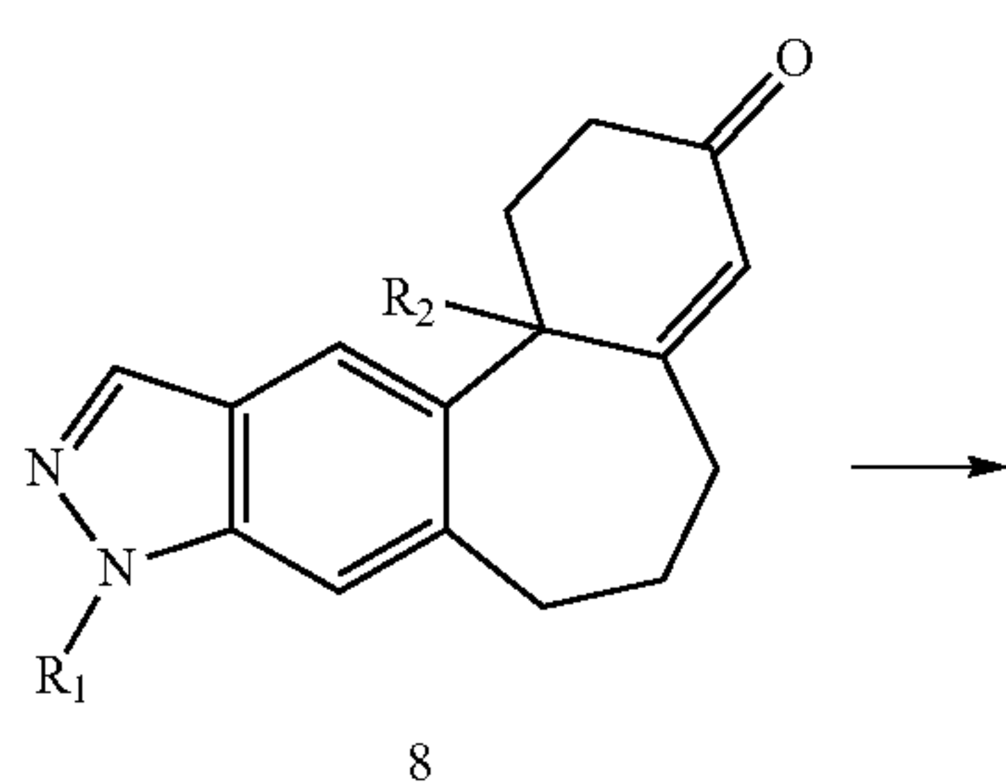
Scheme 15
