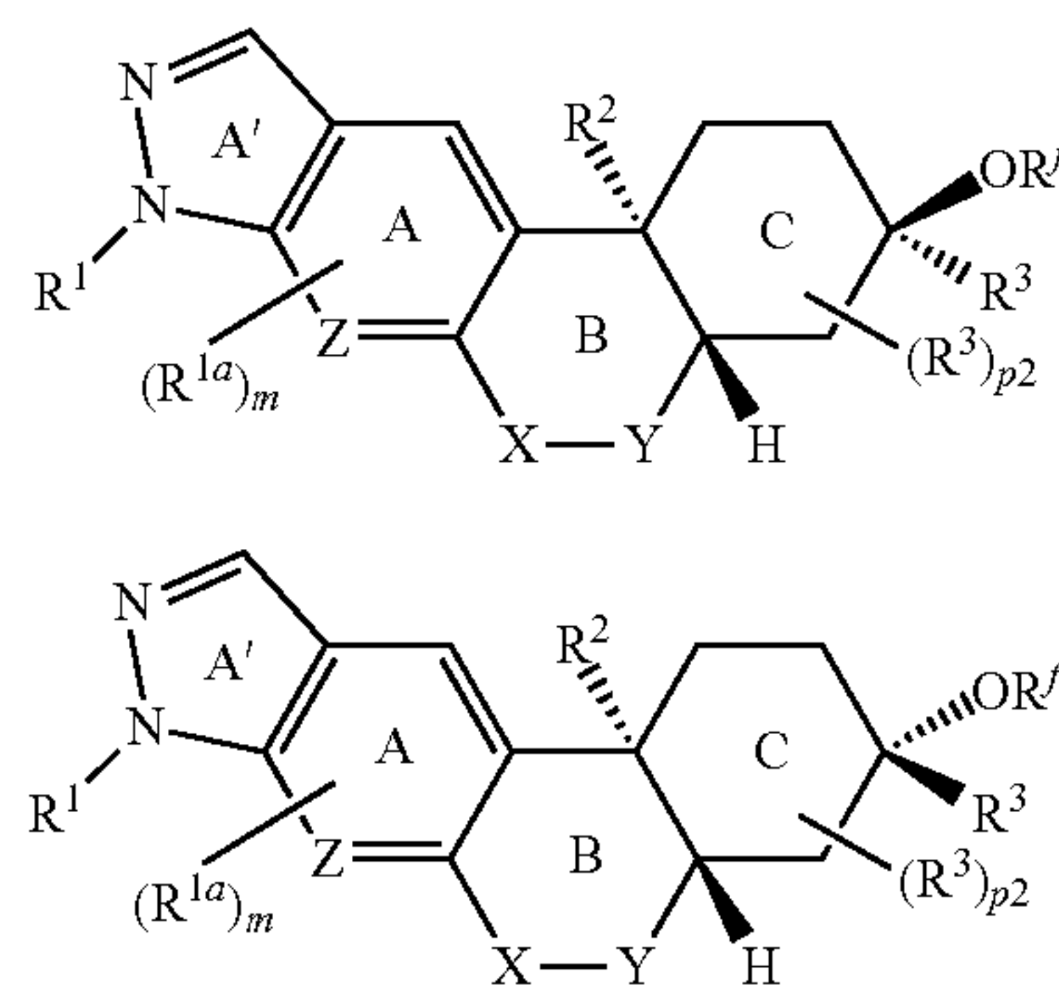
Formula (I)D4E2
