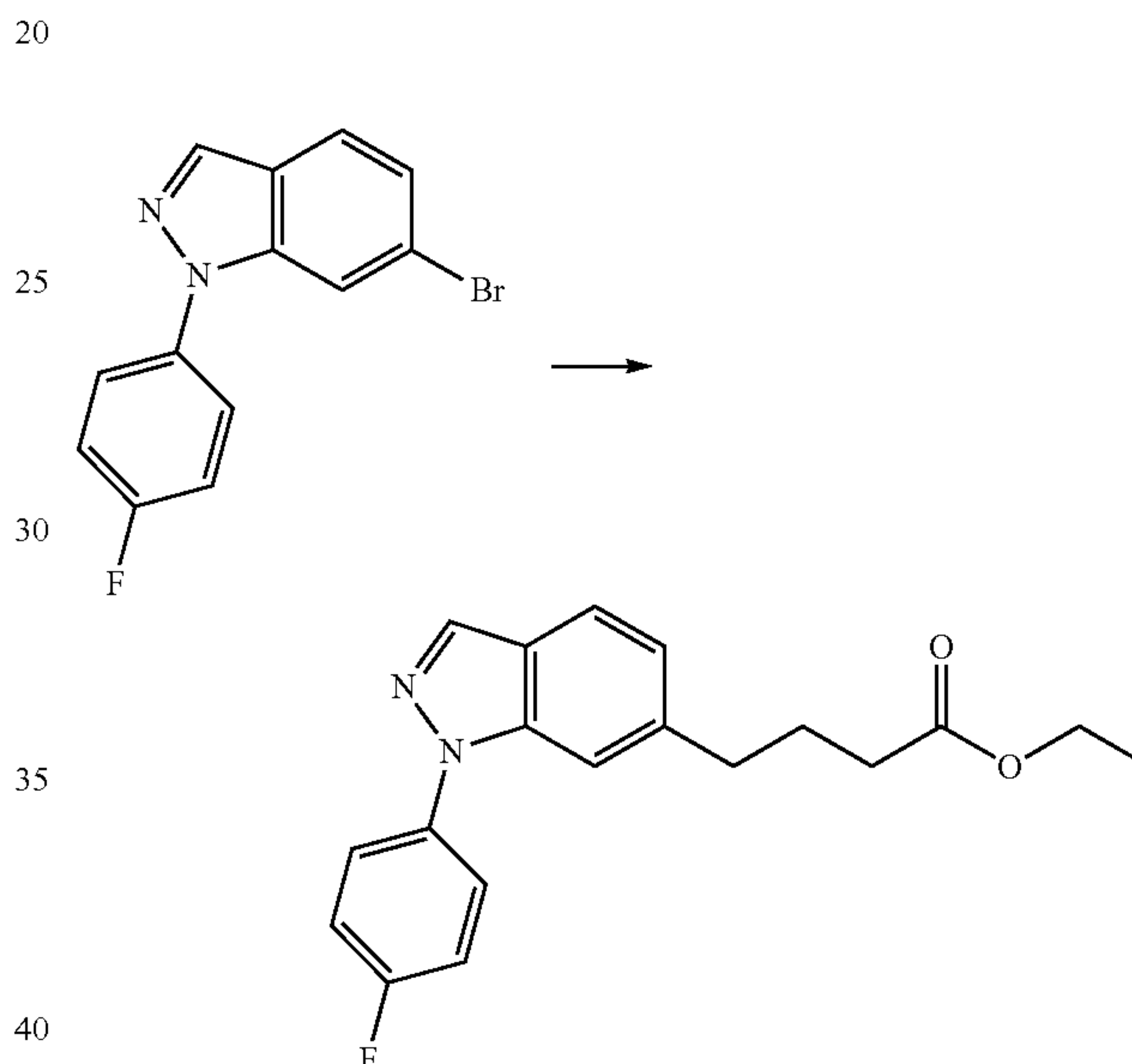
Step #2: Ethyl 4-(1-(4-fluorophenyl)-1H-indazol-6-yl)butanoate (2, R 1 =4-Fluorophenyl)
