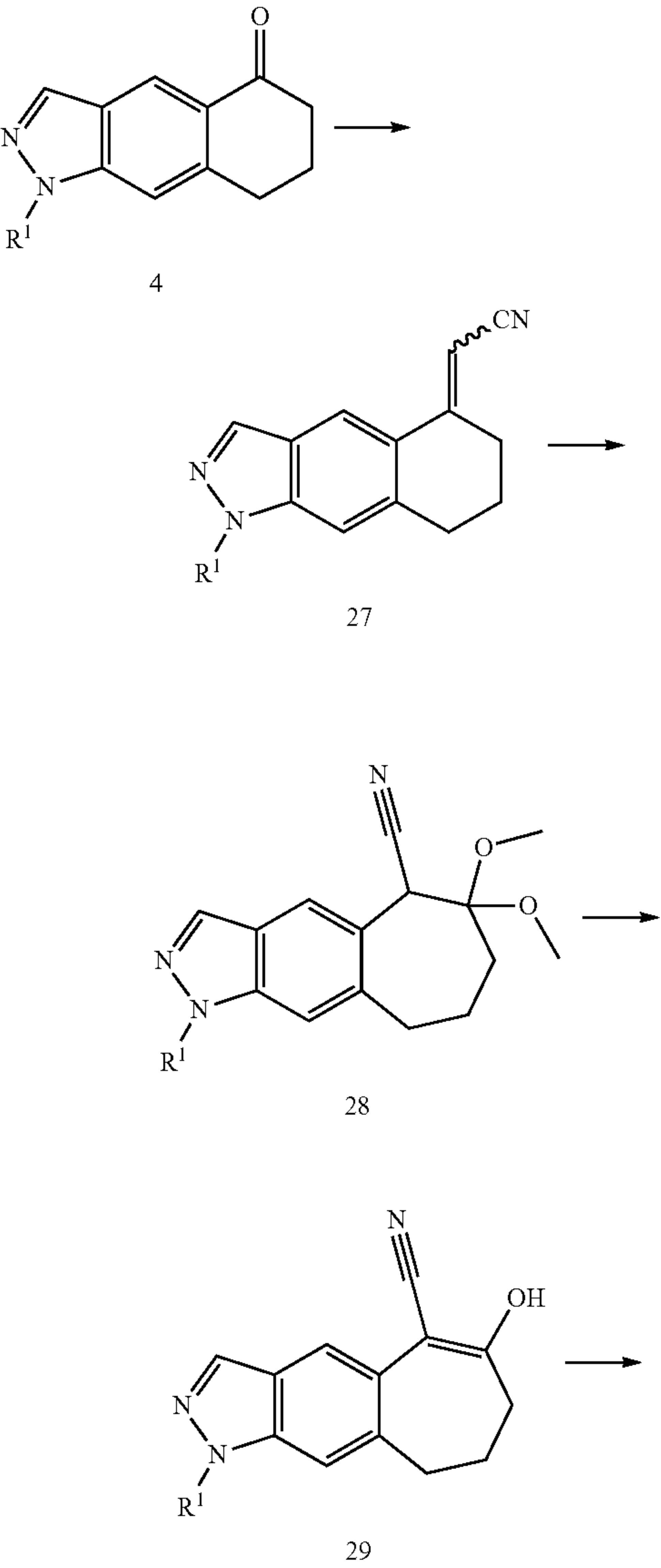
Scheme 3:
