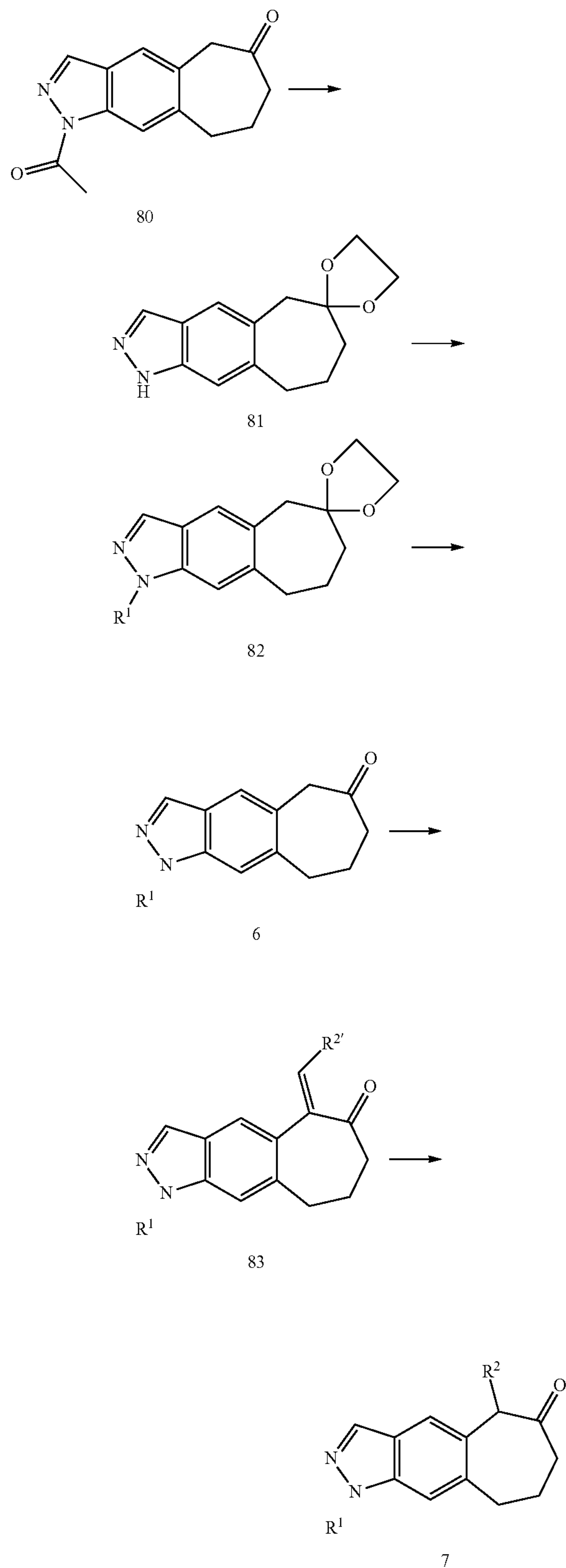
Scheme 19:
