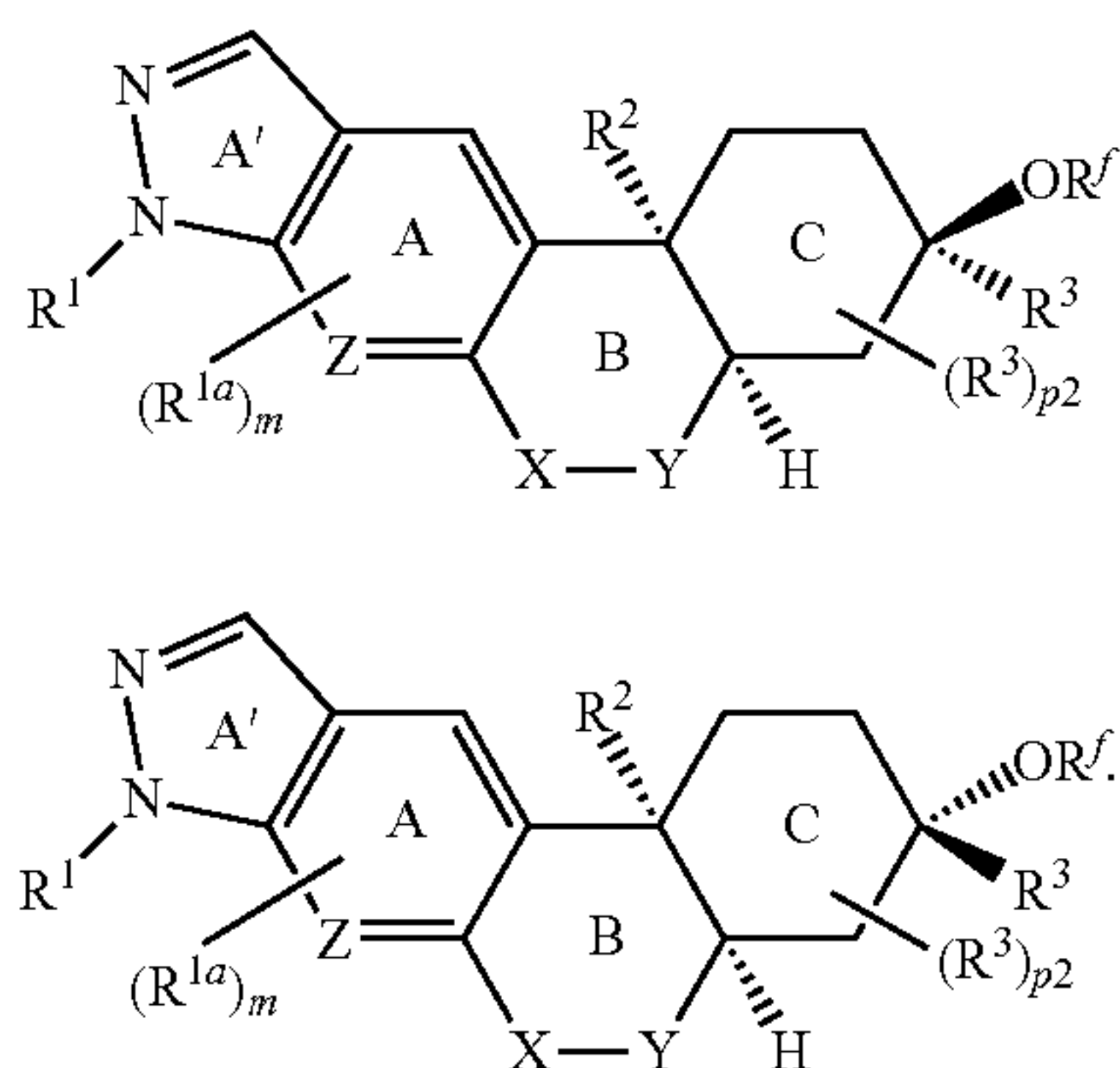
Formula (I)D2E2
