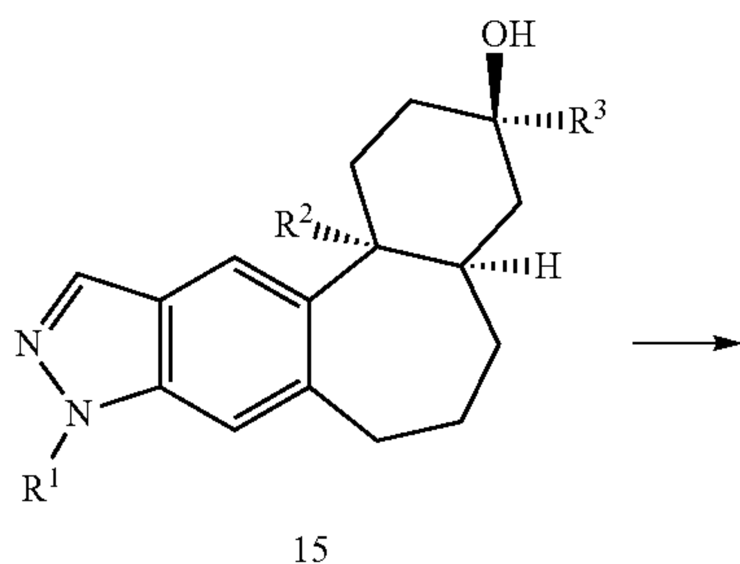
Scheme 8:
