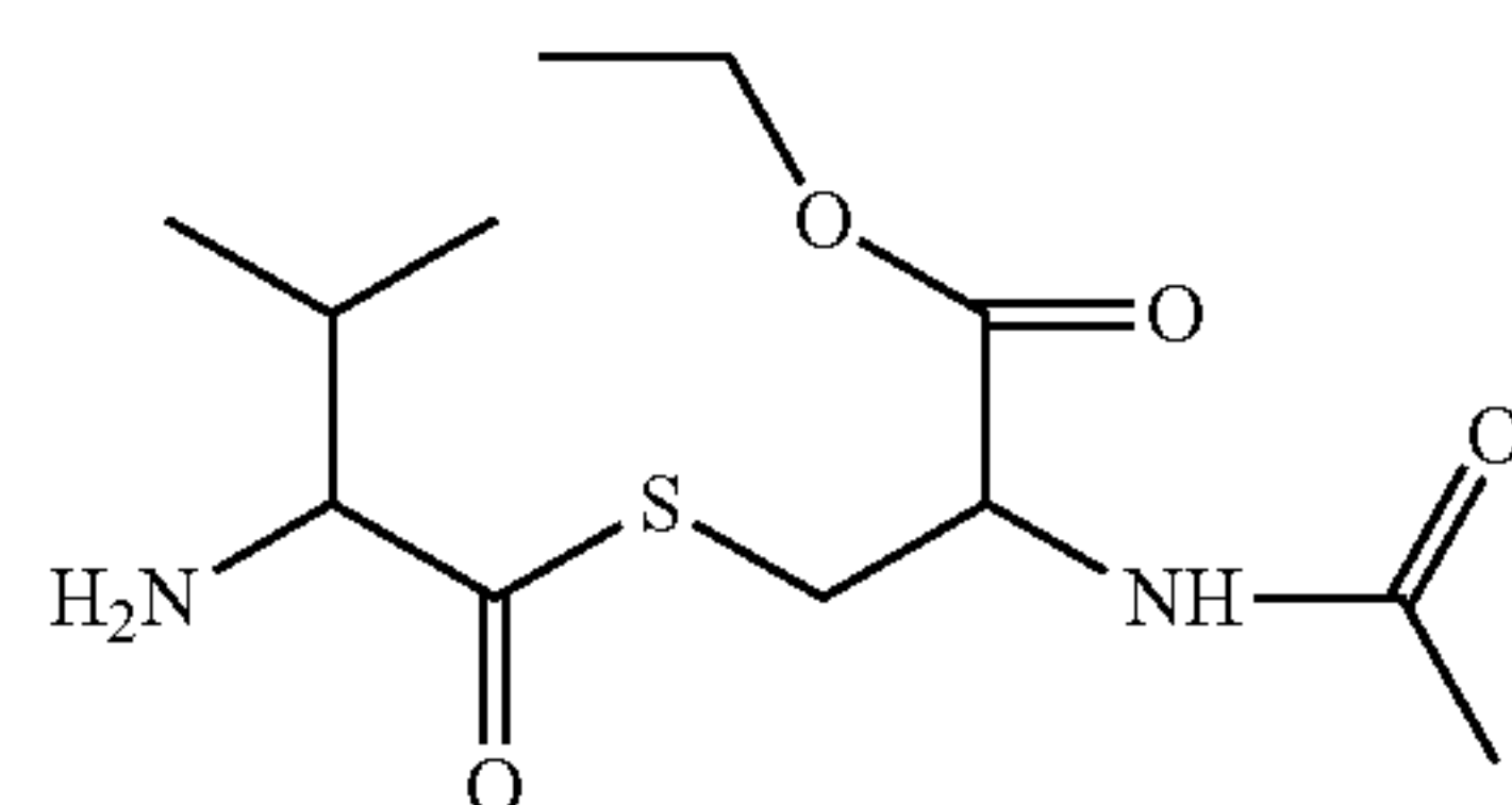
(R)-ethyl-2-acetamido-3-([(S)-2-amino-3-methylbutanoyl]thio)propanoate
