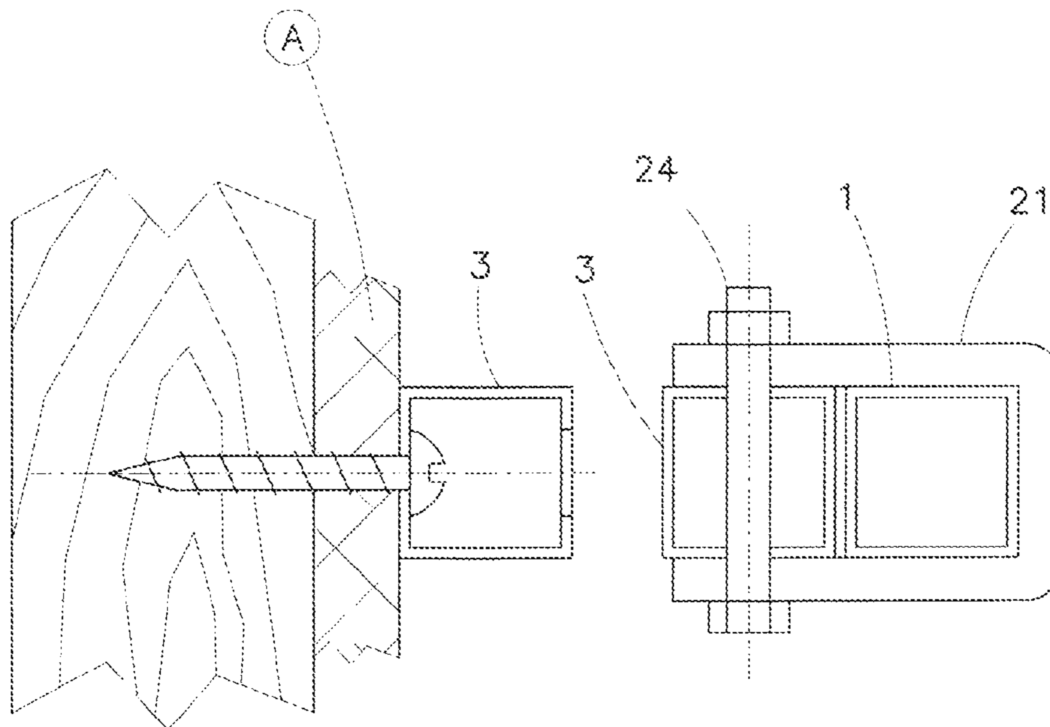
SECTION "A" - "A"
