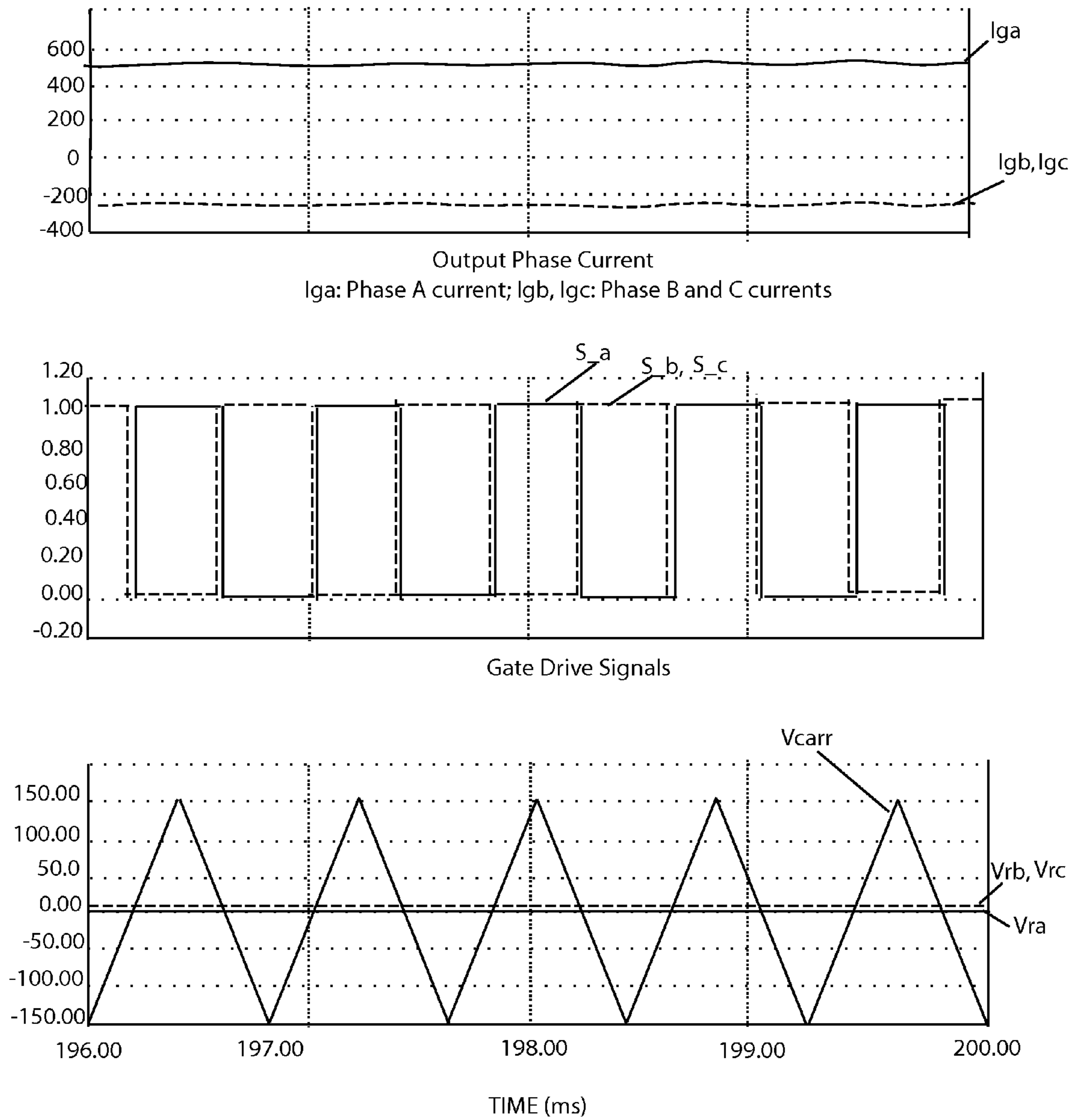
REGULAR PWM CONTROL FOR ROTOR LOCK OPERATION
