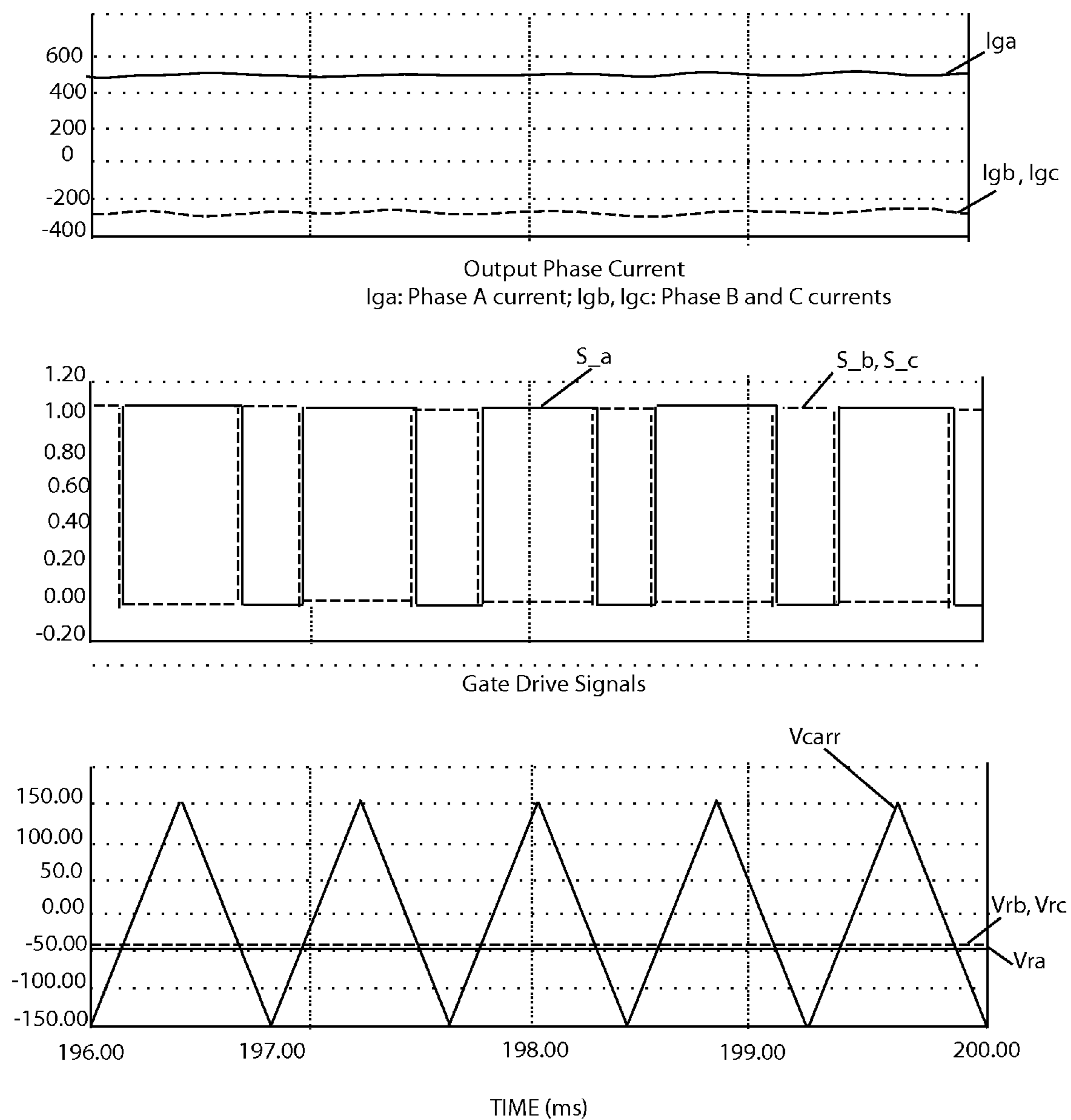
PROPPED PWM CONTROL FOR ROTOR LOCK OPERATION
