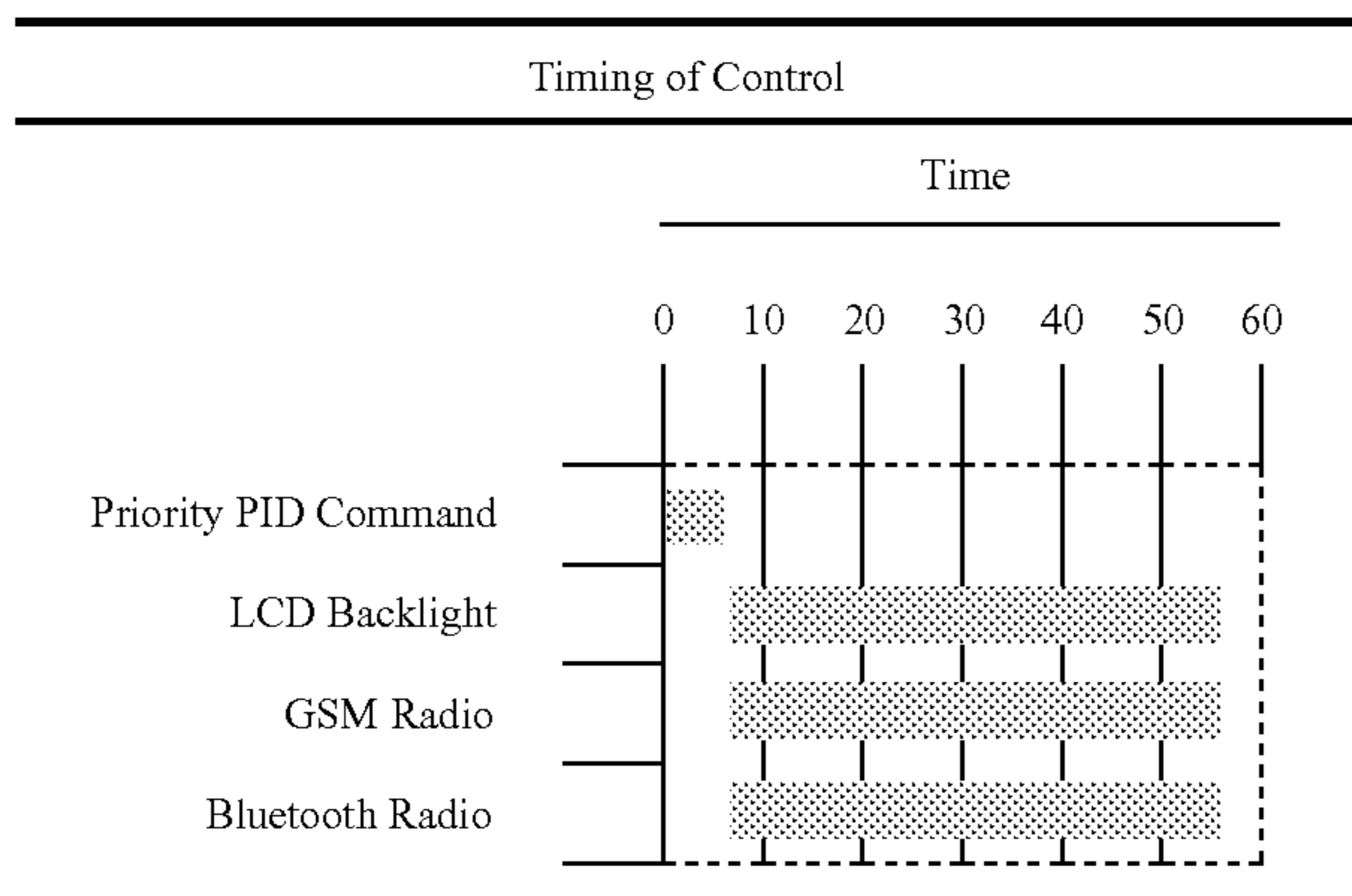
Timing of control for primary and secondary side power management coordination. It should be noted latency of power control for each system may be considered for control.
