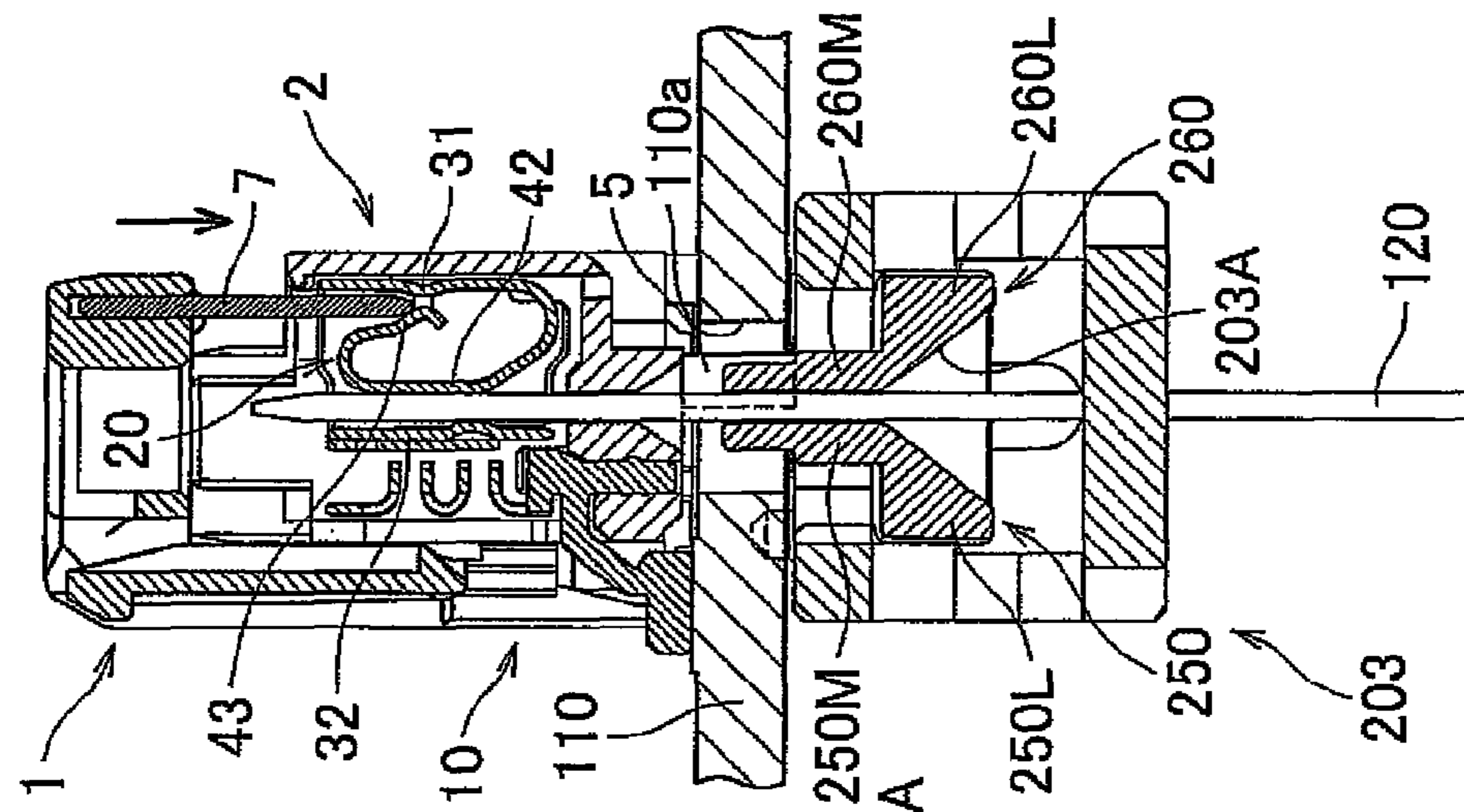
FIG. 19B CLOSE STATE
