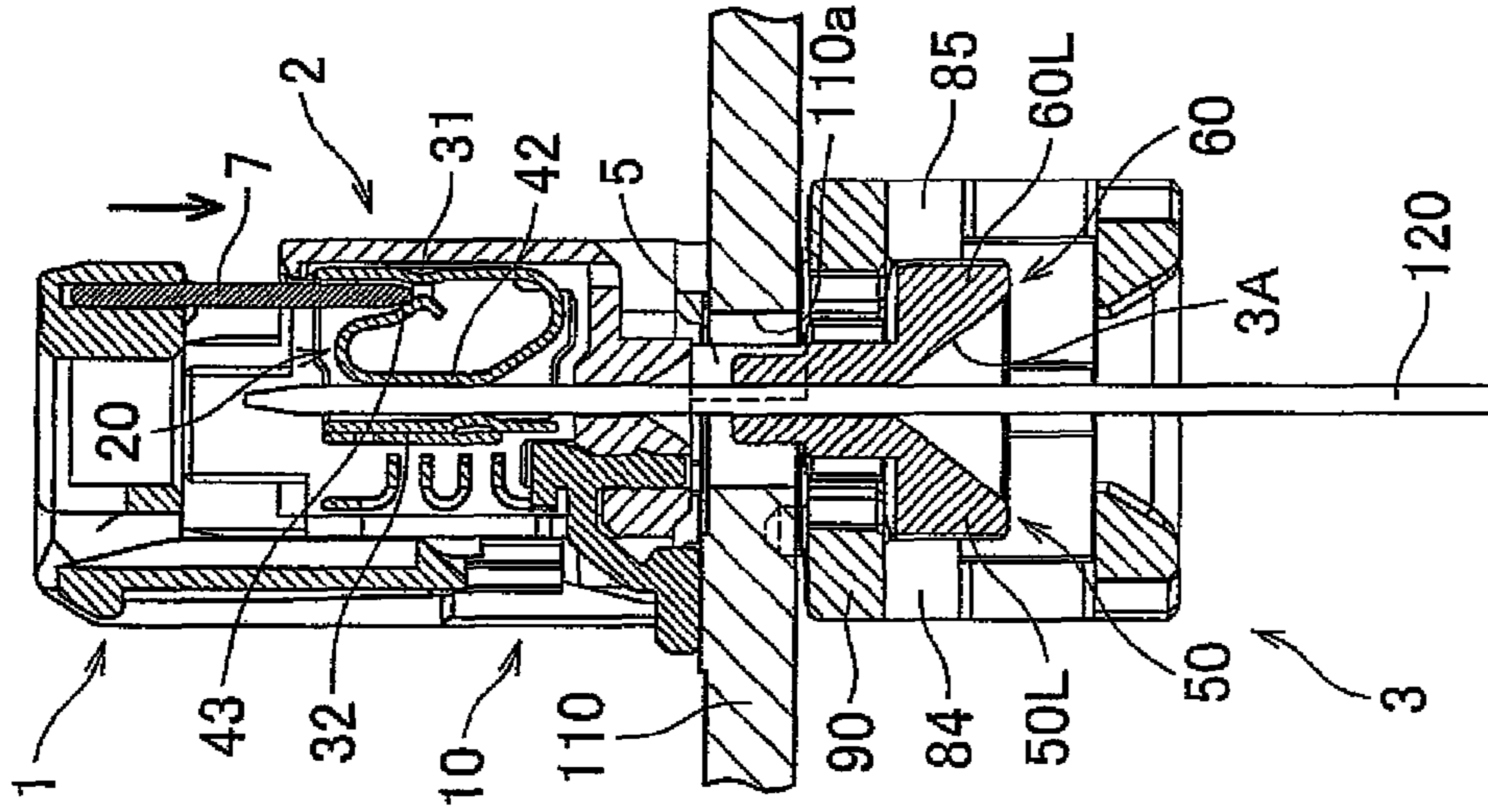
FIG.8B CLOSE STATE
