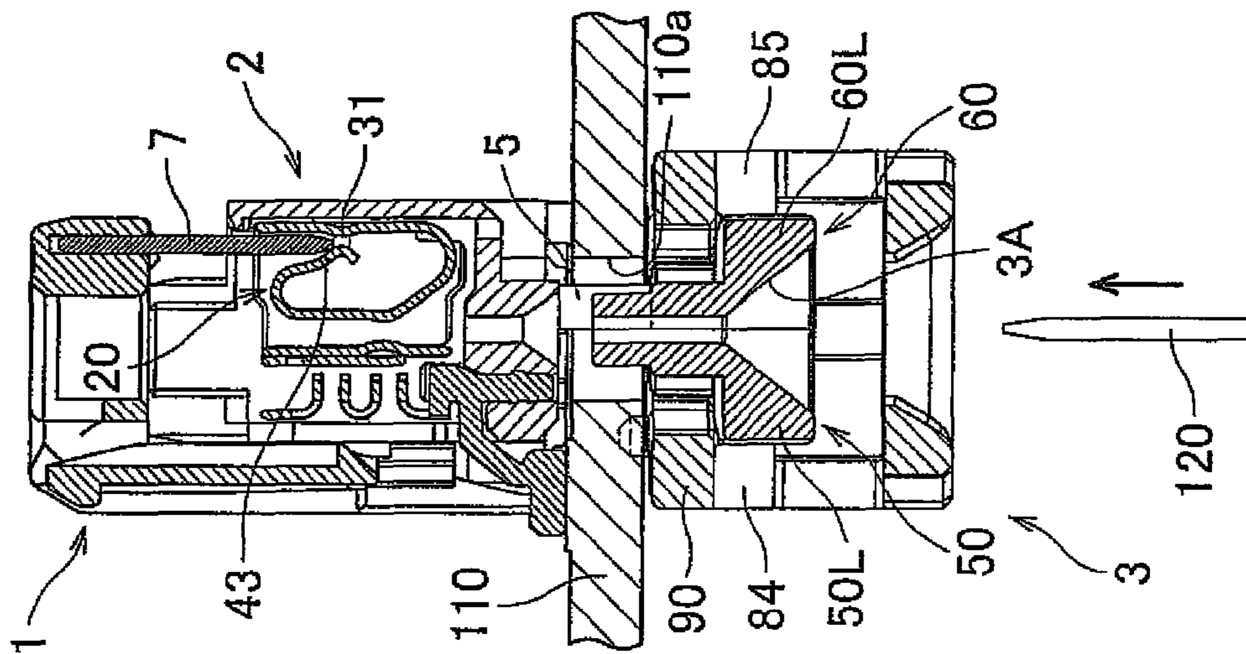
FIG.8A CLOSE STATE
