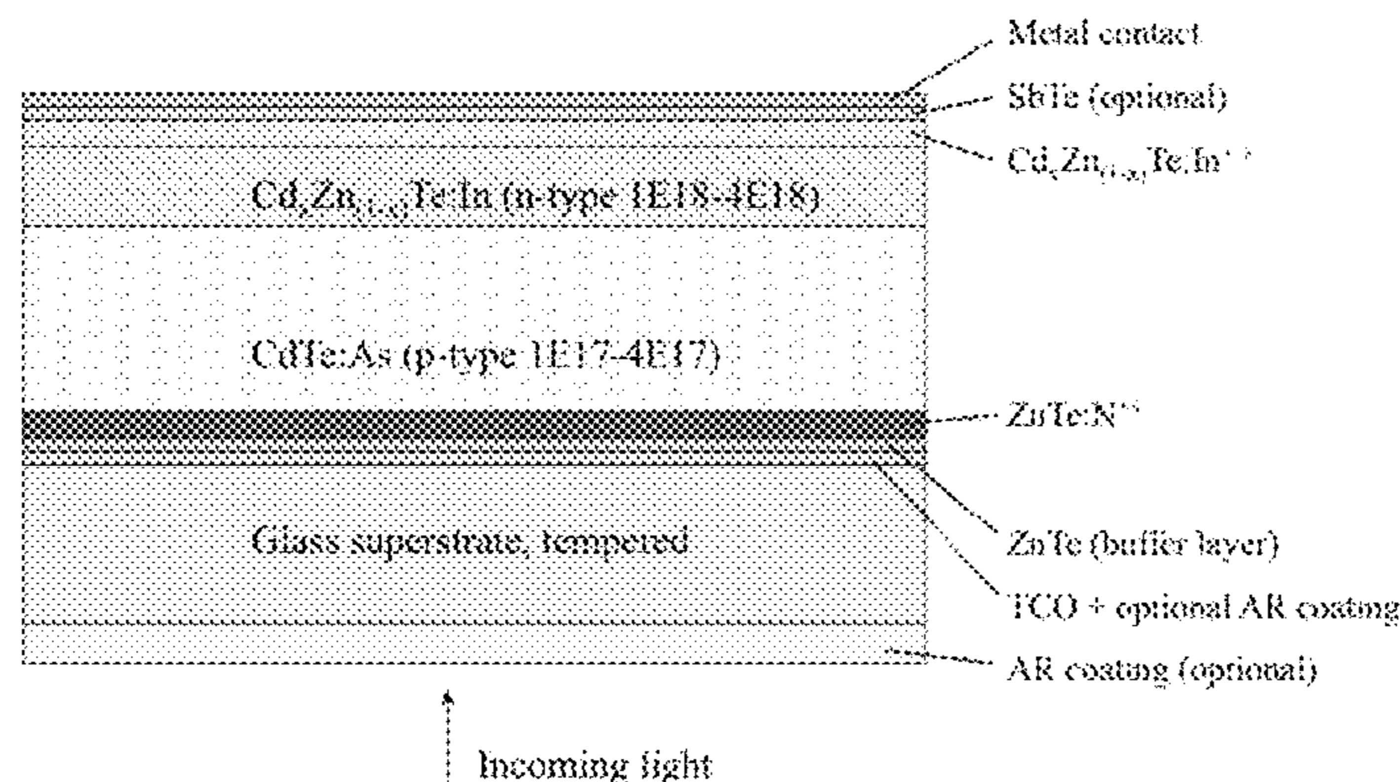
“Reversed” p-n junction solar cell
