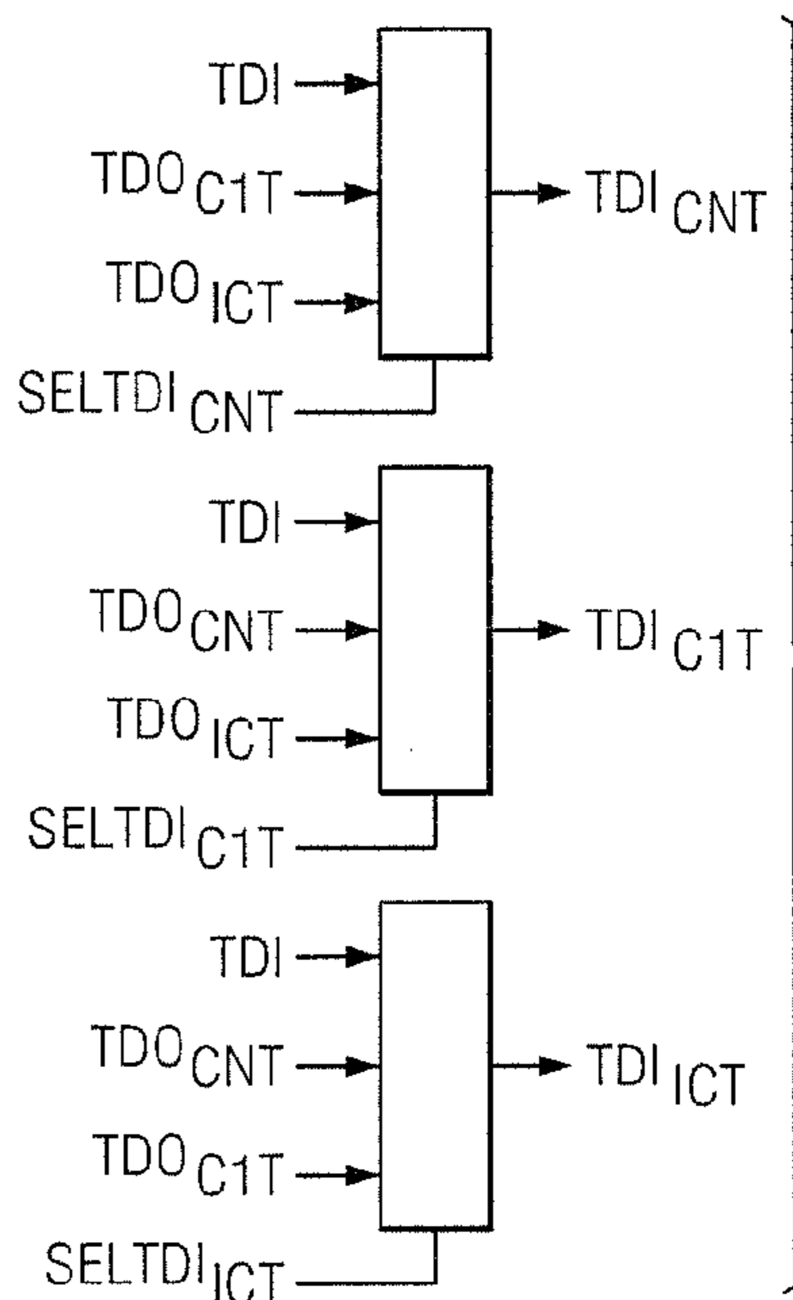
FIG. 6 (PRIOR ART)
