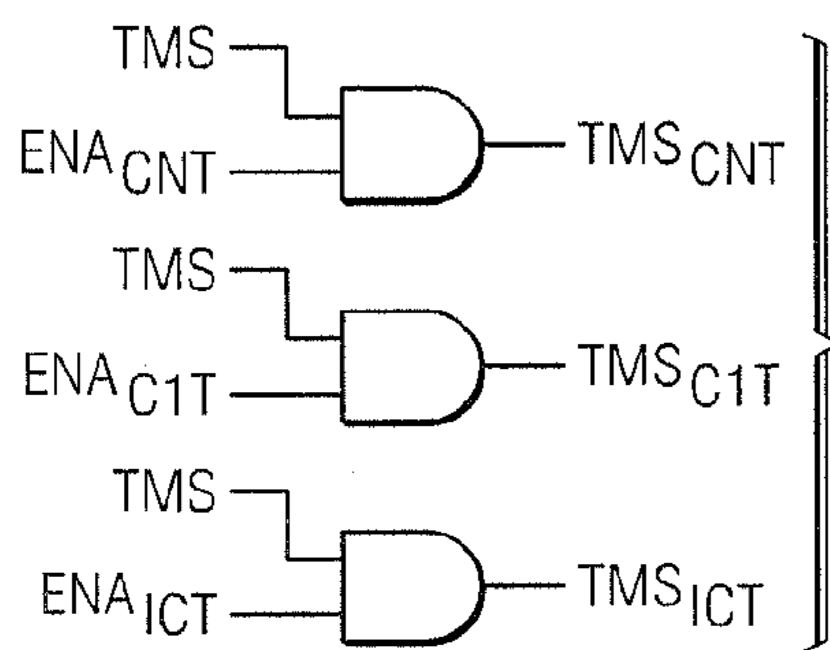
FIG. 5 (PRIOR ART)
