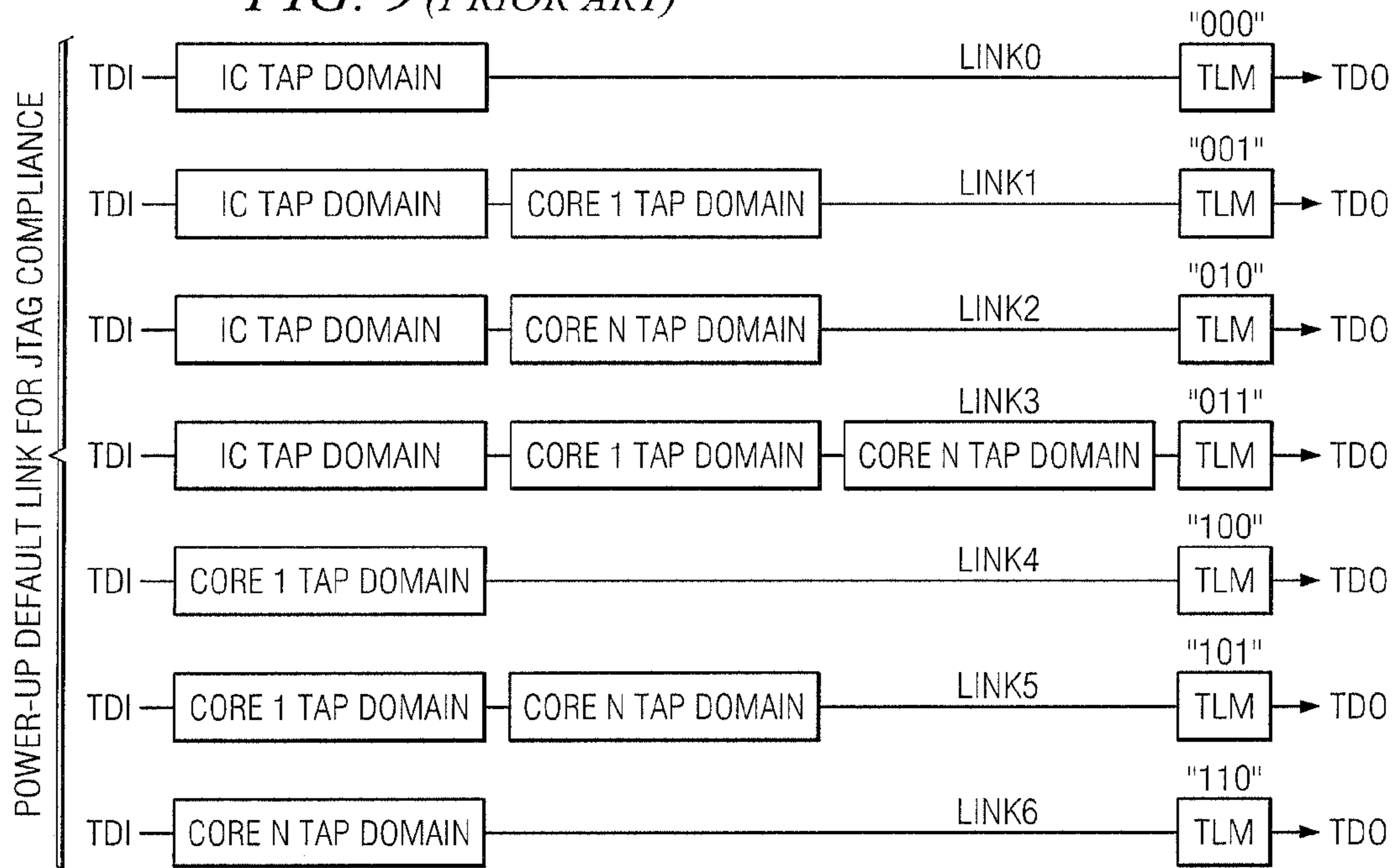
FIG. 9 (PRIOR ART)
