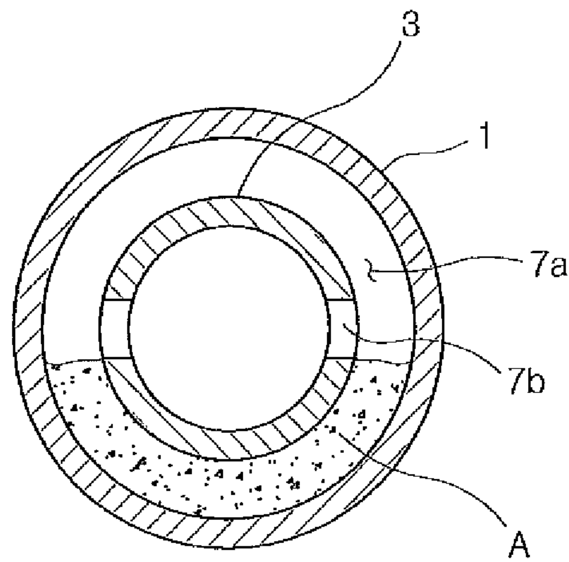
Fig. 2 (Prior Art)
