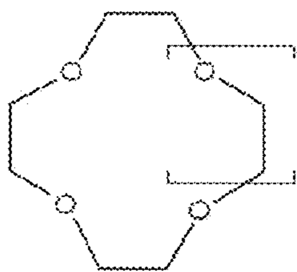
1-3 Crown ethers
