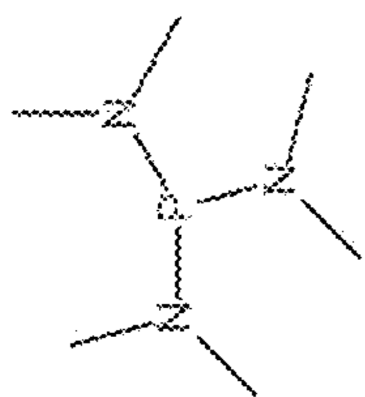
Tris(dimethylamino)phosphine
