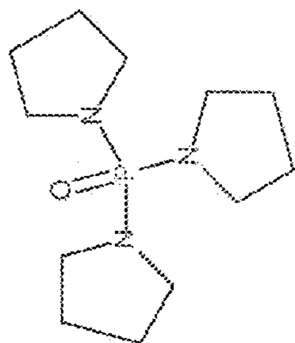
Tris(dimethylamino)phosphine
