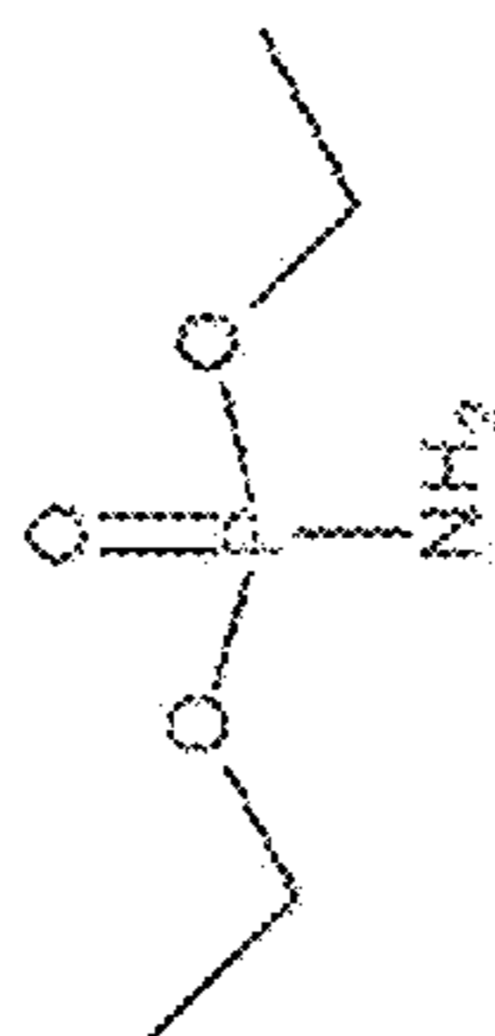
Diethyl phosphoramidate
