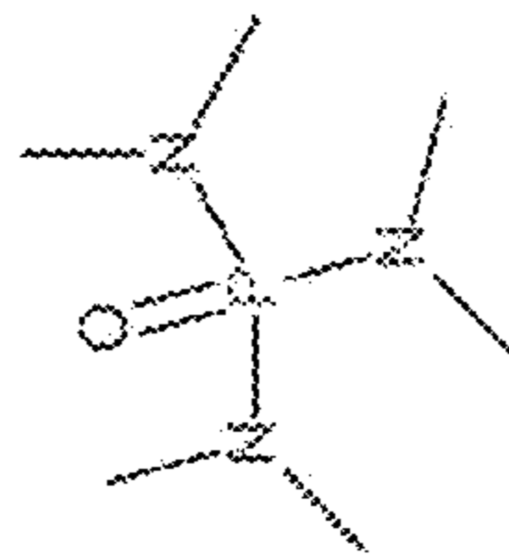
Hexamethylphosphoramide
