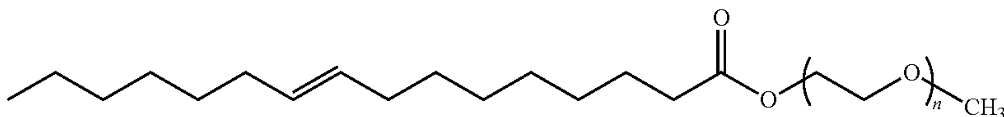
C16-8: C16 11EO eFAME
