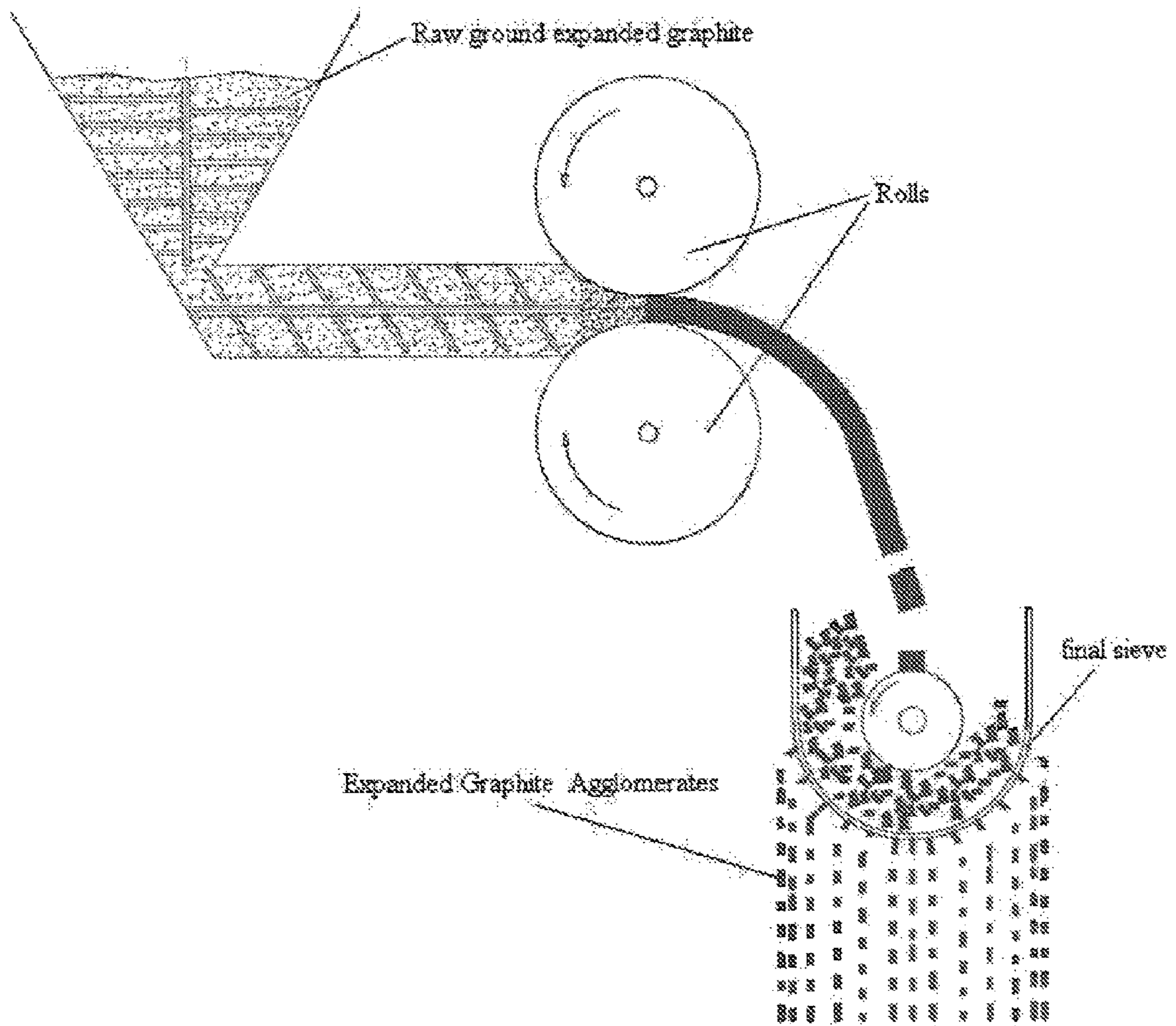
Figure 15: Process for Preparing Ground Expanded Graphite Agglomerates
