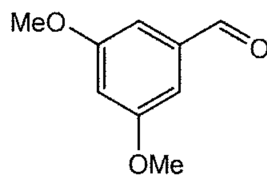
3,5-dimethoxybenzaldehyde
