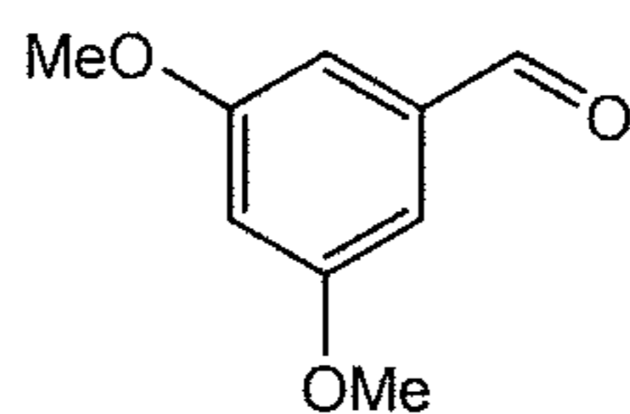
3,5-dimethoxybenzaldehyde
