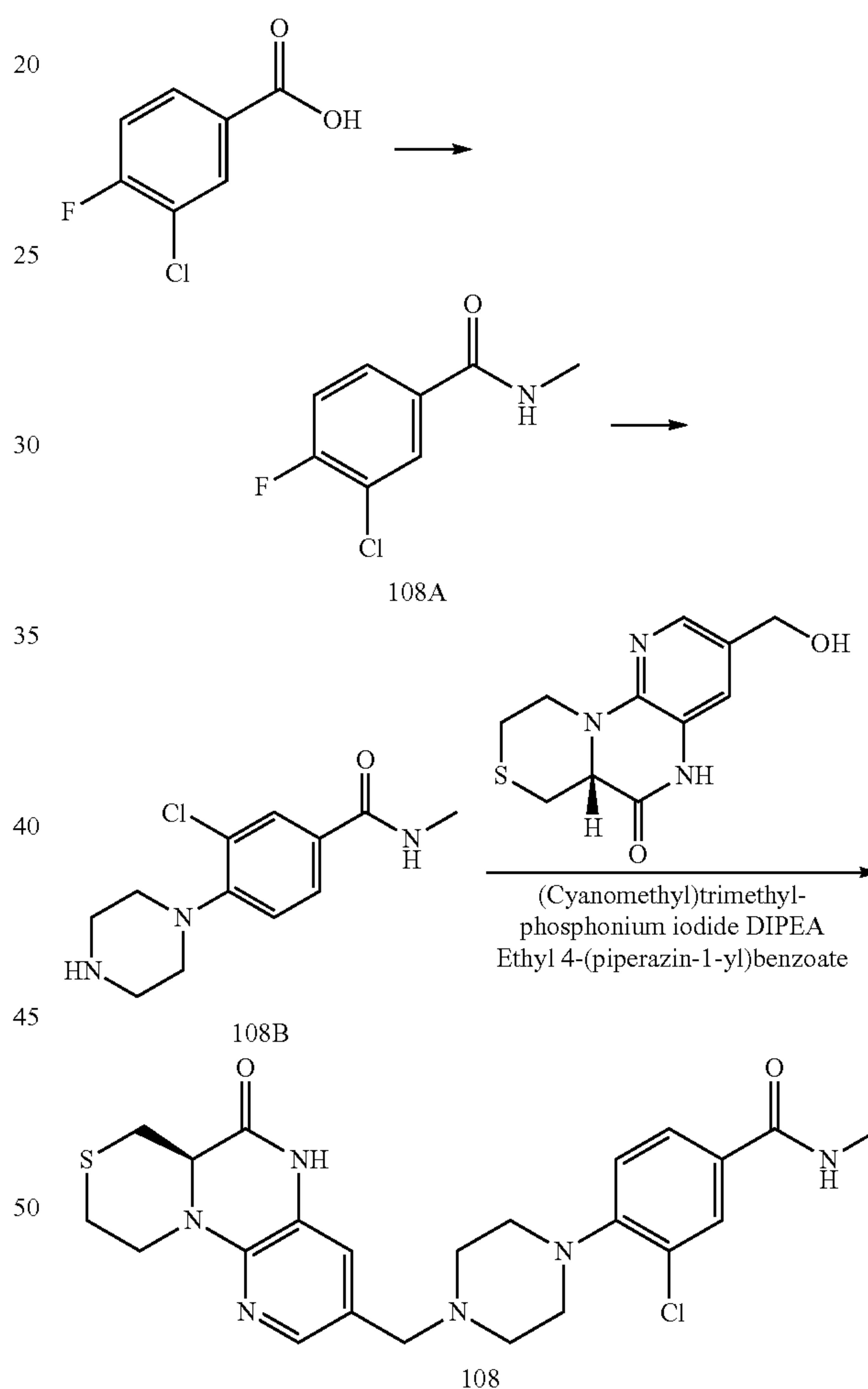
Compound 108: (R)-3-chloro-N-methyl-4-(4-((6-oxo-5,6,6a,7,9,10-hexahydropyrido[3,2-e][1,4]thiazino[4,3-a]pyrazin-3-yl)methyl)piperazin-1-yl)benzamide
