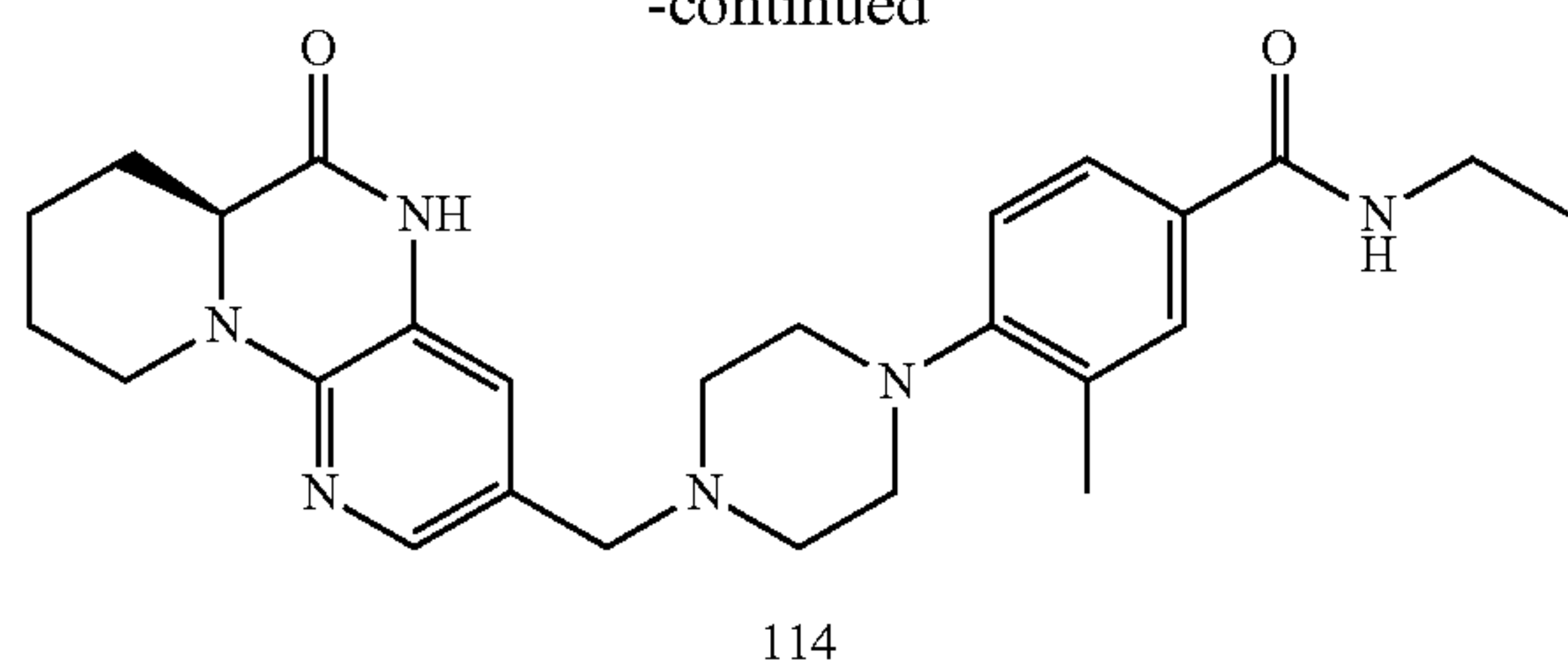
Compound 114A:
