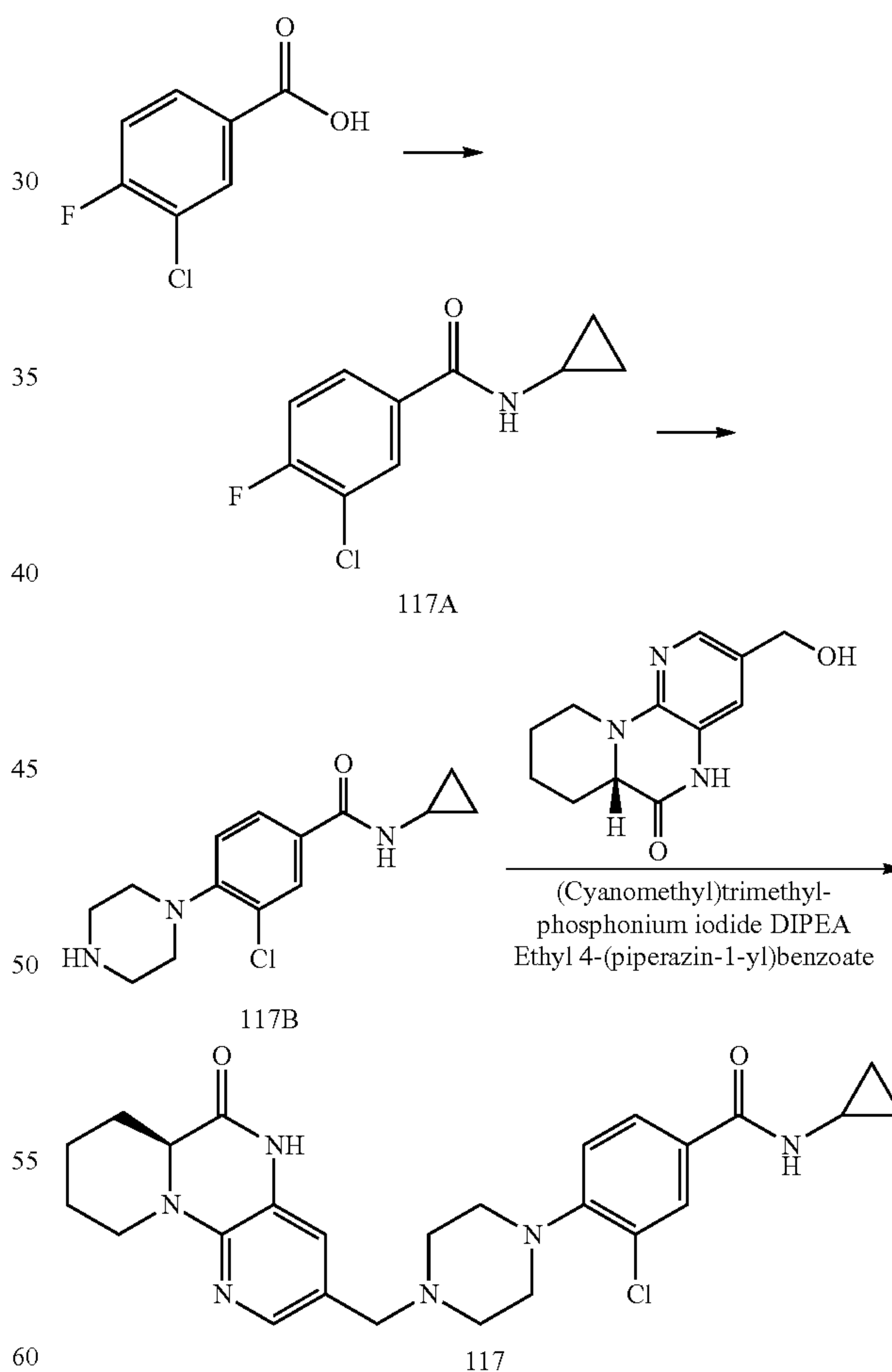
Compound 117A:
