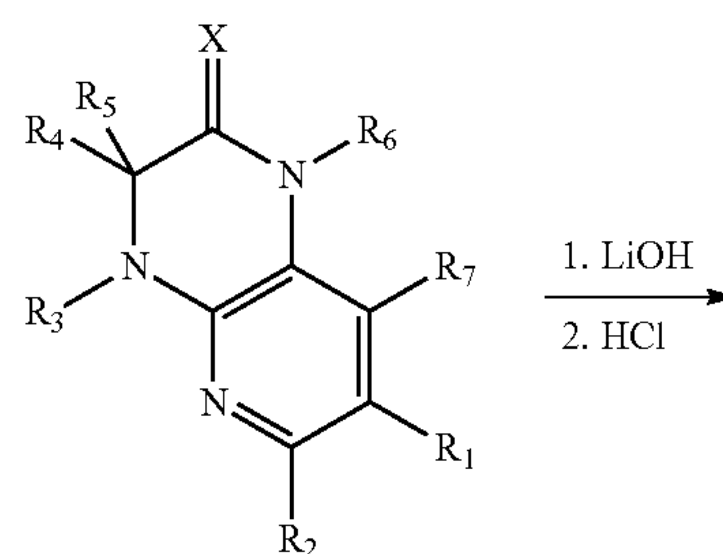
Scheme 3
