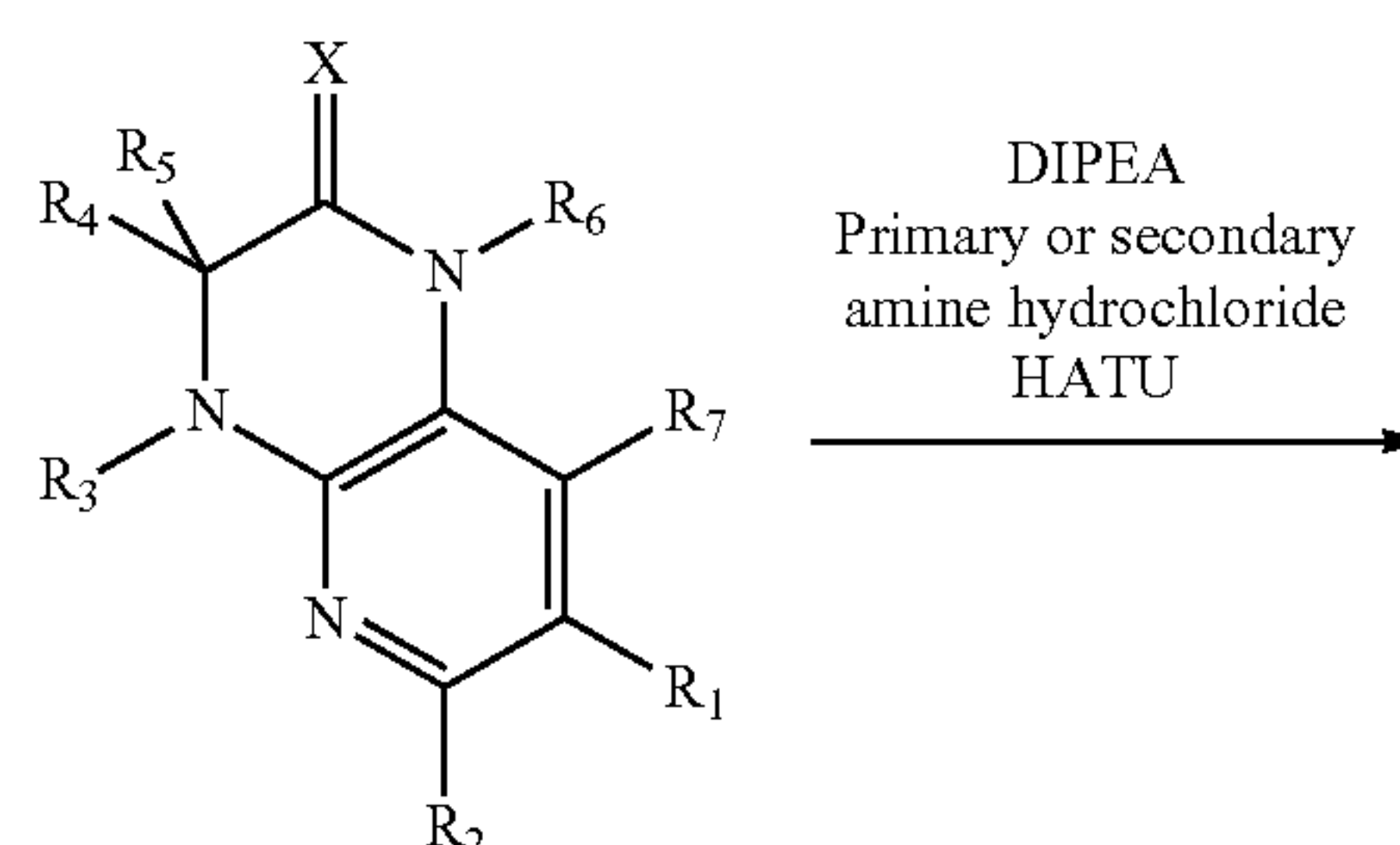
Scheme 4
