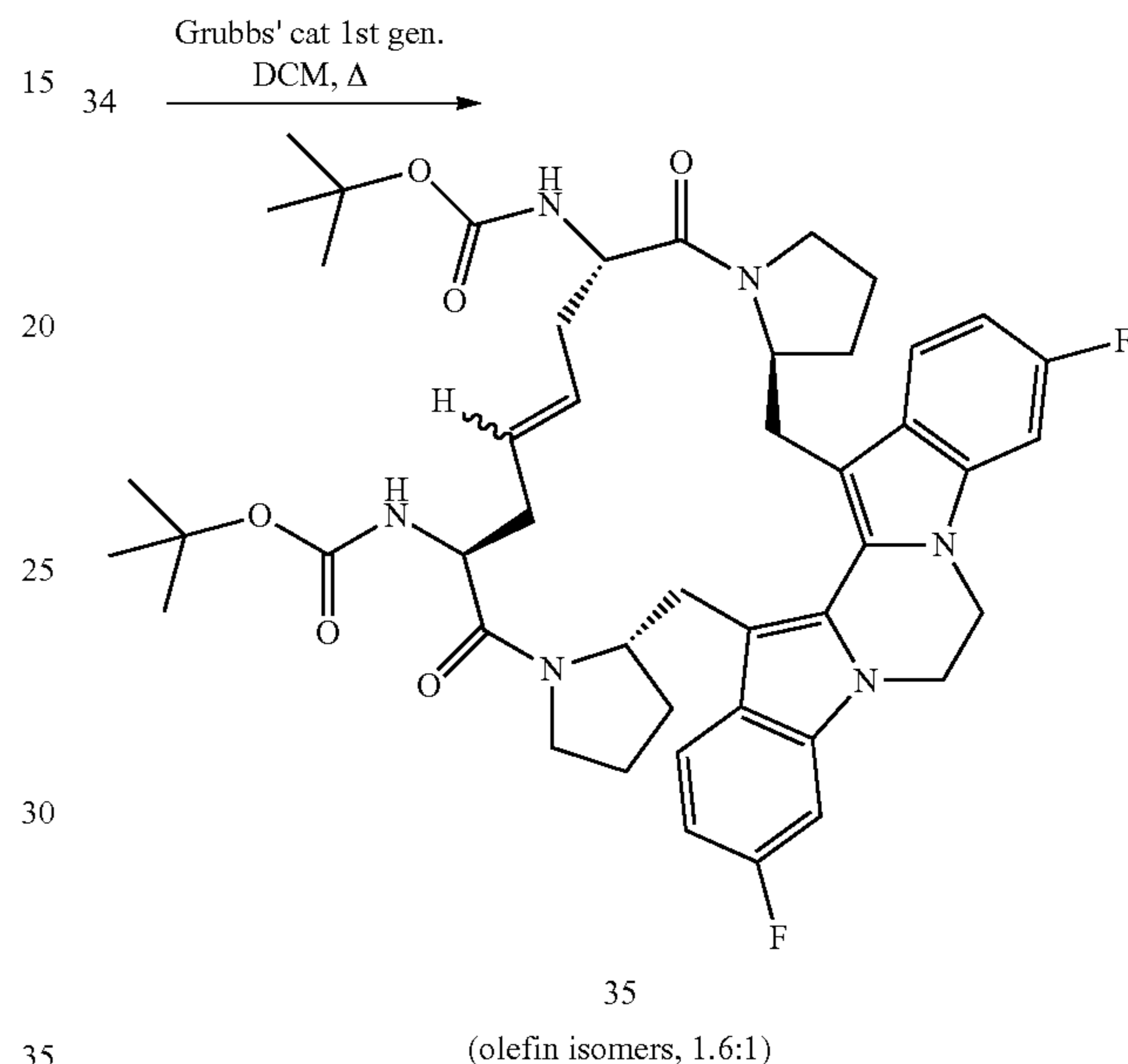
Scheme XV
