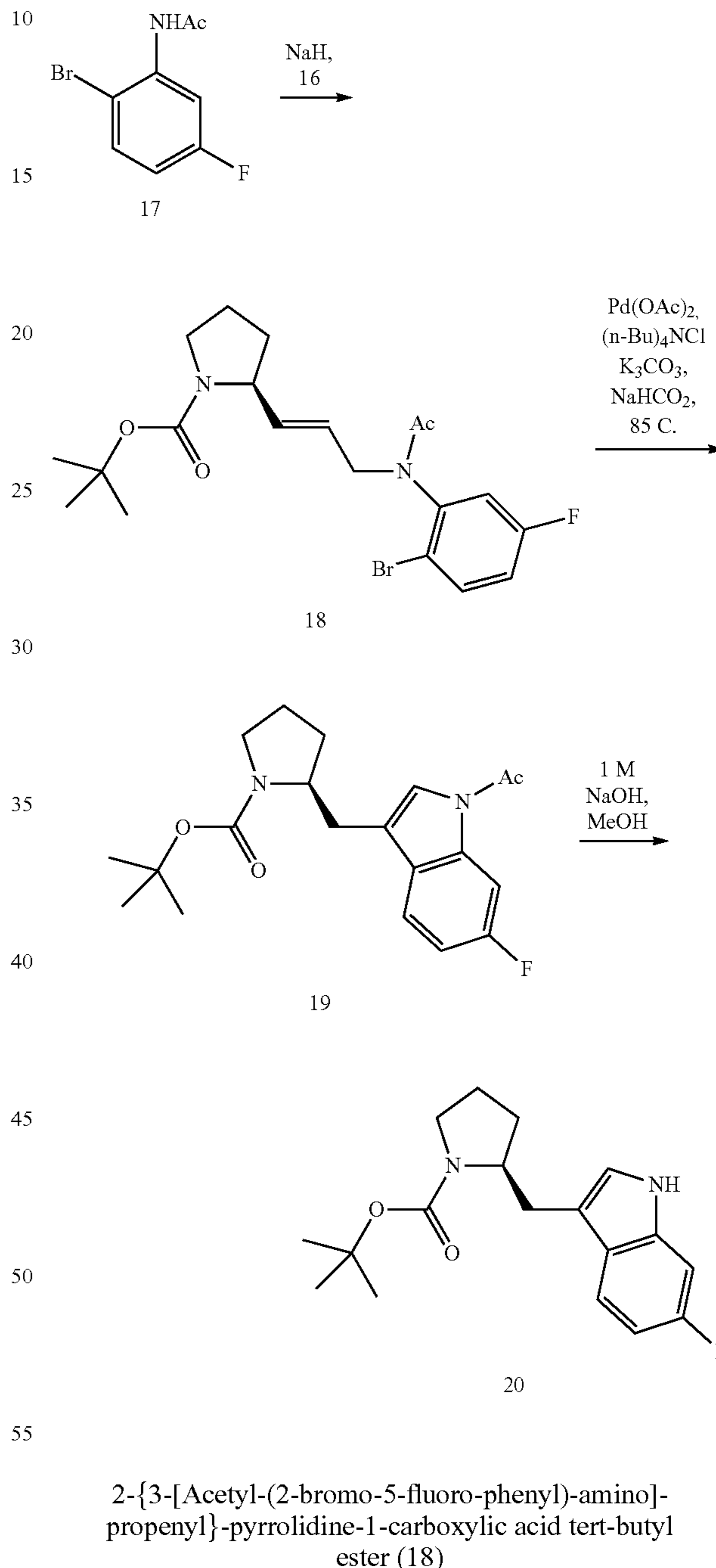
Scheme VII
