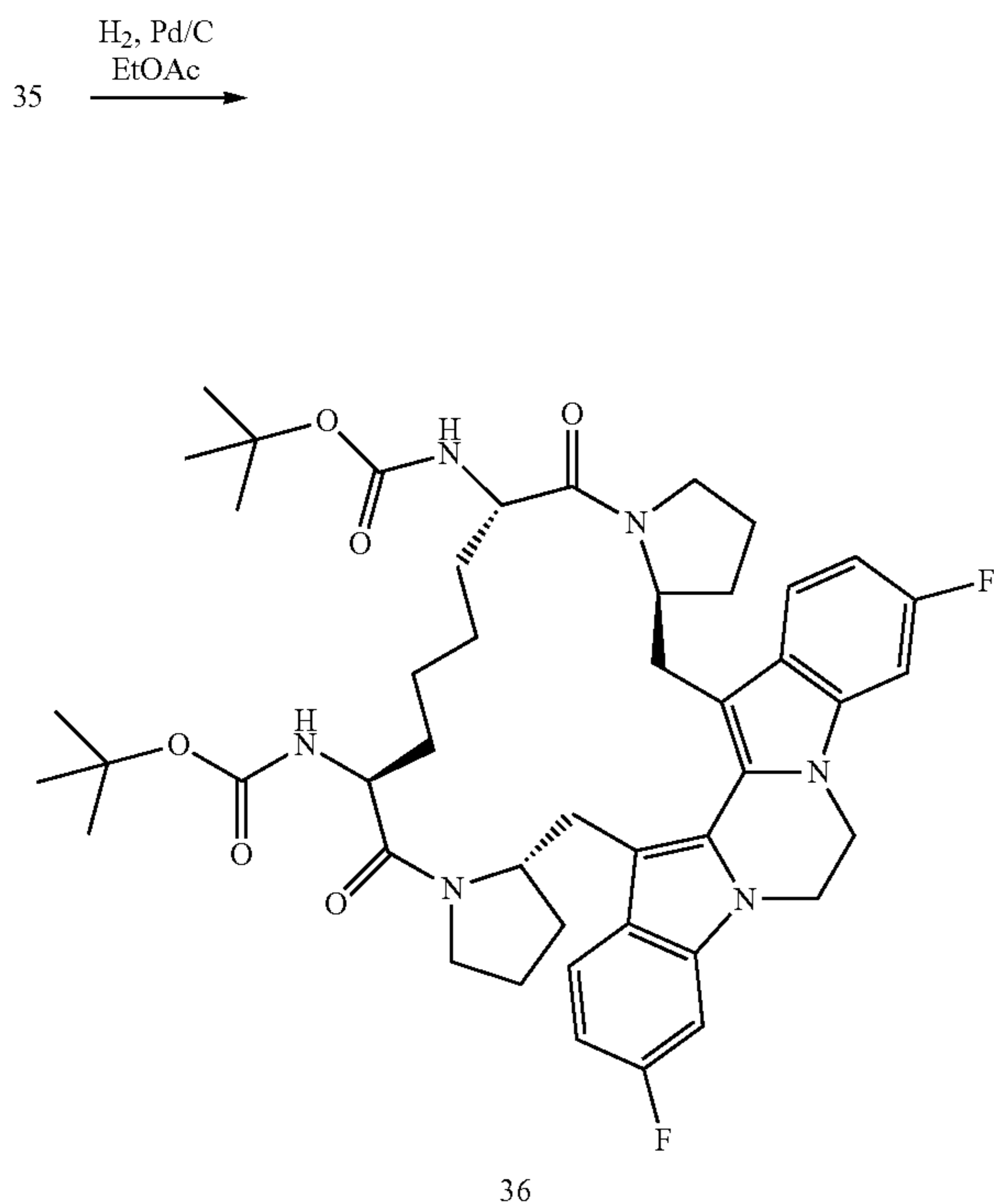
Scheme XVI
