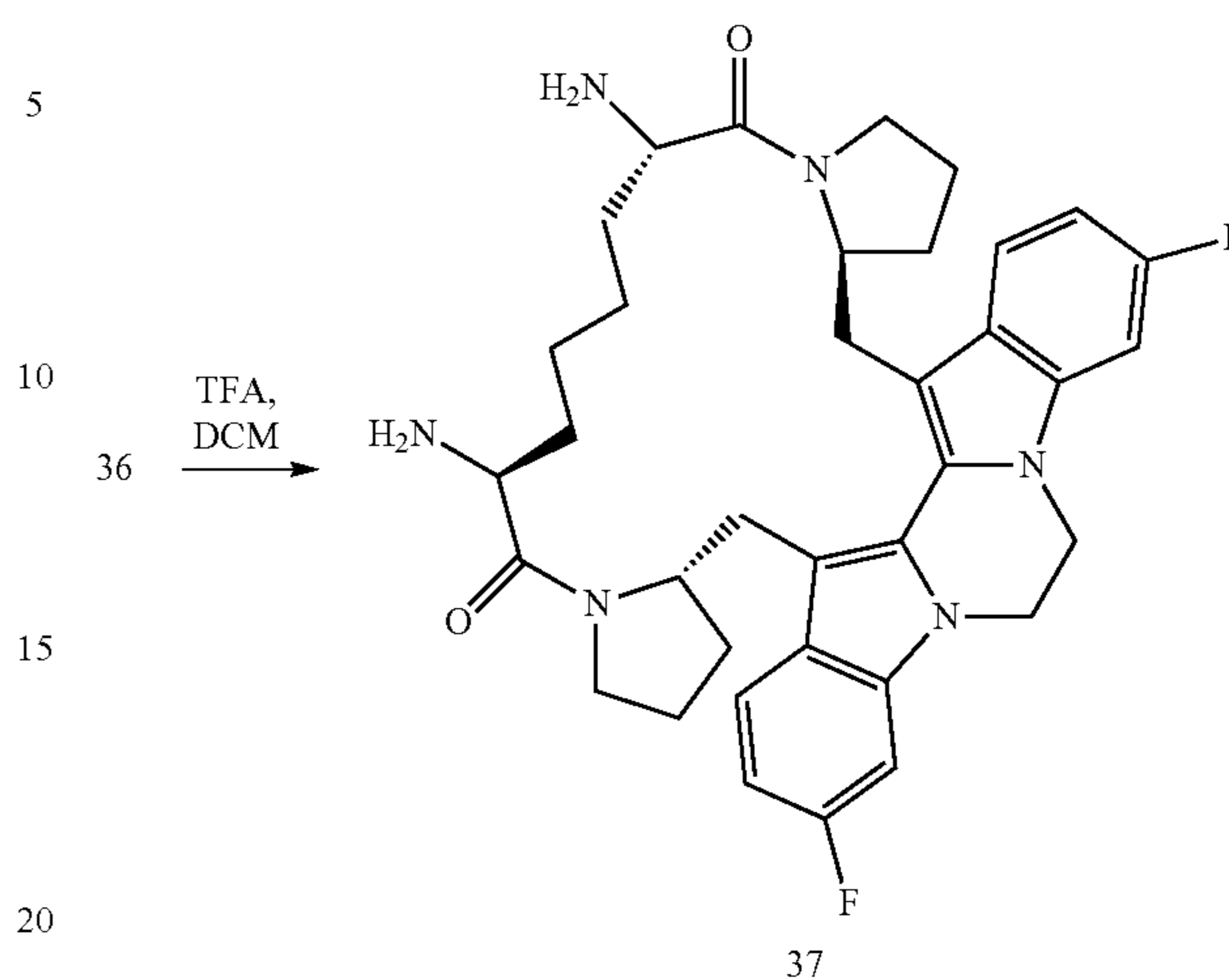
Scheme XVII
