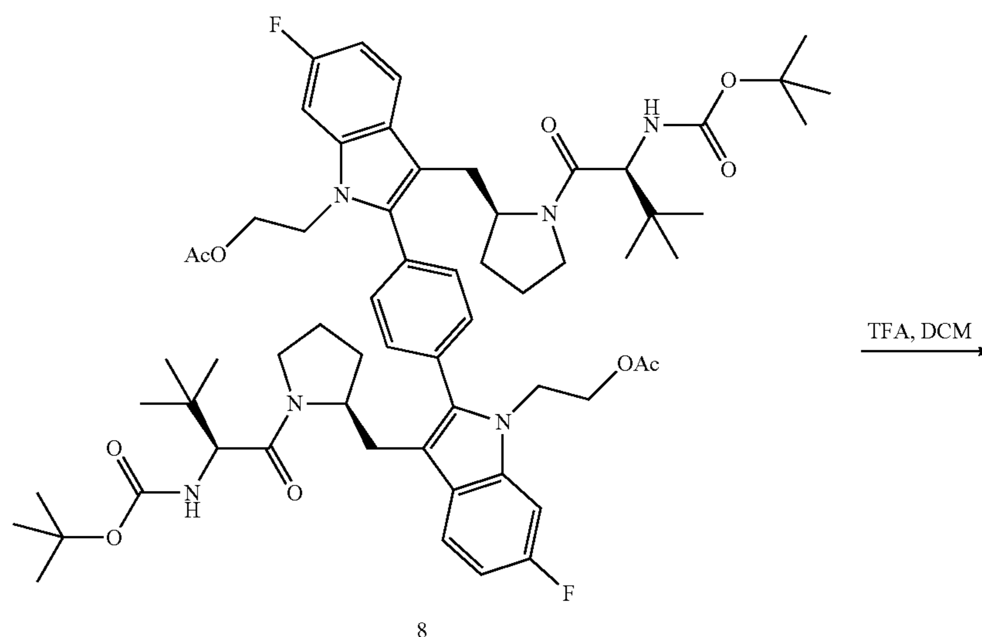
Scheme IV
