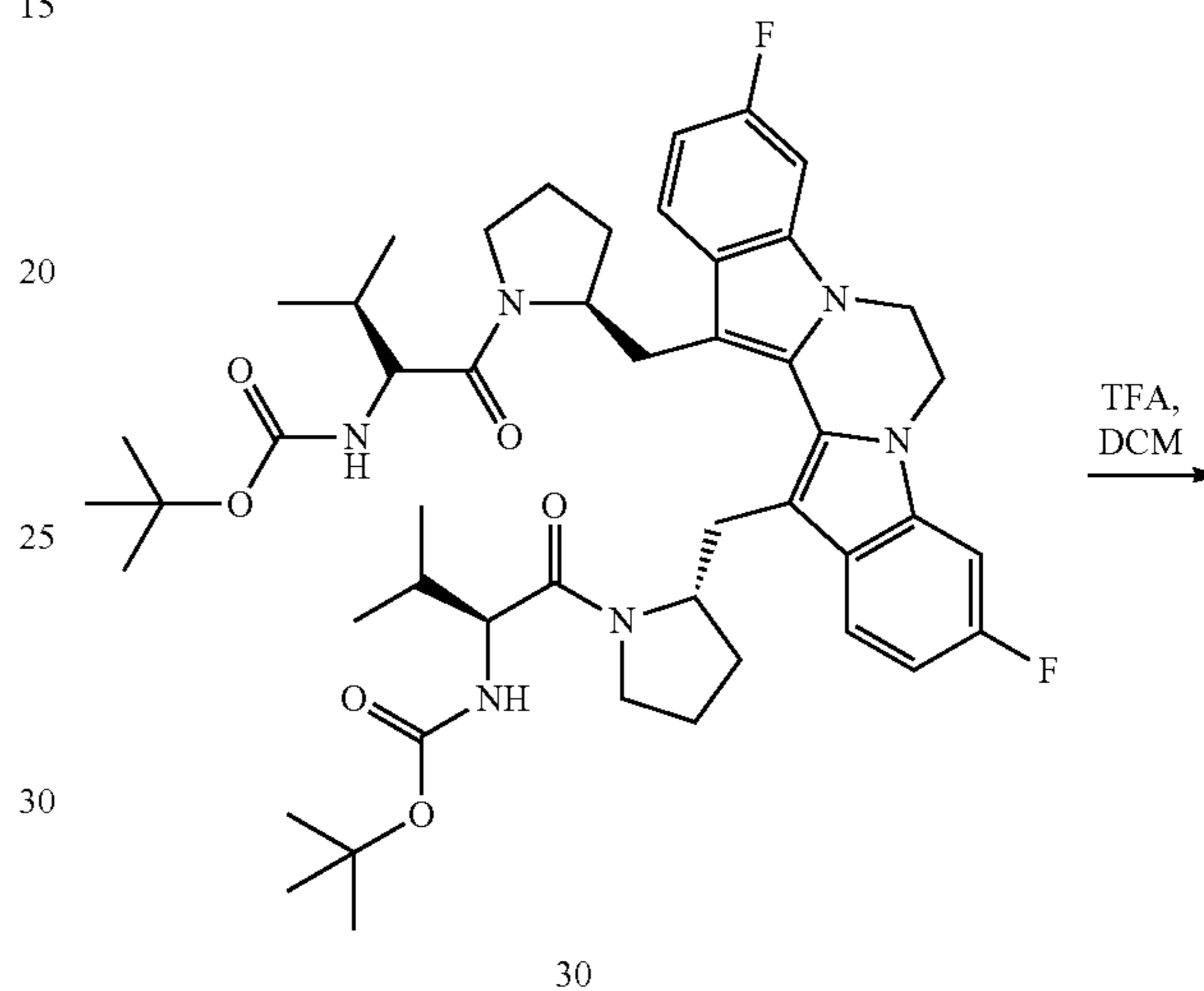
Scheme XII
