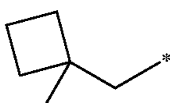
1-methylcyclobutylmethyl
