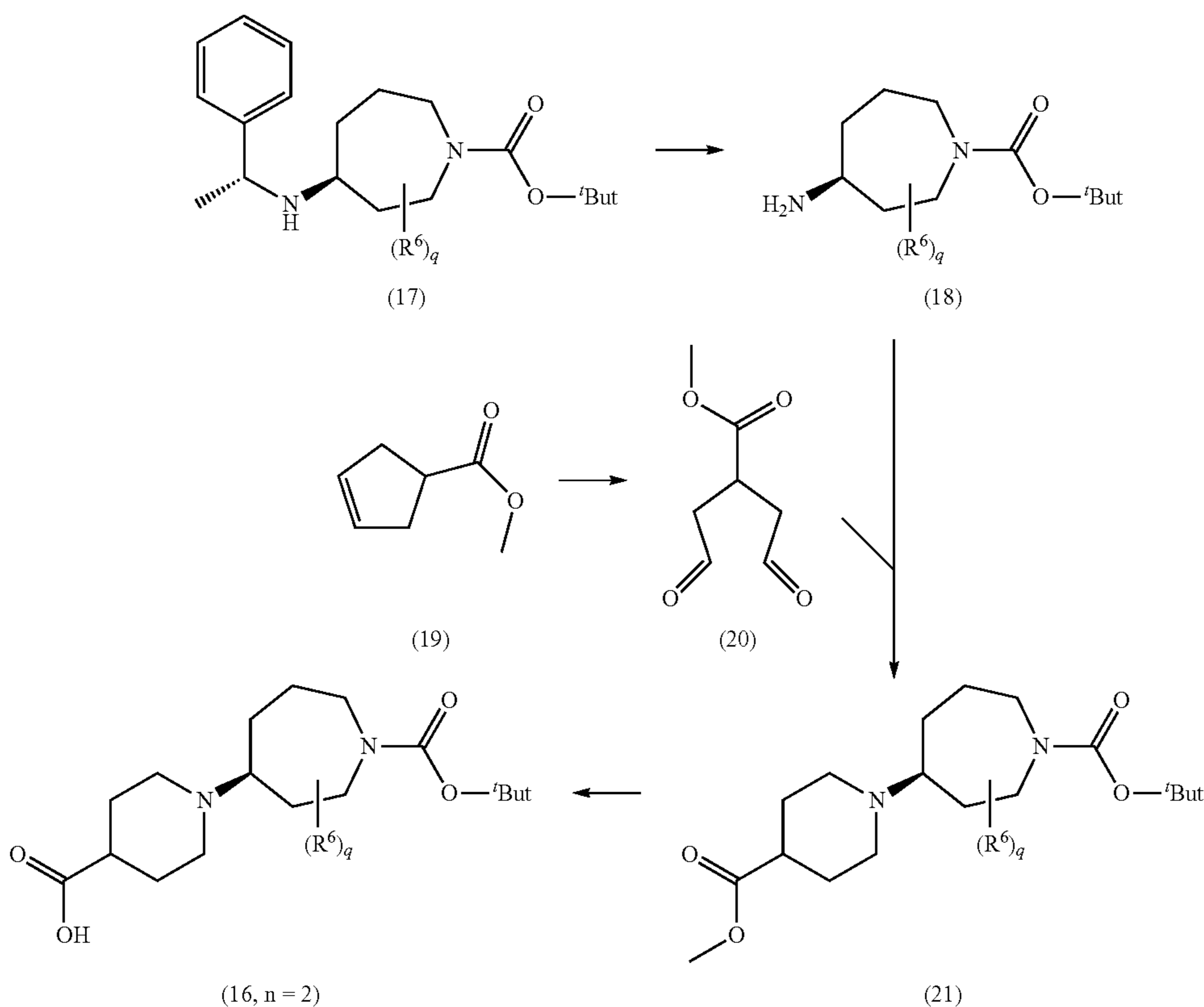
Scheme 3
