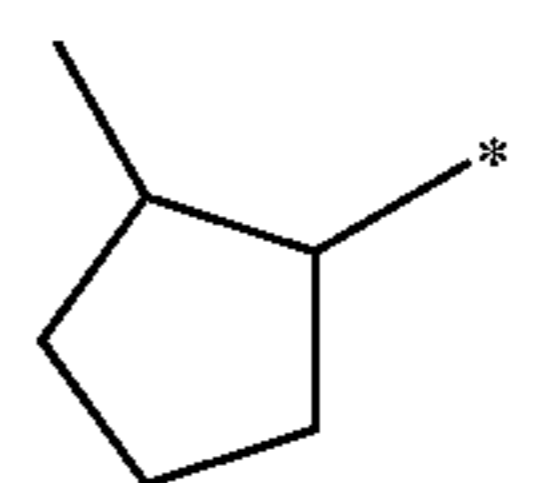
2-methylcyclopentyl
