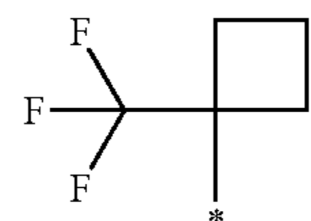
1-trifluoromethylcyclobutyl
