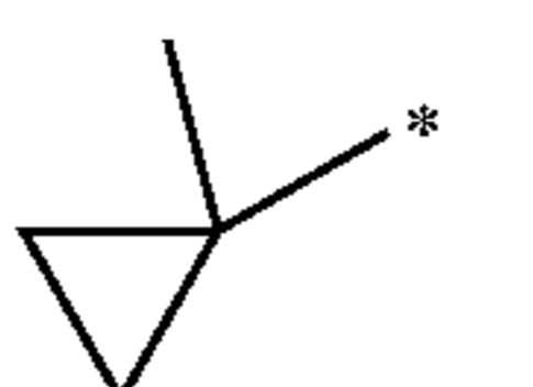
1-methylcyclopropyl
