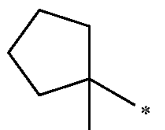
1-methylcyclopentyl
