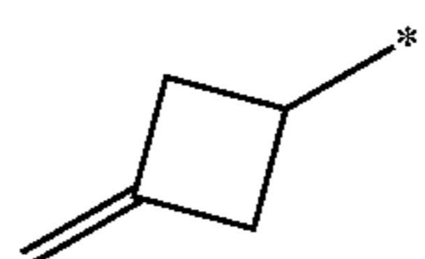
3-methylidenecyclobutyl
