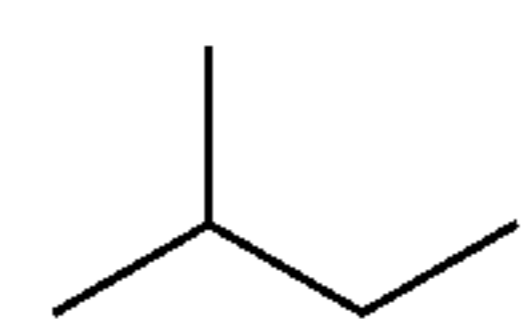
2-methylpropyl
