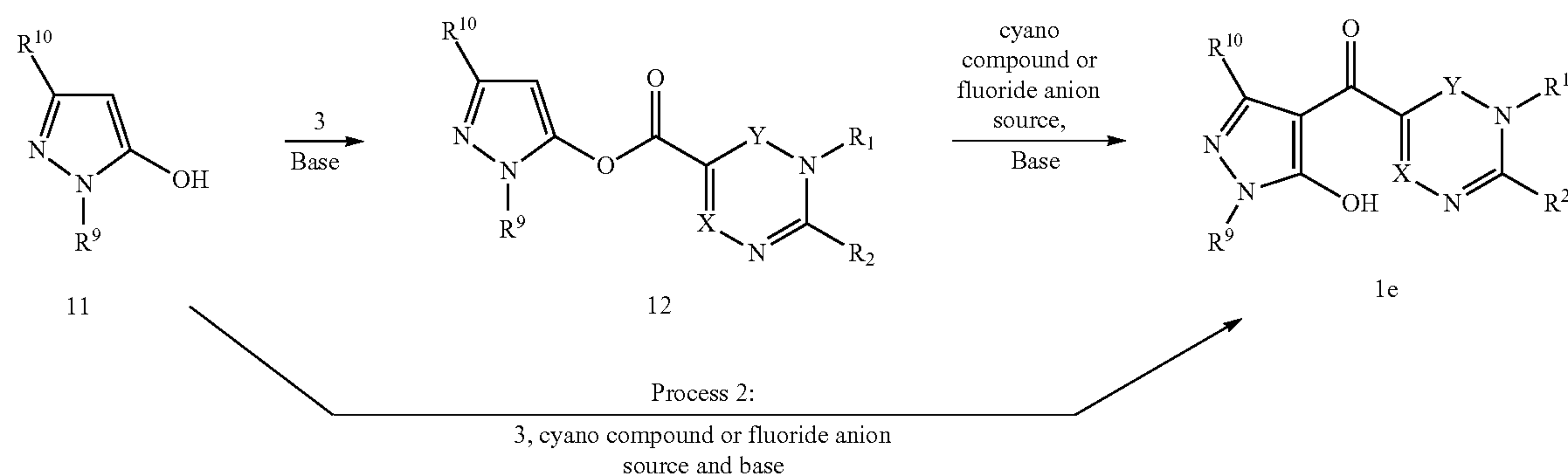
Scheme 7
