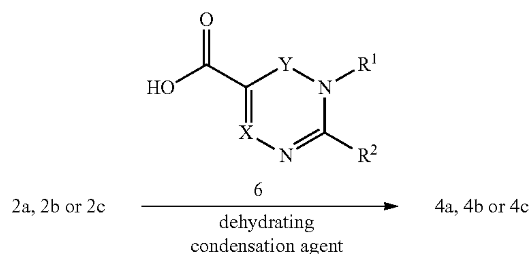
Scheme 3
