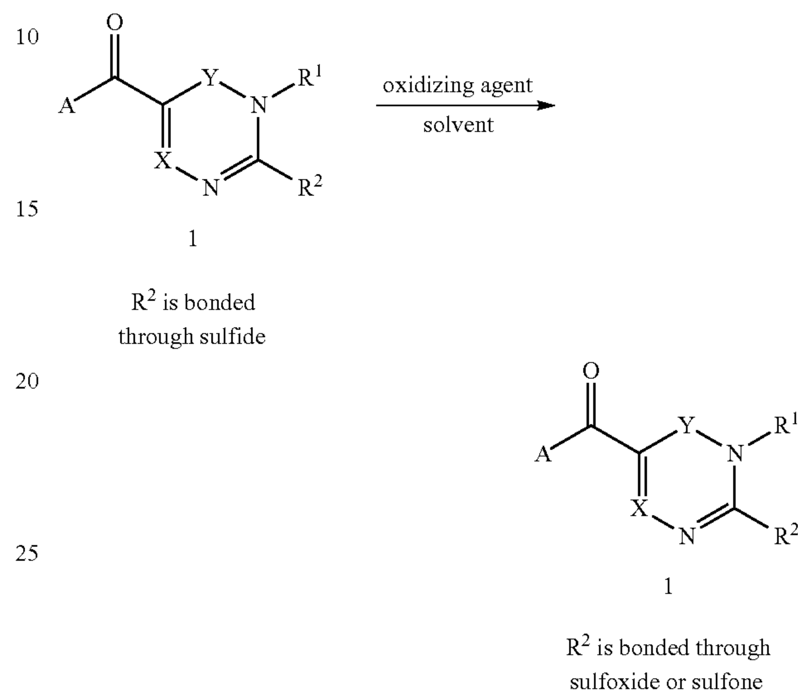
Scheme 11
