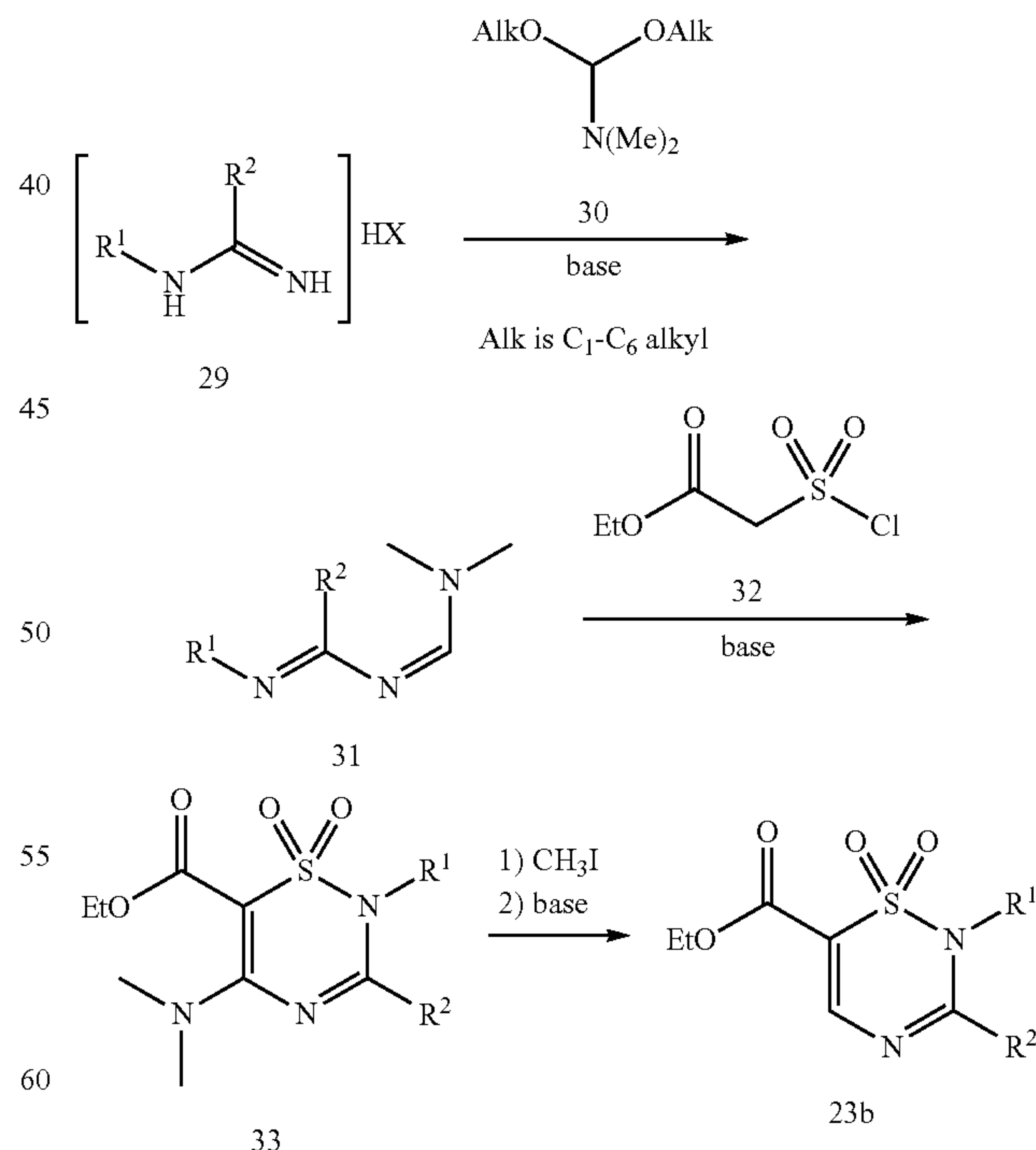
Scheme 17
