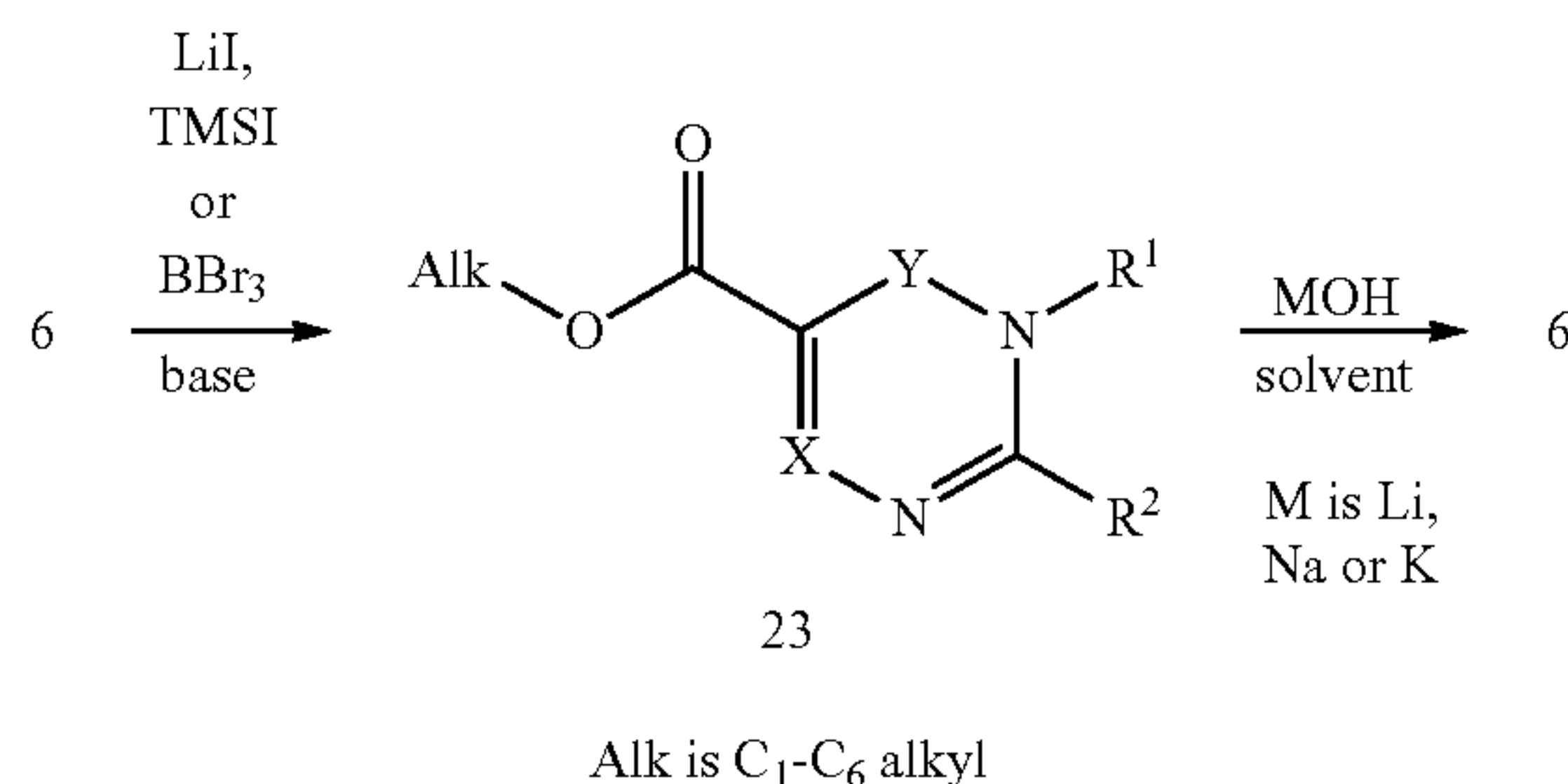
Scheme 13
