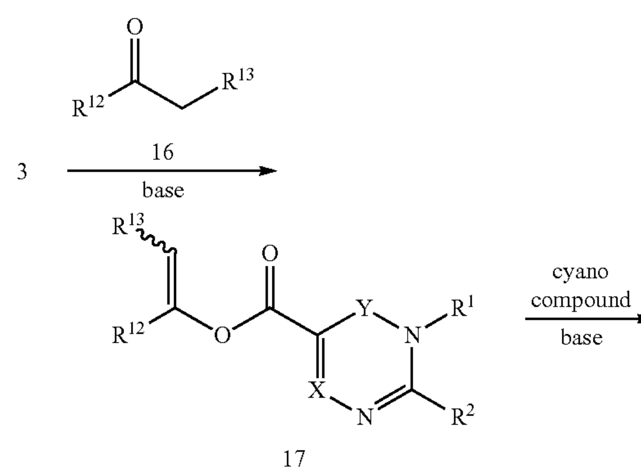
Scheme 9
