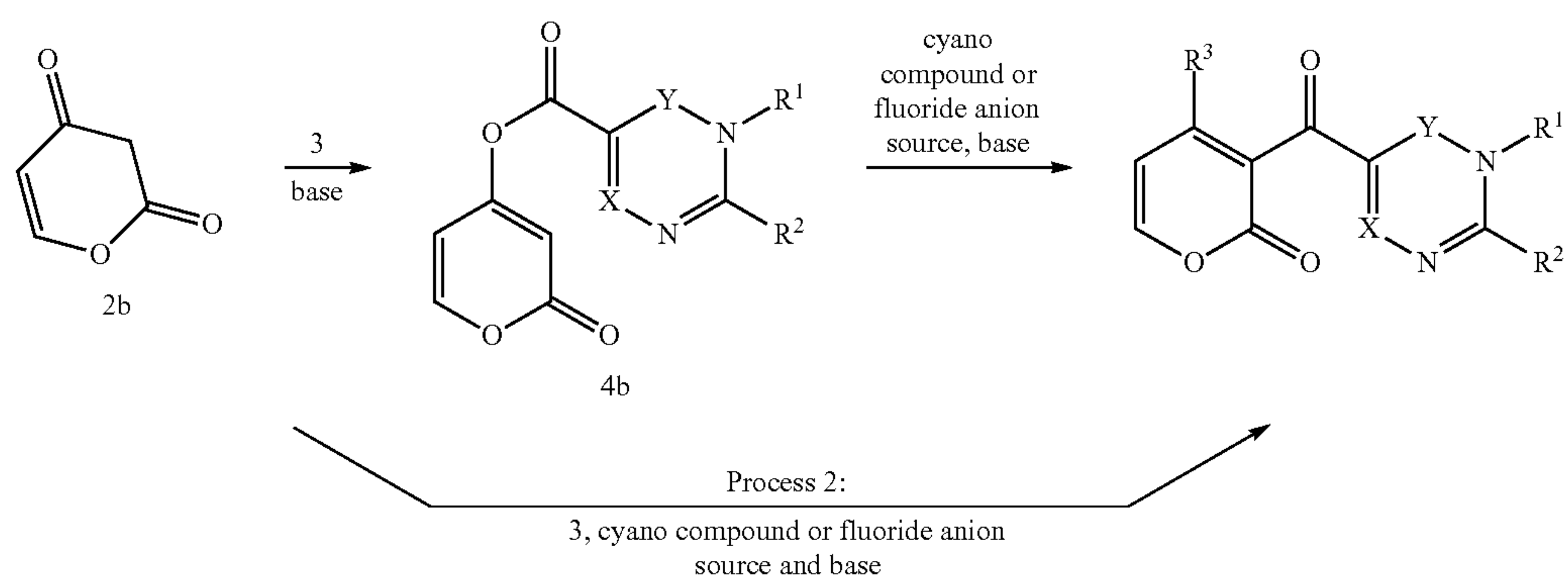
Scheme 1b
