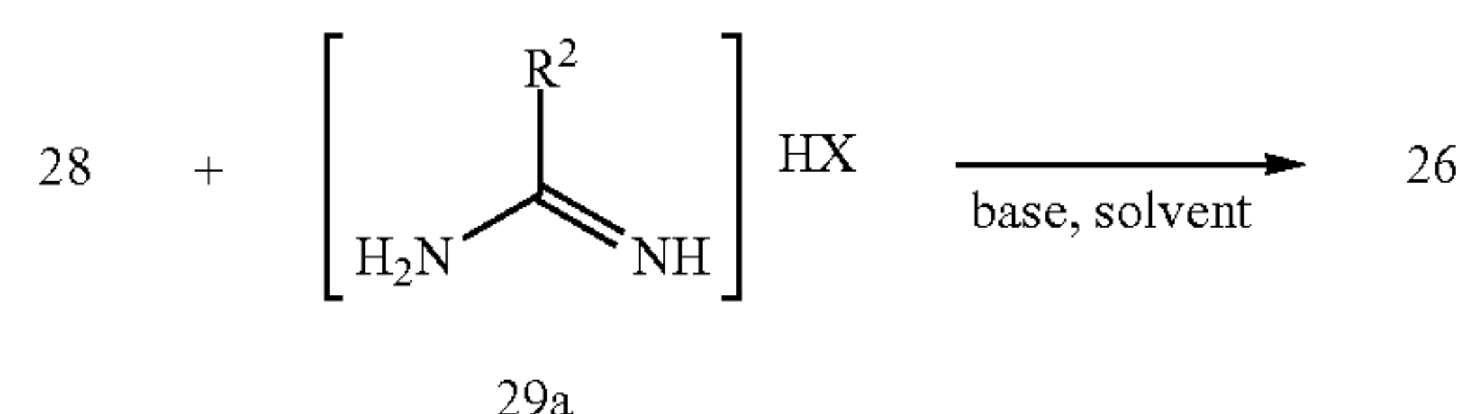
Scheme 16
