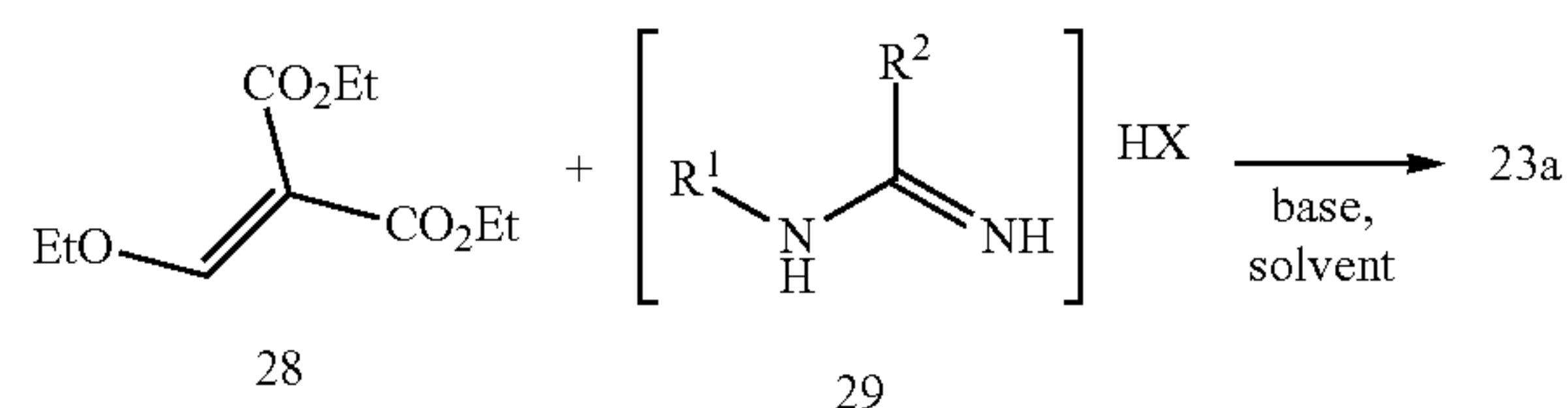
Scheme 15
