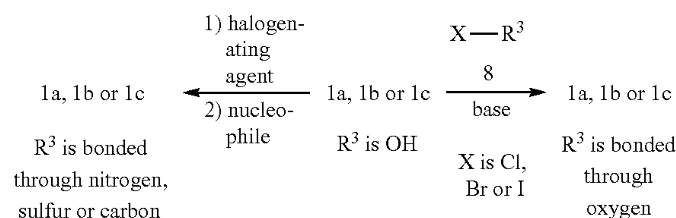
Scheme 5
