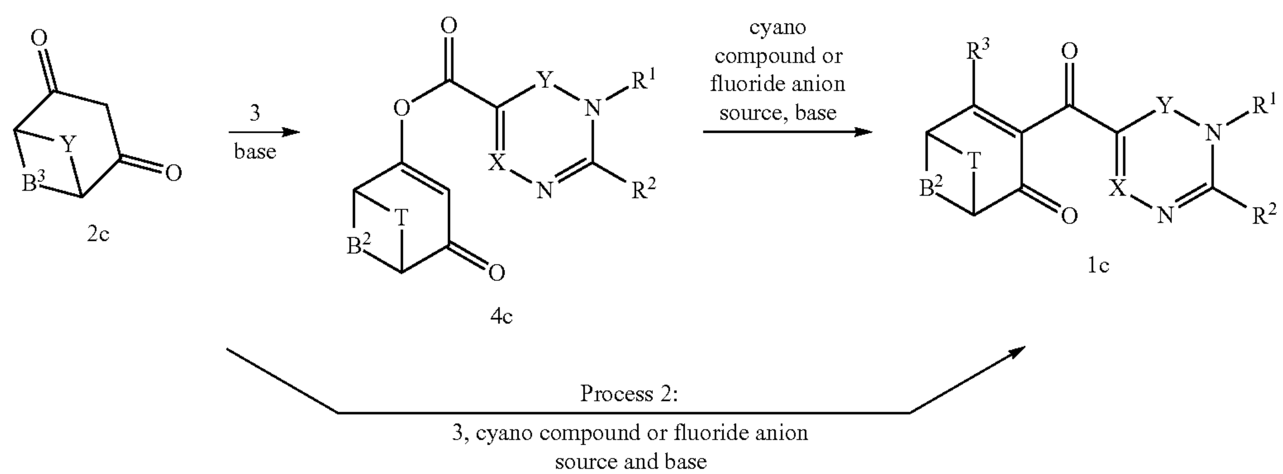
Scheme 1c
