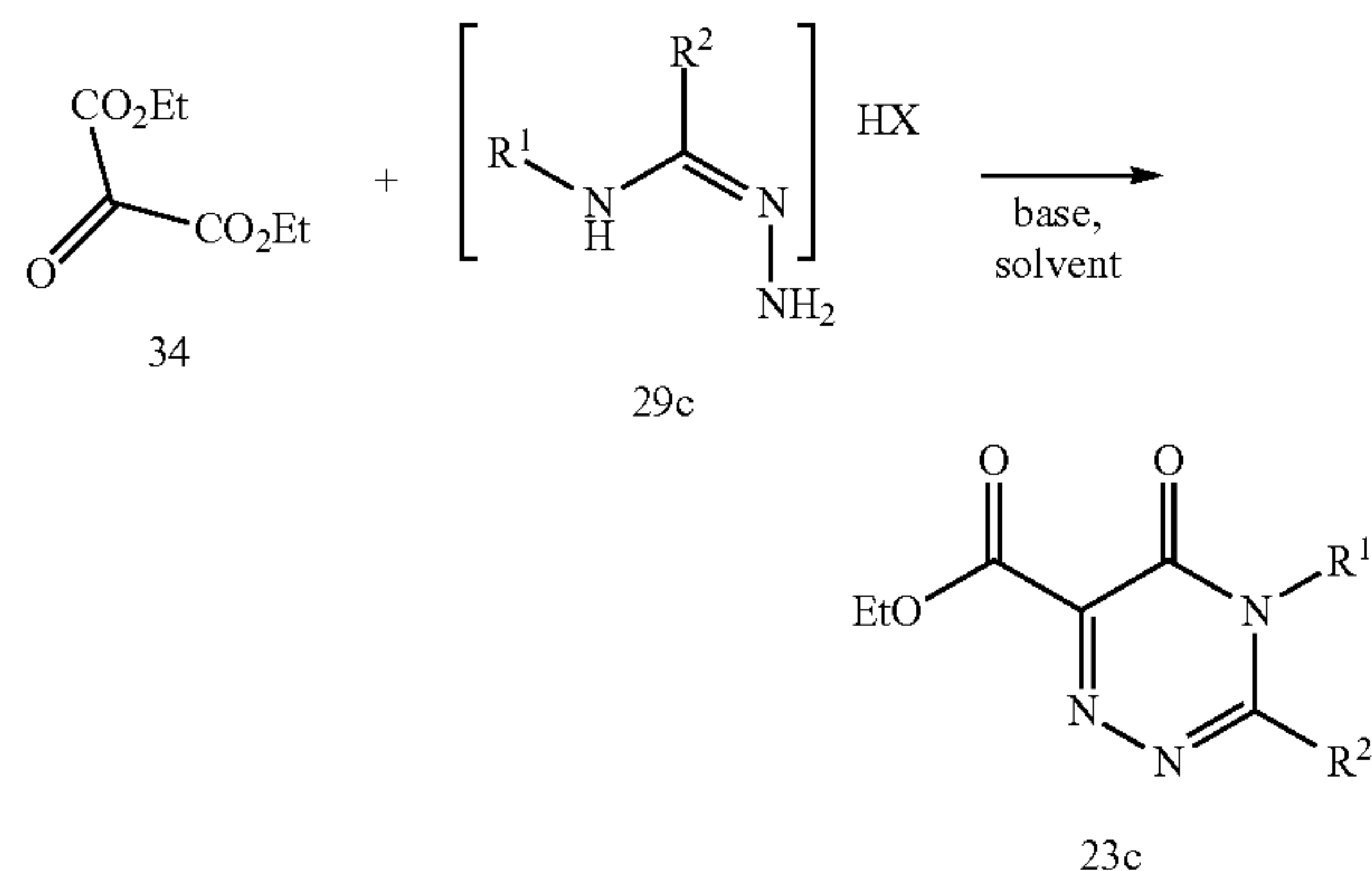
Scheme 18
