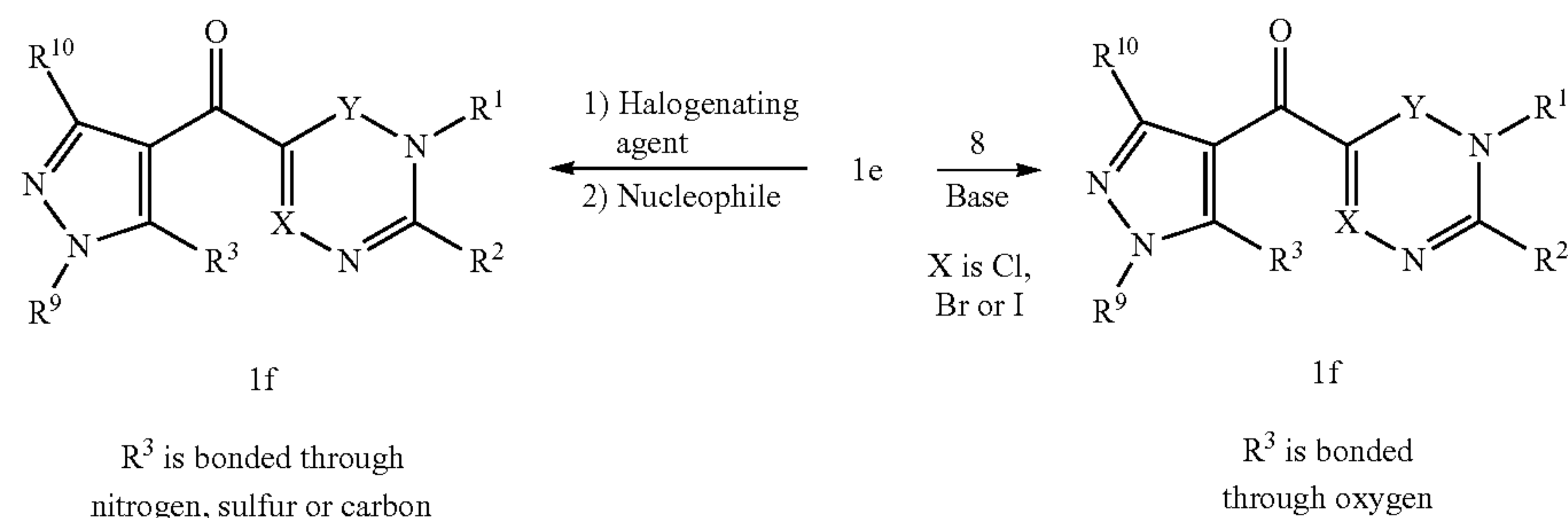
Scheme 8
