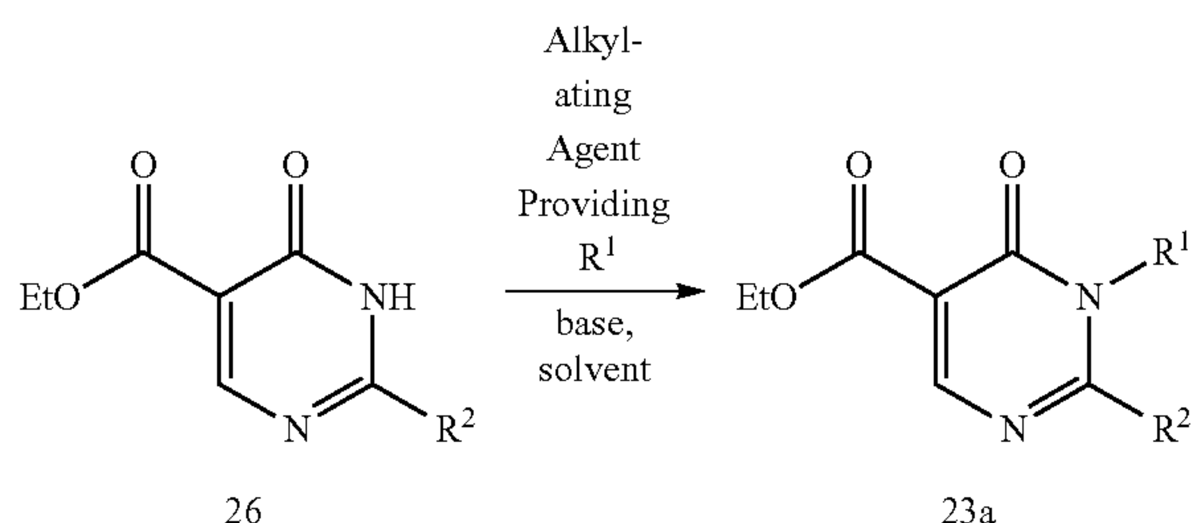
Scheme 14
