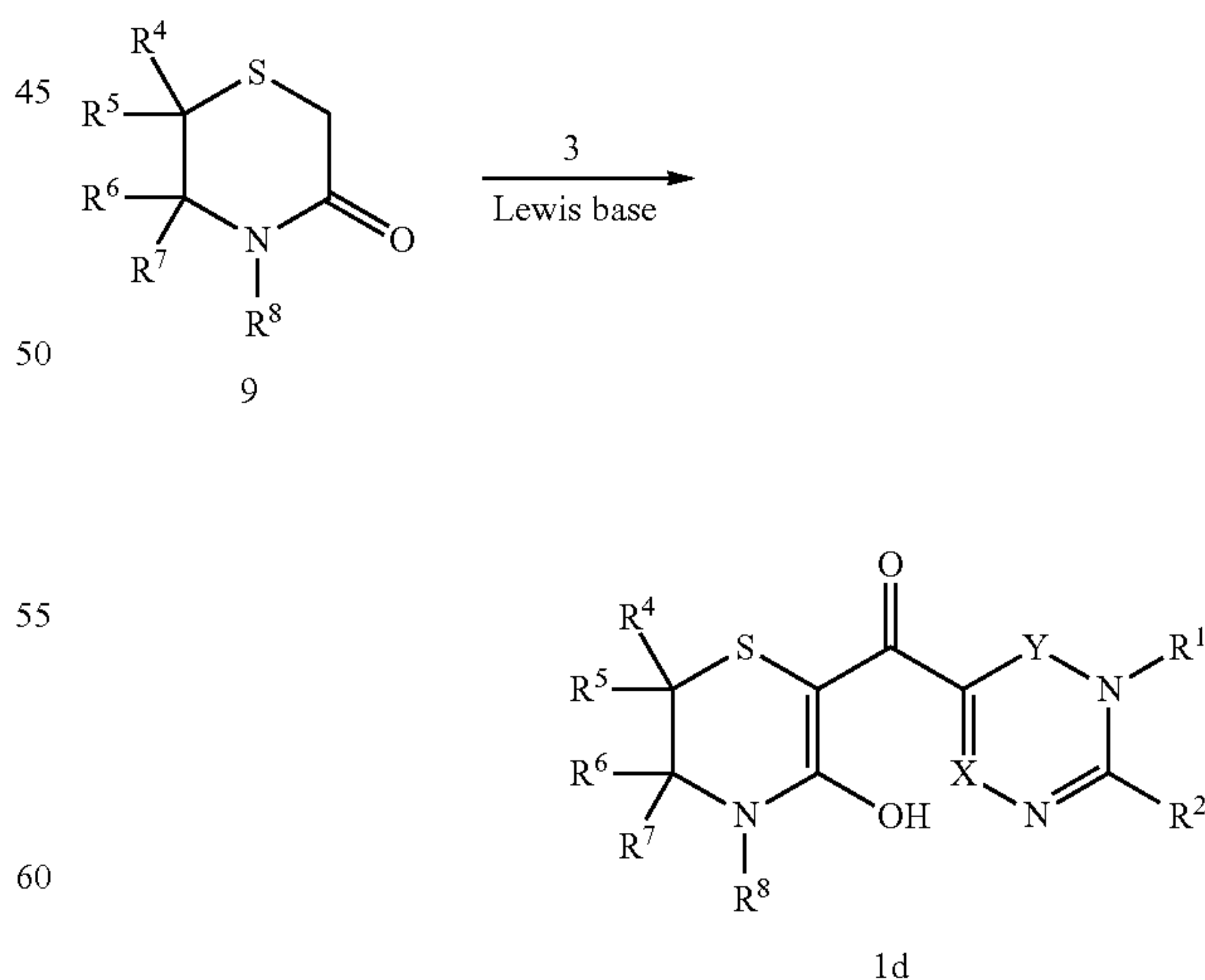
Scheme 6
