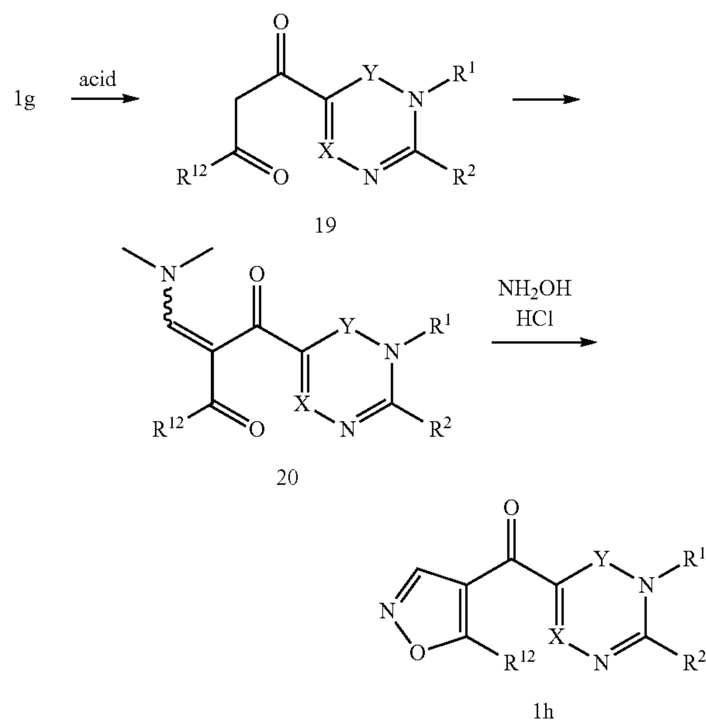
Scheme 10
