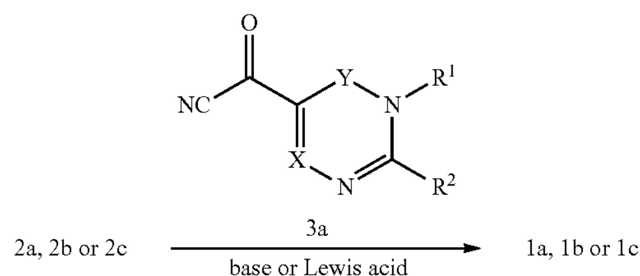
Scheme 2
