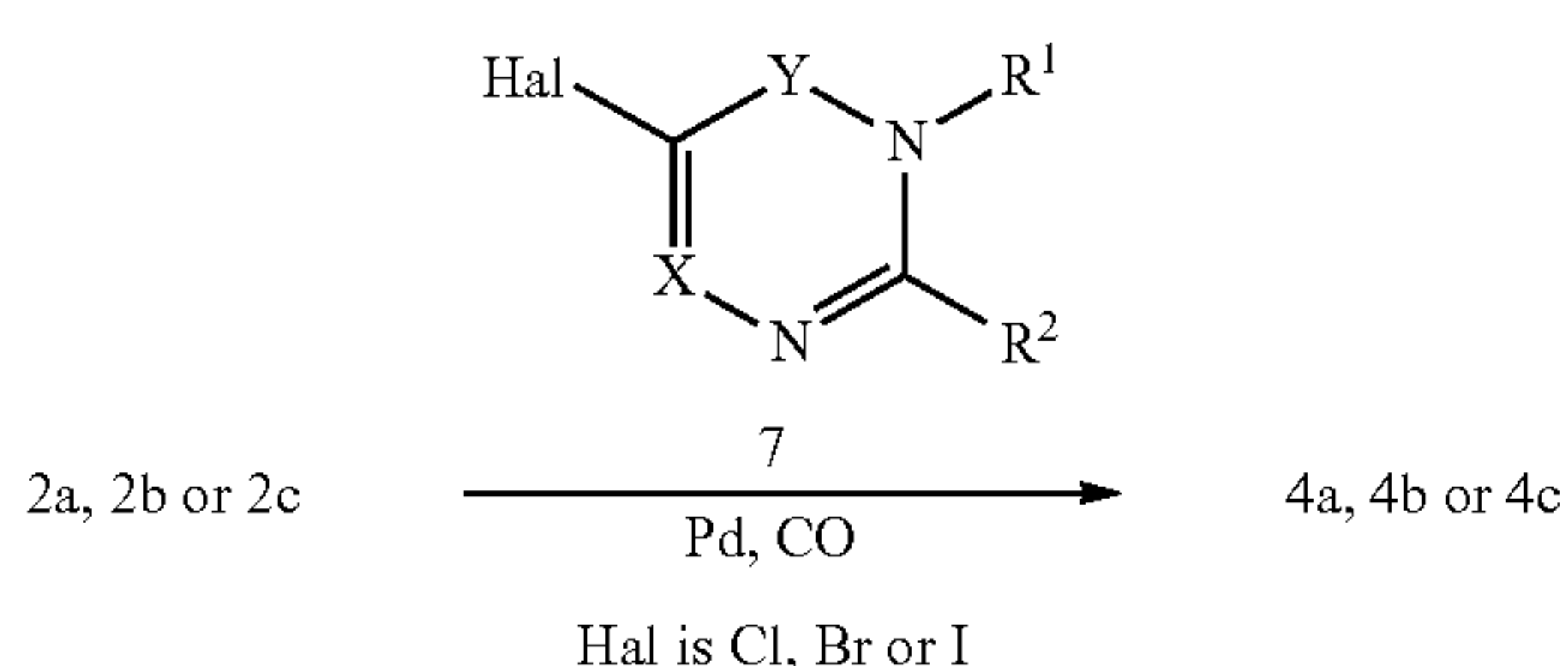
Scheme 4
