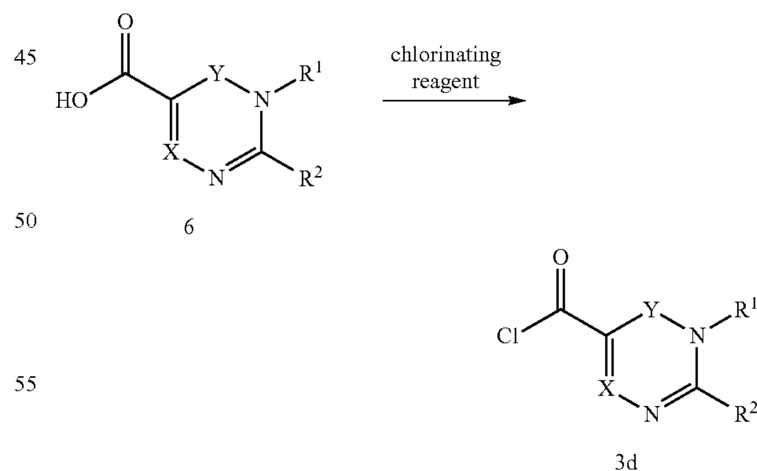
Scheme 12
