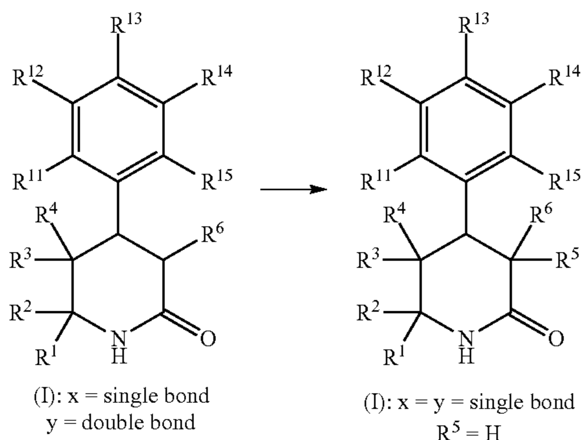
Scheme 11
