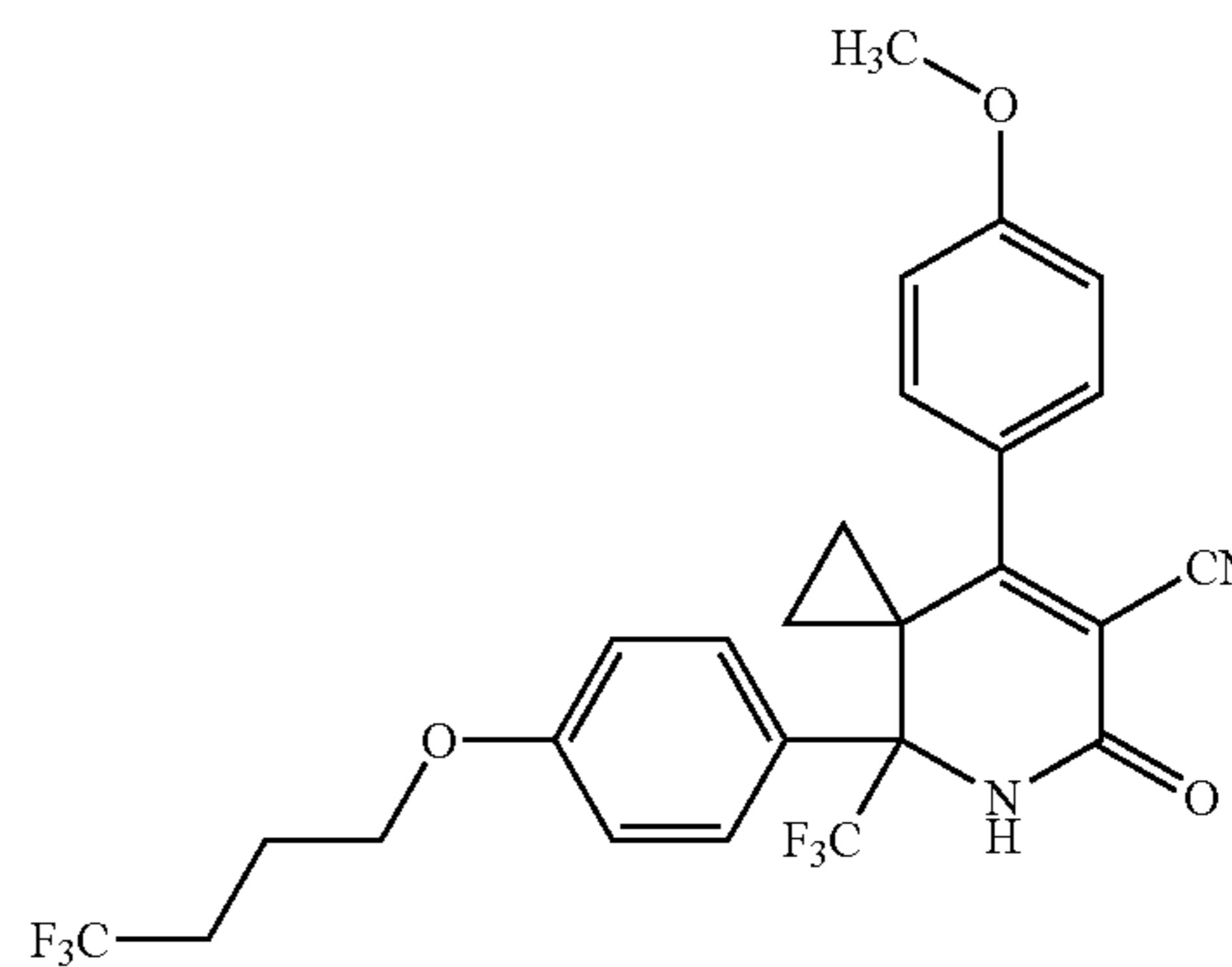
Intermediate 14A
