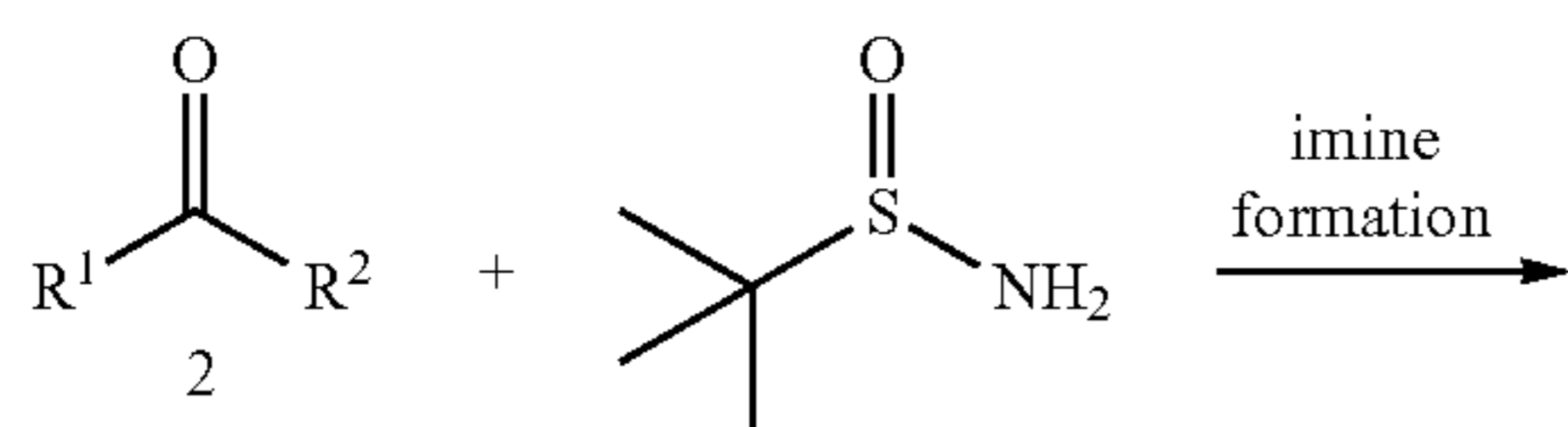
Scheme 12
