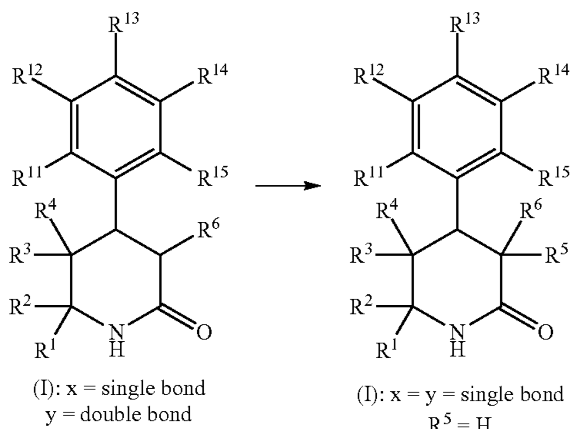
Scheme 11
