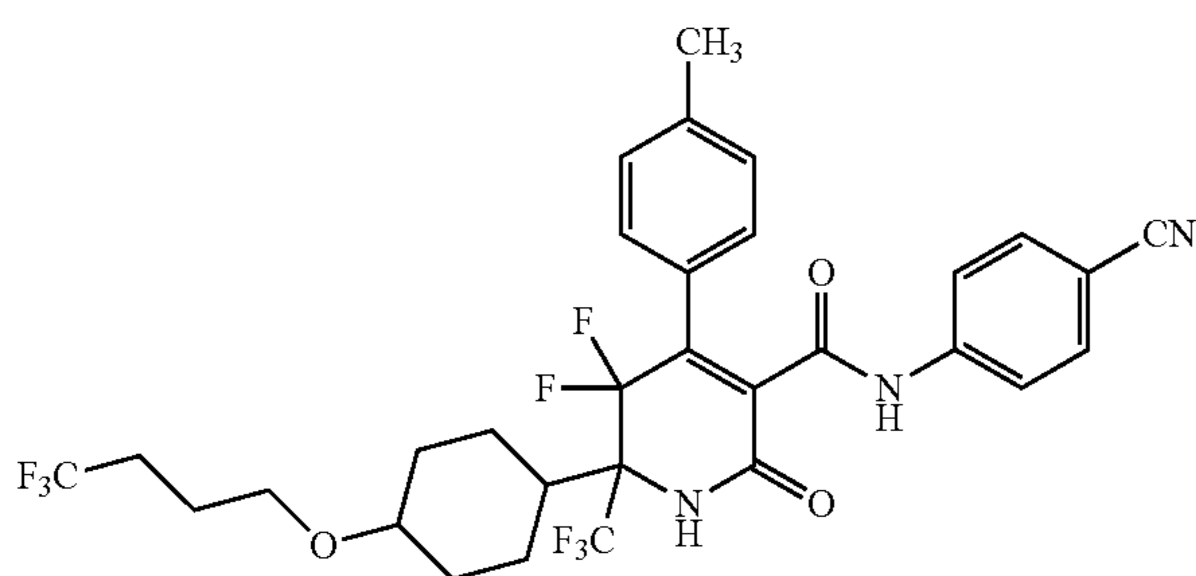
Intermediate 103A
