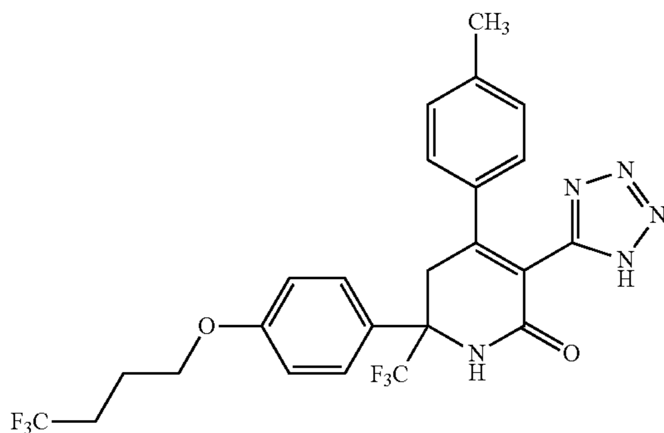
Intermediate 2A
