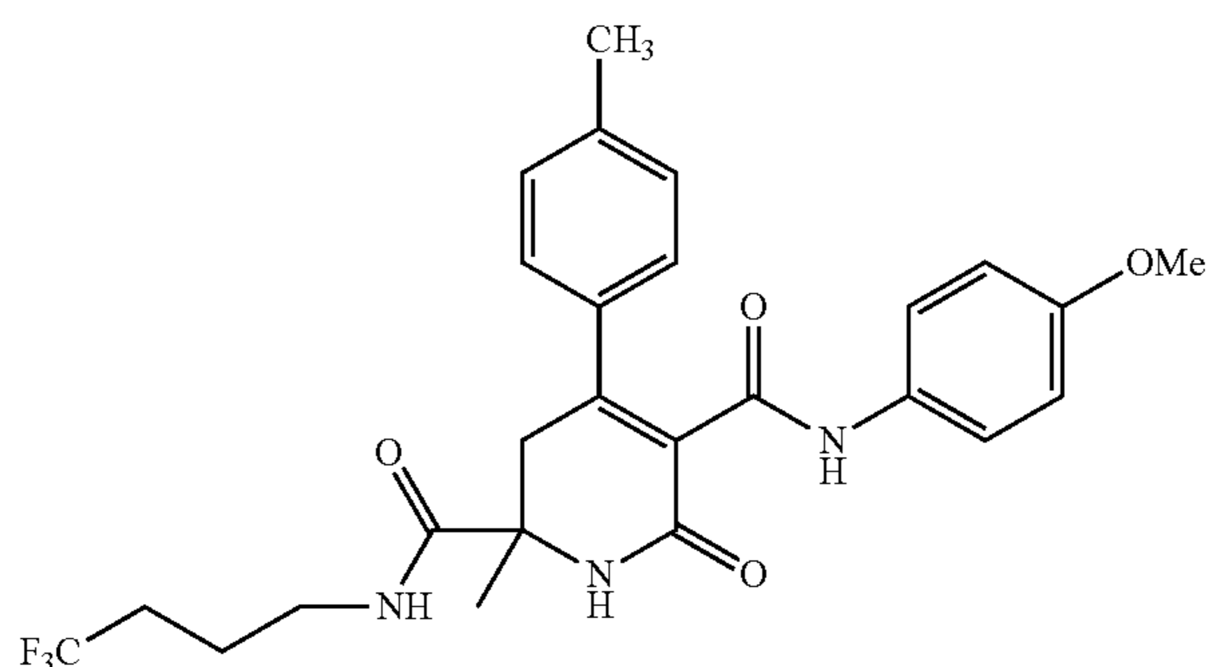
Intermediate 102A
