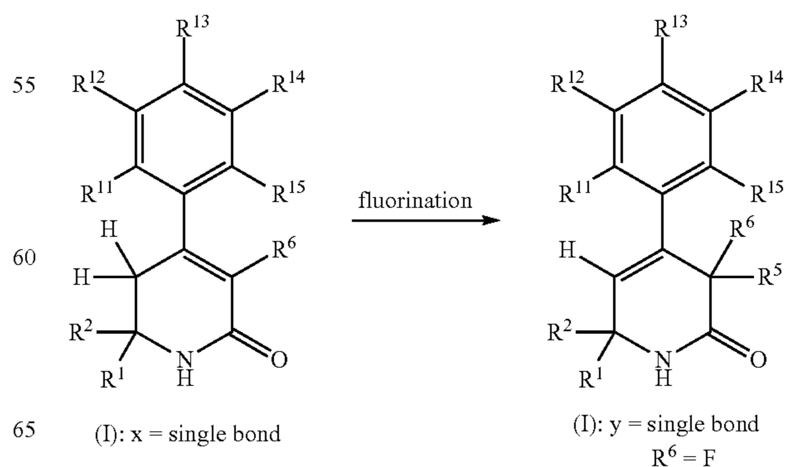
Scheme 10
