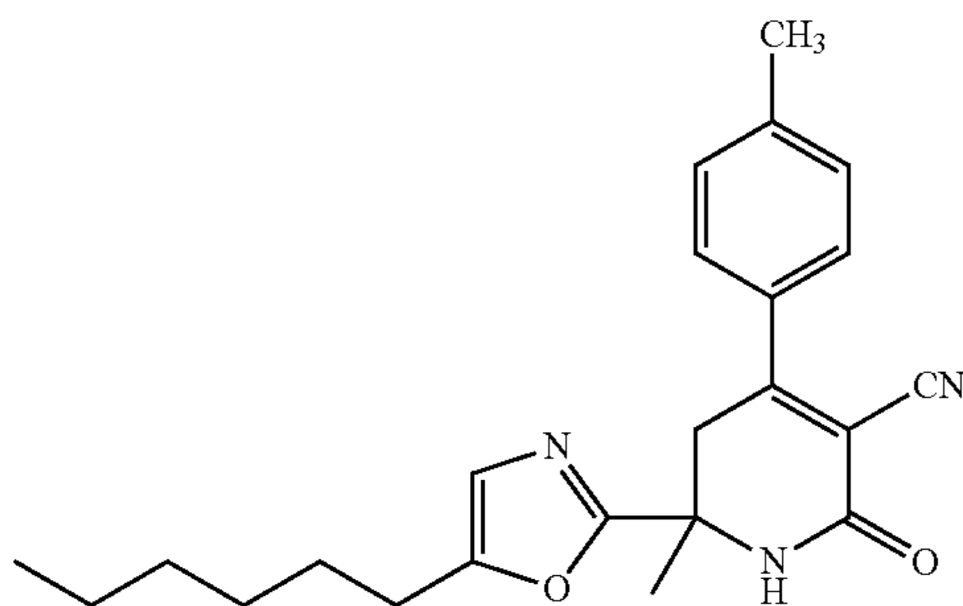
Intermediate 108A
