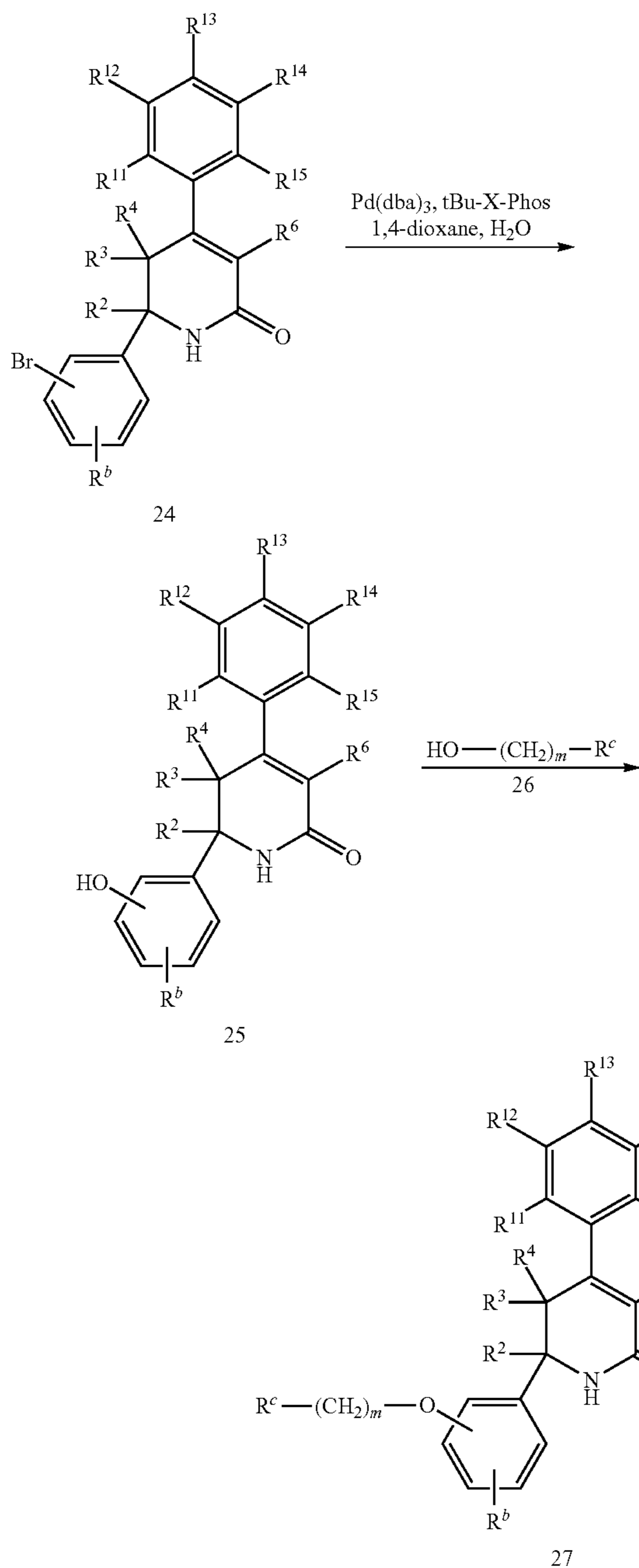
Scheme 7
