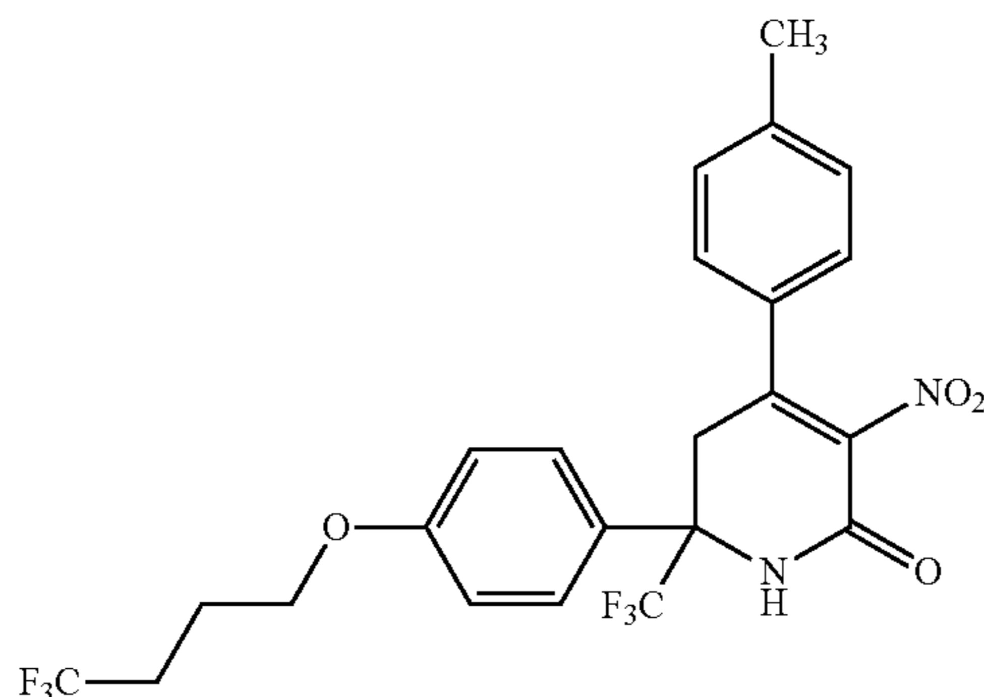
Intermediate 13A
