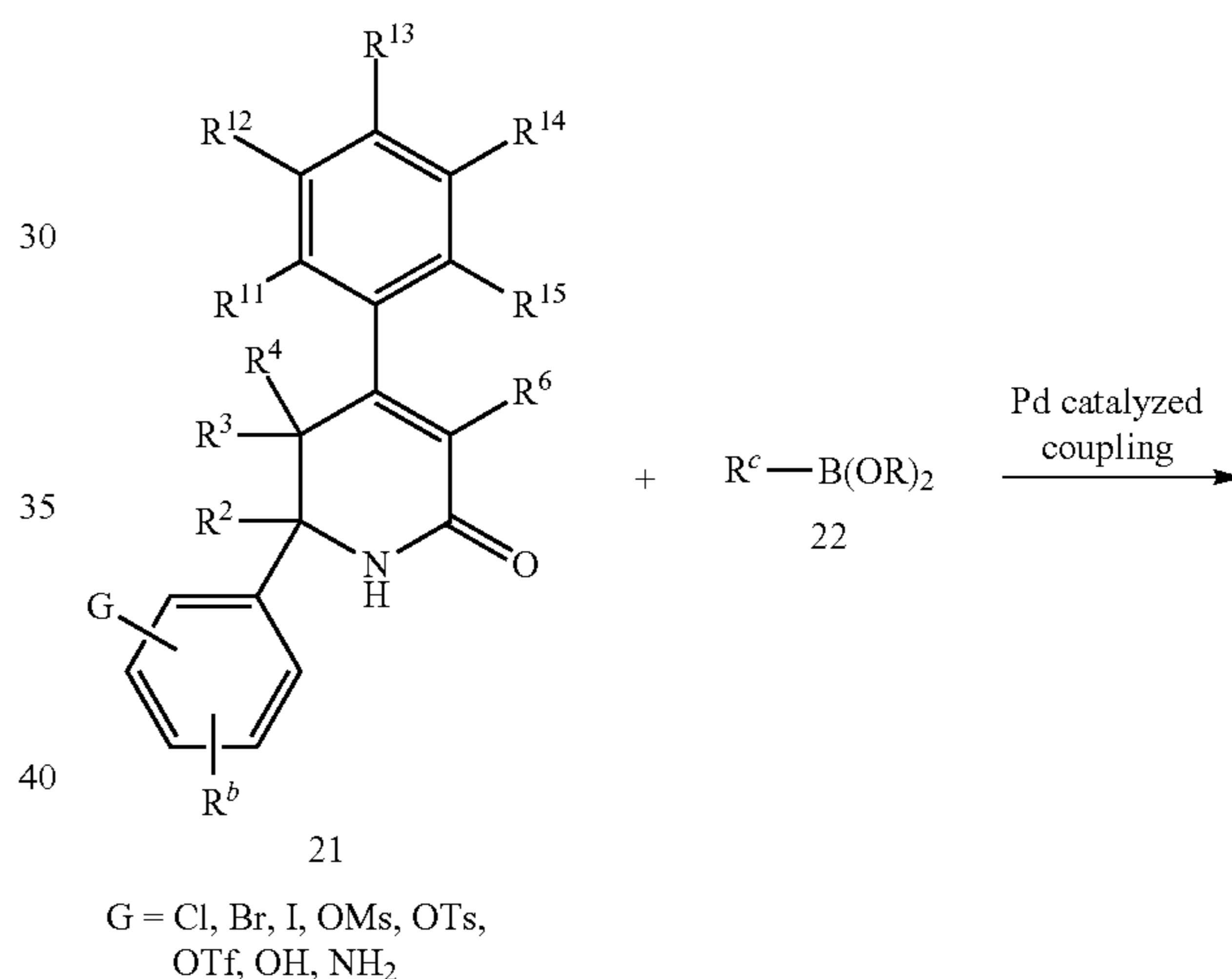
Scheme 6
