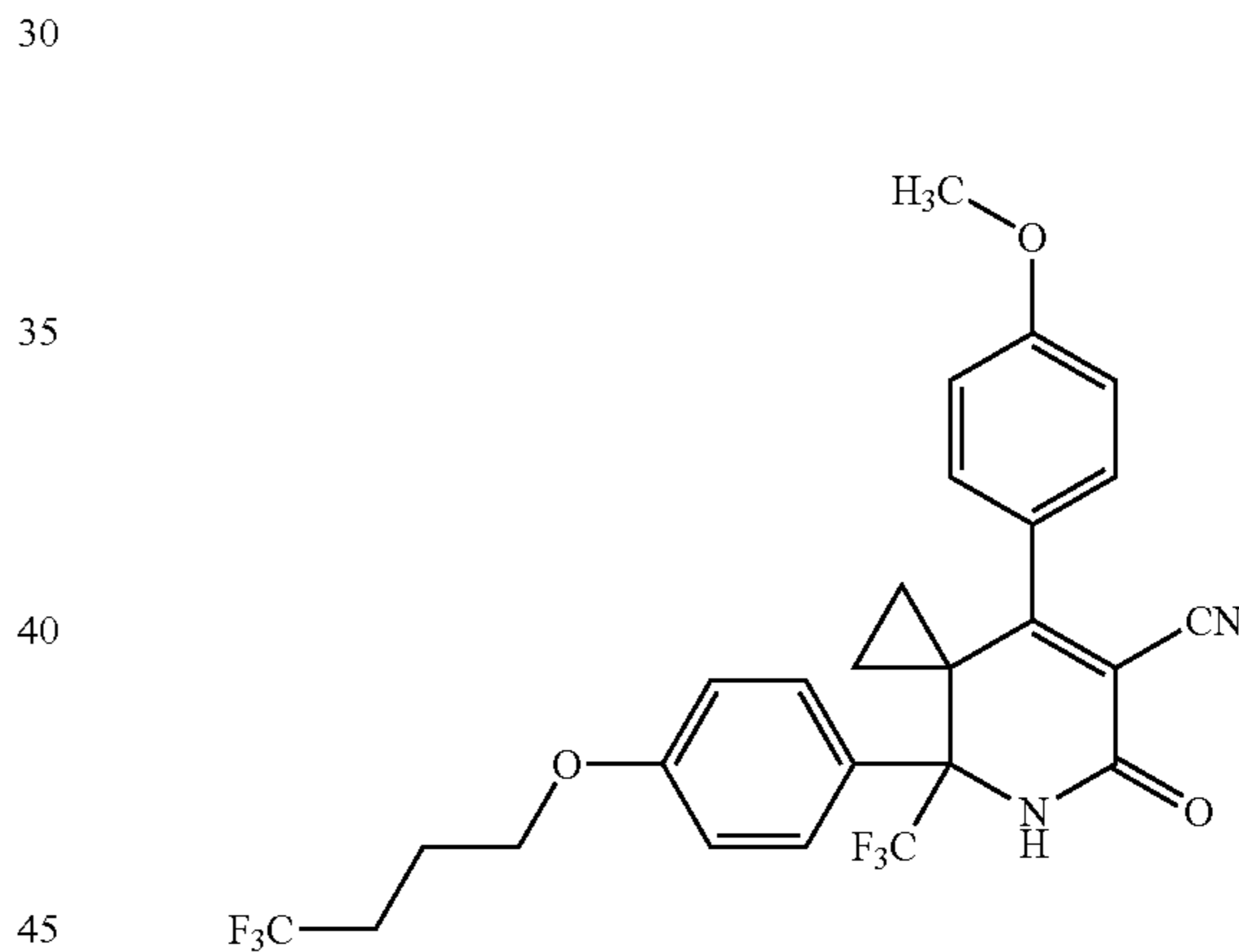
Intermediate 14A
