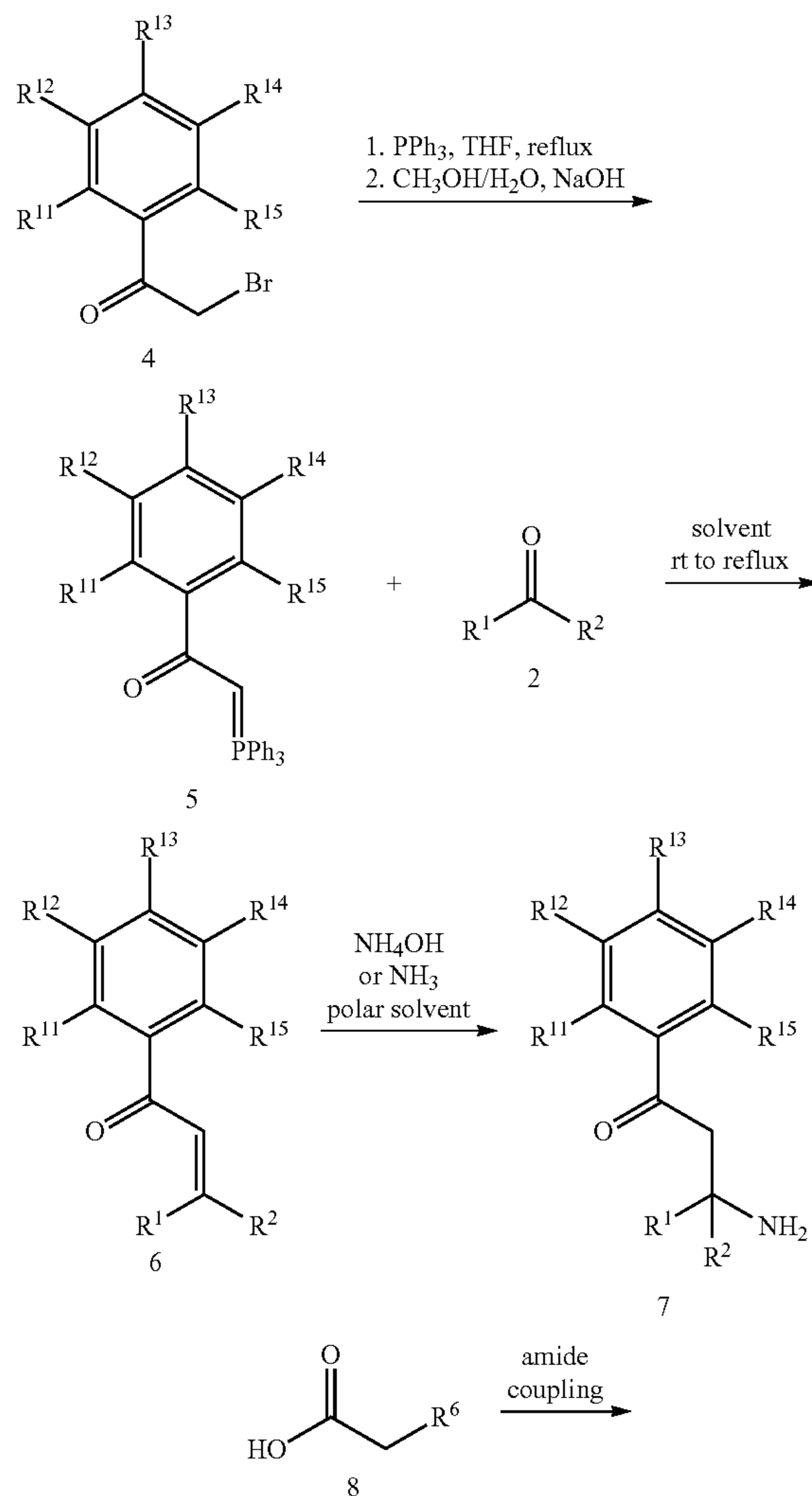
Scheme 2
