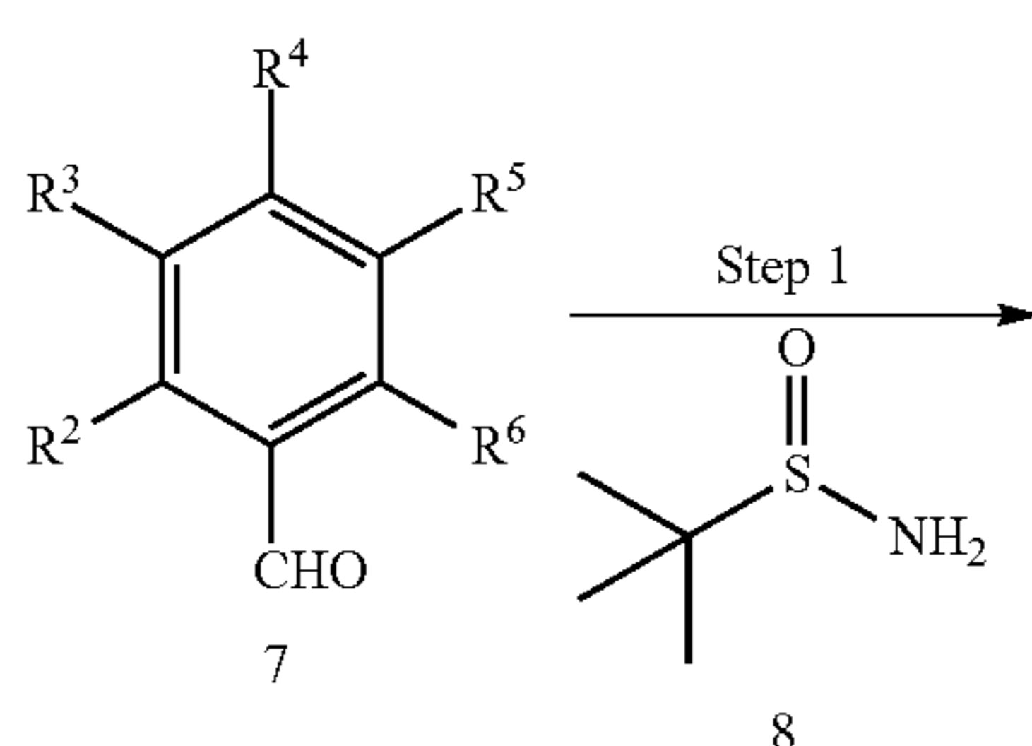
SCHEME 2
