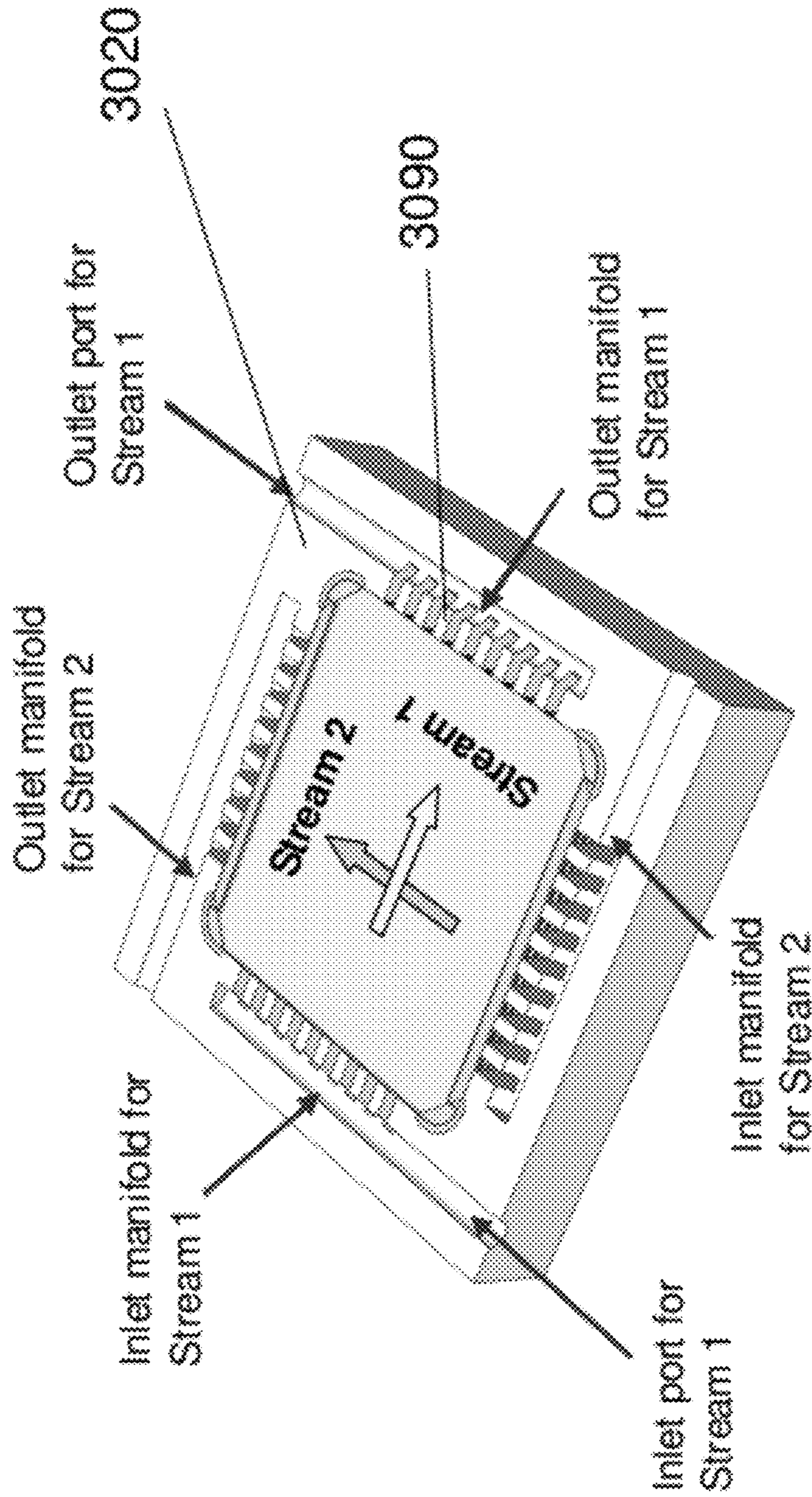
Section view
