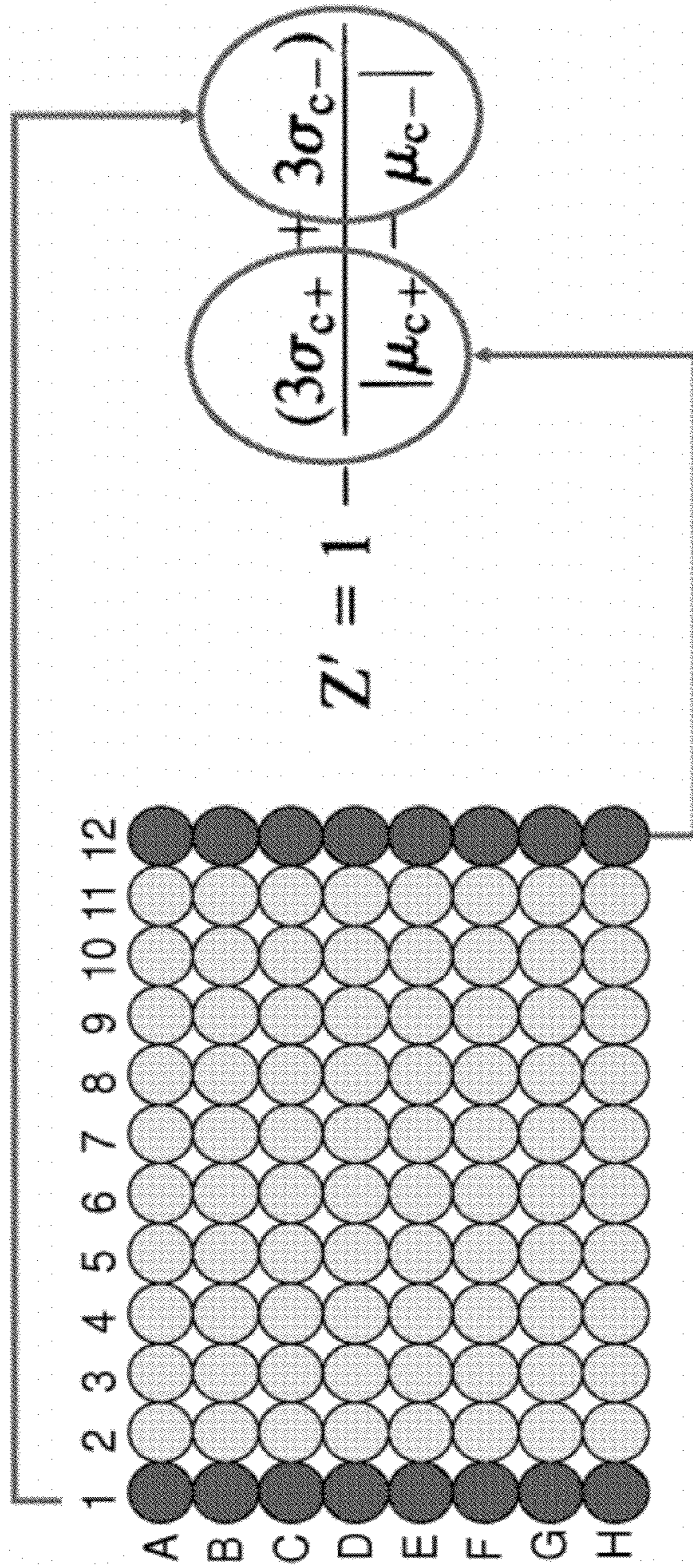
FIG. 2 Experimental design Assay Quality: Z-Score
