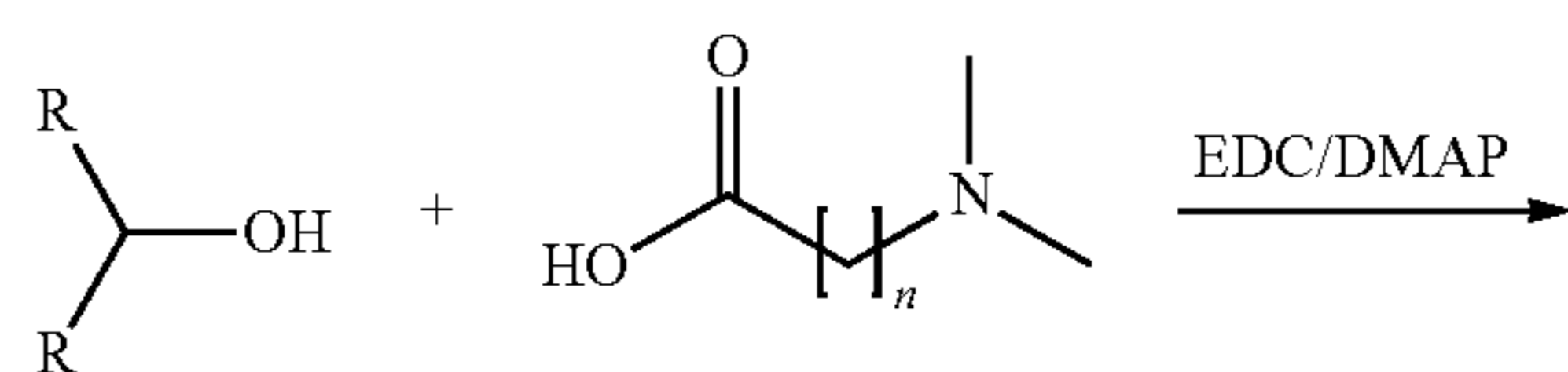
Scheme 1: M series (esters) synthesis
