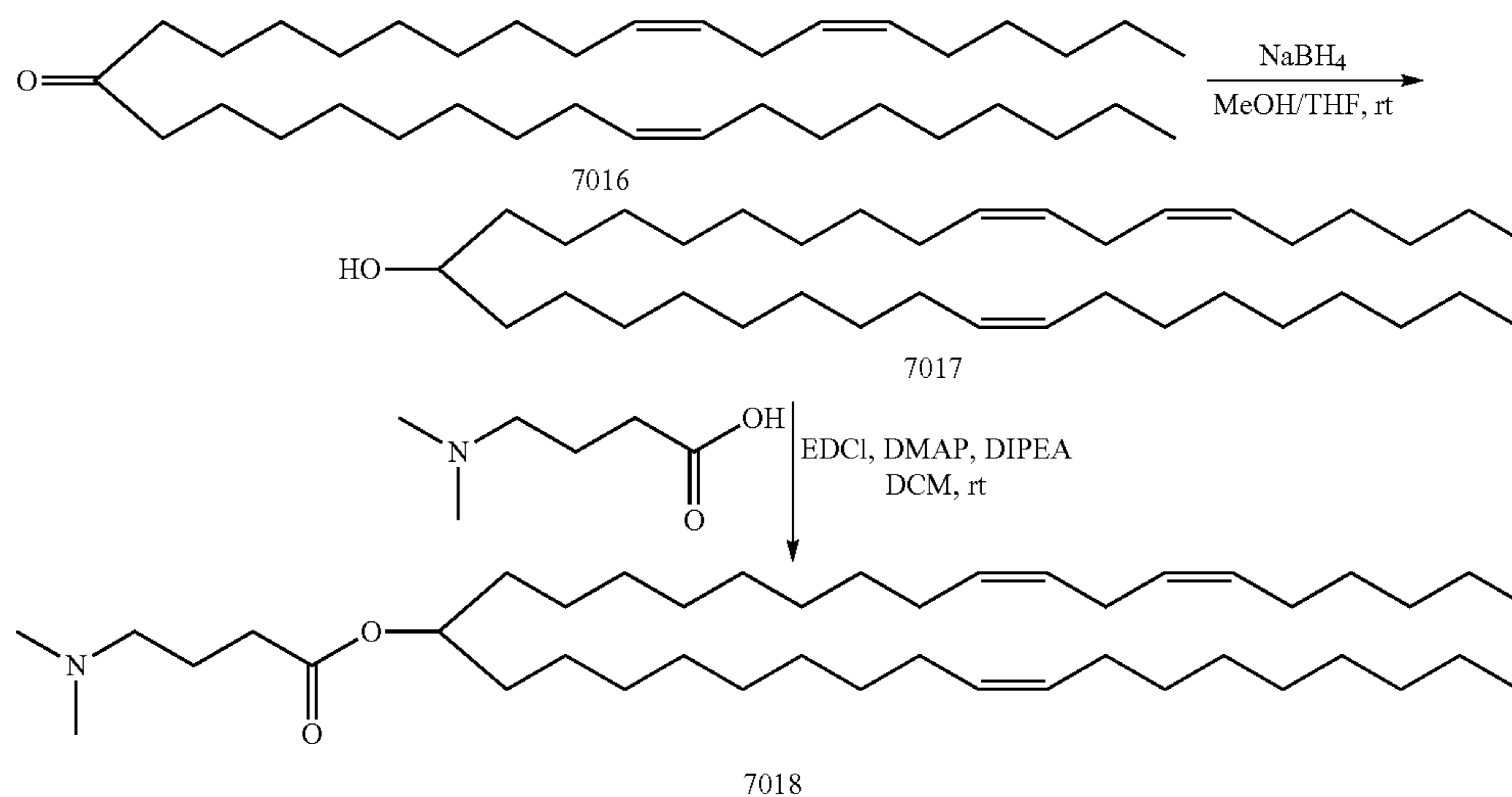
Scheme 4
