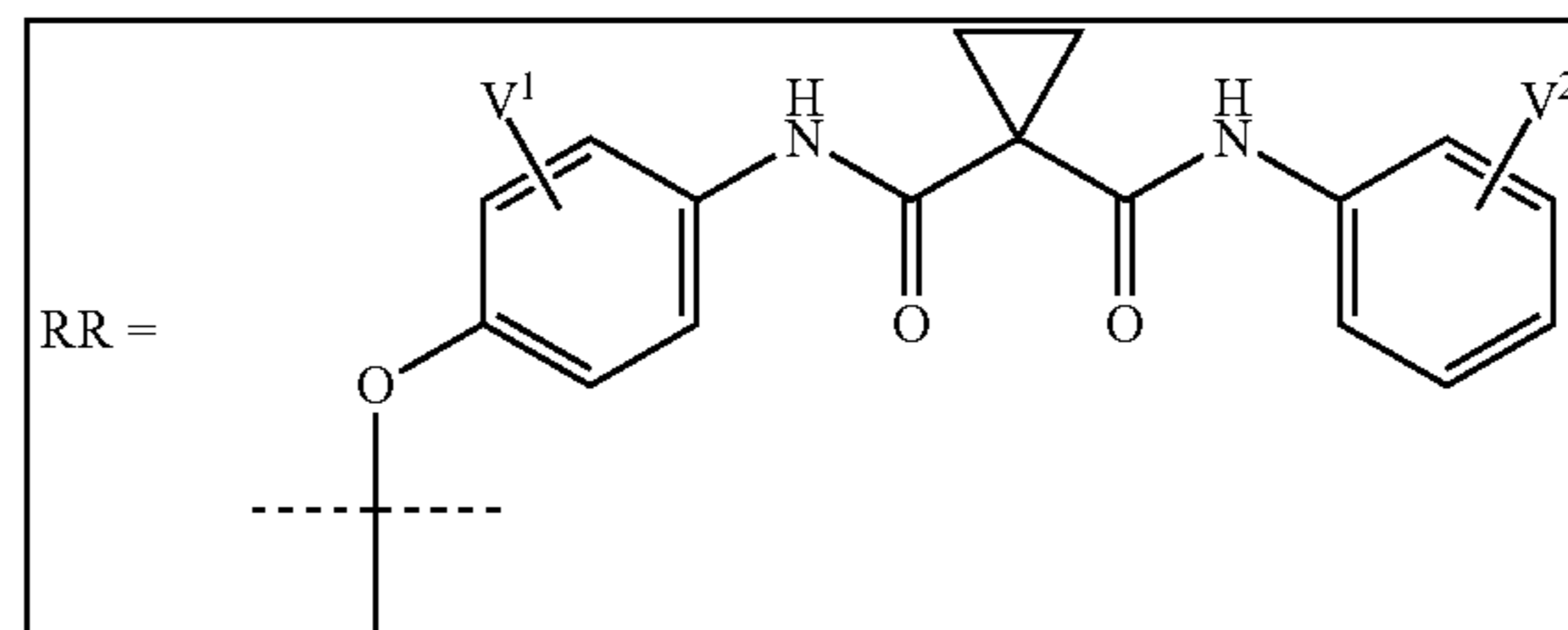
Scheme 1
