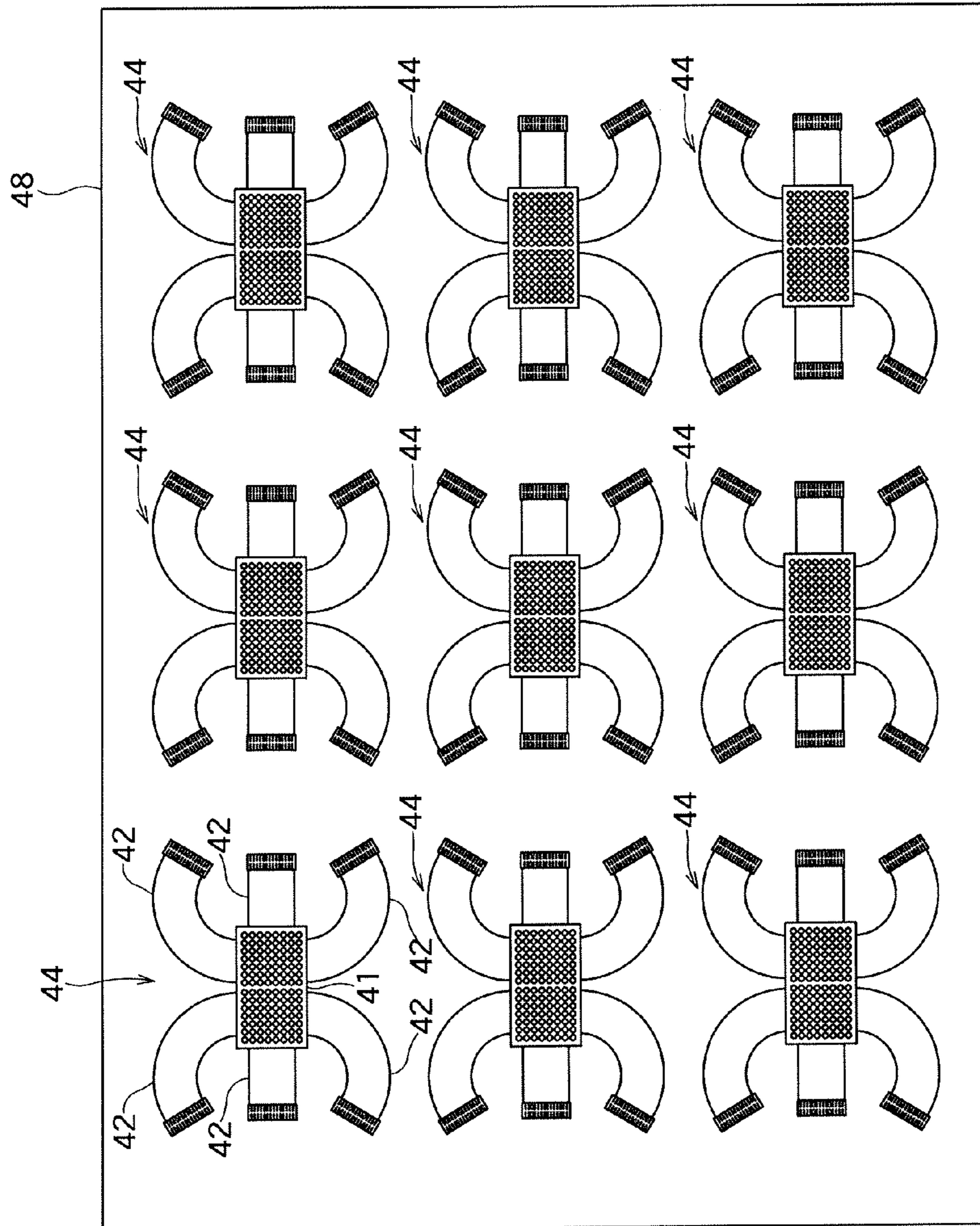
FIG. 9 PRIOR ART
