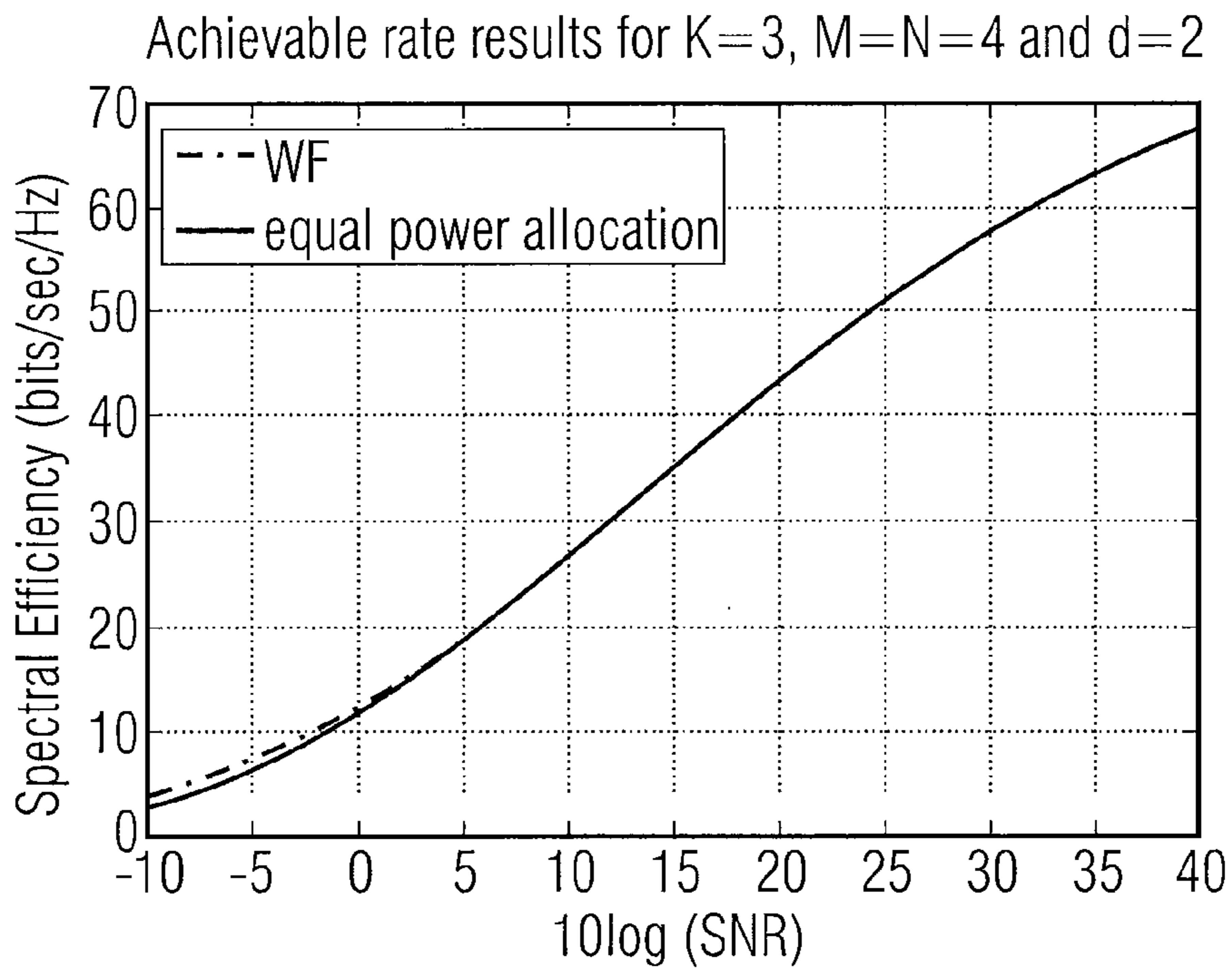
Effect of WF on performance
