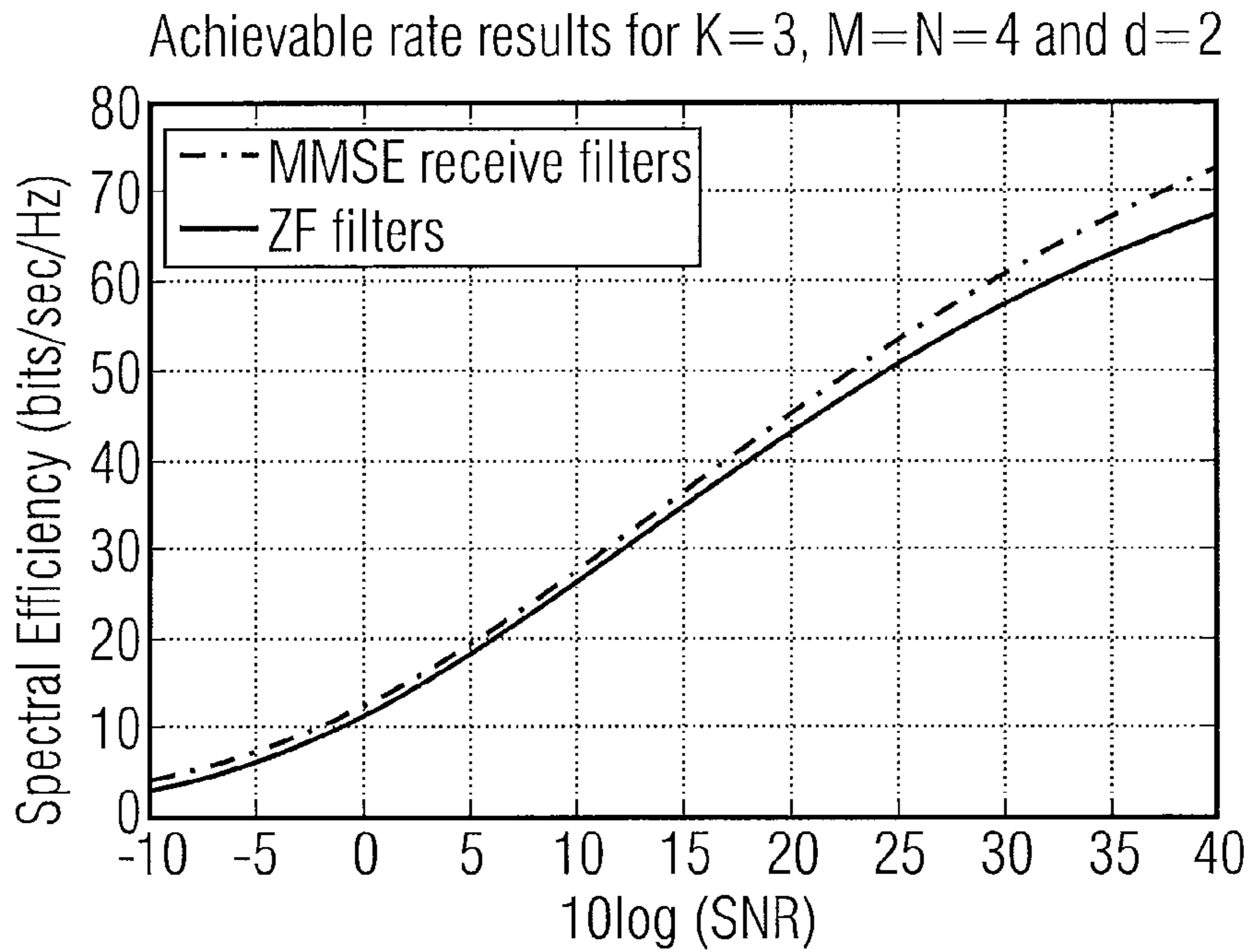
Effect of using ZF vs. MMSE filters on performance
