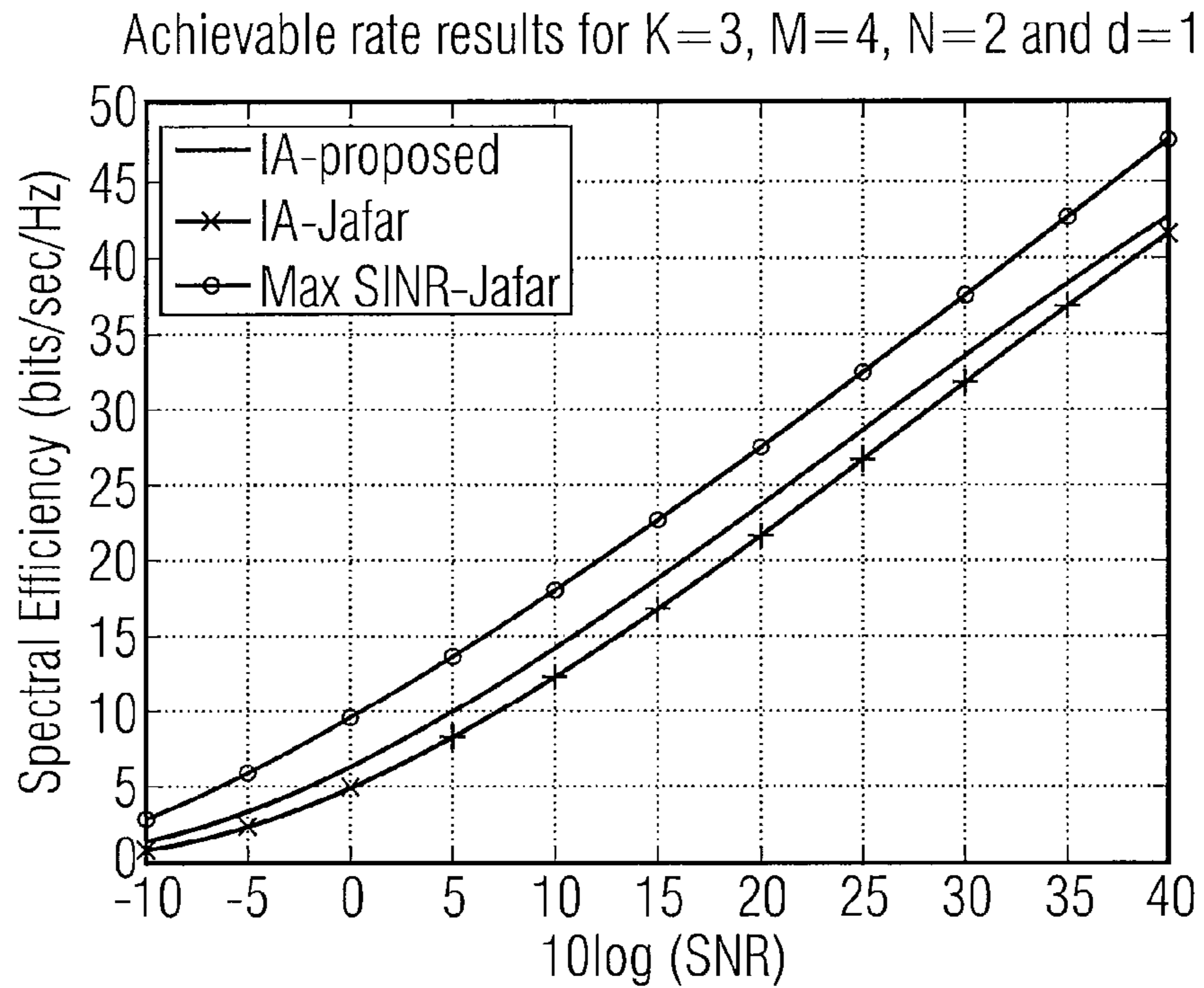
Spectral efficiency results for scenario 1
