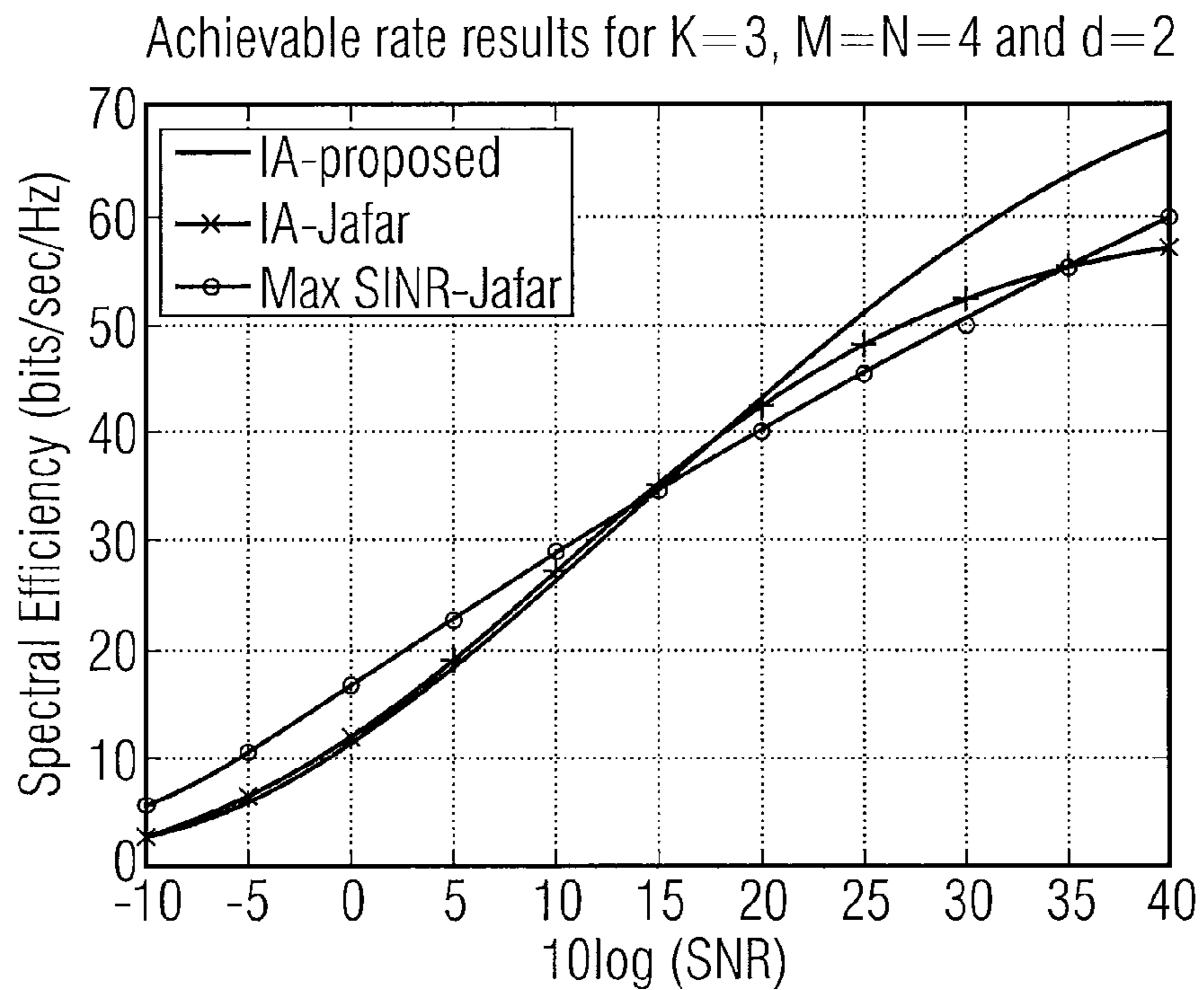
Spectral efficiency results for scenario 2
