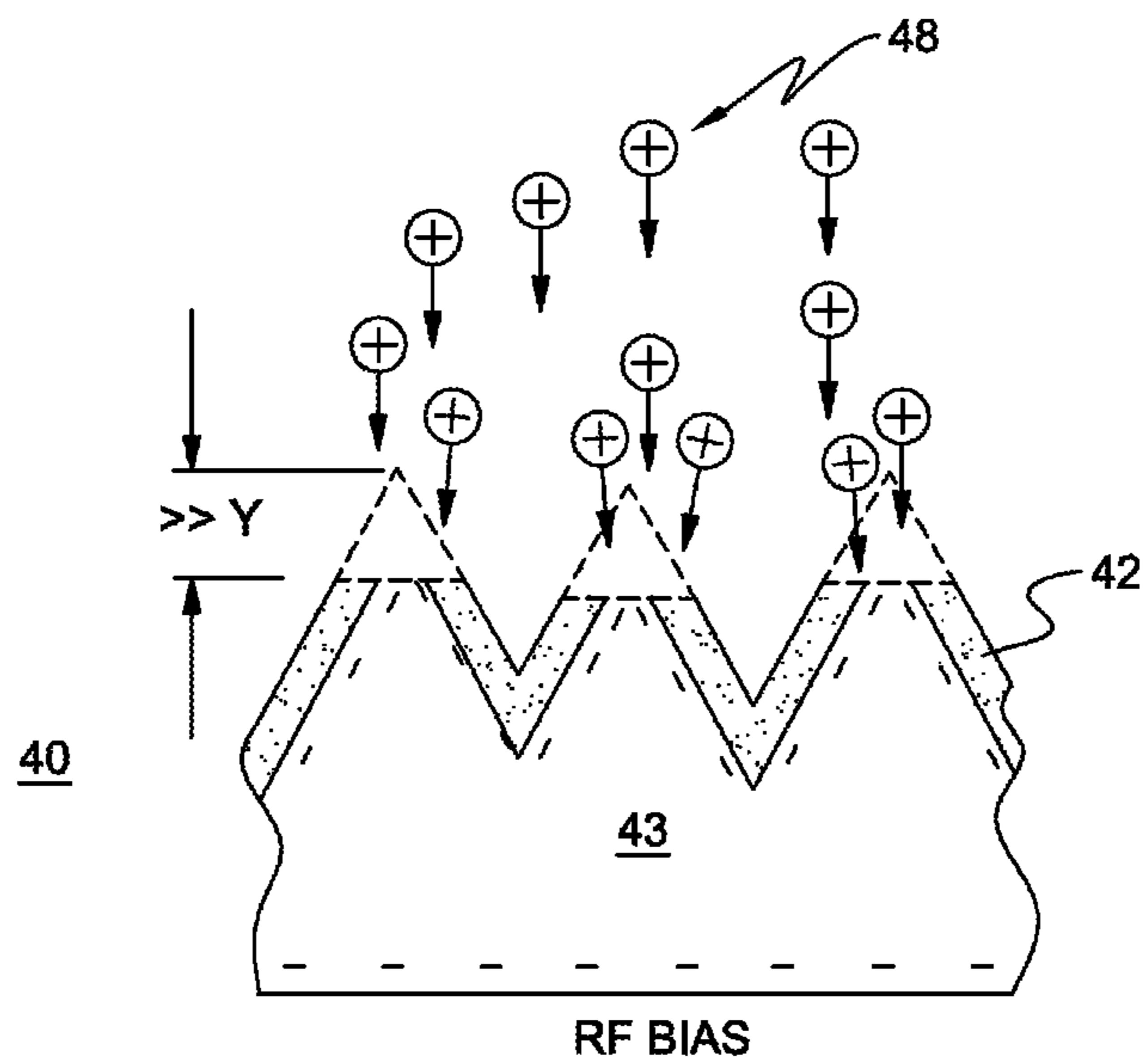
RF BIAS FIG. 4b
