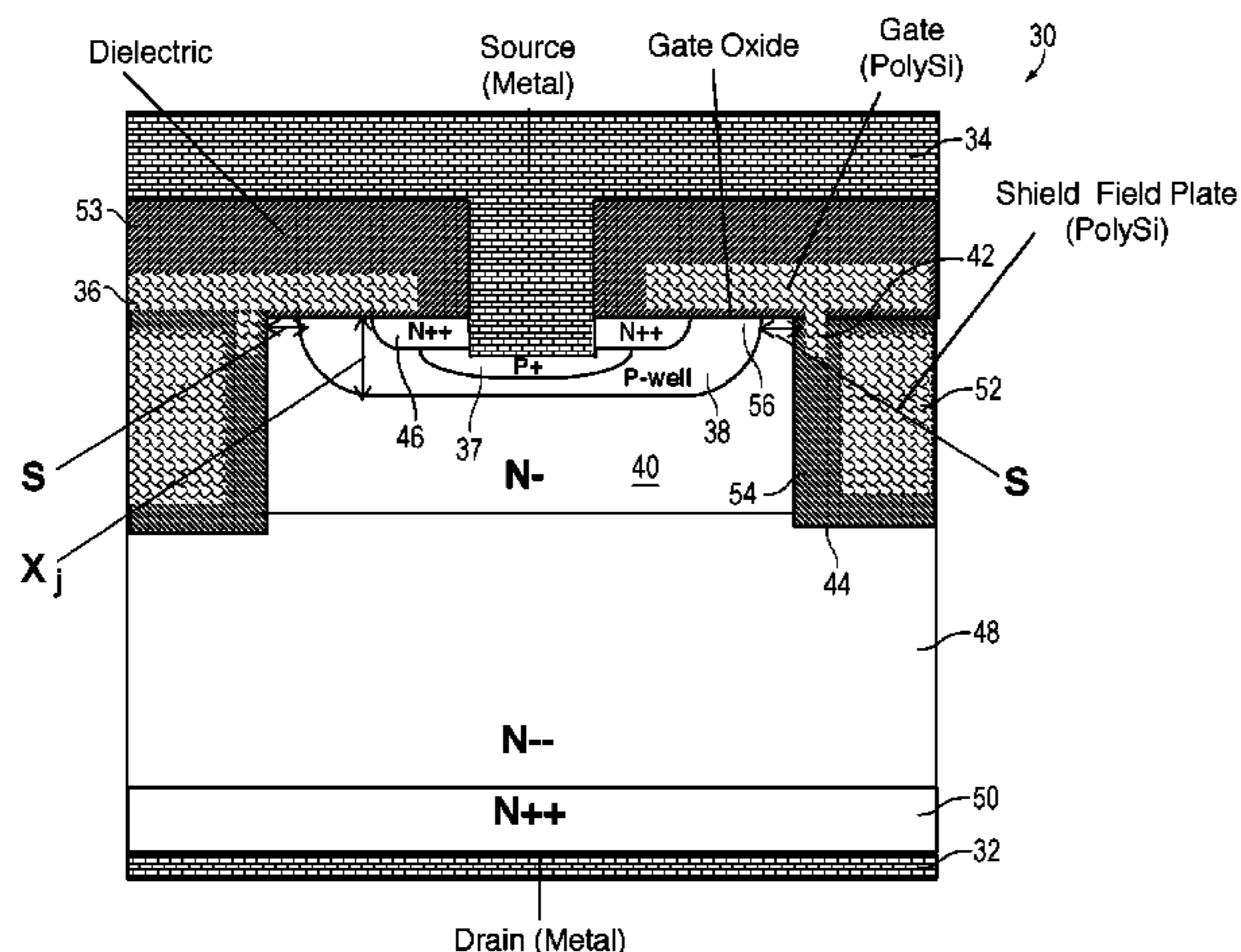
DMOS Transistor with Wrapped Around Gate Structure
