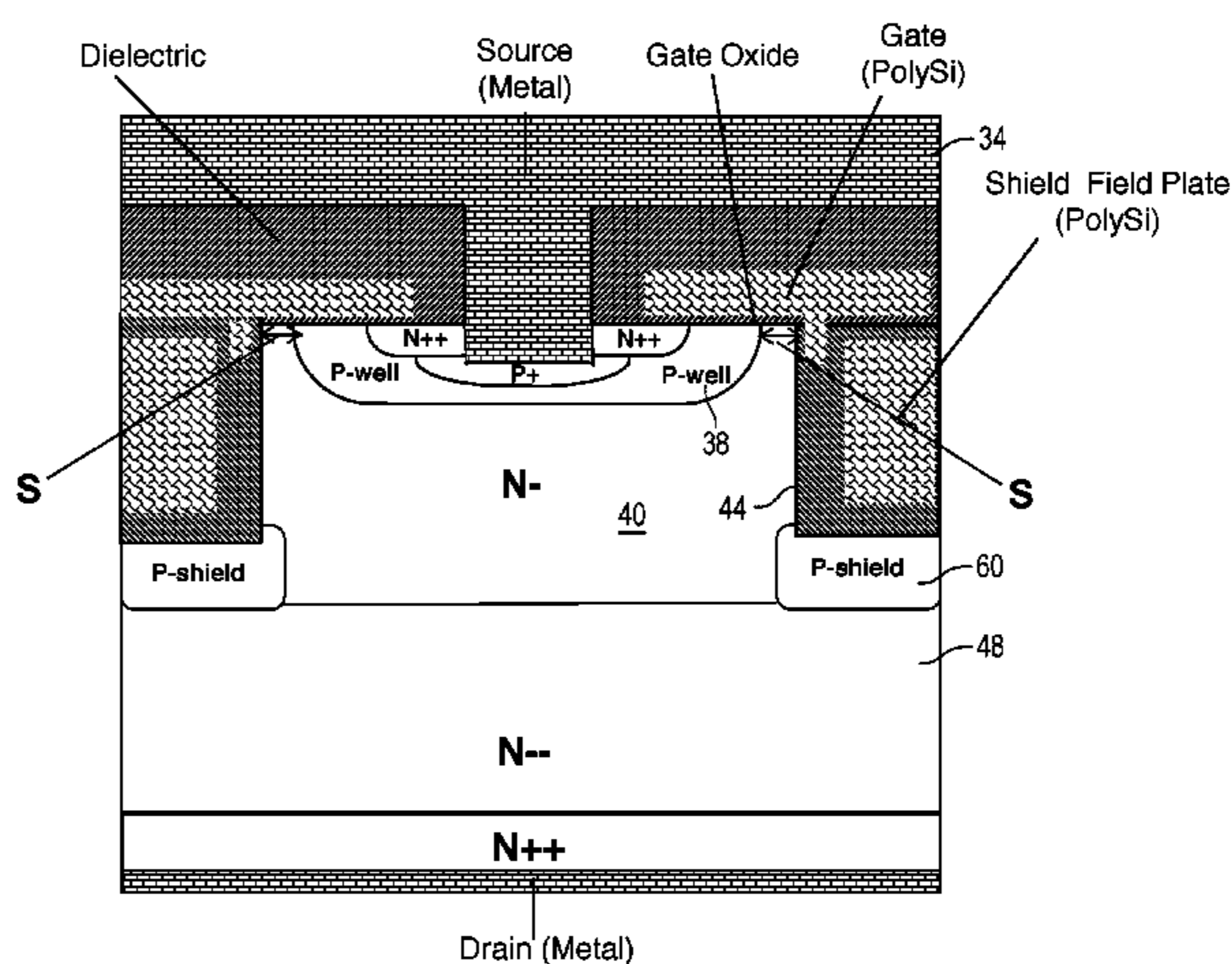
Device Structure with P-Shield Region
