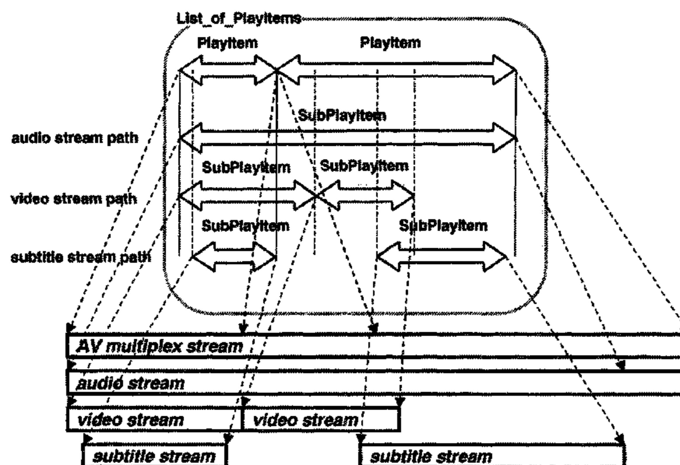
List_of_PlayItems Example
