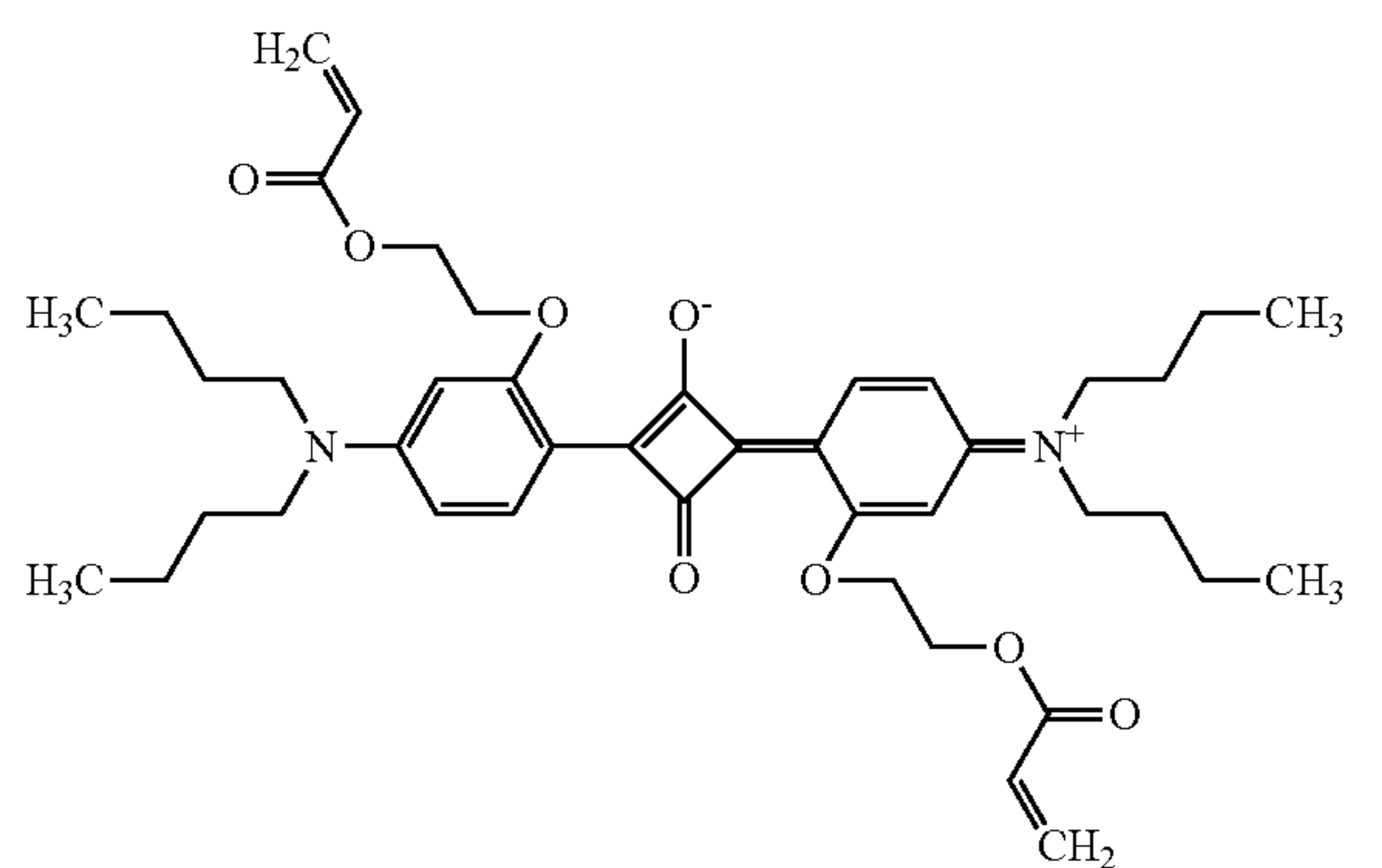
[Chemical Formula 3]
