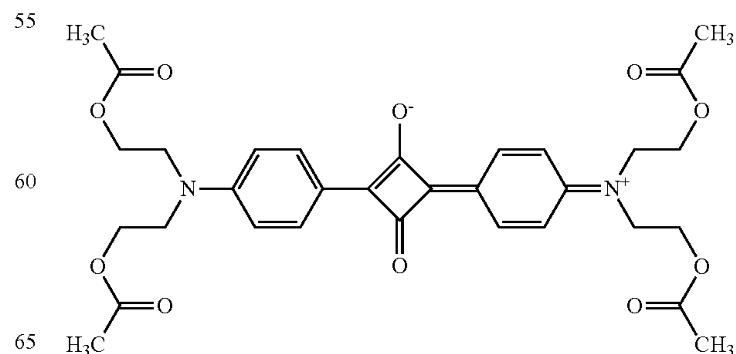
[Chemical Formula 6]
