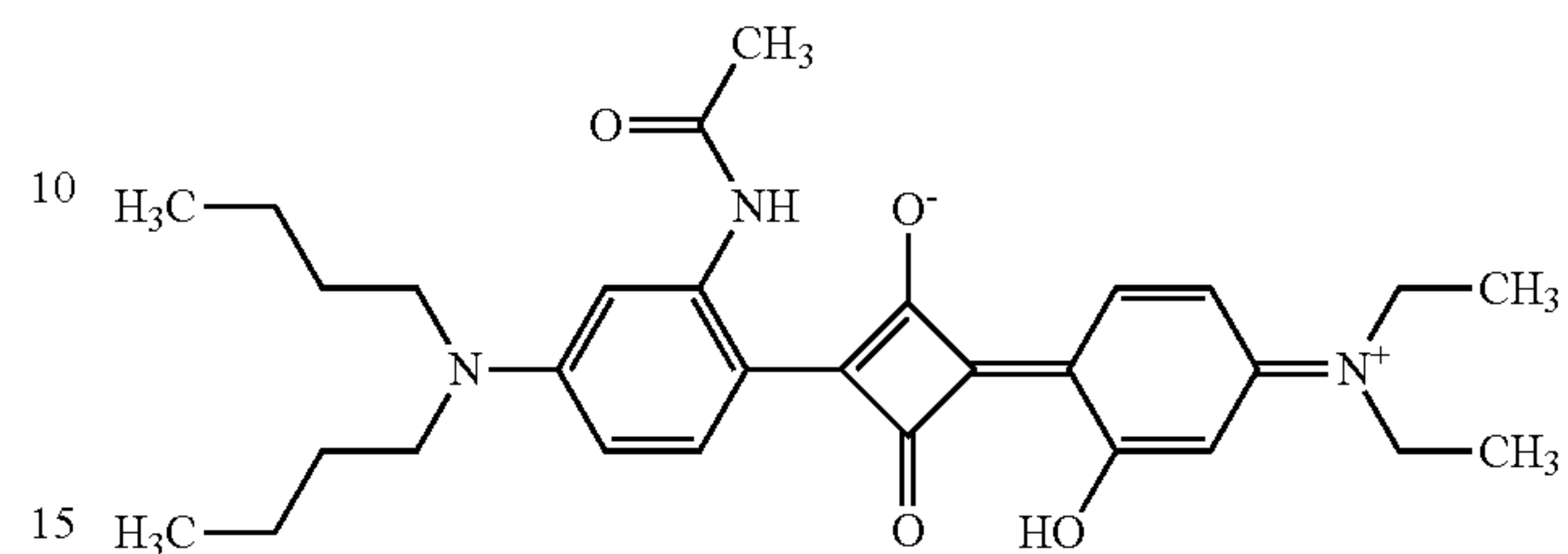
[Chemical Formula 4]
