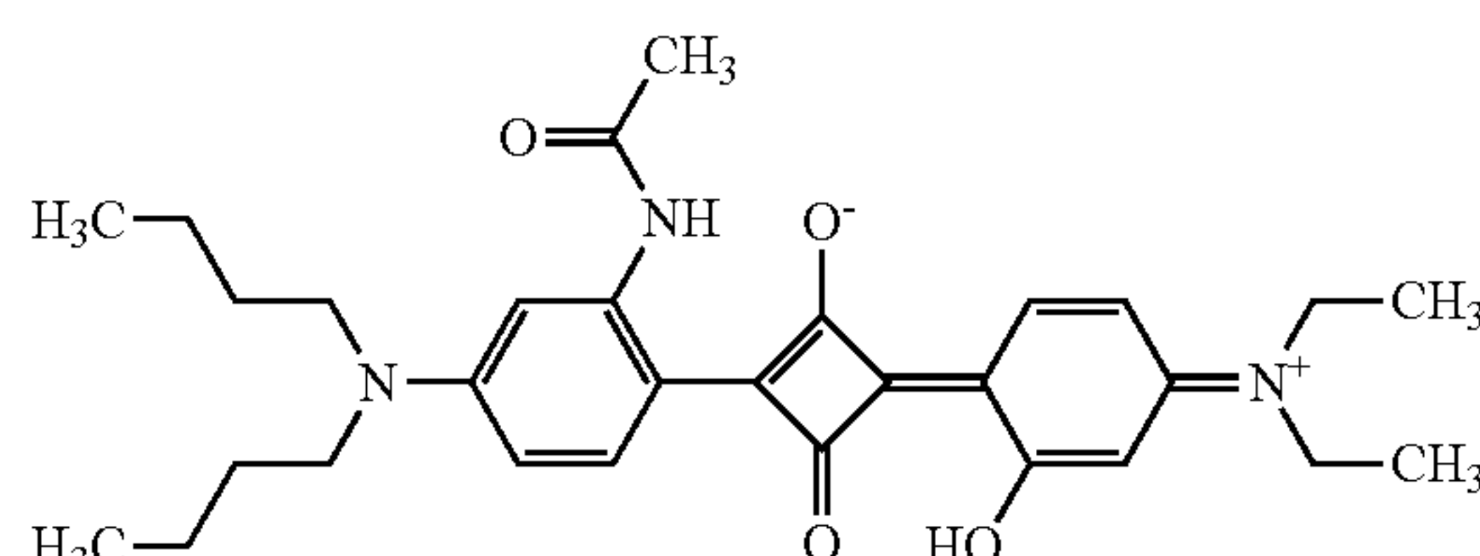
[Chemical Formula 4]
