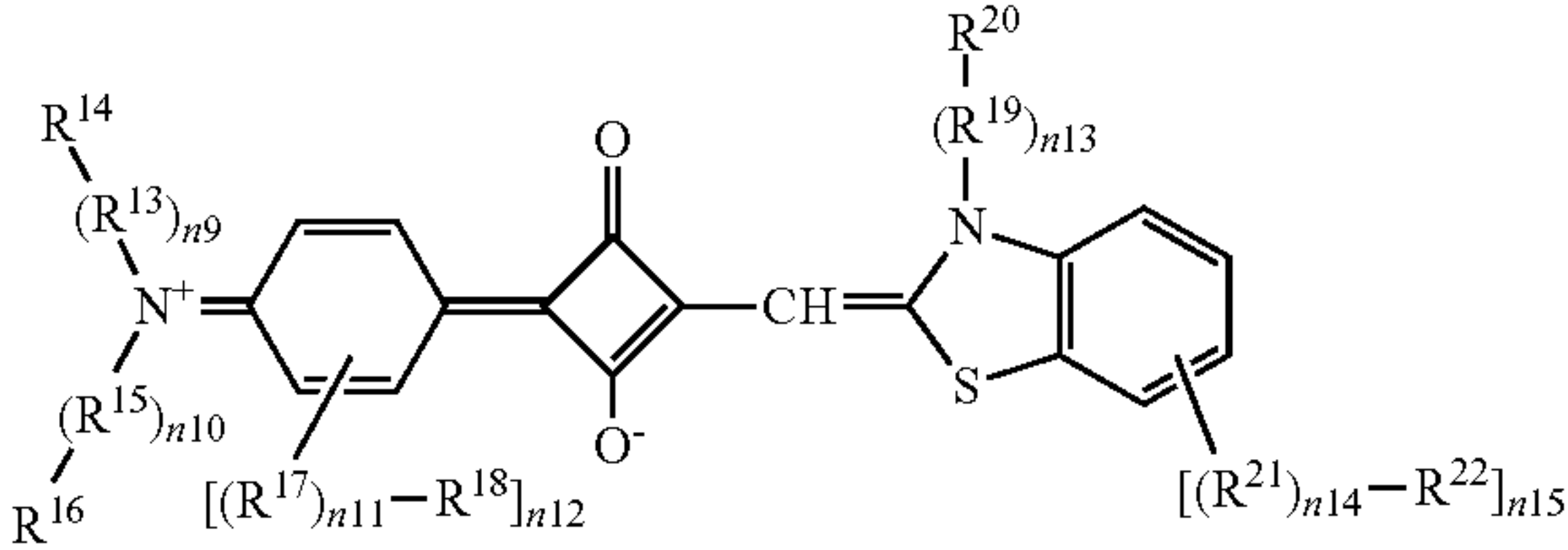
[Chemical Formula 2]
