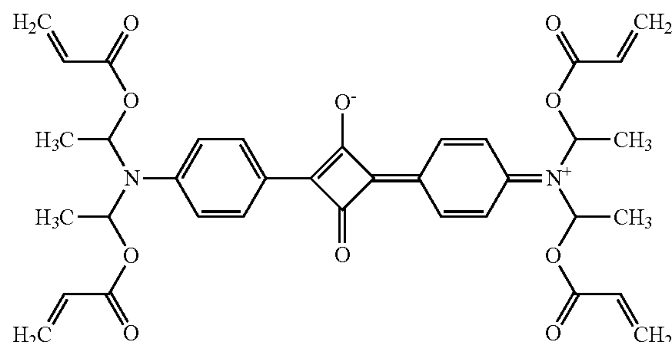
[Chemical Formula 7]
