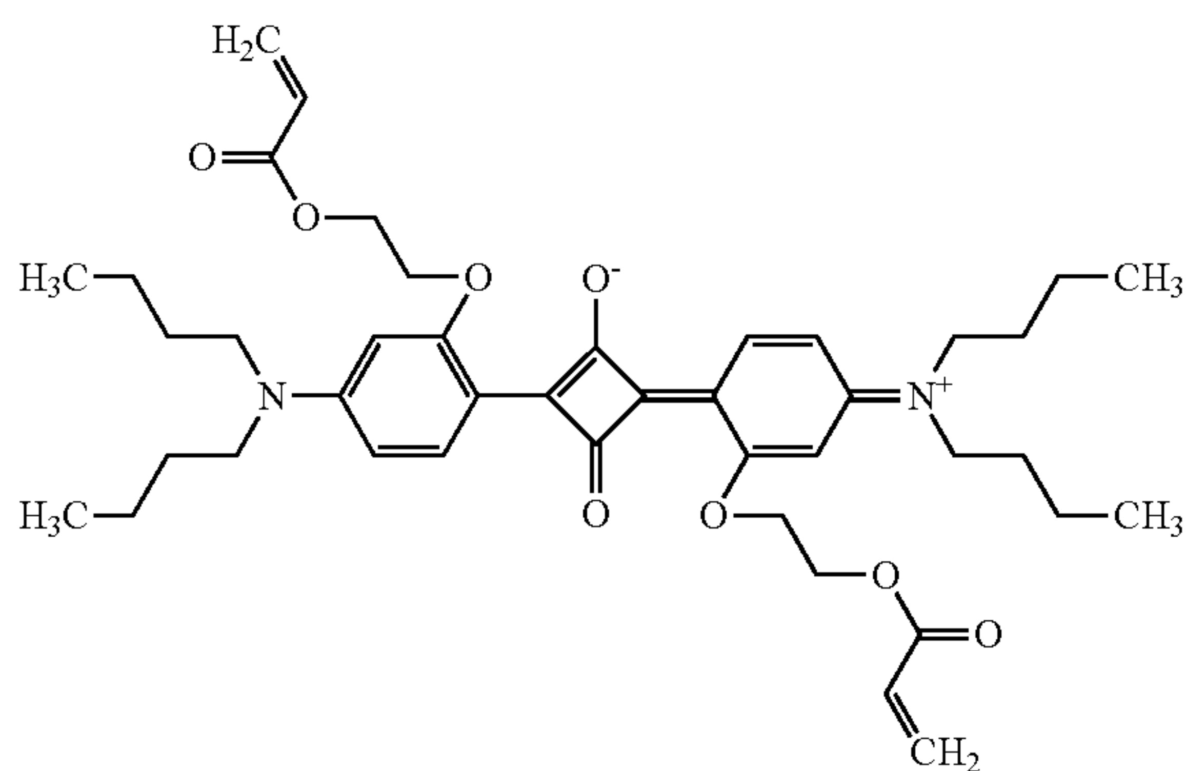
[Chemical Formula 3]
