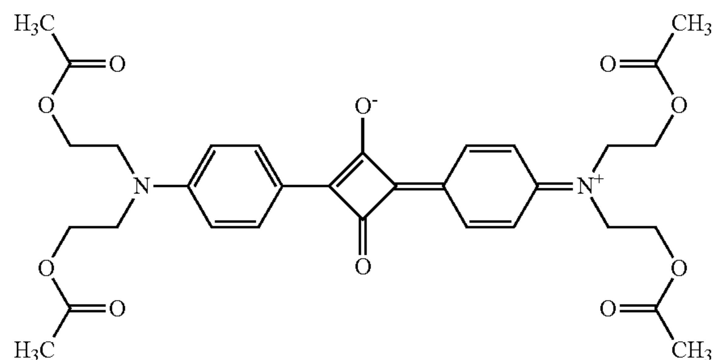
[Chemical Formula 6]
