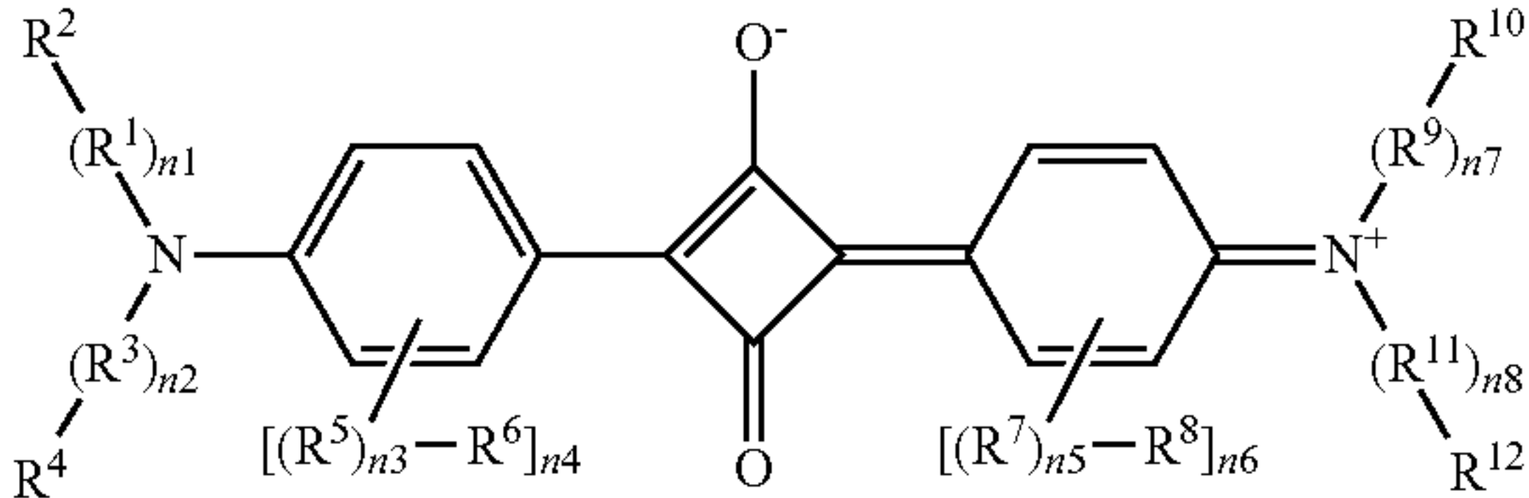
[Chemical Formula 2]
