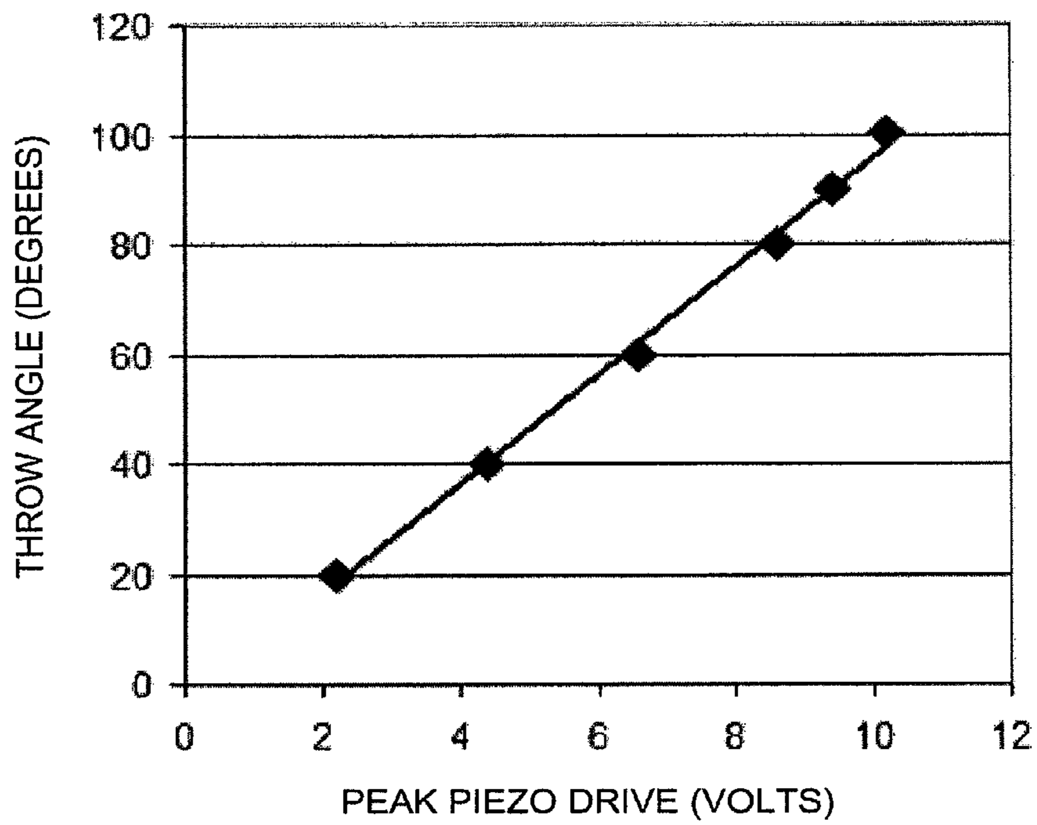
PROJECTOR THROW ANGLE AS FUNCTION OF PIEZO DRIVE VOLTAGE
