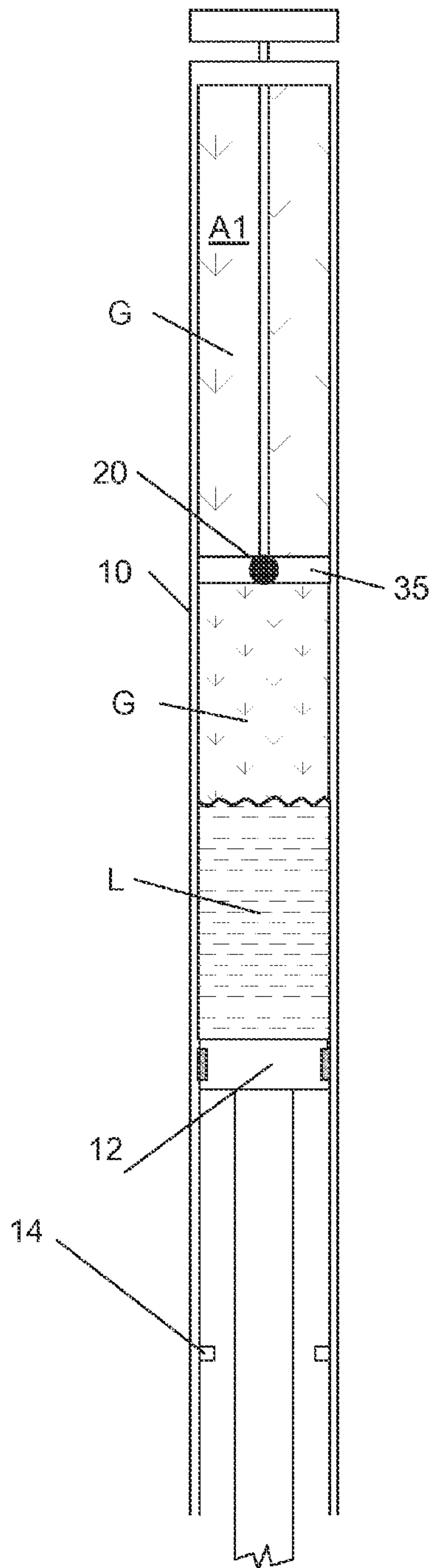
FIG 3A (Short Travel)
