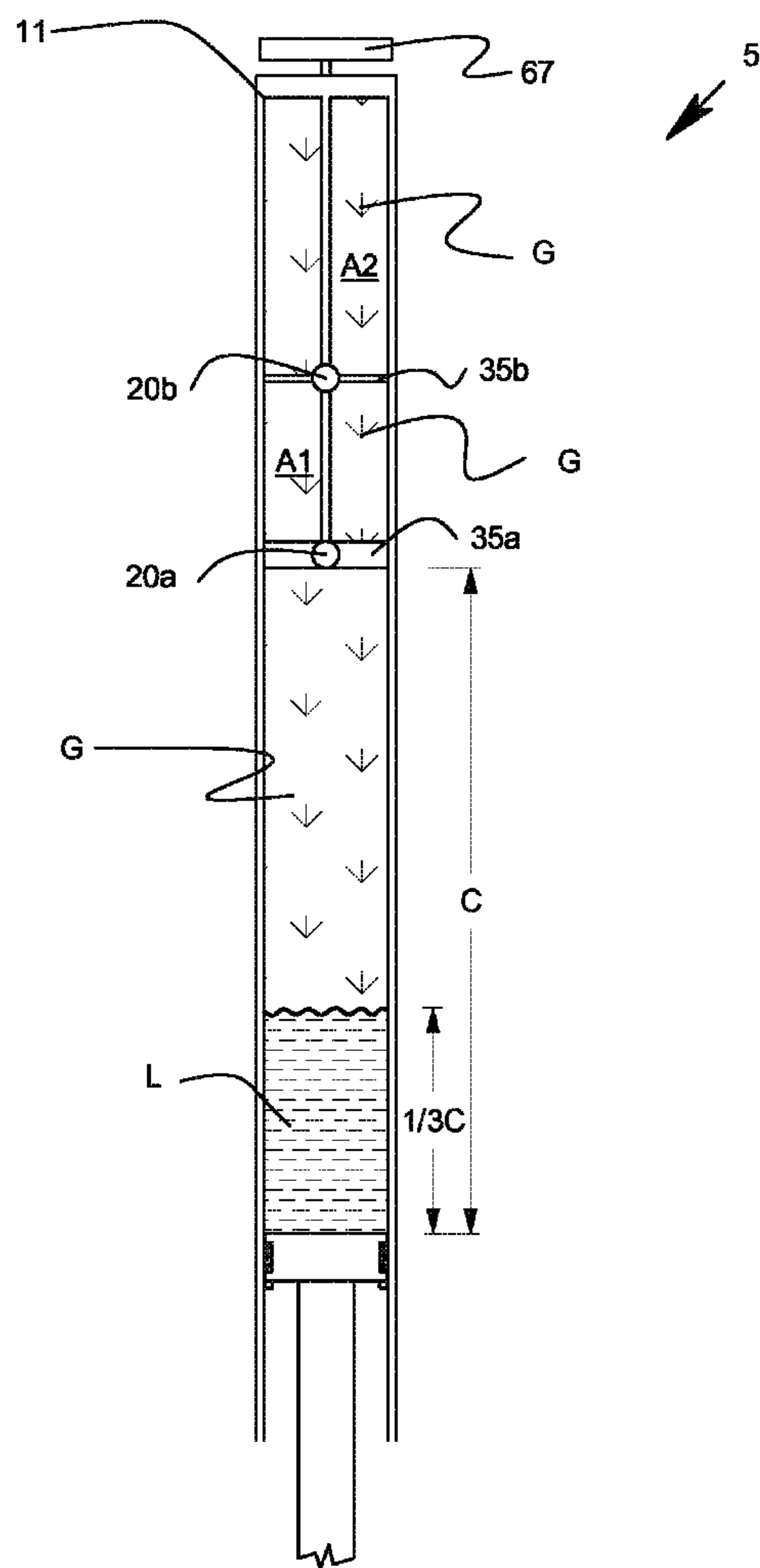
FIG 6 (Two Auxiliary Chambers)
