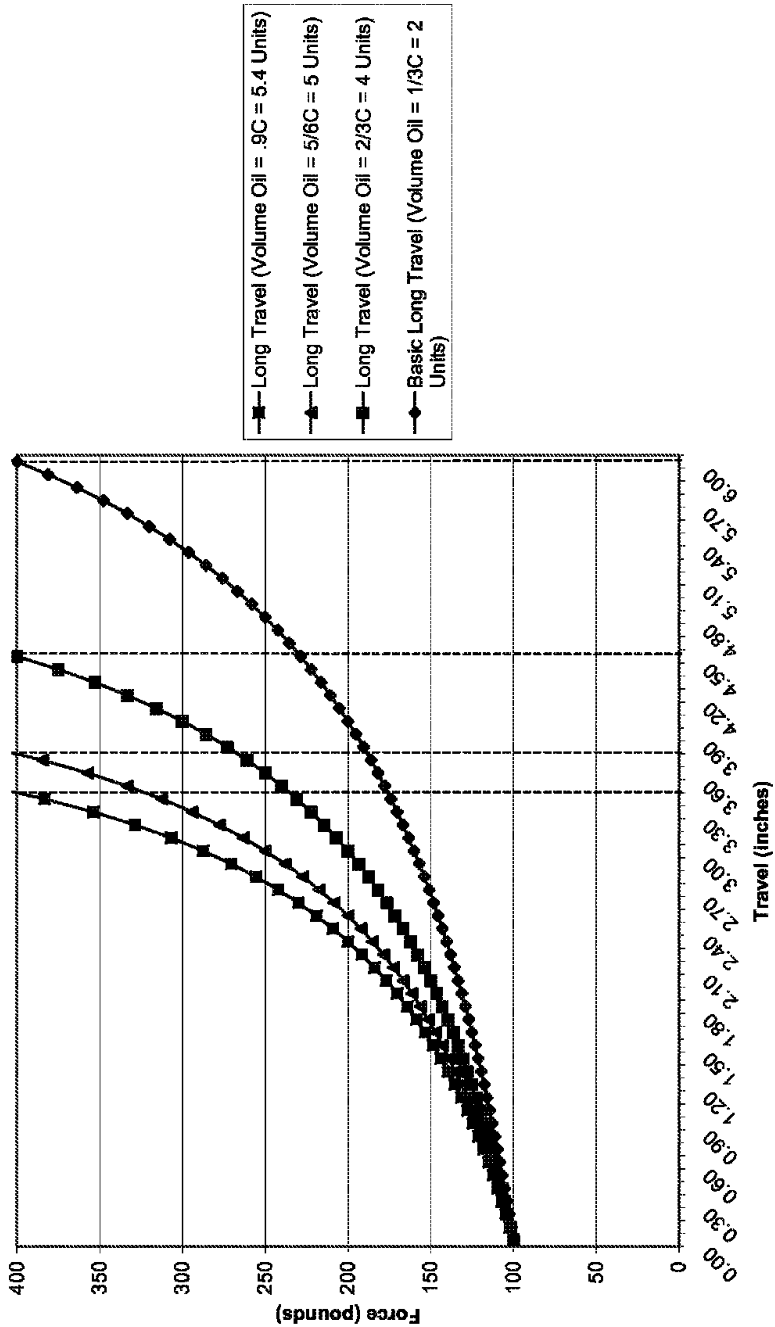
FIG 4E Comparison of Long Travel Modes
