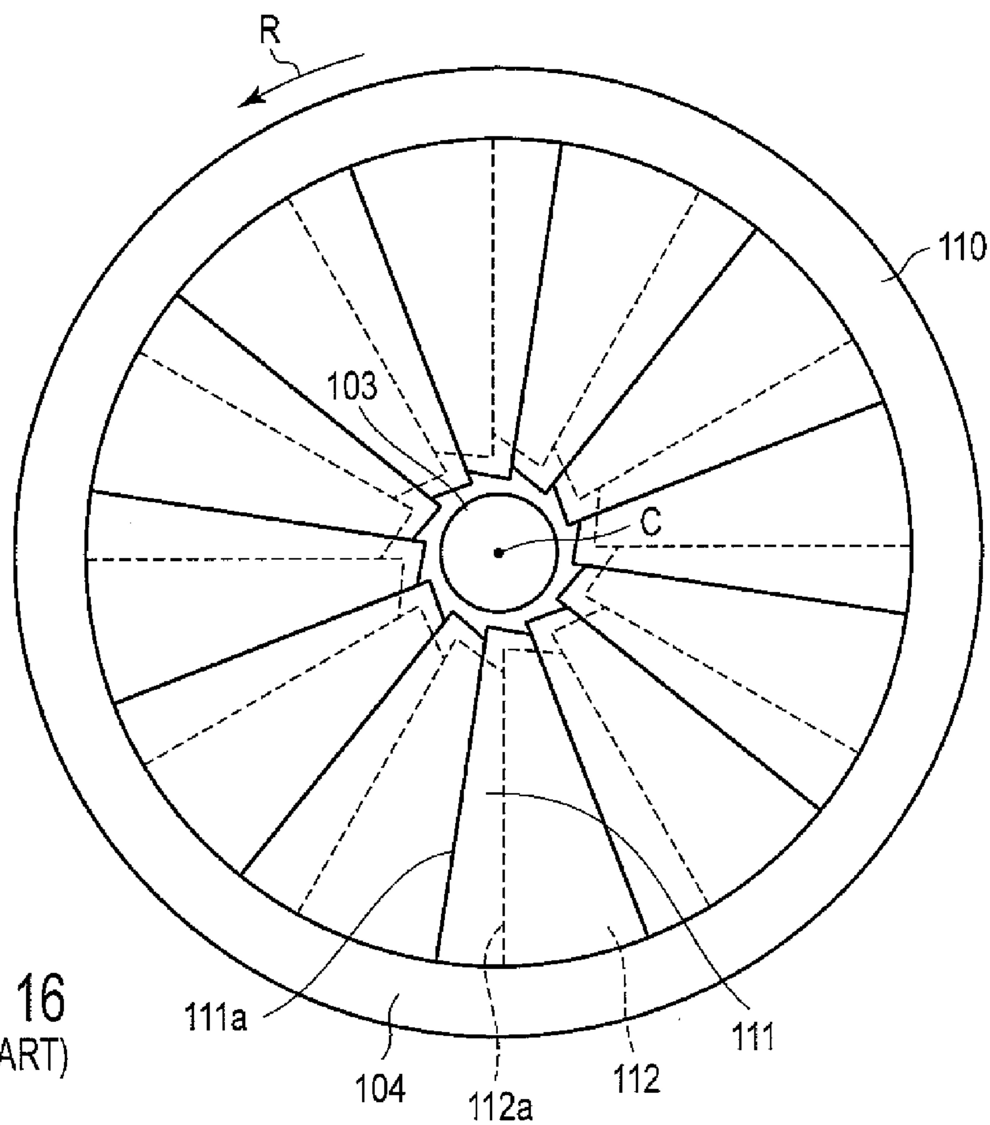
FIG. 15 (PRIOR ART)
