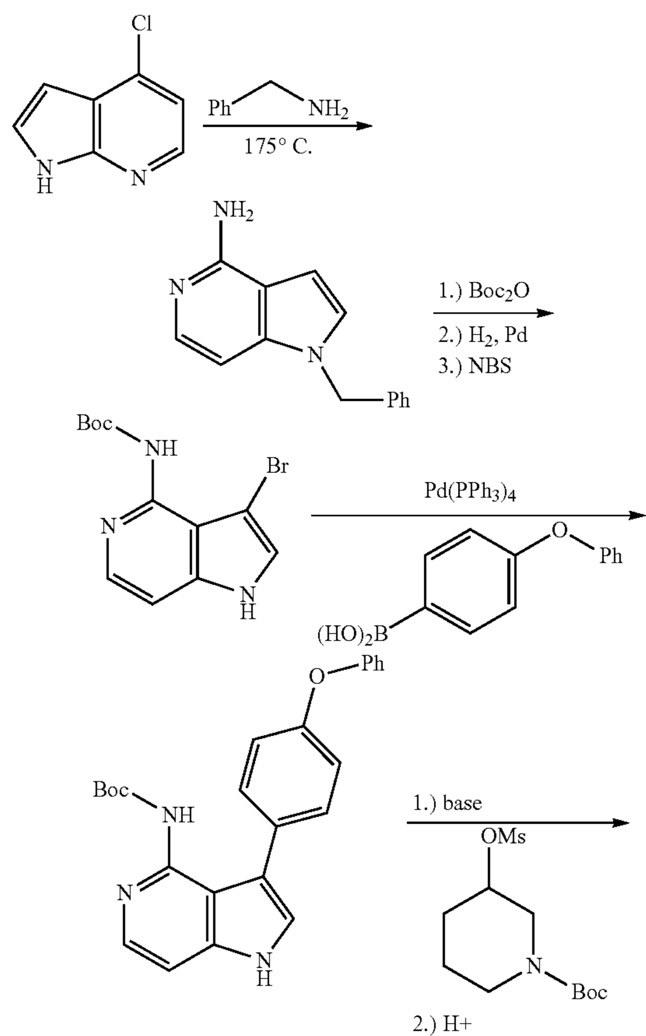
Scheme V.
