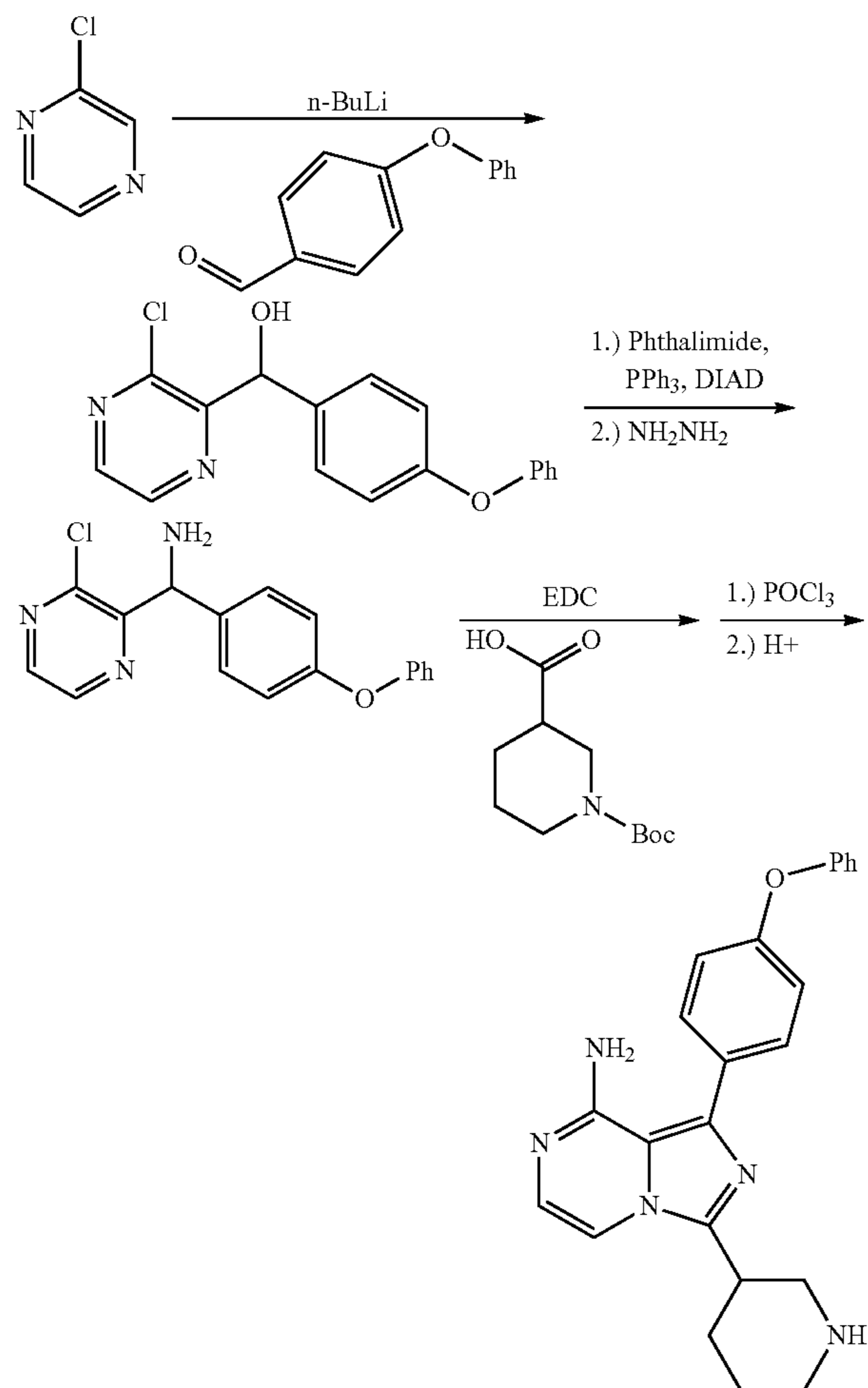
Scheme III
