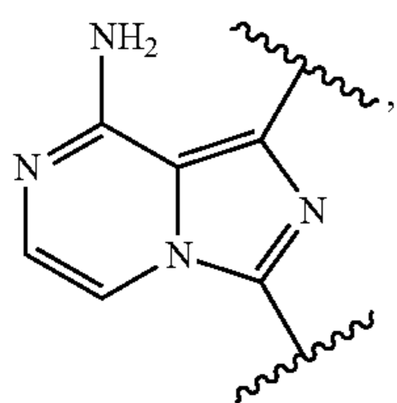
Scheme III
