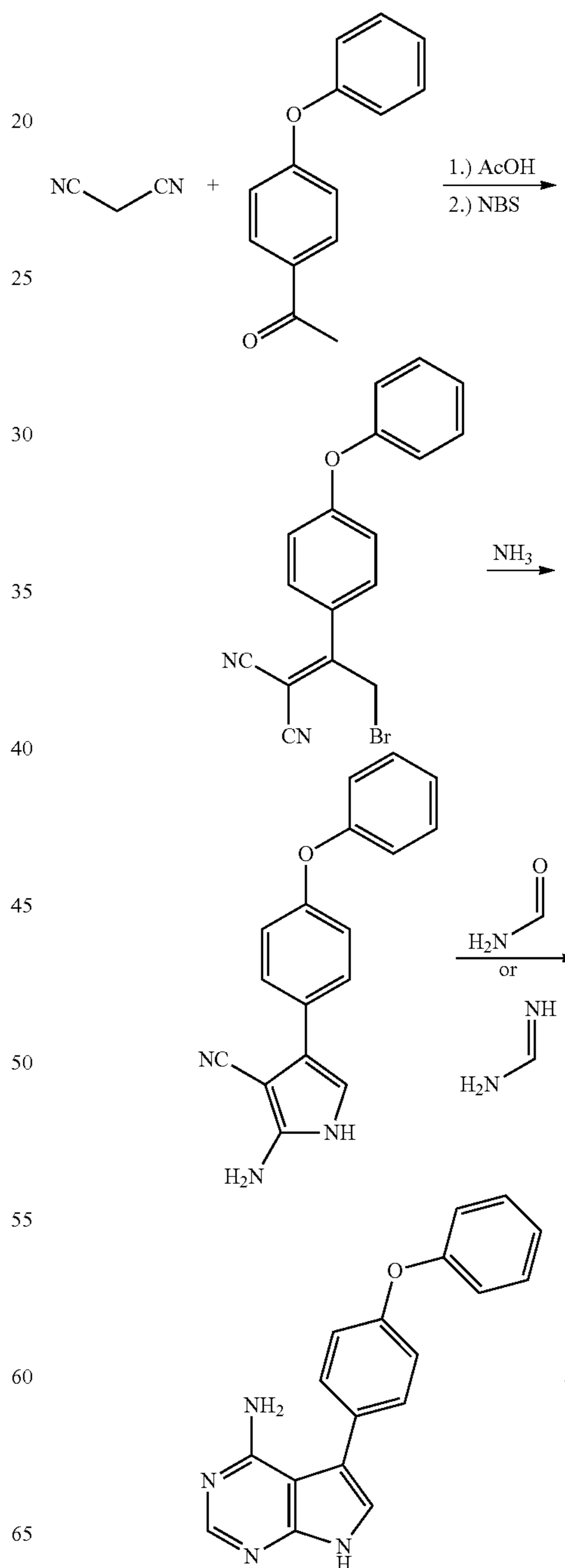
Scheme IV.
