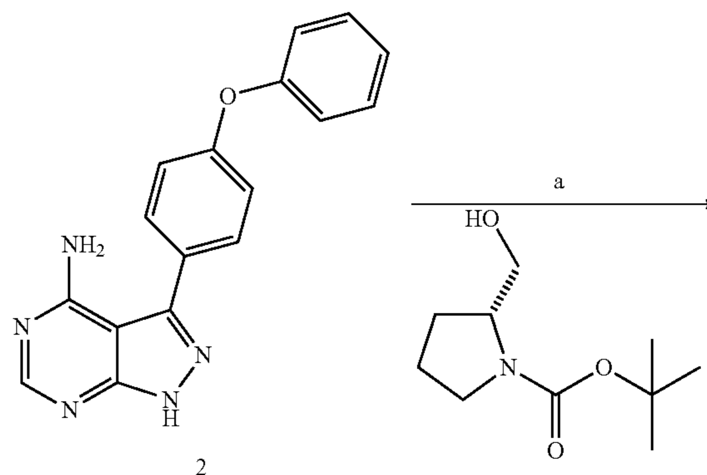
Scheme 1.
