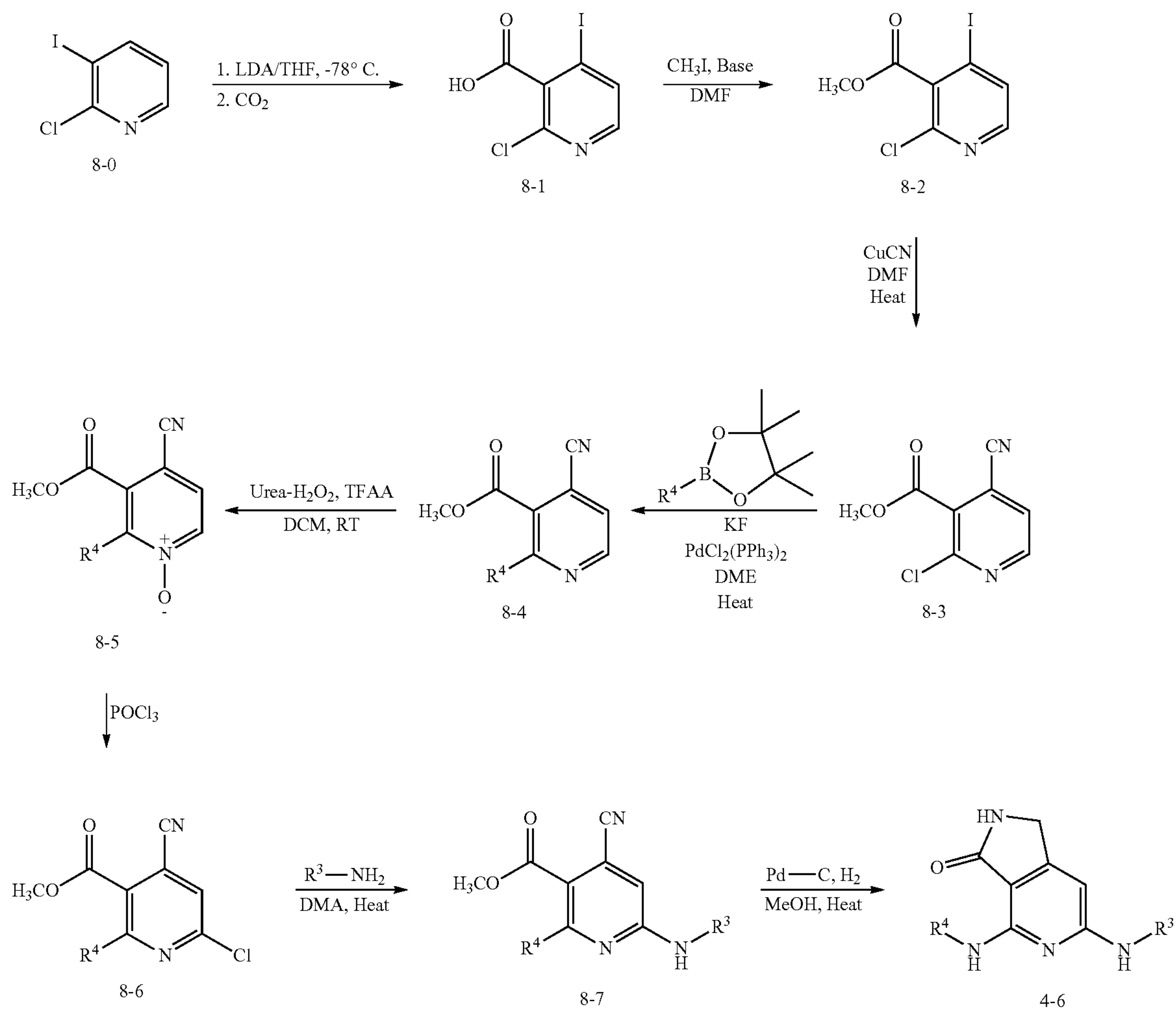
Scheme 8
