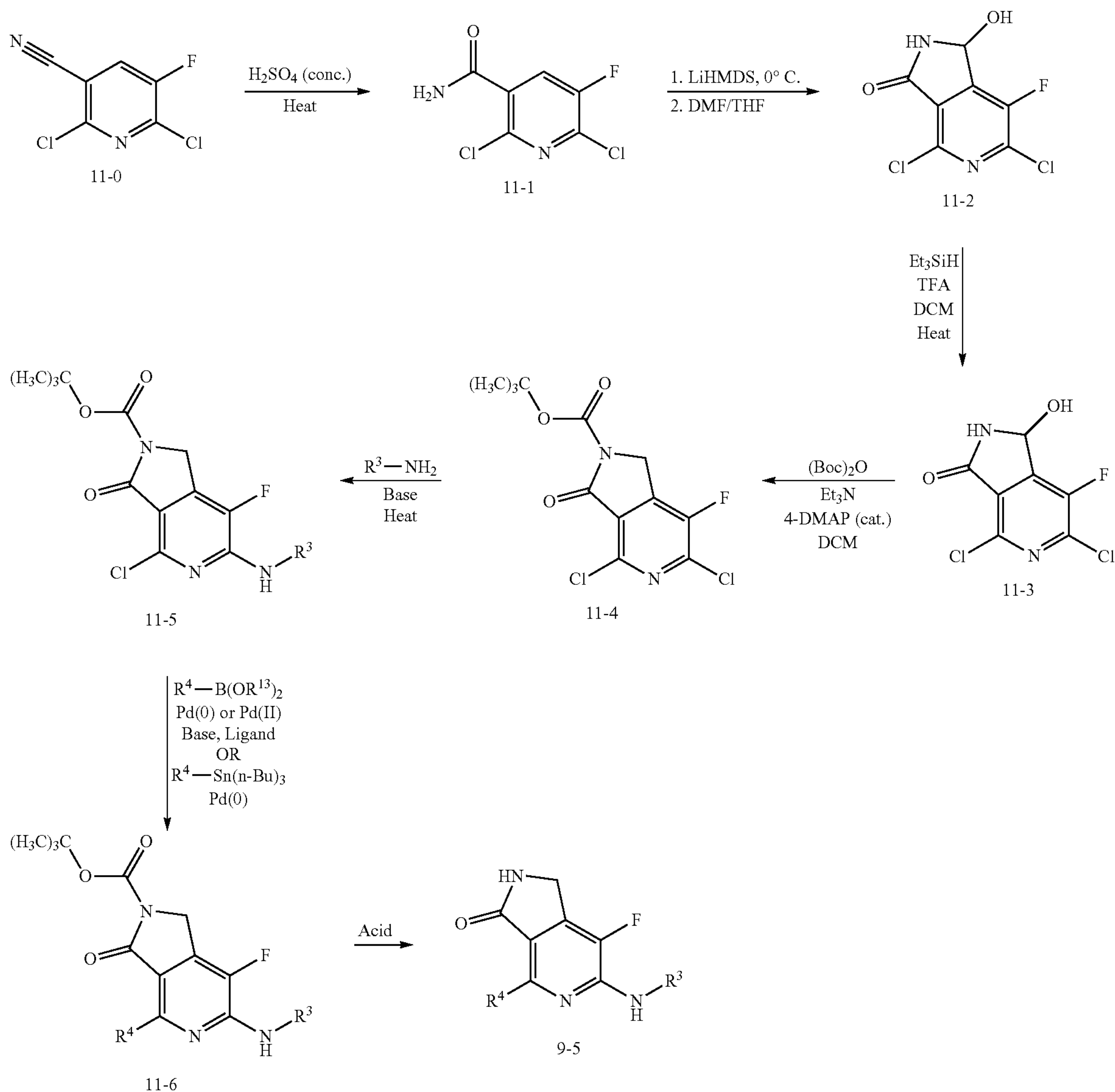
Scheme 11
