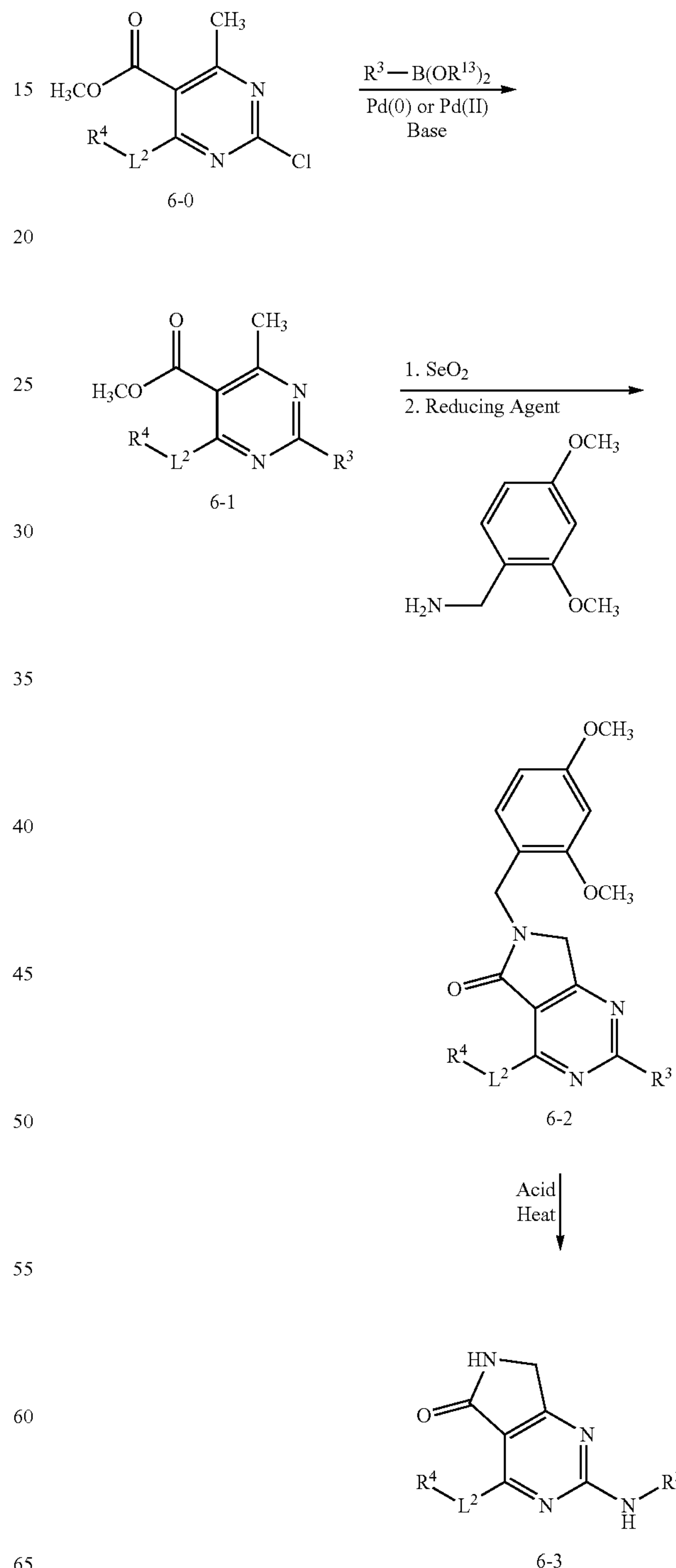
Scheme 6
