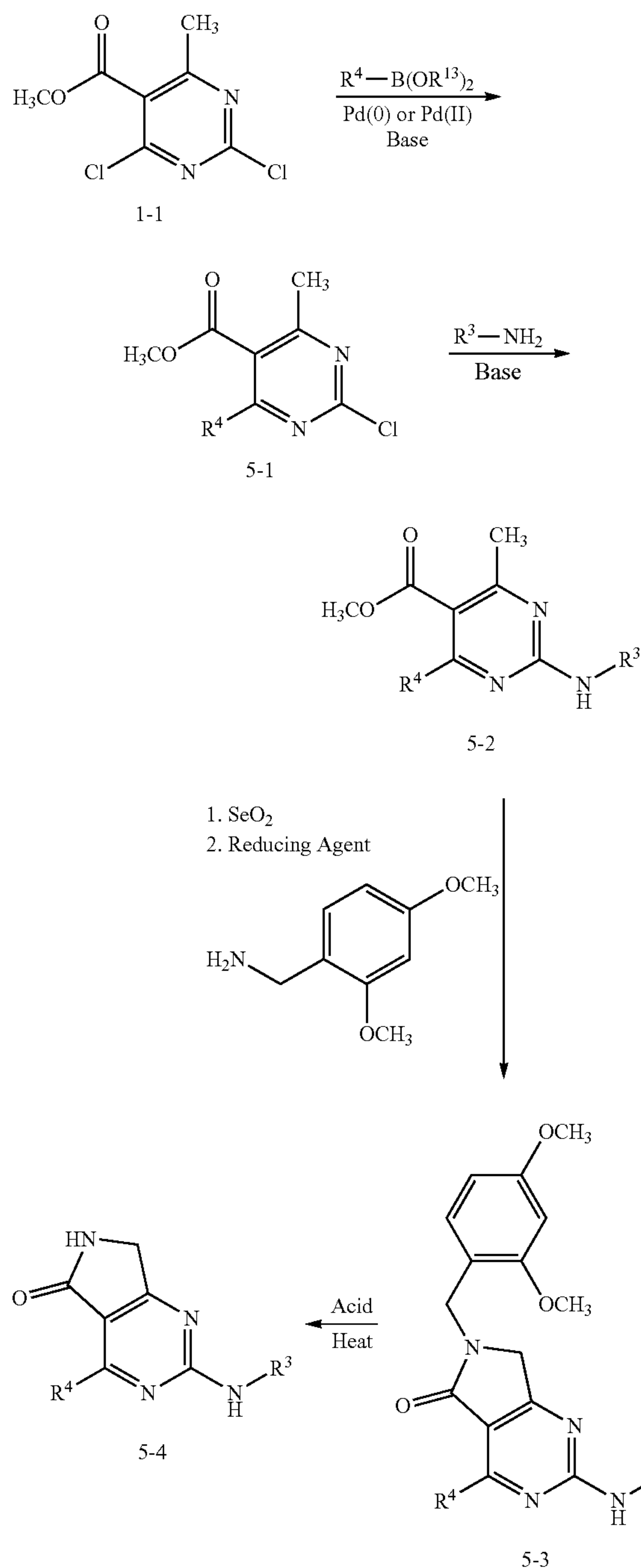
Scheme 5
