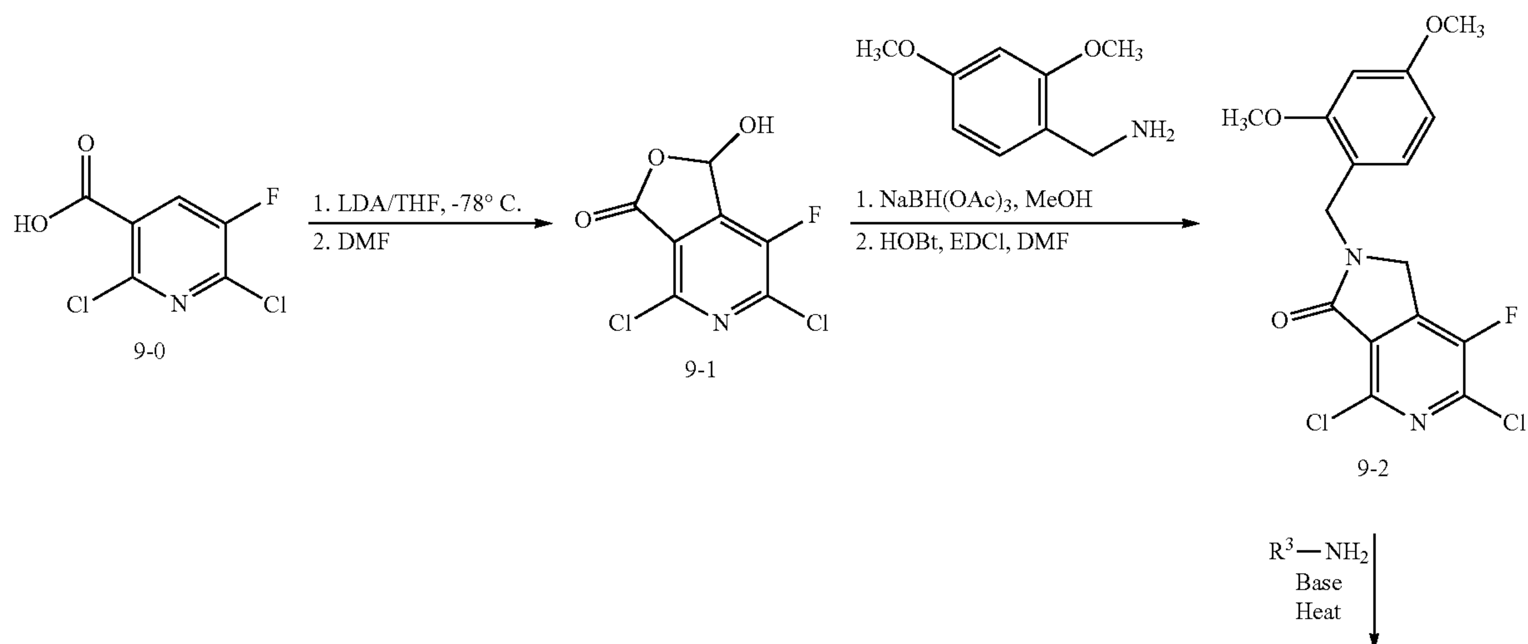
Scheme 9
