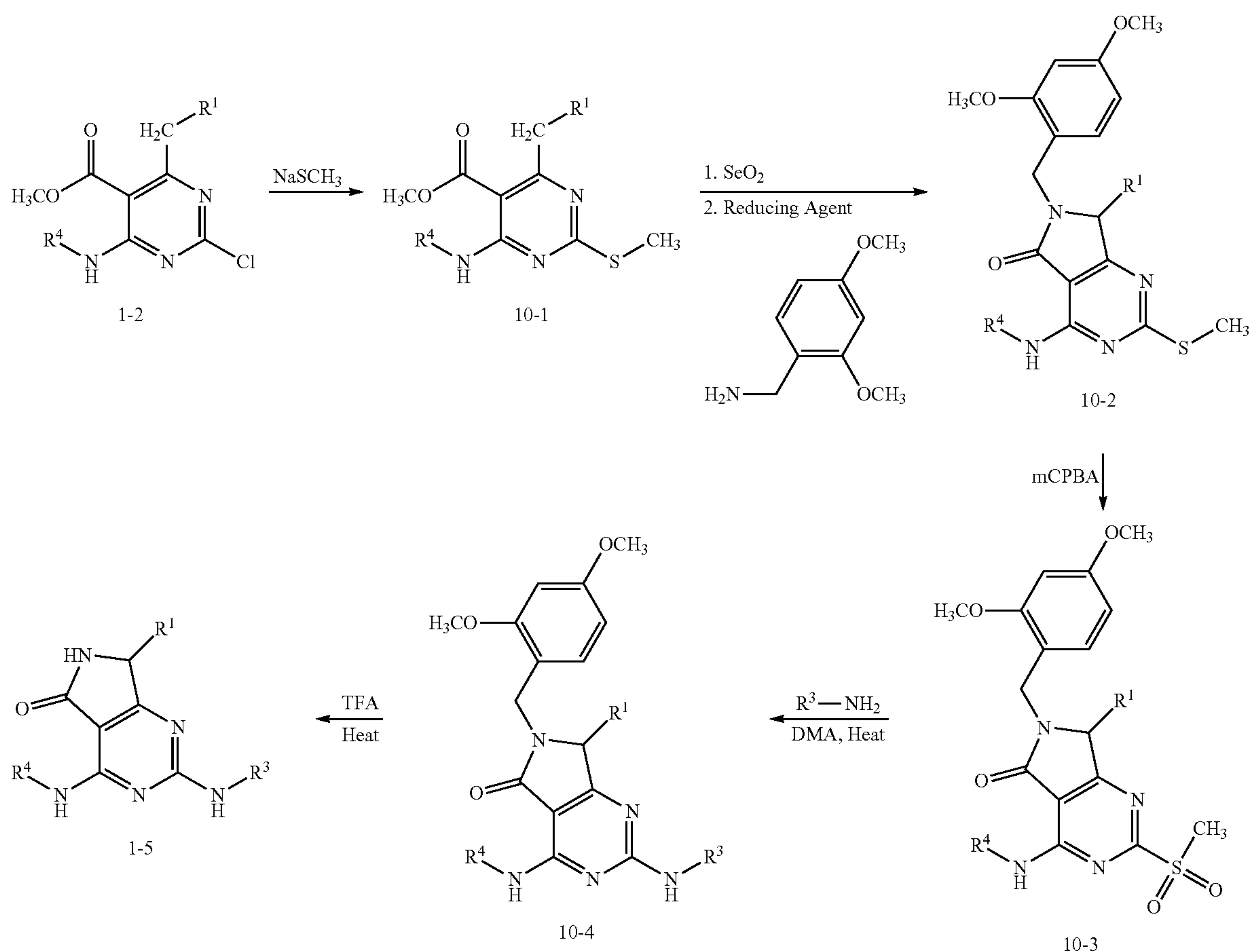
Scheme 10
