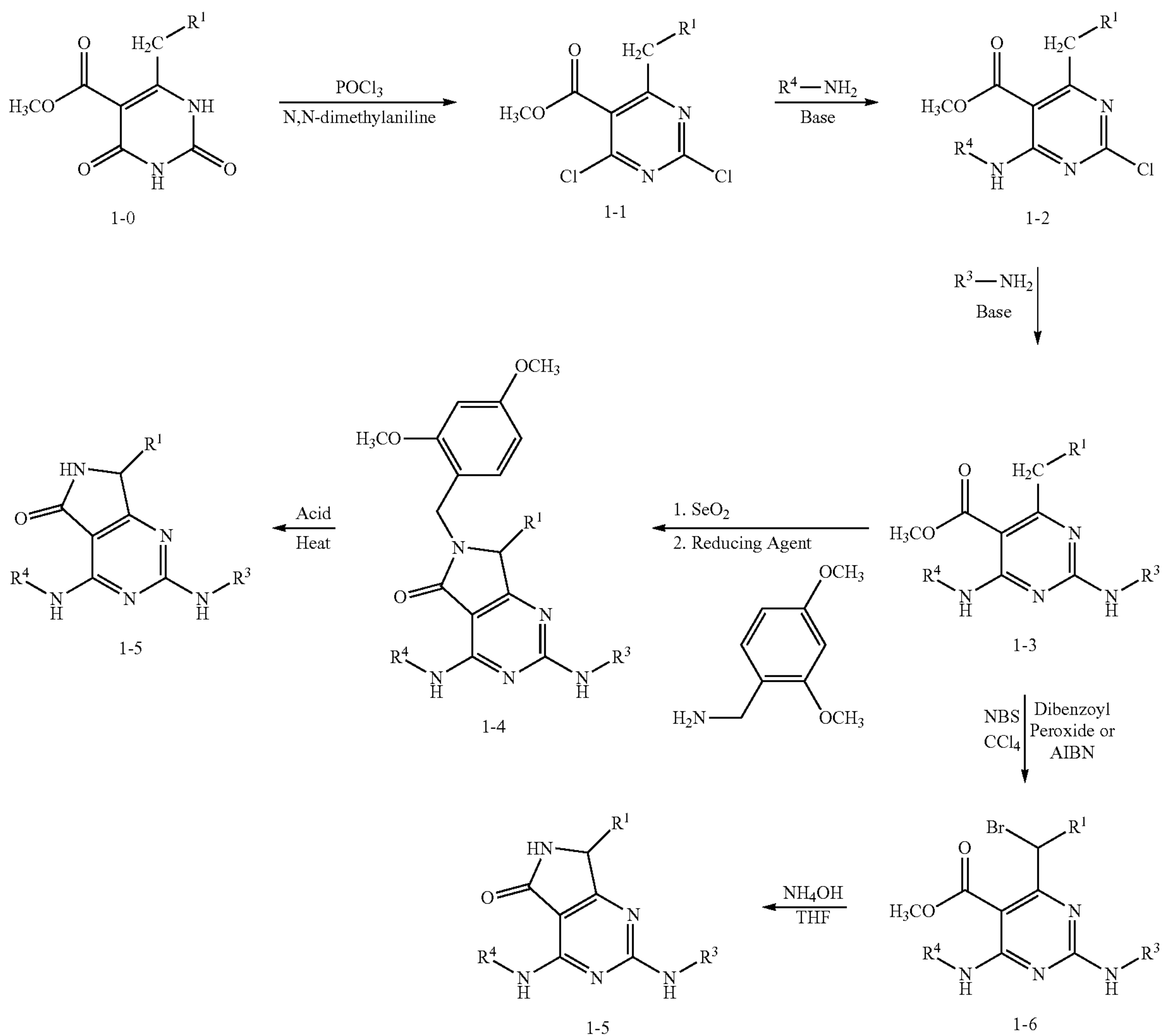
Scheme 1
