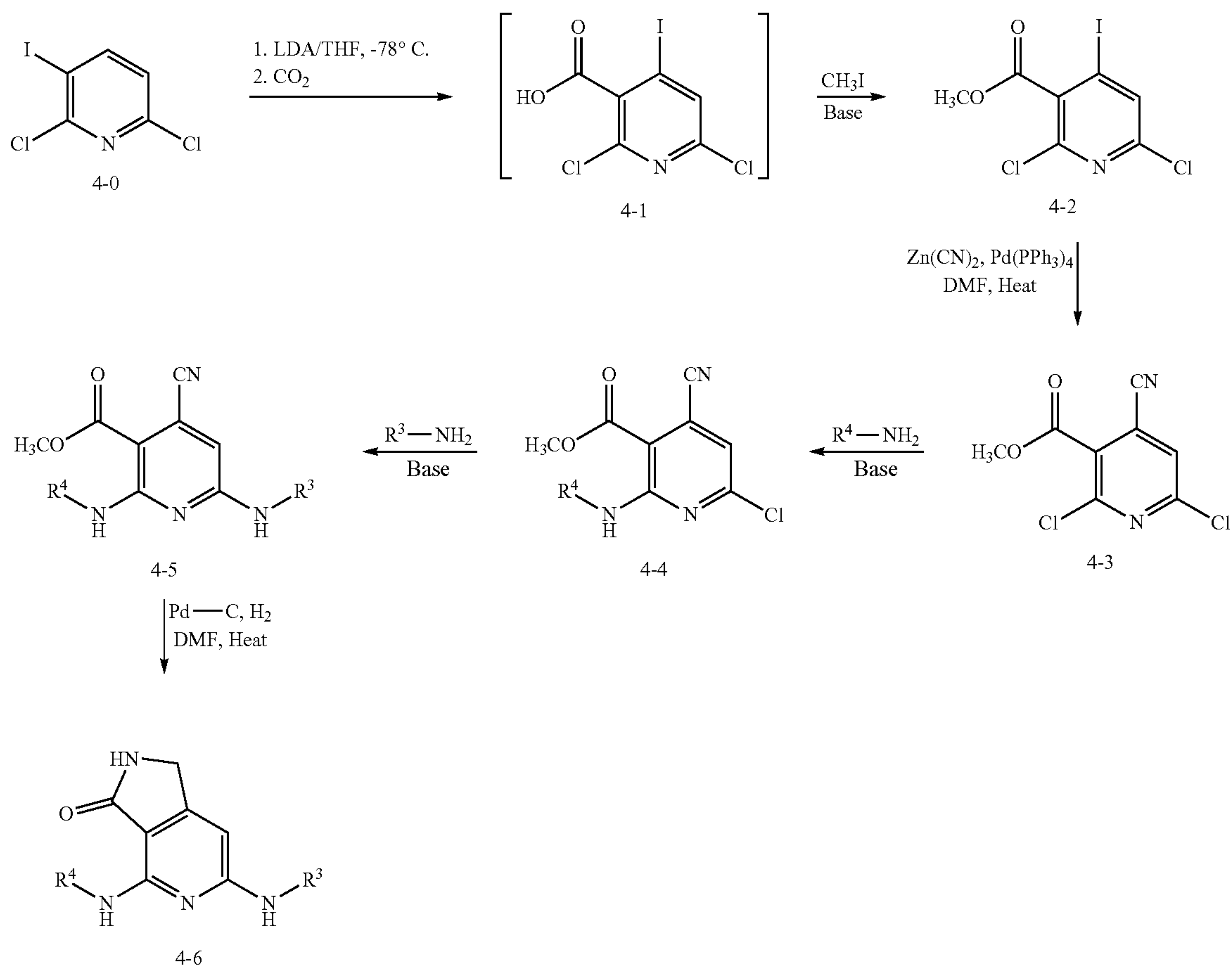
Scheme 4
