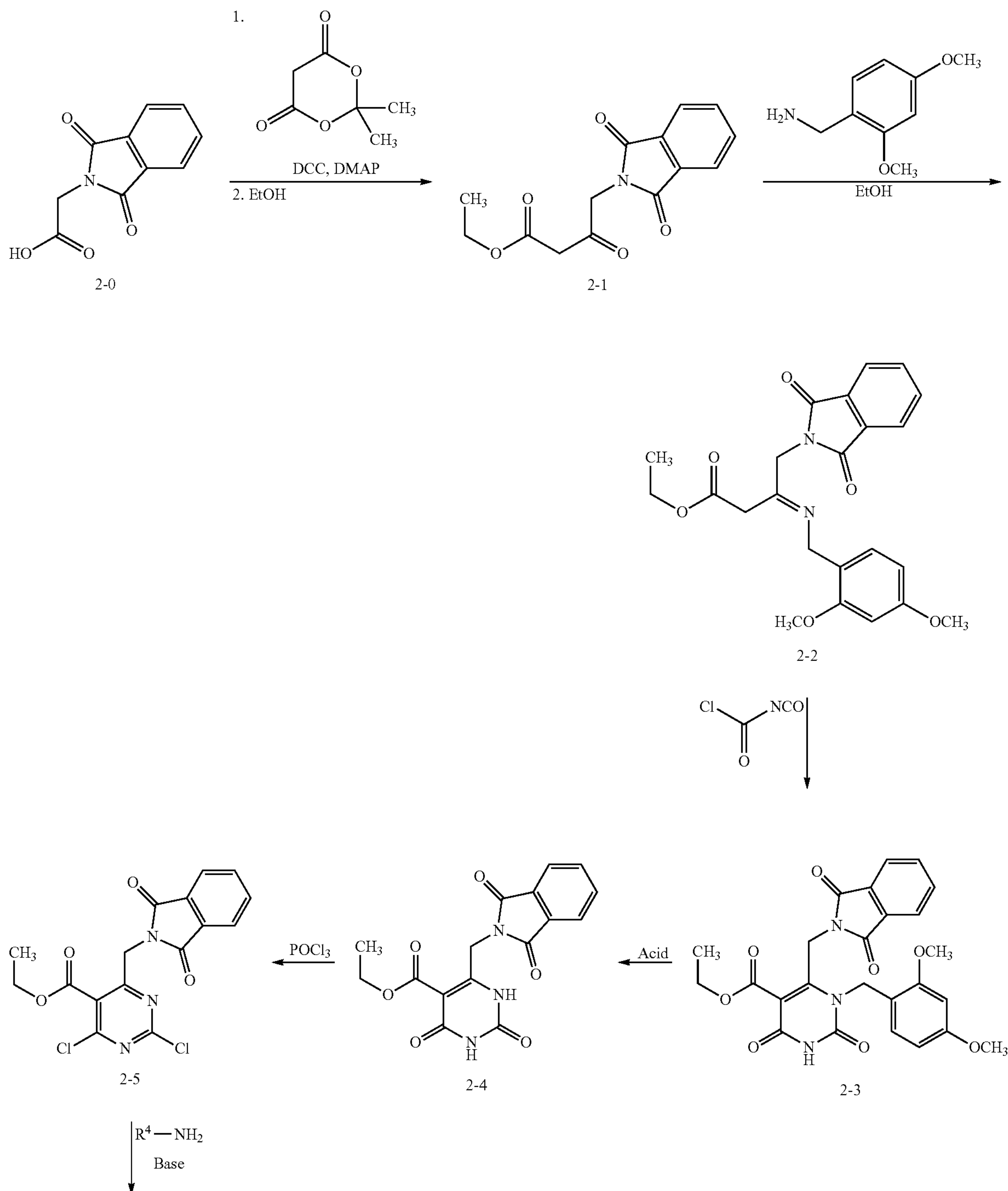
Scheme 2
