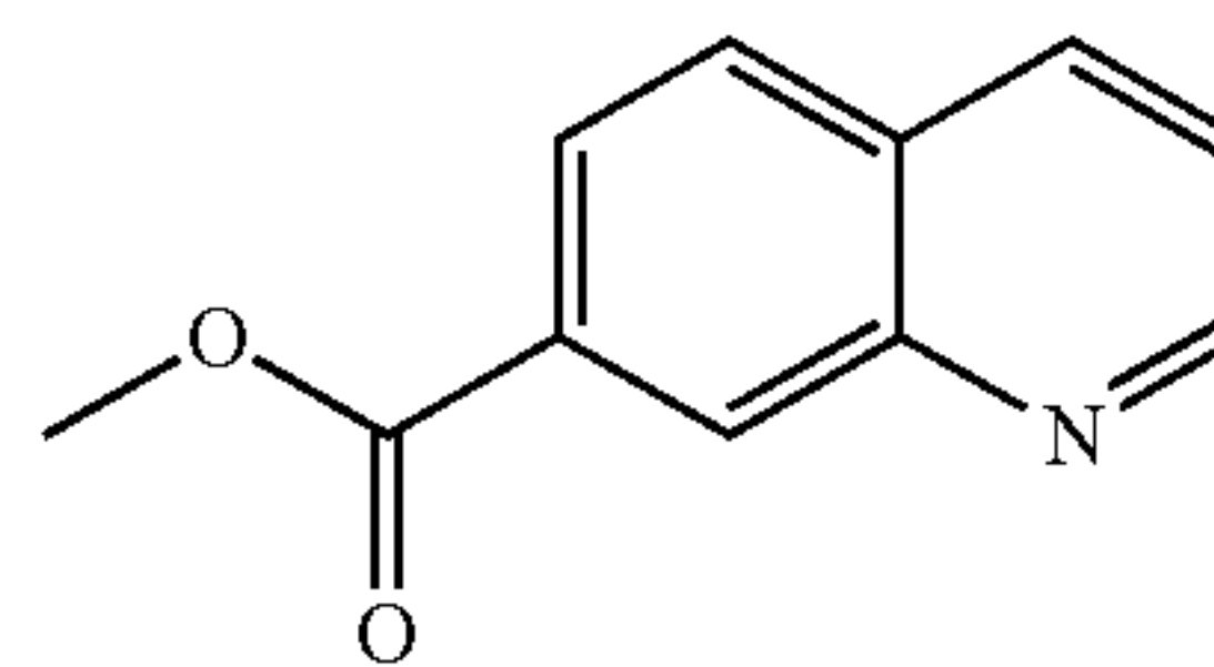
Step 1: methyl quinoline-7-carboxylate
