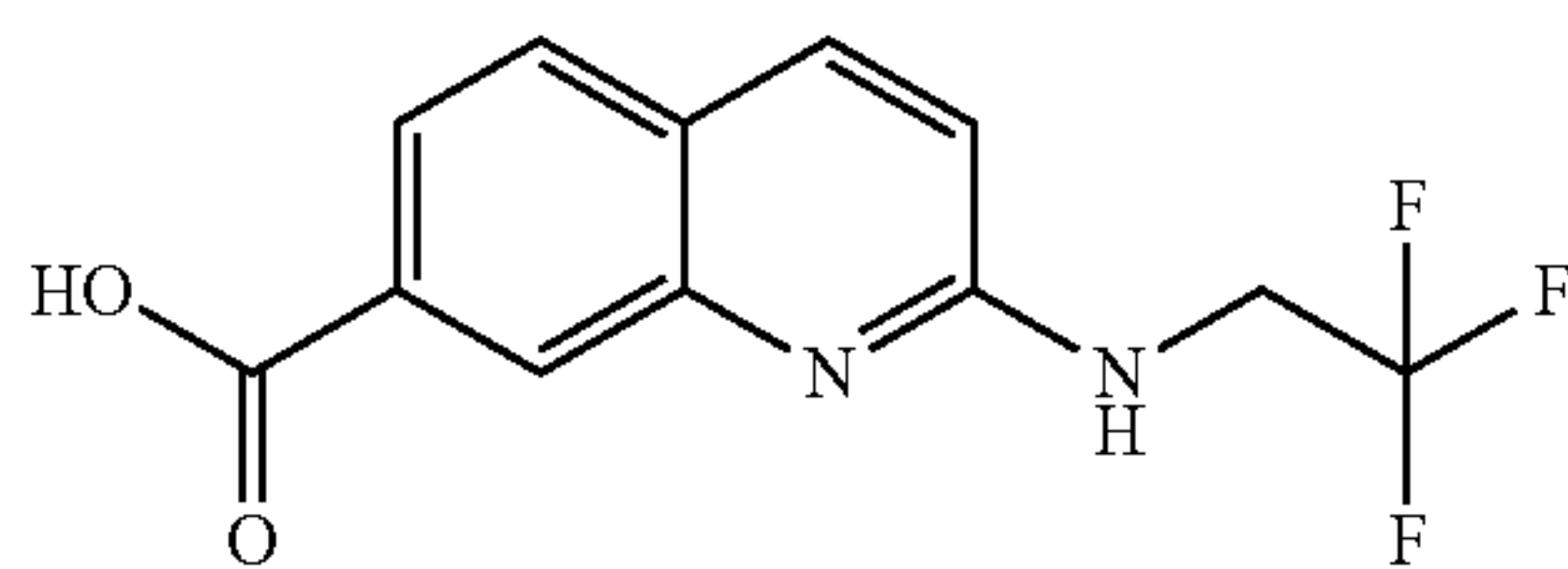
2-((2,2,2-trifluoroethyl)amino)quinoline-7-carboxylic acid
