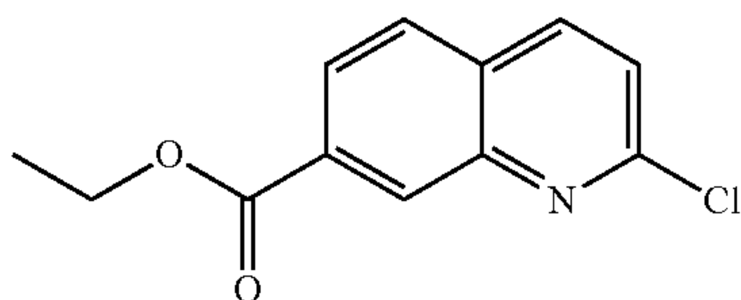
Step 1: ethyl 2-chloroquinoline-7-carboxylate
