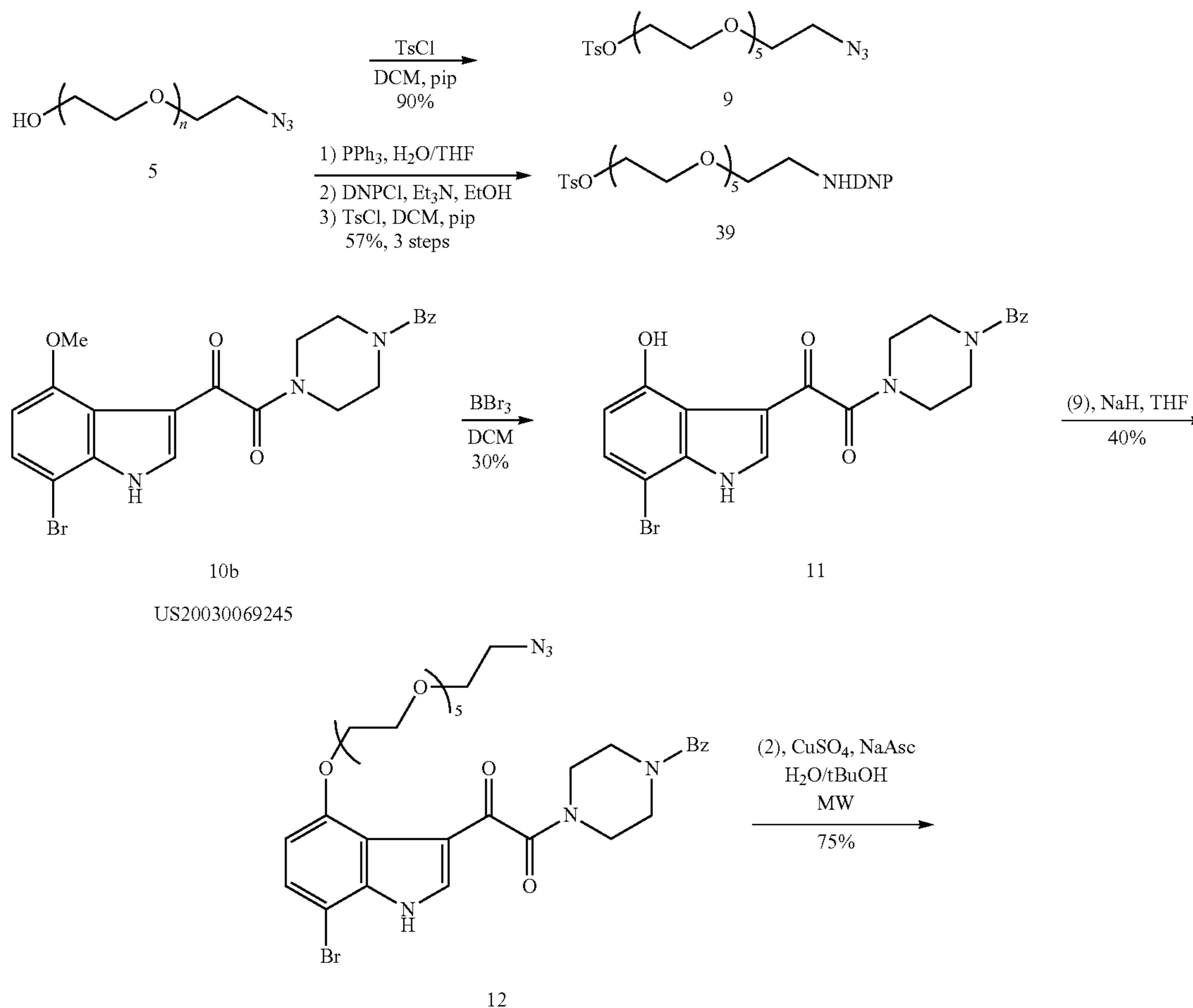
Supplementary Scheme 4. Representative Synthesis of ARM-H type (14) and type (28) molecules
