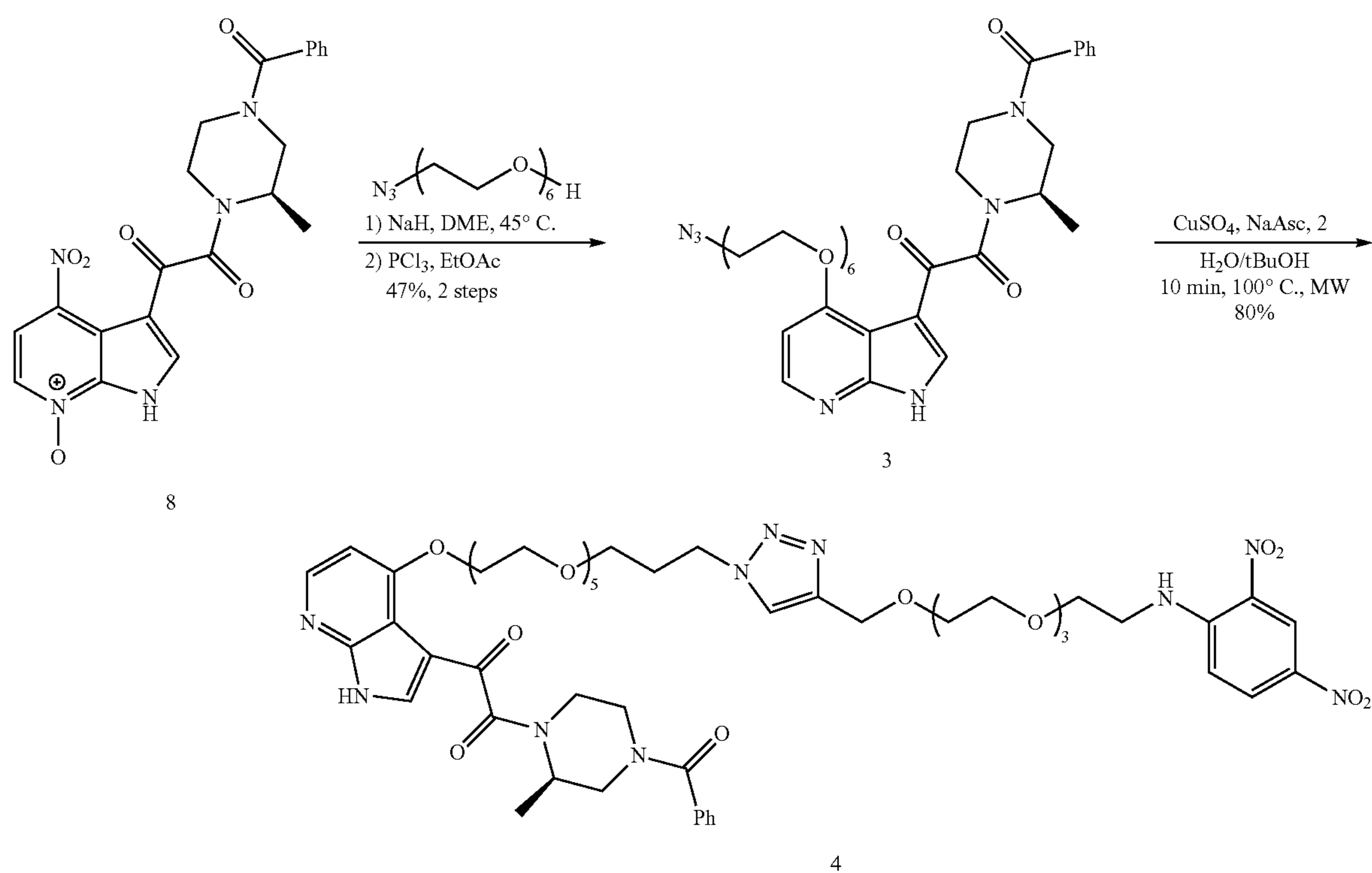
Supplementary Scheme 3. Representative synthesis of ARM-H type (4) analogs.
