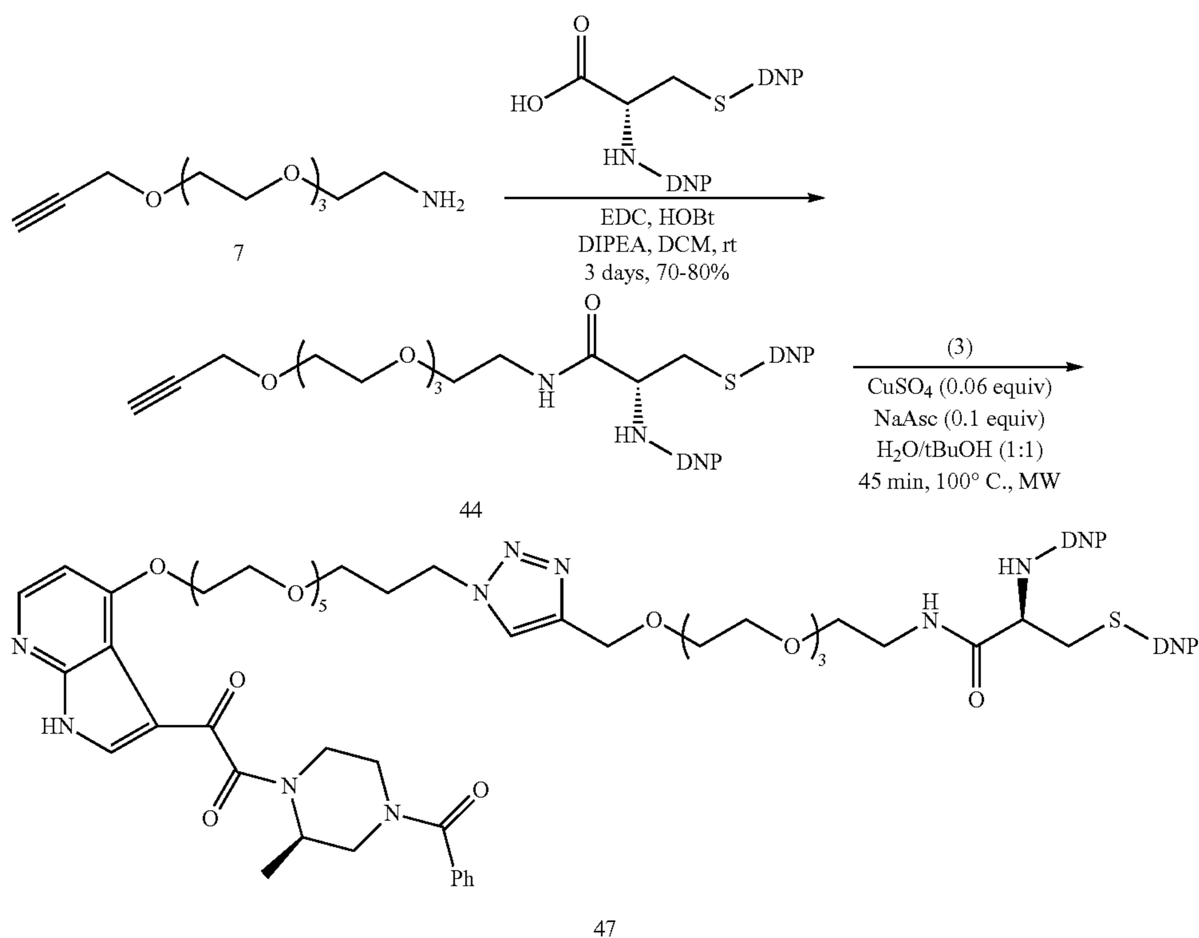
Supplementary Scheme 2. Representative Synthesis of ARM-H type (47) molecules with DNP containing Amino Acids
