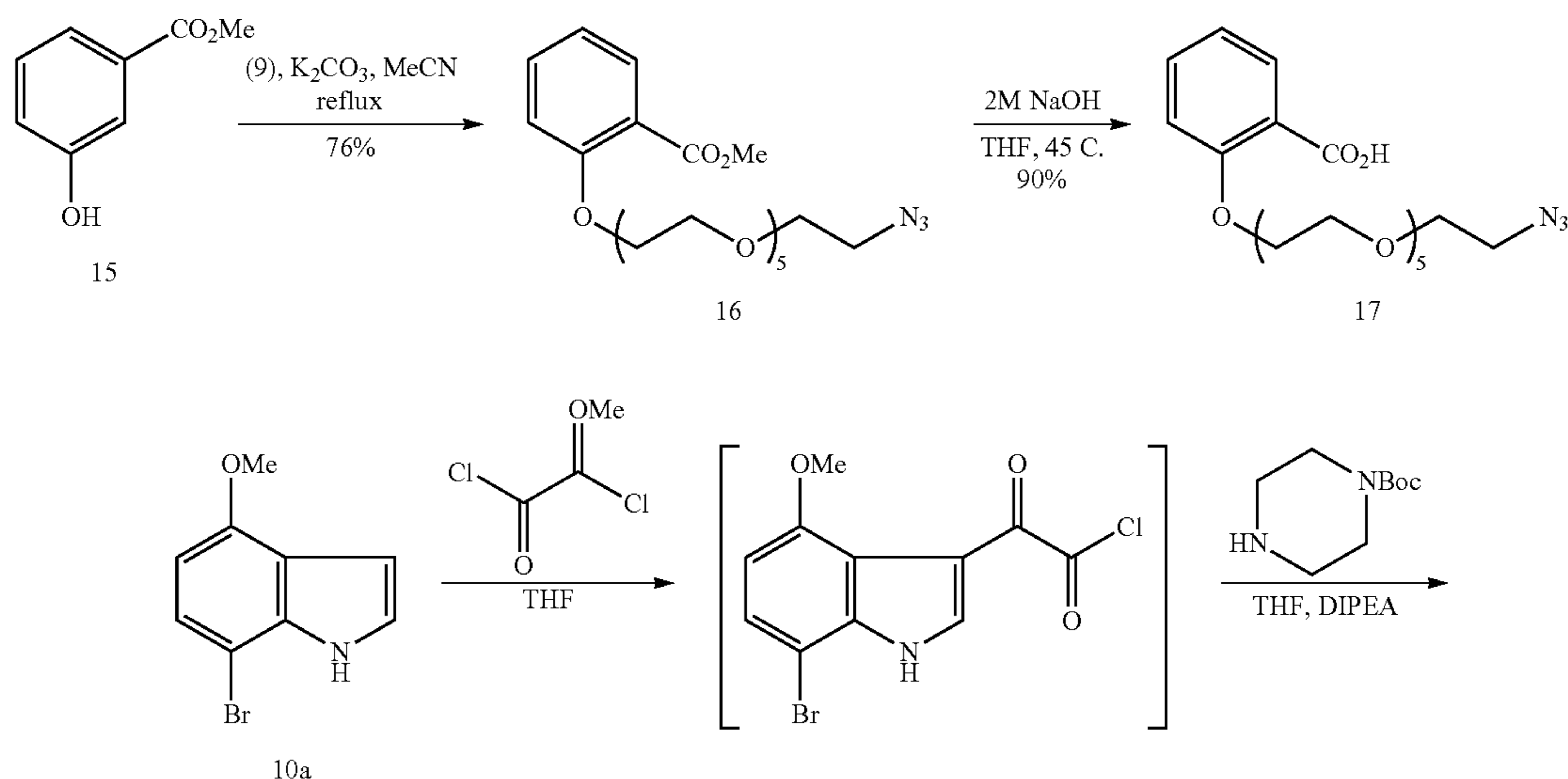
Supplementary Scheme 5. Representative Synthesis of ARM-H type (22) molecules
