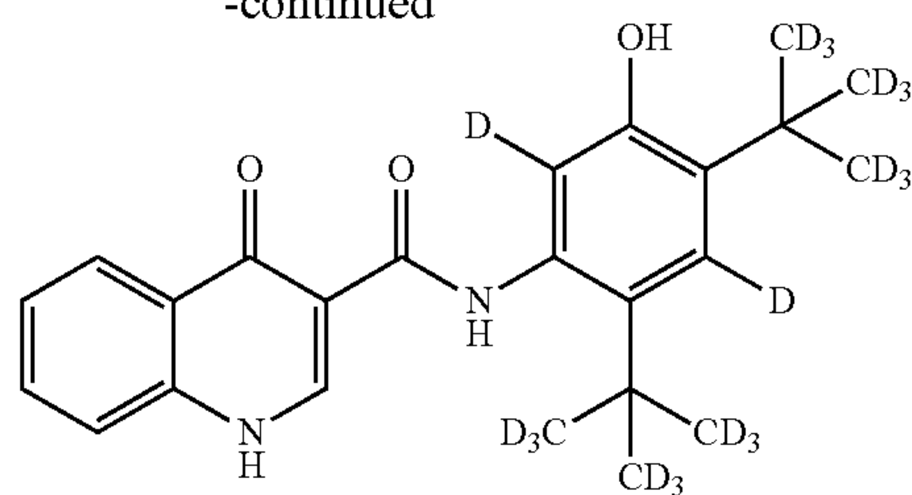
Compound 110
