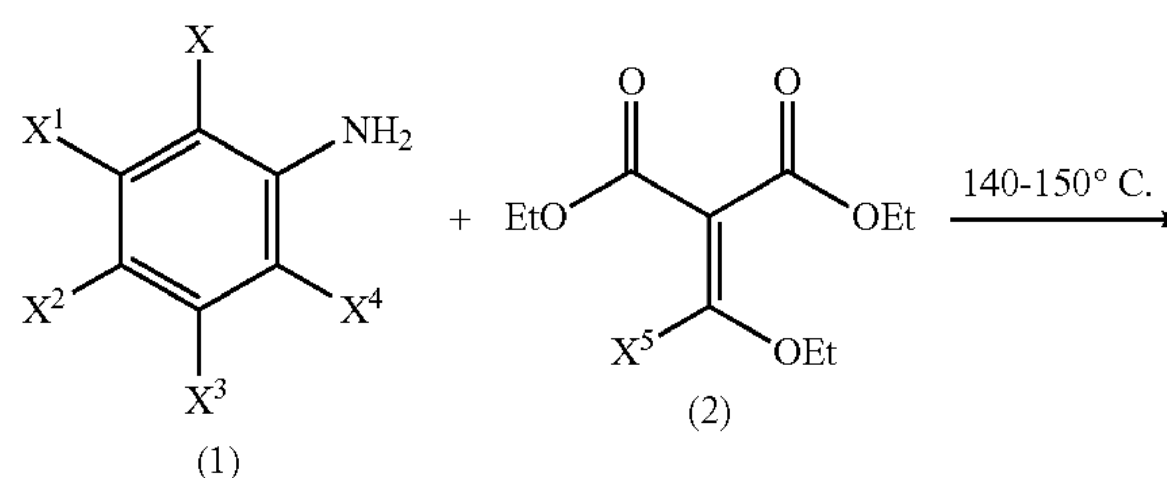
Scheme 2:
