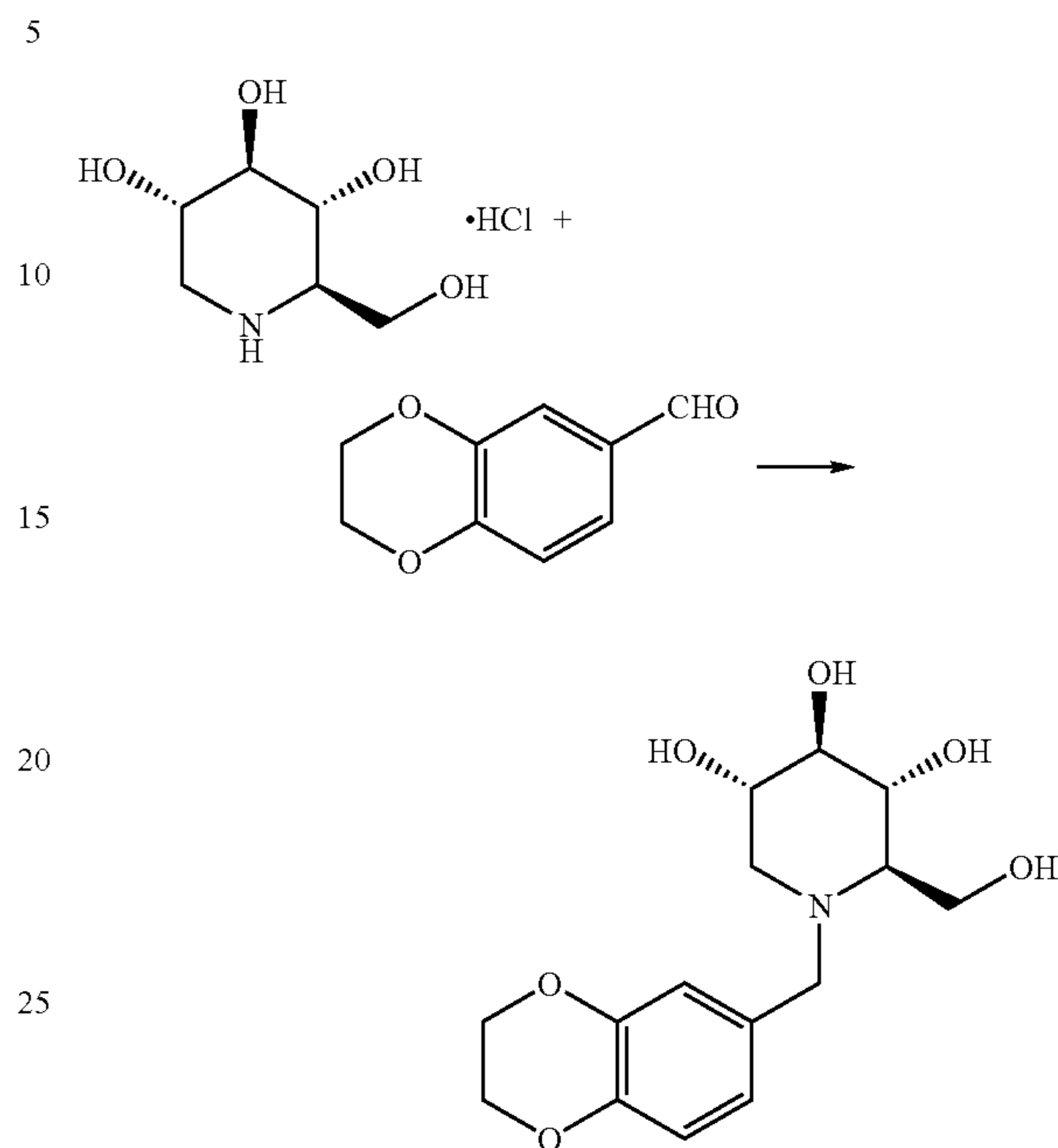
N-((1,4-Benzodioxan-6-yl)methyl)deoxynorjirimycin (Compound 28)
