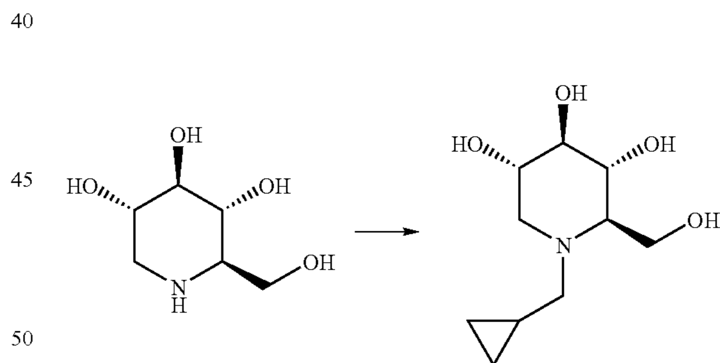
N-Cyclopropylmethyl-1-deoxynojirimycin (Compound 11) [GENERAL IMINOSUGAR PREP-3]
