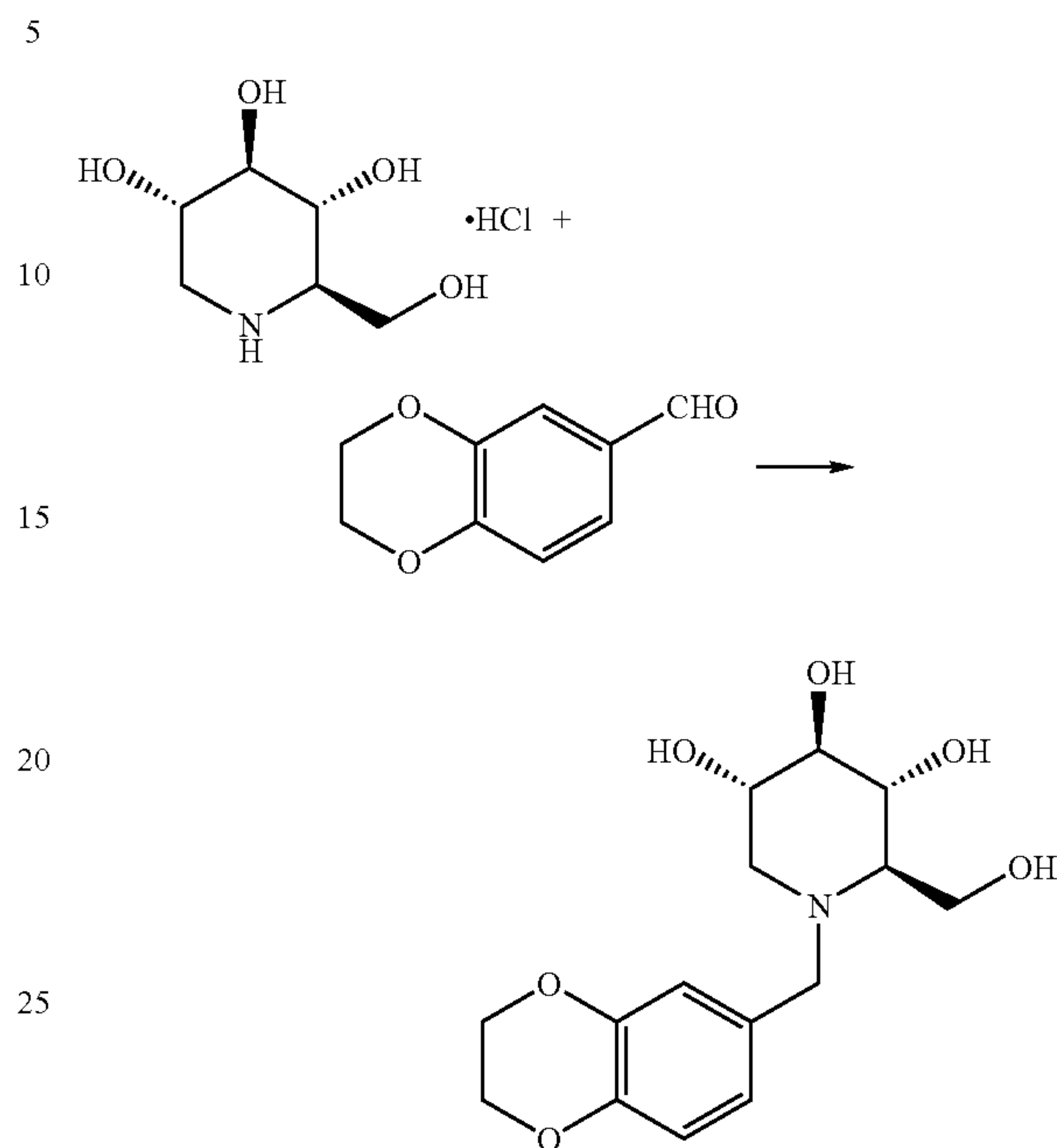
N-((1,4-Benzodioxan-6-yl)methyl)deoxynorjirimycin (Compound 28)
