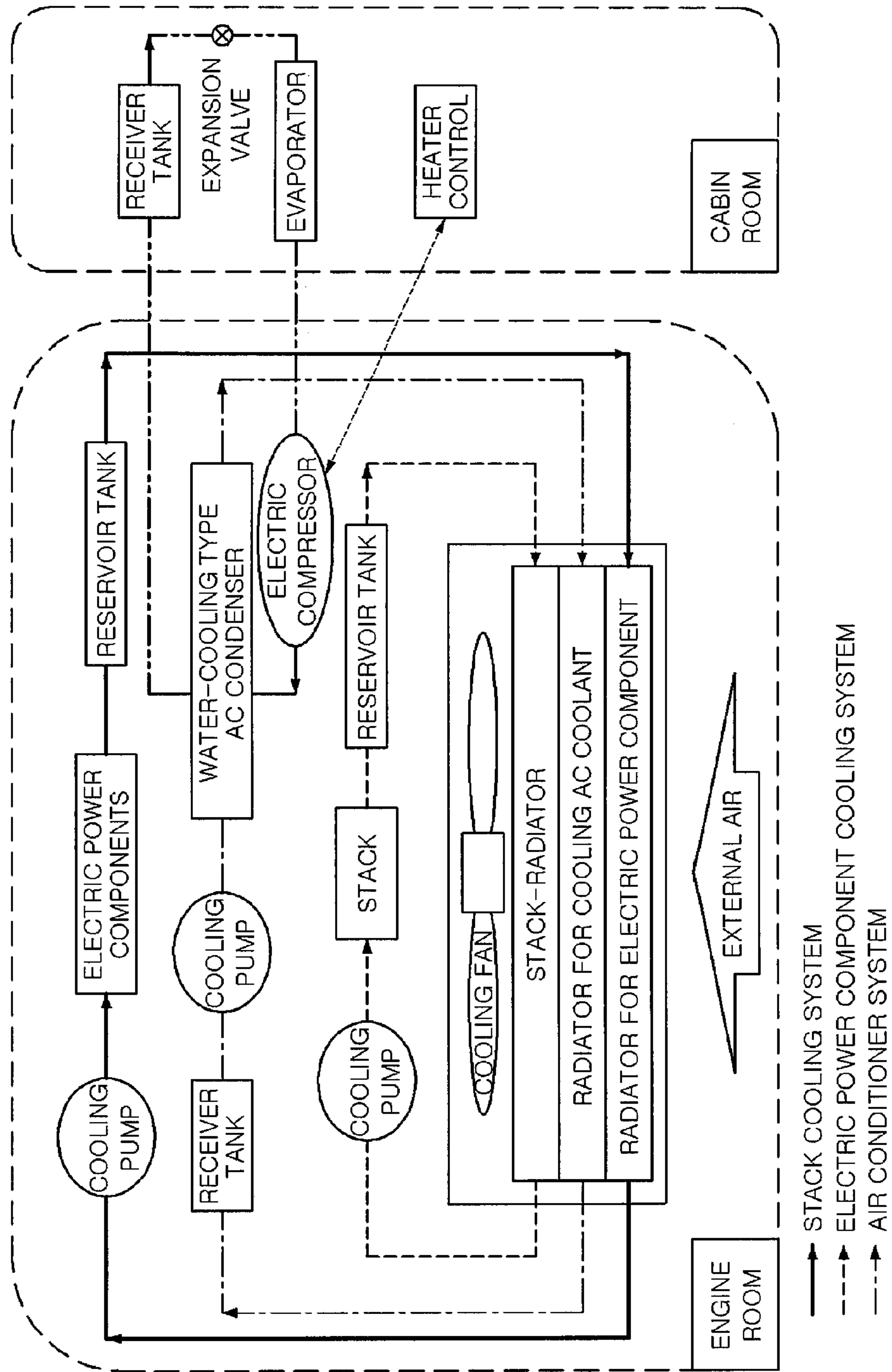
FIG.2 (Prior Art)
