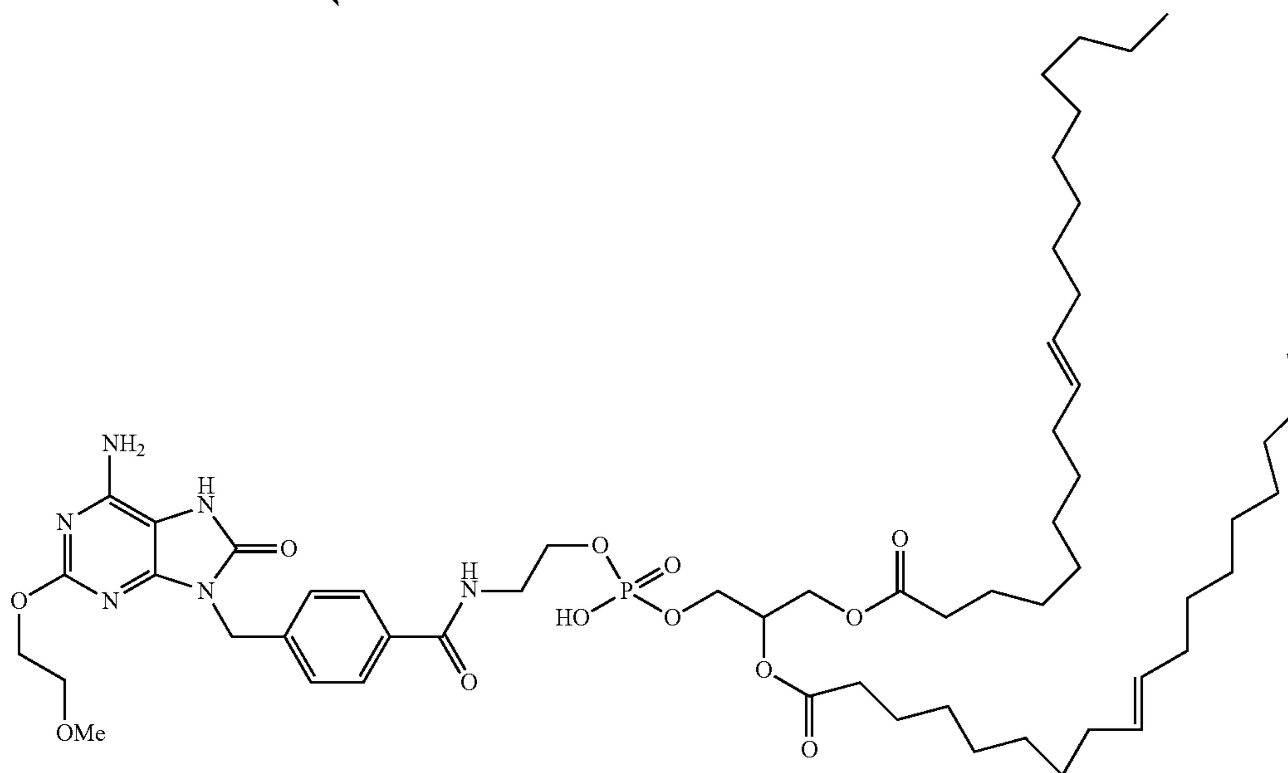
Compound A
