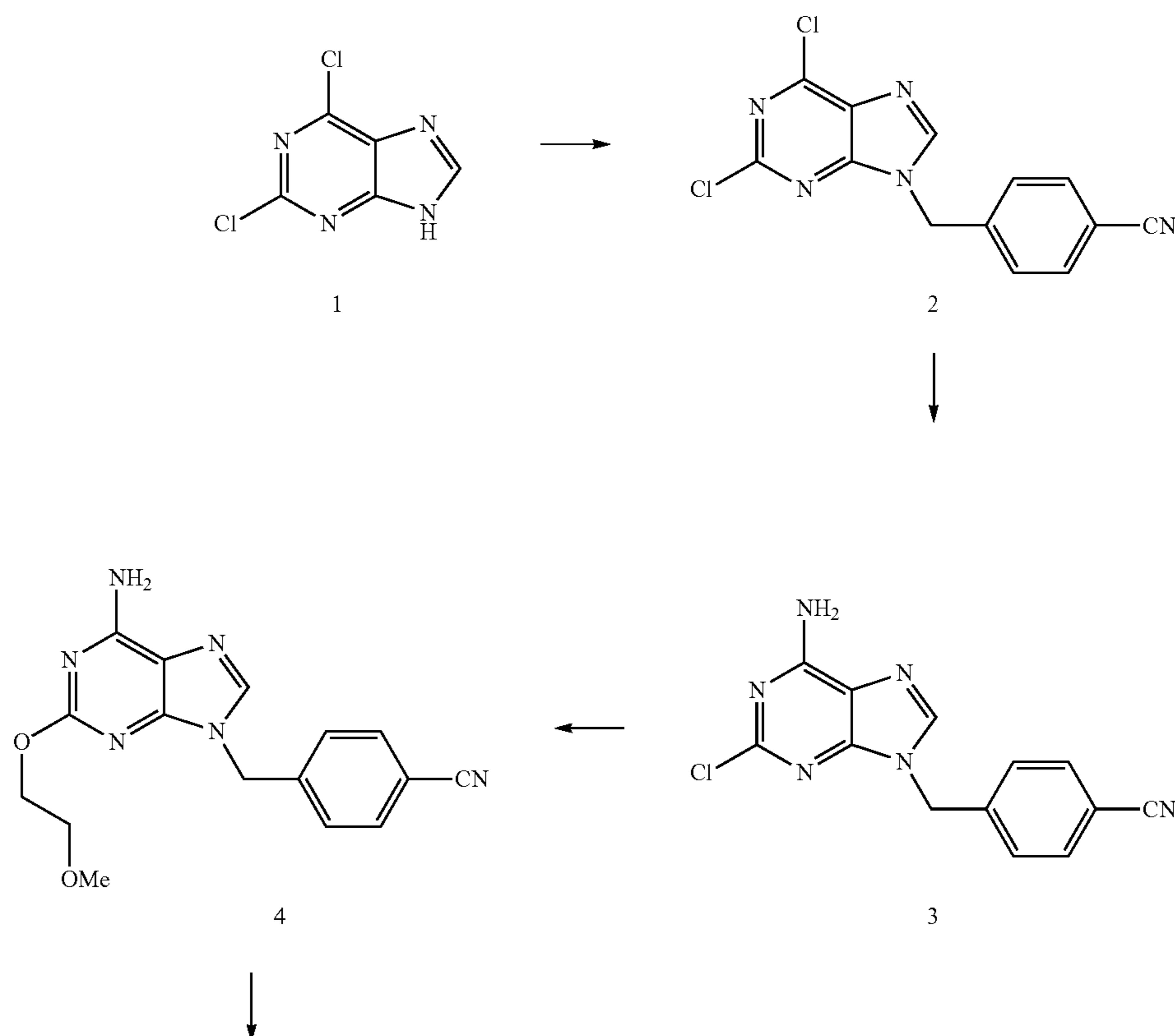
Scheme 1
