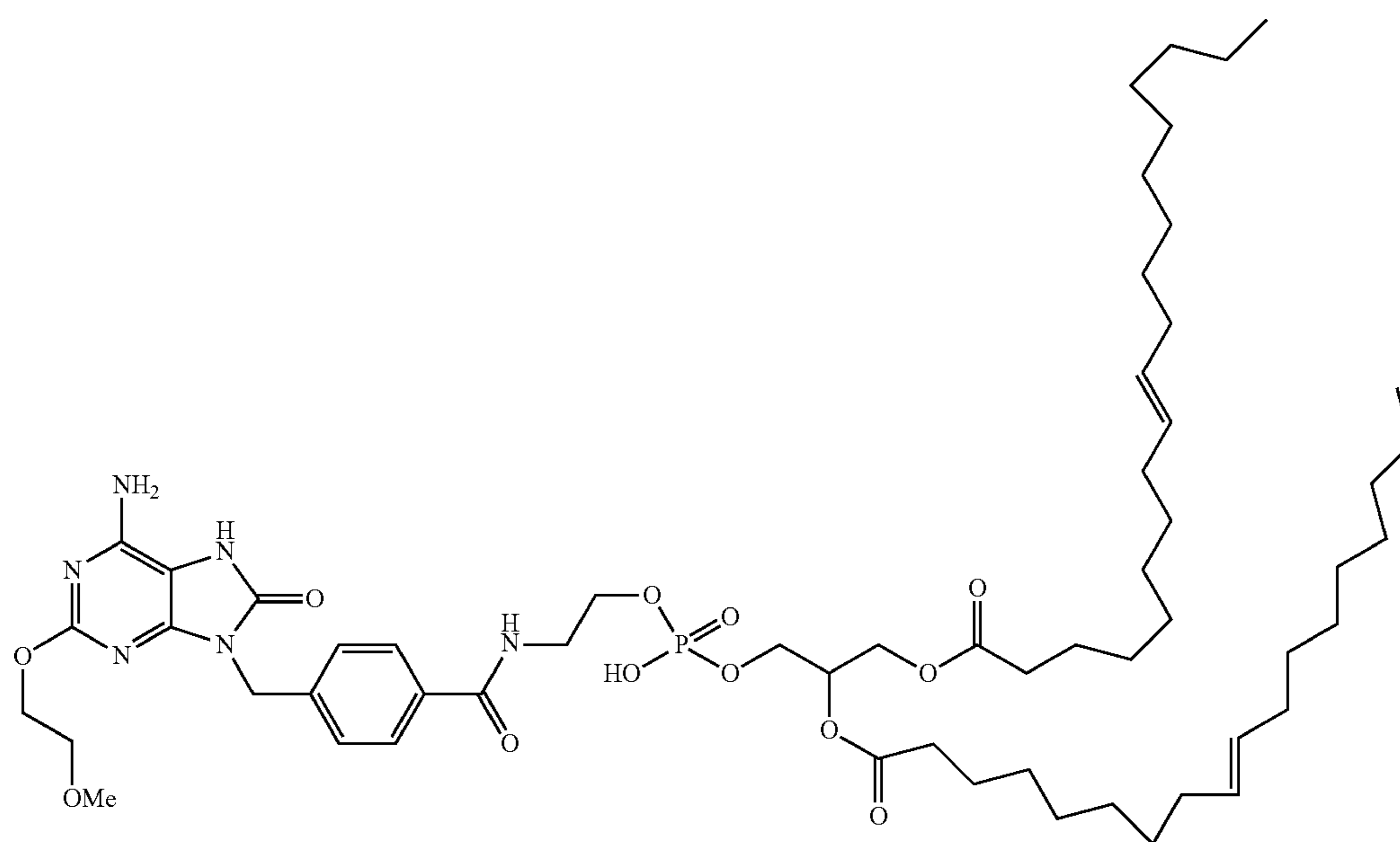
Compound A
