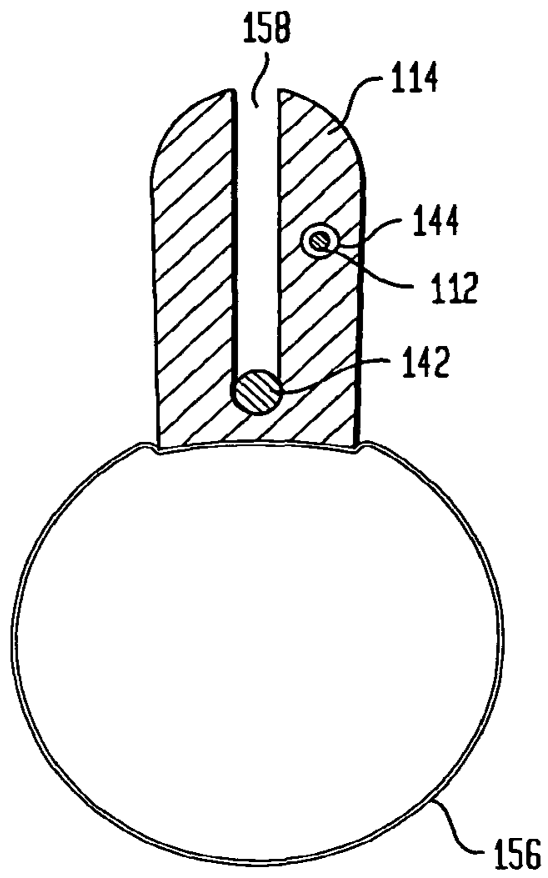
FIG. 5 SECTION A/A'
