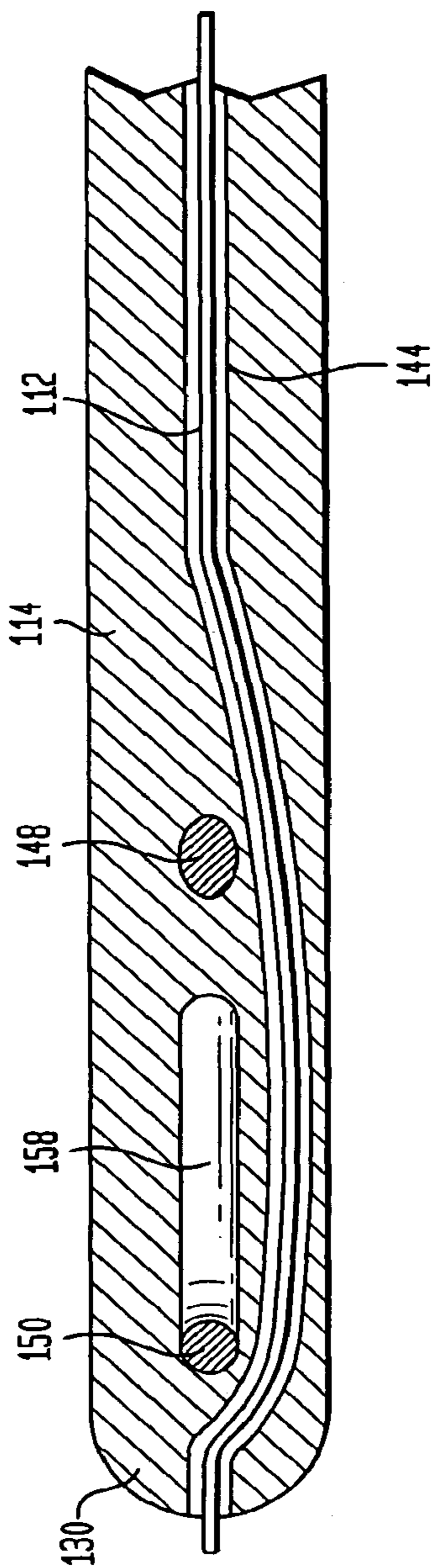
FIG. 8 SECTION D/D'
