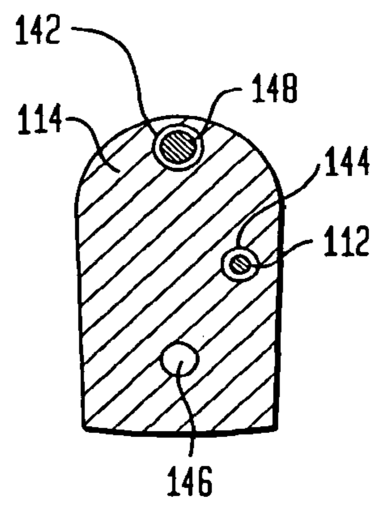
FIG. 7 SECTION C/C'
