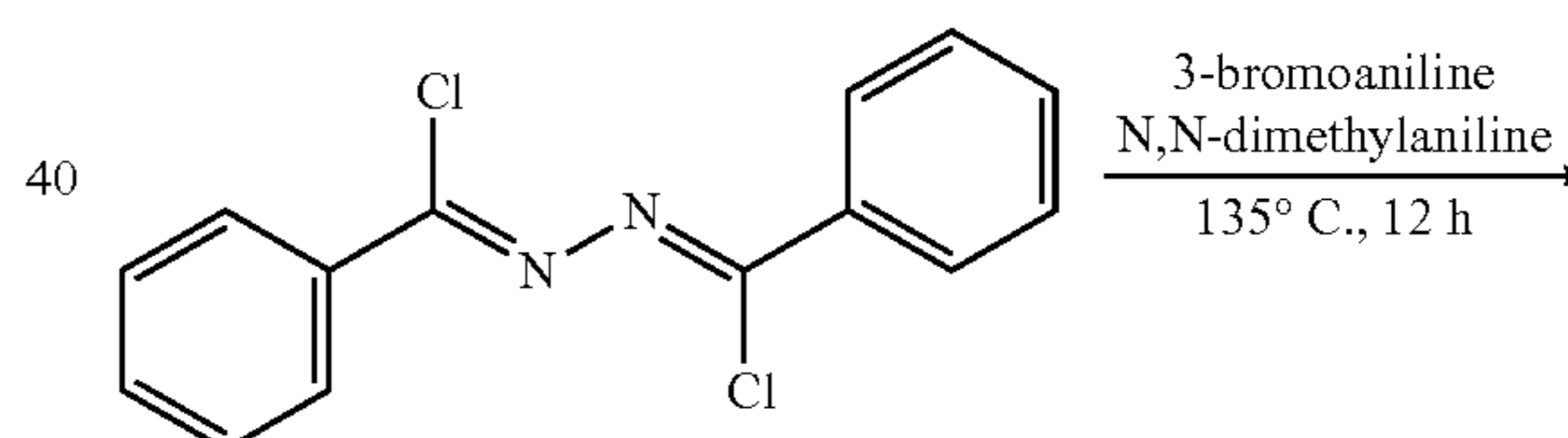
Compound (3)
