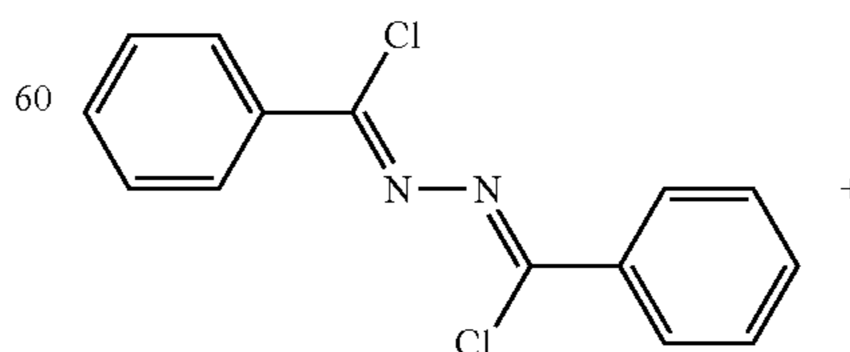
Compound (3)
