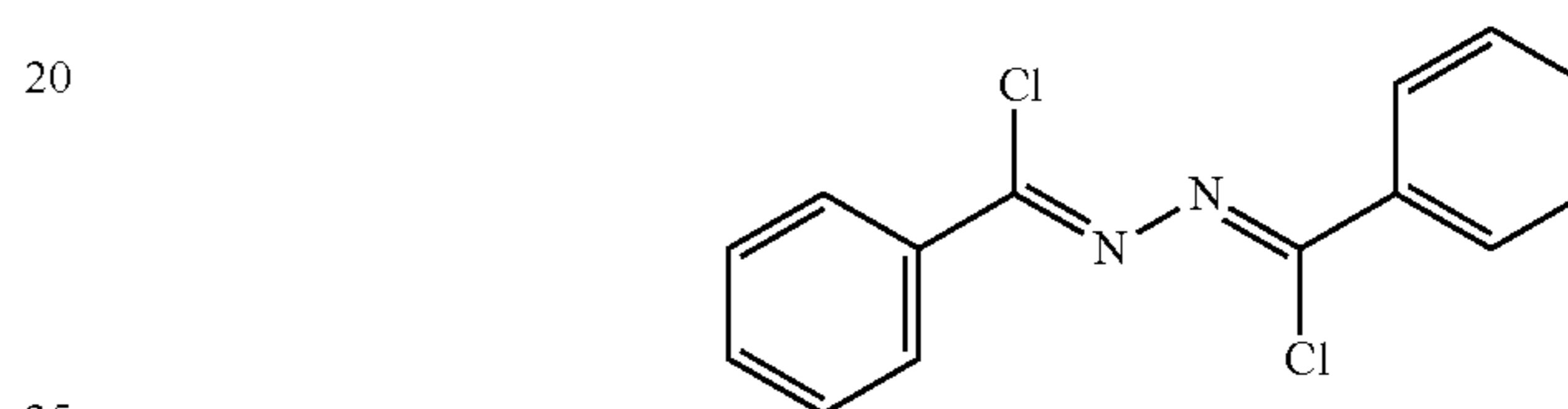
Compound (3)
