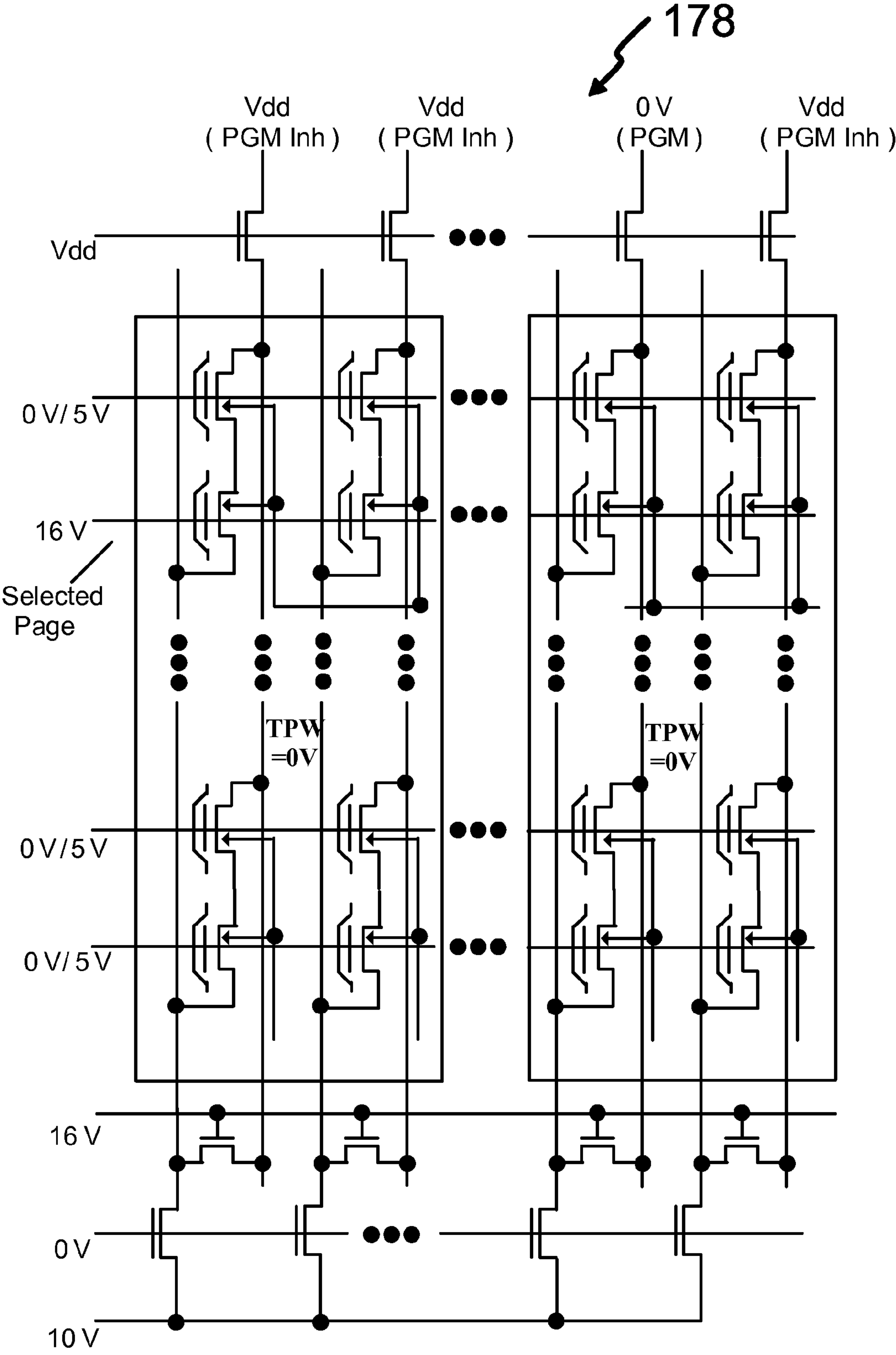
Fig. 13D
