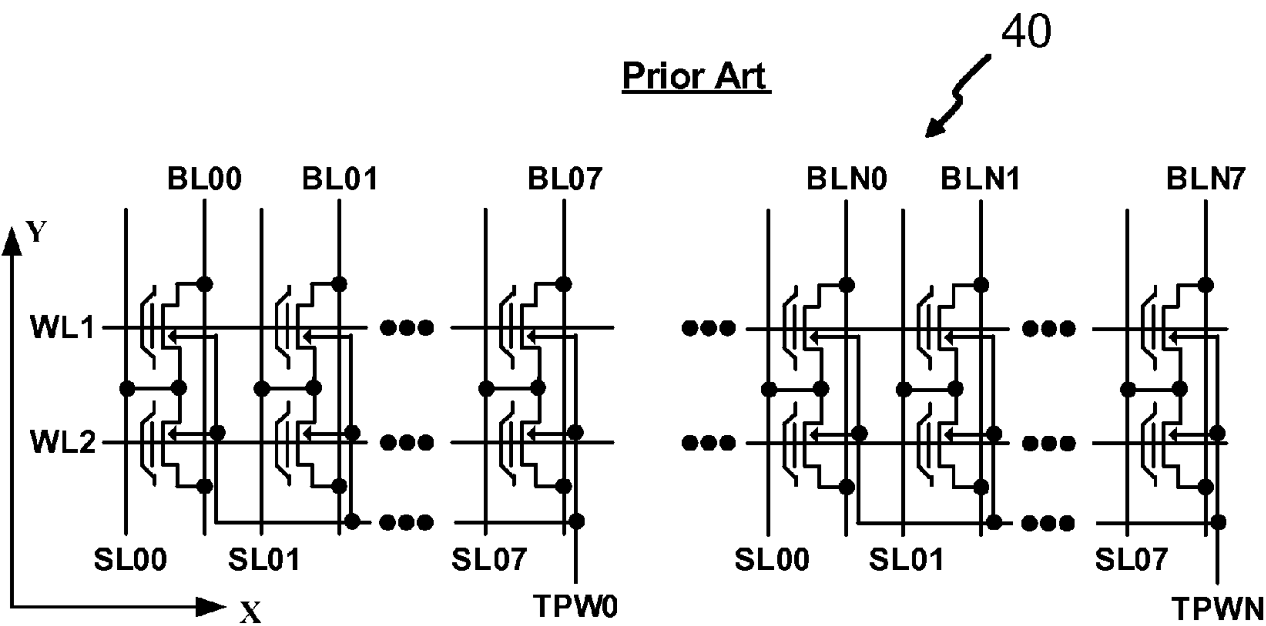
Fig. 2 Prior Art 50
